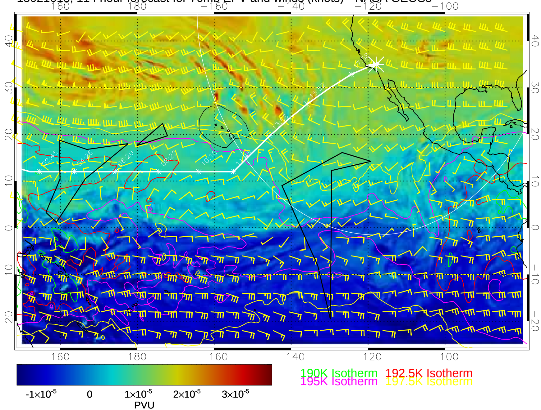
15021618, 114 hour forecast for 70mb EPV and winds (knots)-- NASA GEOS5
