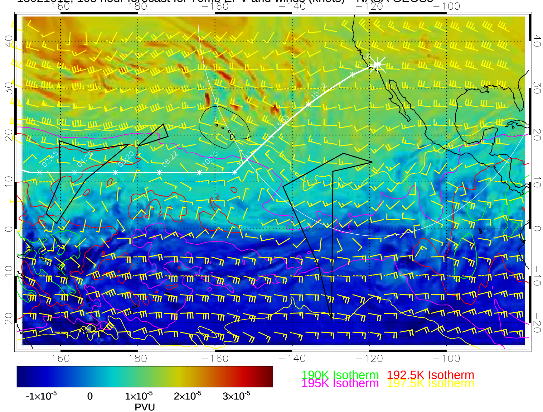
15021612, 108 hour forecast for 70mb EPV and winds (knots)-- NASA GEOS5
