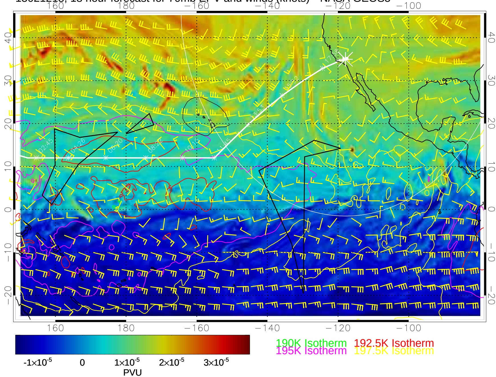
15021218, 18 hour forecast for 70mb EPV and winds (knots)-- NASA GEOS5
