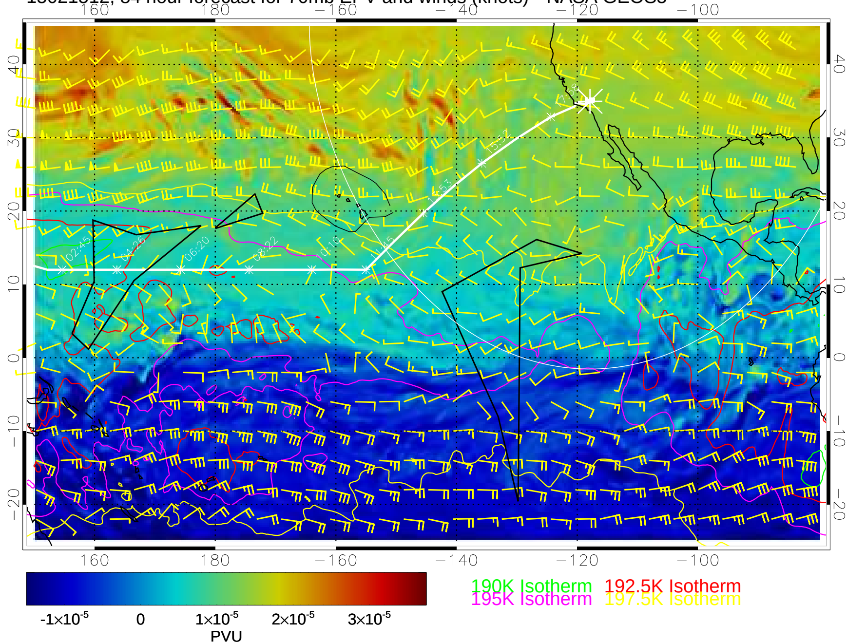
15021512, 84 hour forecast for 70mb EPV and winds (knots)-- NASA GEOS5
