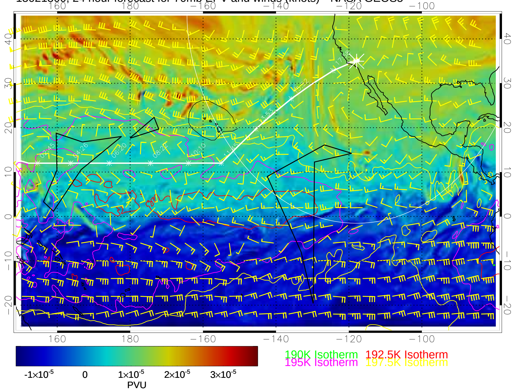
15021300, 24 hour forecast for 70mb EPV and winds (knots)-- NASA GEOS5
