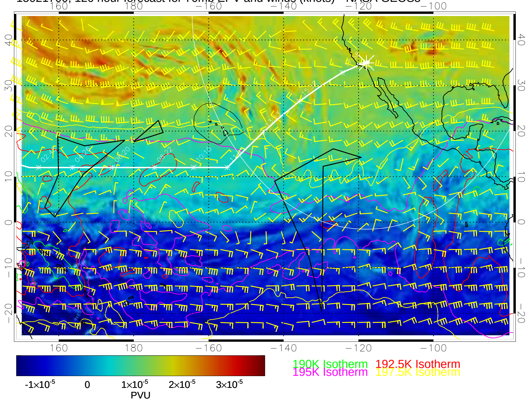
15021700, 120 hour forecast for 70mb EPV and winds (knots)-- NASA GEOS5
