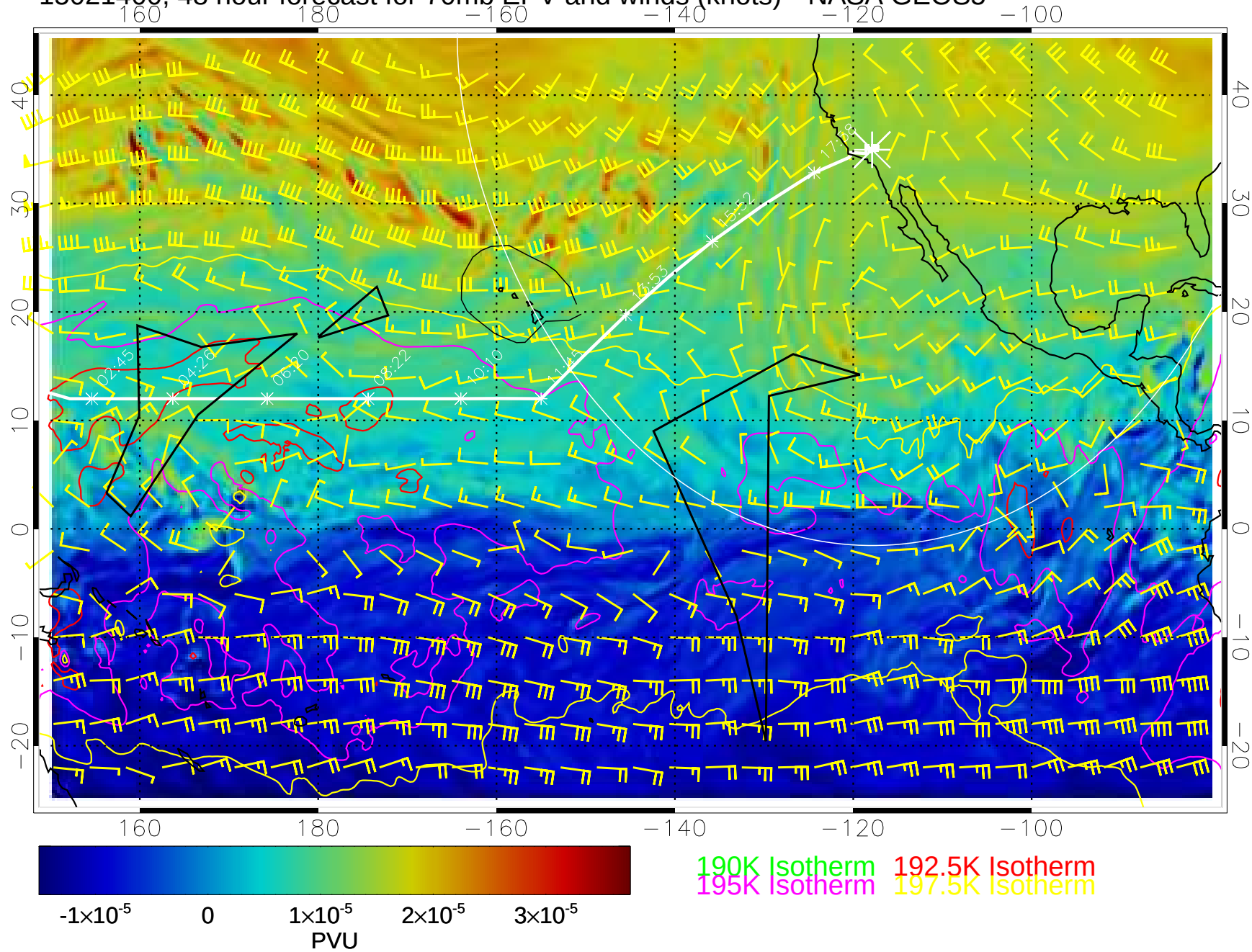
15021400, 48 hour forecast for 70mb EPV and winds (knots)-- NASA GEOS5
