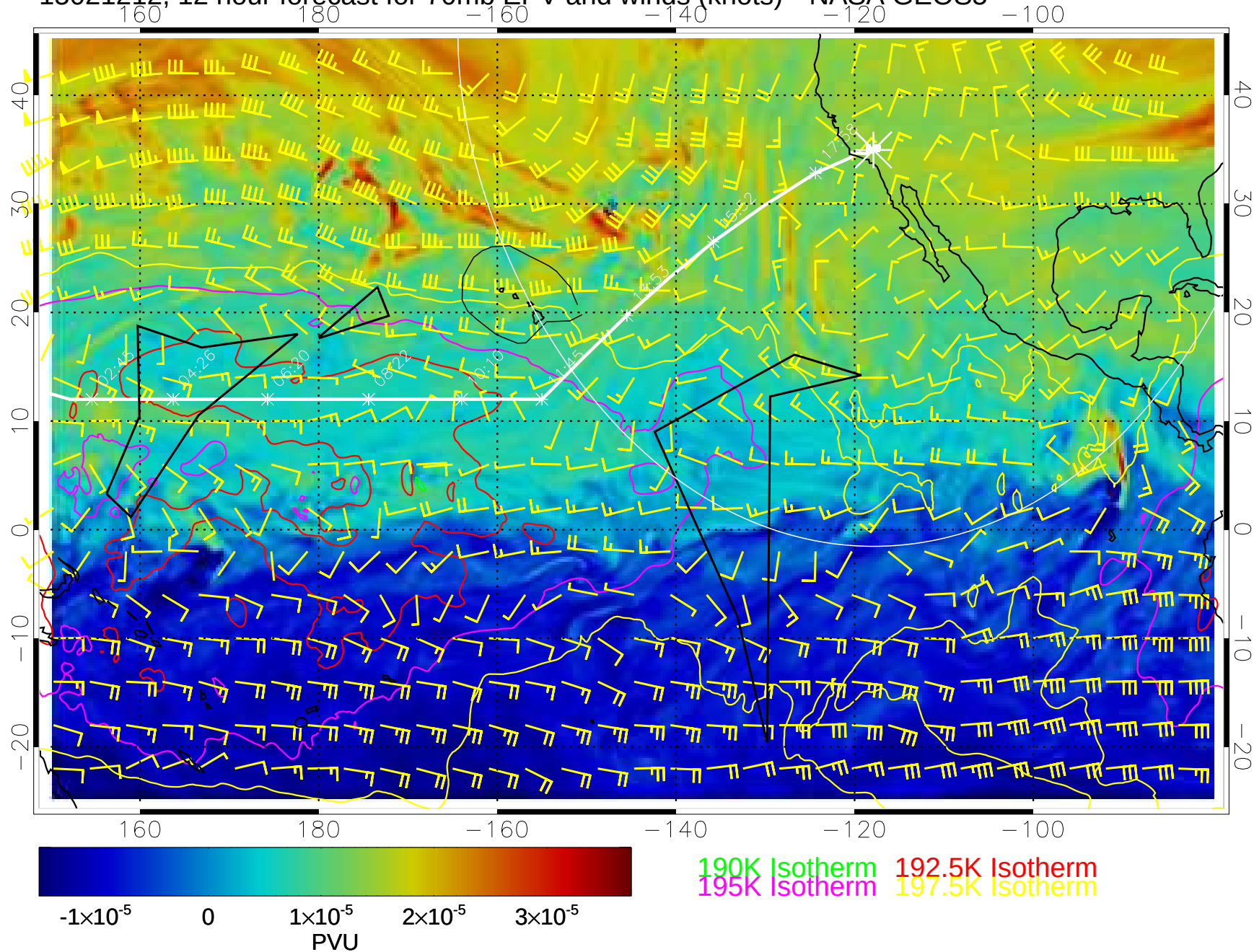
15021212, 12 hour forecast for 70mb EPV and winds (knots)-- NASA GEOS5
