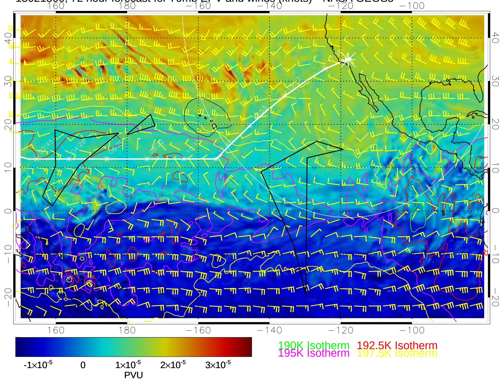
15021500, 72 hour forecast for 70mb EPV and winds (knots)-- NASA GEOS5
