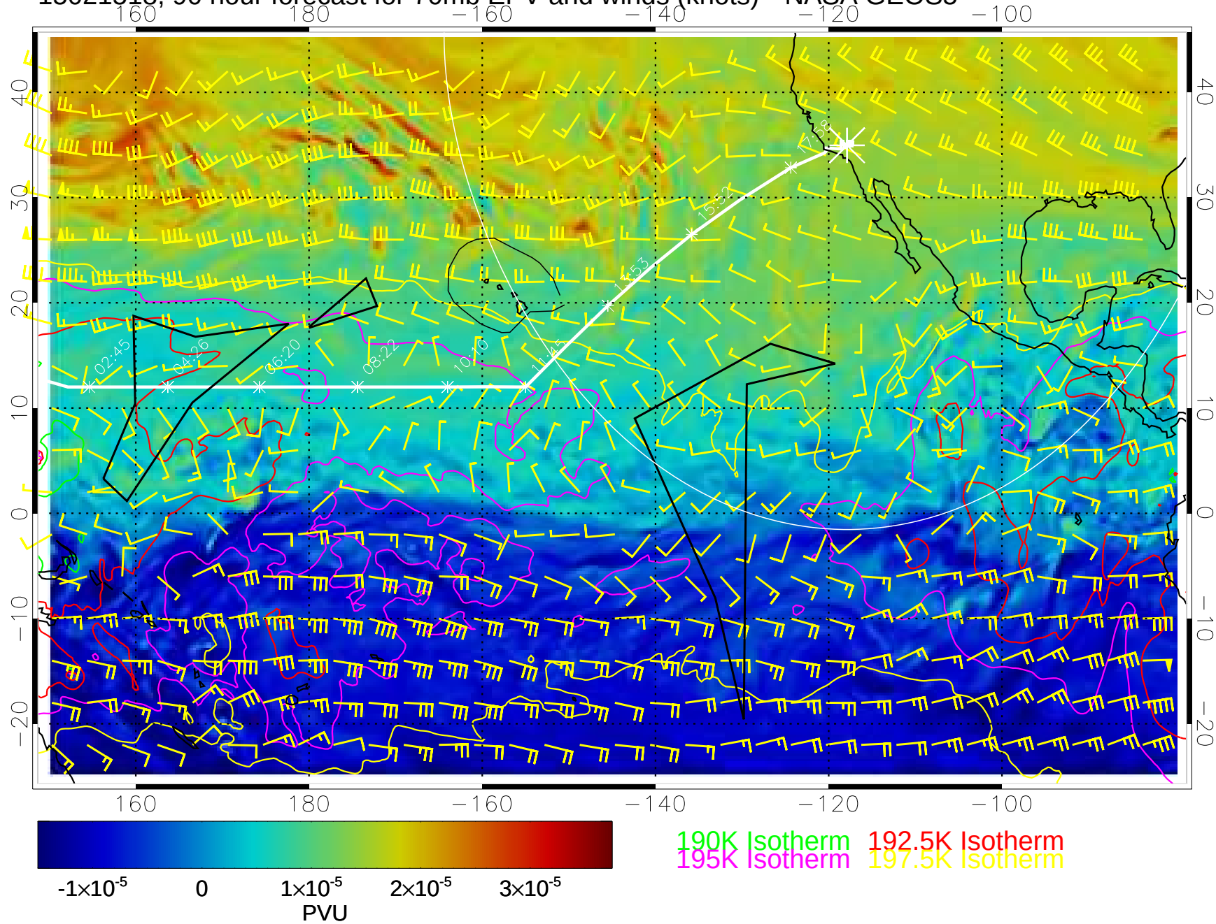
15021518, 90 hour forecast for 70mb EPV and winds (knots)-- NASA GEOS5
