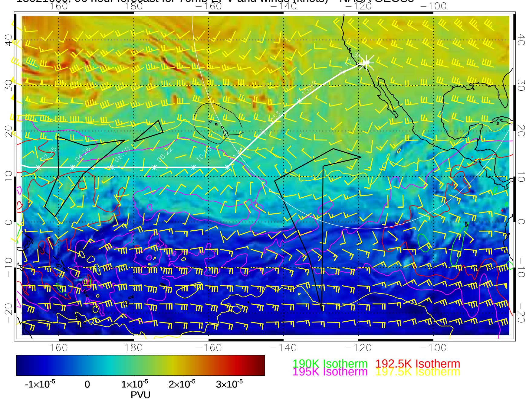
15021600, 96 hour forecast for 70mb EPV and winds (knots)-- NASA GEOS5
