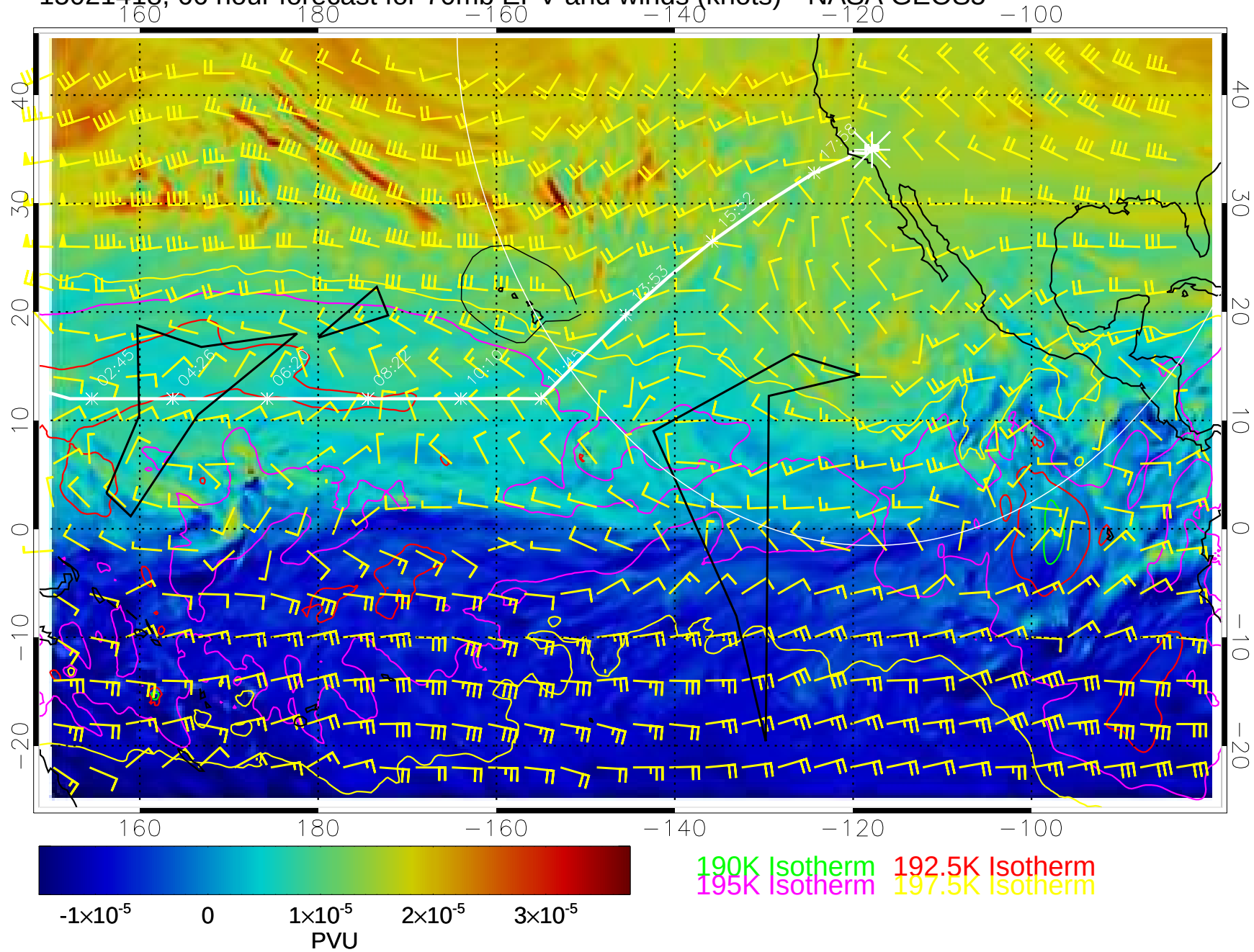
15021418, 66 hour forecast for 70mb EPV and winds (knots)-- NASA GEOS5
