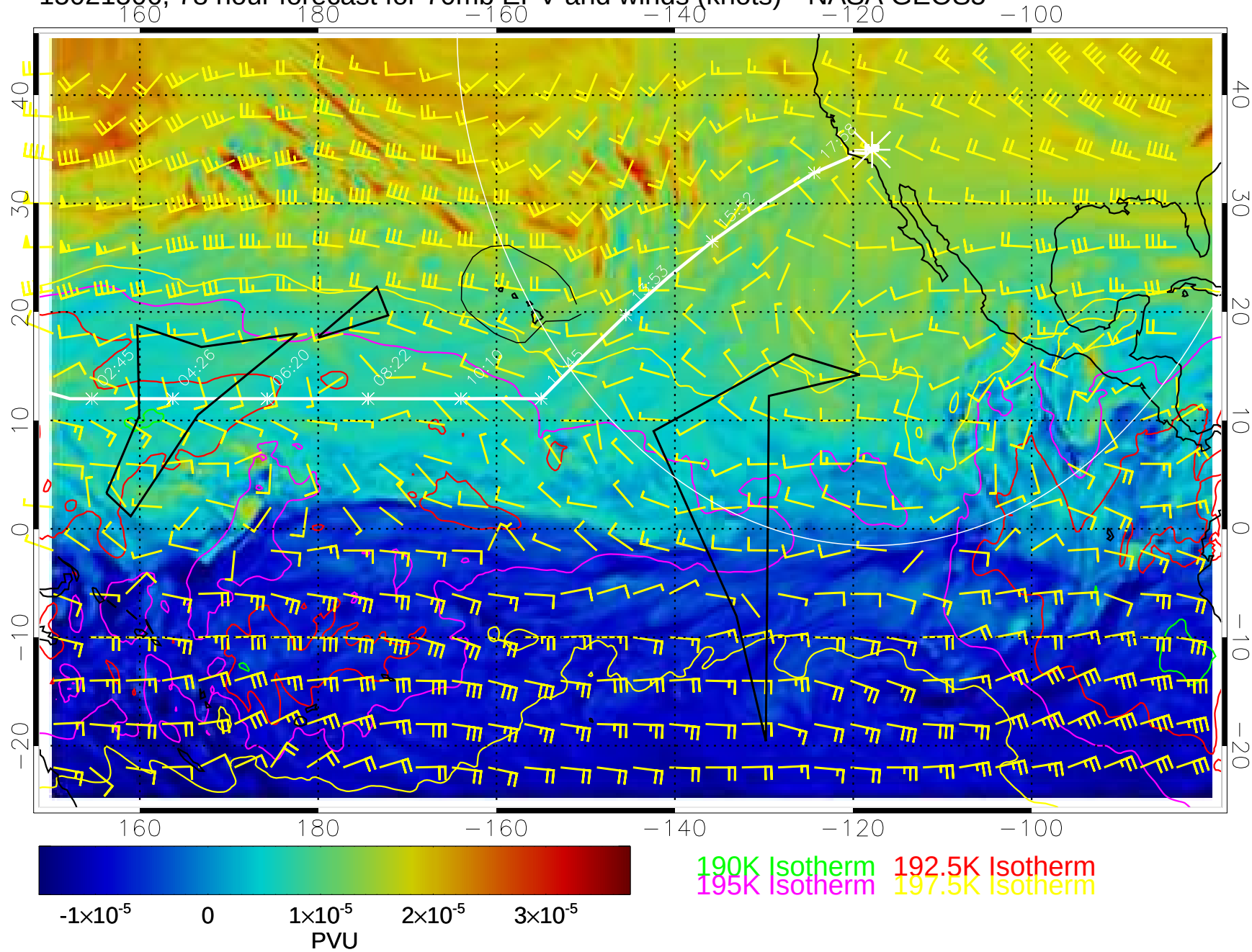
15021506, 78 hour forecast for 70mb EPV and winds (knots)-- NASA GEOS5
