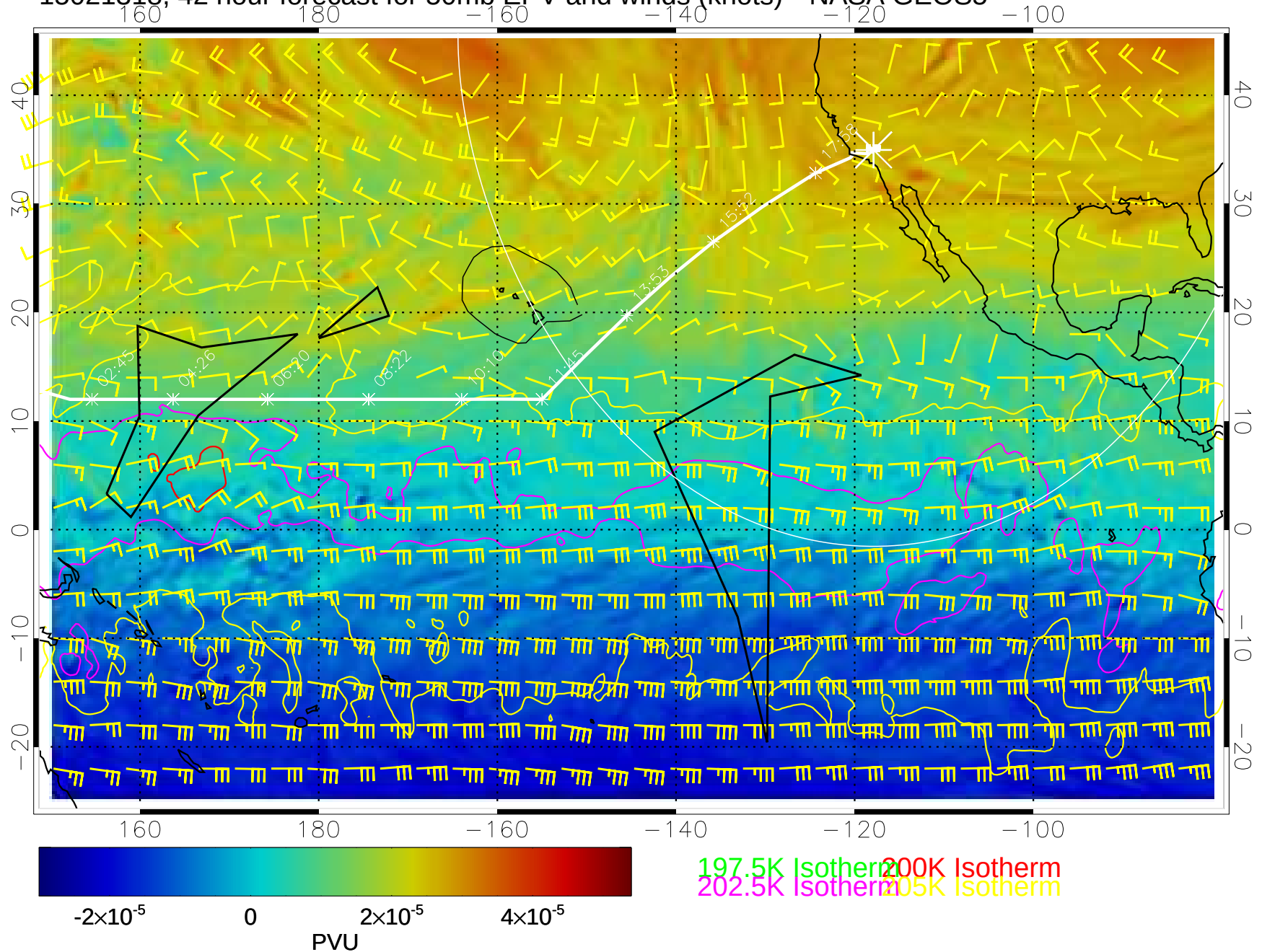
15021318, 42 hour forecast for 50mb EPV and winds (knots)-- NASA GEOS5
