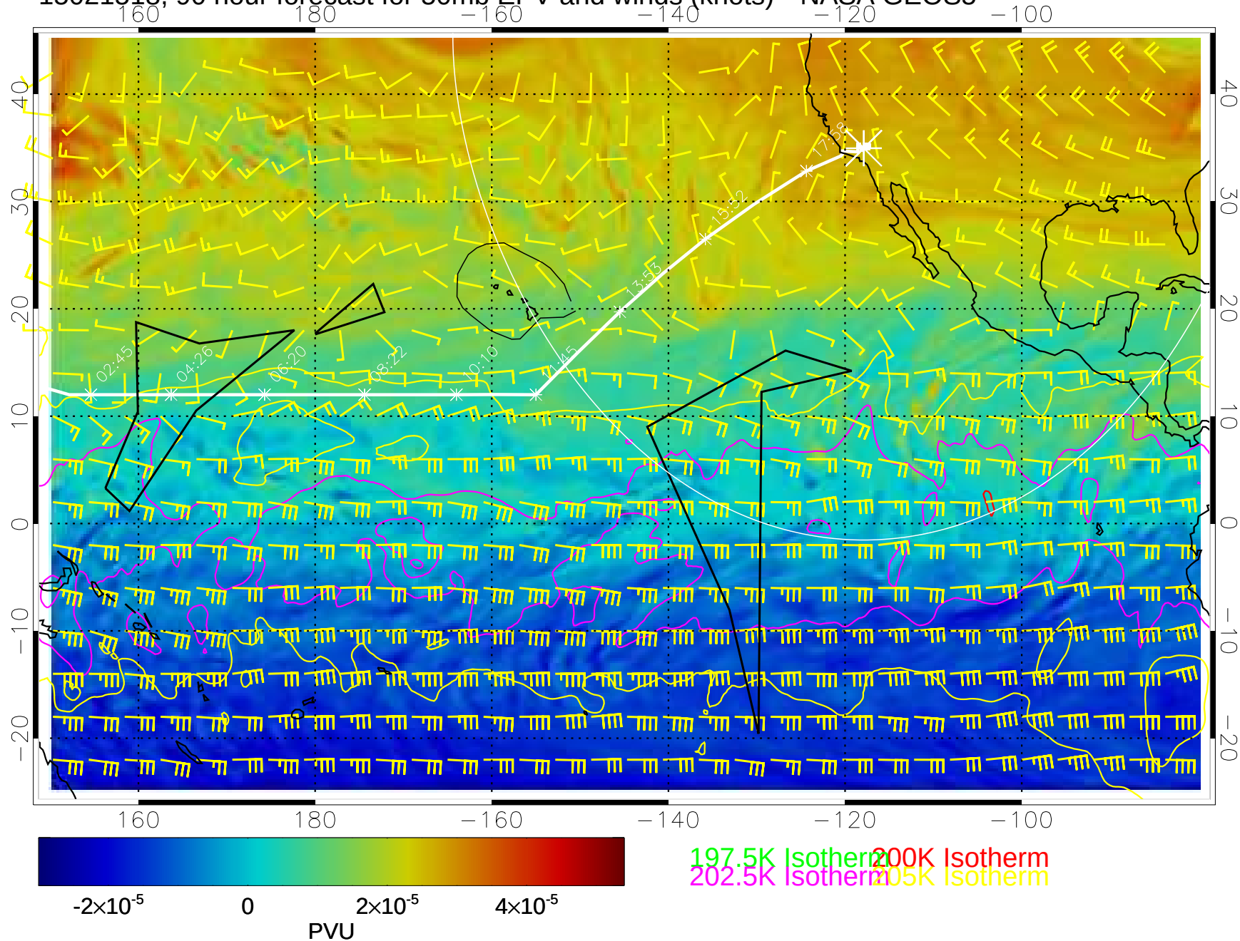
15021518, 90 hour forecast for 50mb EPV and winds (knots)-- NASA GEOS5
