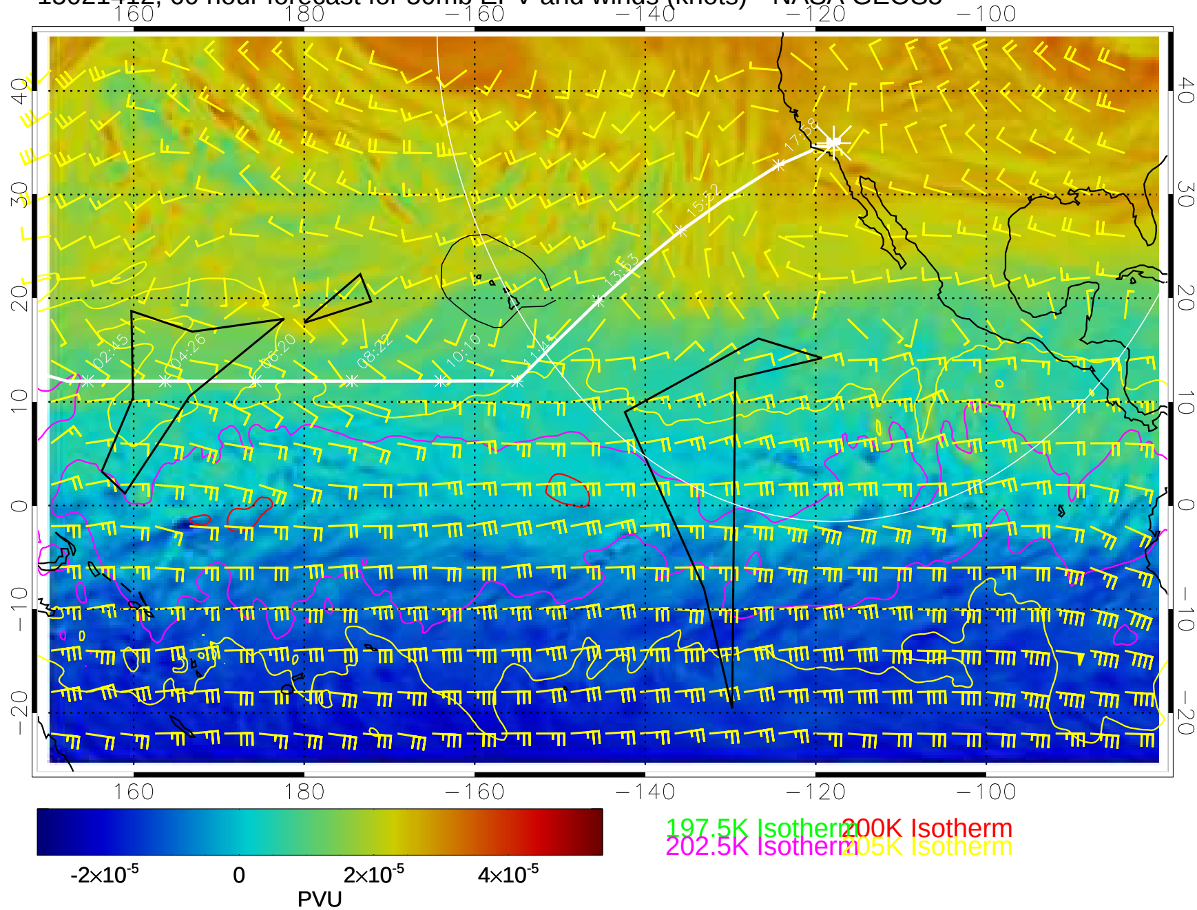
15021412, 60 hour forecast for 50mb EPV and winds (knots)-- NASA GEOS5
