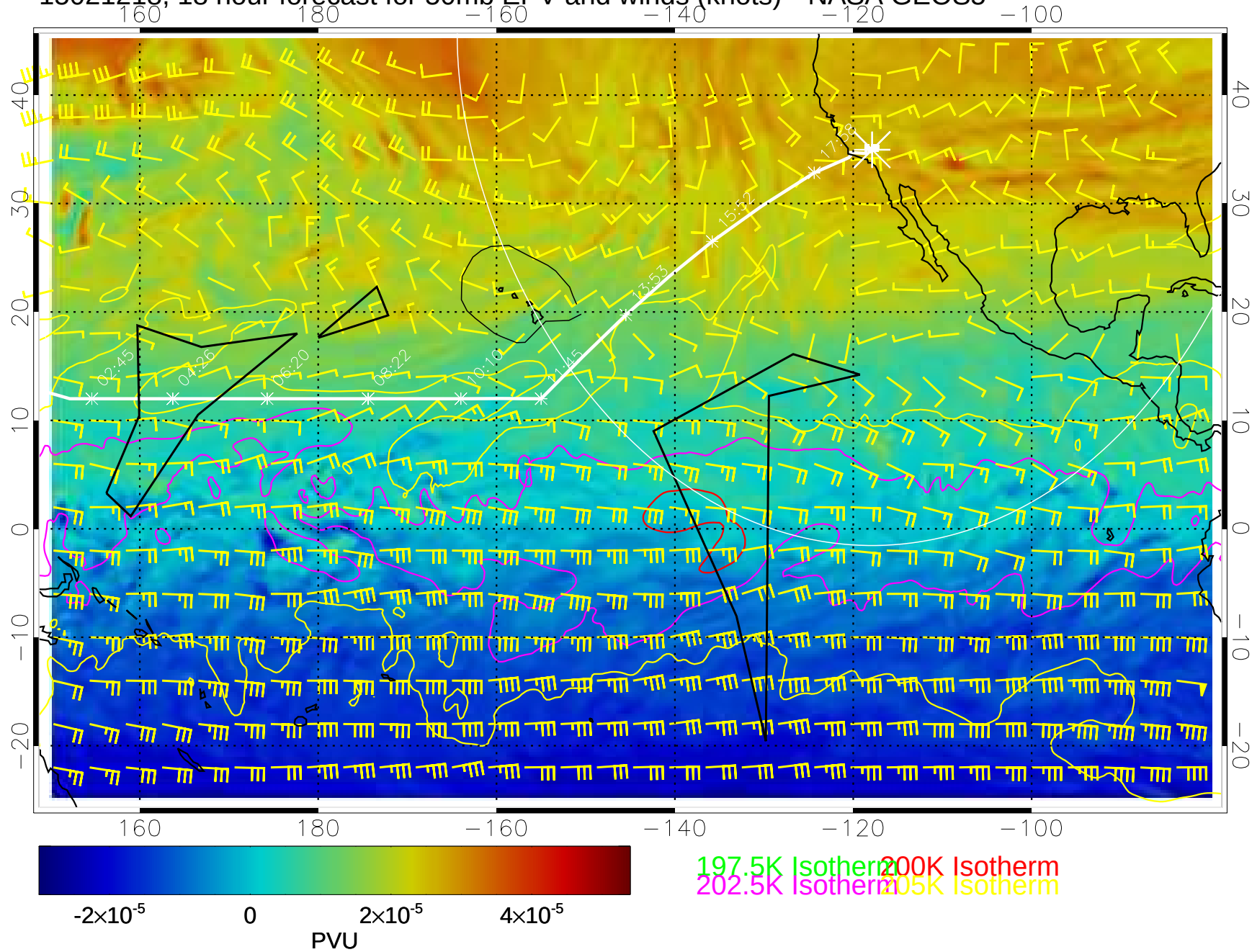
15021218, 18 hour forecast for 50mb EPV and winds (knots)-- NASA GEOS5
