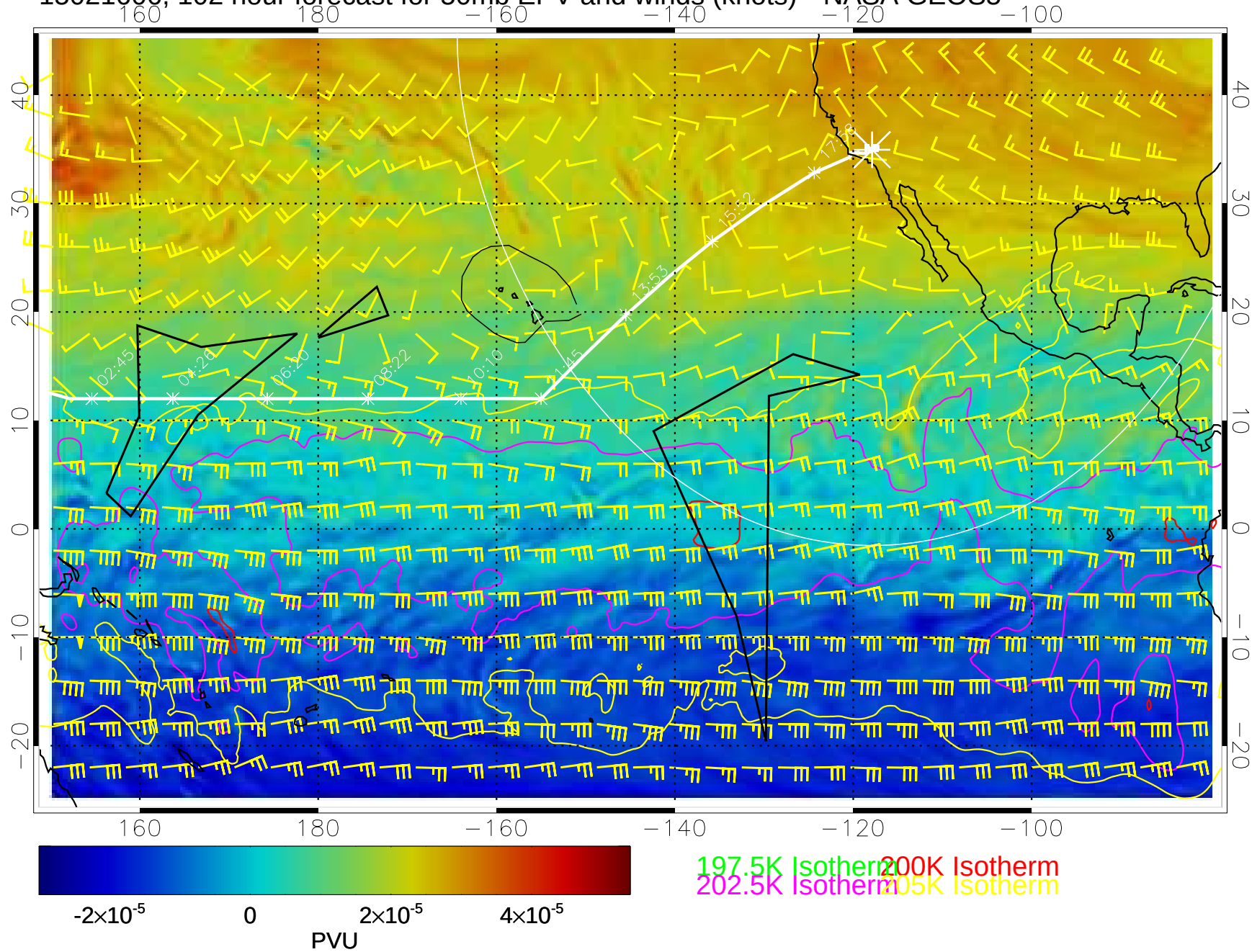
15021606, 102 hour forecast for 50mb EPV and winds (knots)-- NASA GEOS5
