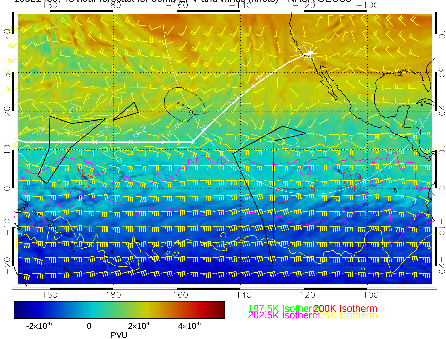
15021400, 48 hour forecast for 50mb EPV and winds (knots)-- NASA GEOS5
