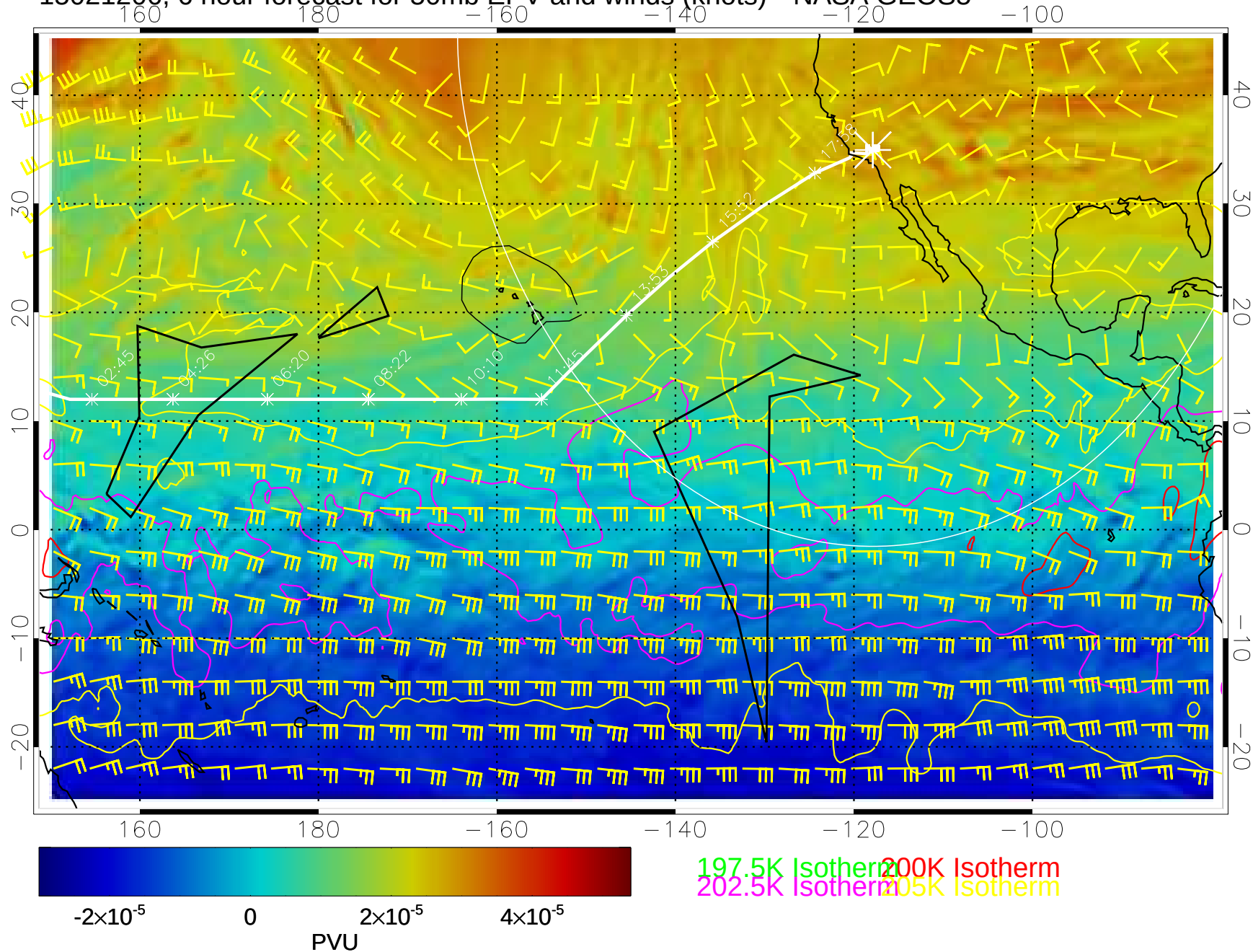
15021206, 6 hour forecast for 50mb EPV and winds (knots)-- NASA GEOS5
