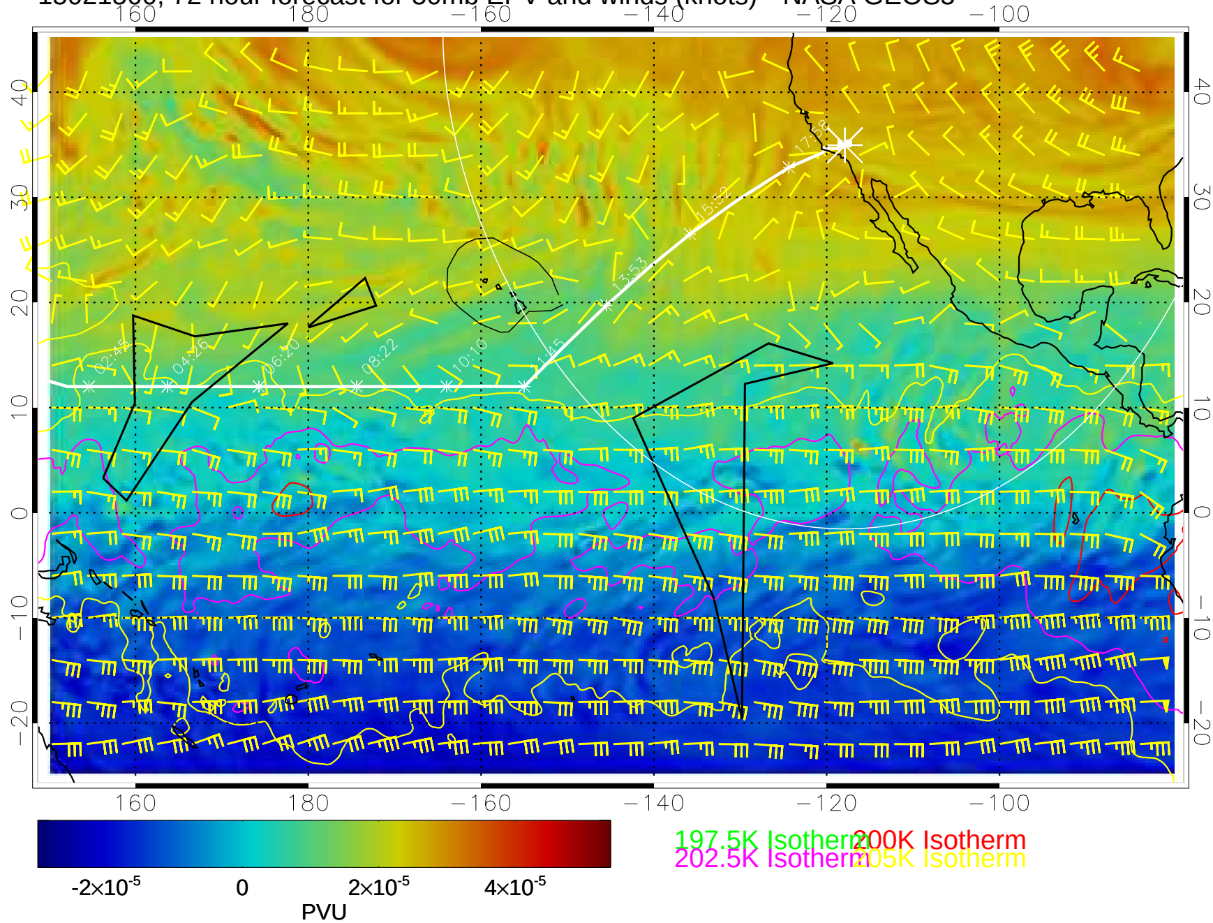
15021500, 72 hour forecast for 50mb EPV and winds (knots)-- NASA GEOS5
