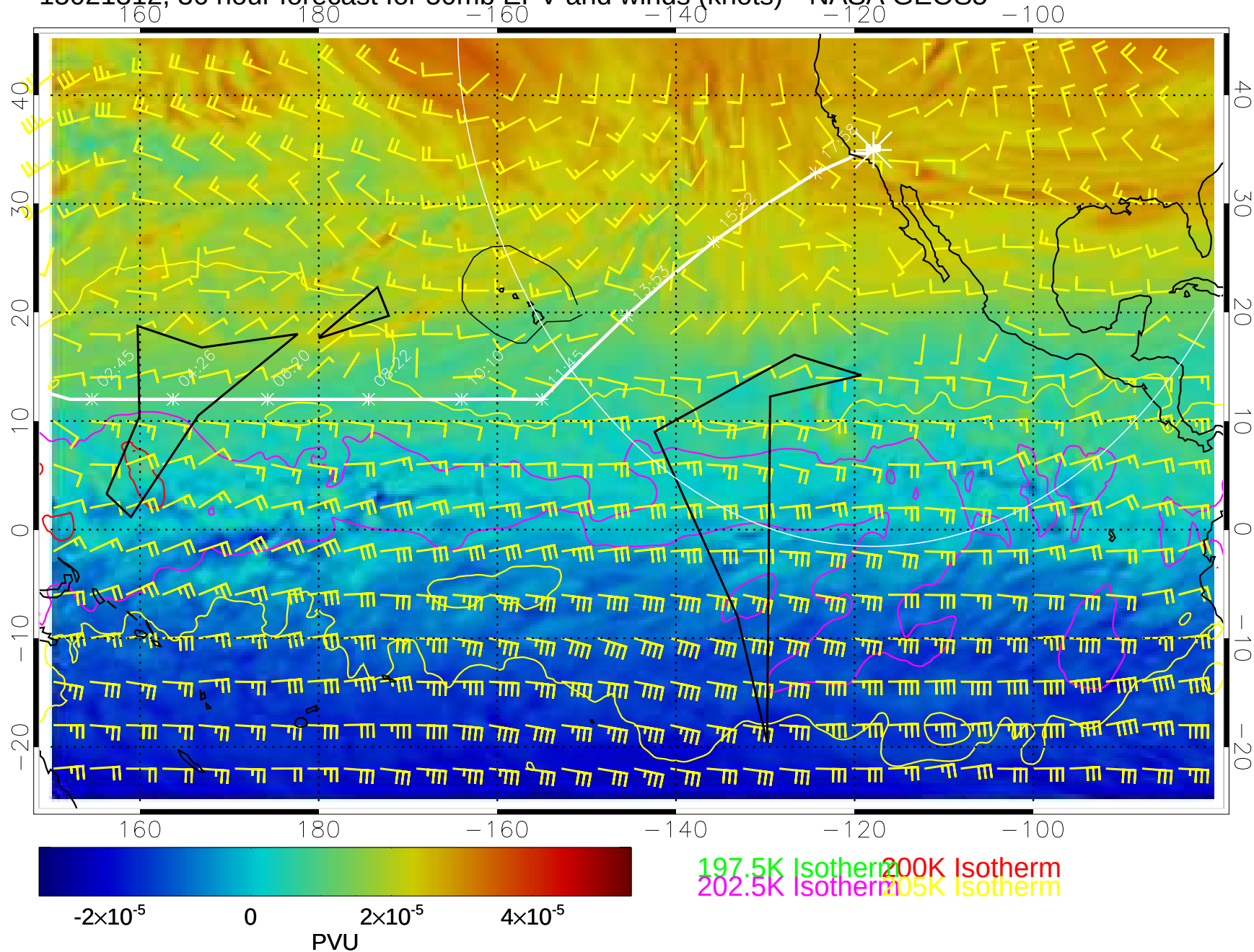
15021312, 36 hour forecast for 50mb EPV and winds (knots)-- NASA GEOS5
