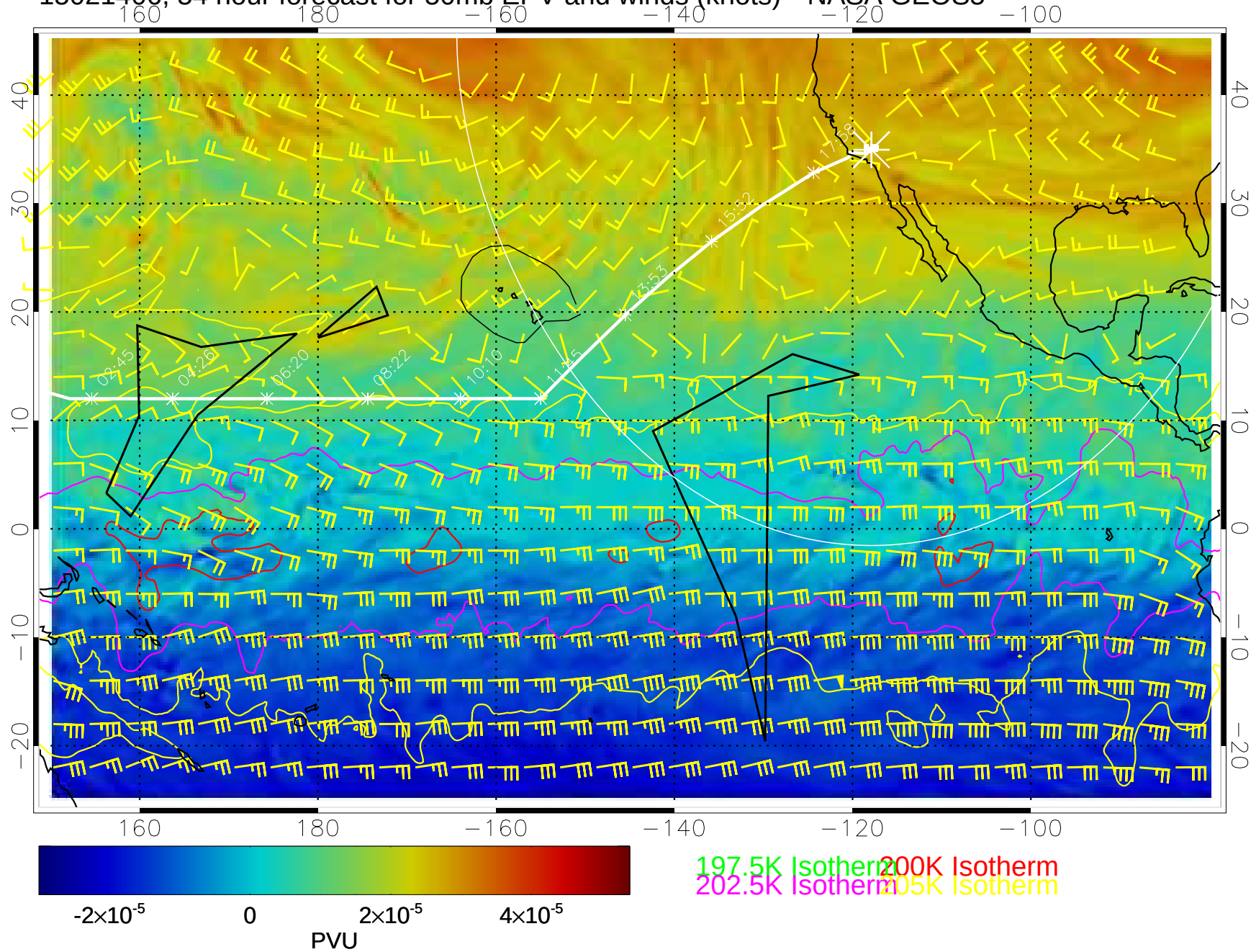
15021406, 54 hour forecast for 50mb EPV and winds (knots)-- NASA GEOS5
