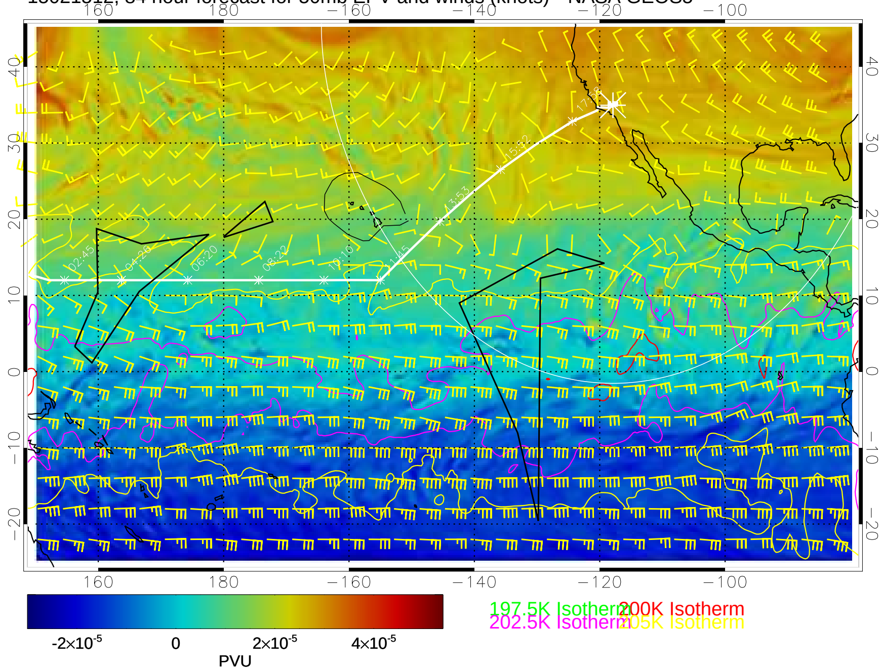
15021512, 84 hour forecast for 50mb EPV and winds (knots)-- NASA GEOS5
