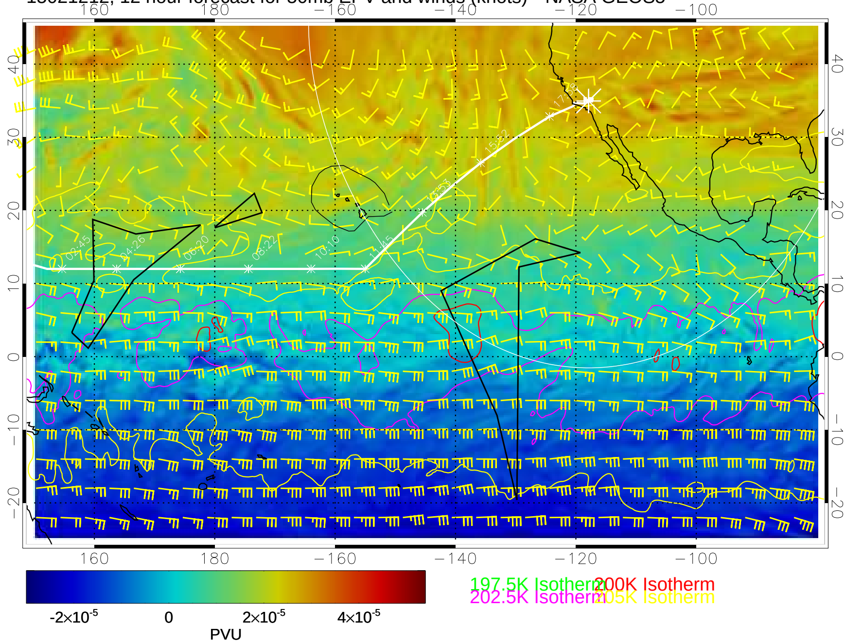
15021212, 12 hour forecast for 50mb EPV and winds (knots)-- NASA GEOS5
