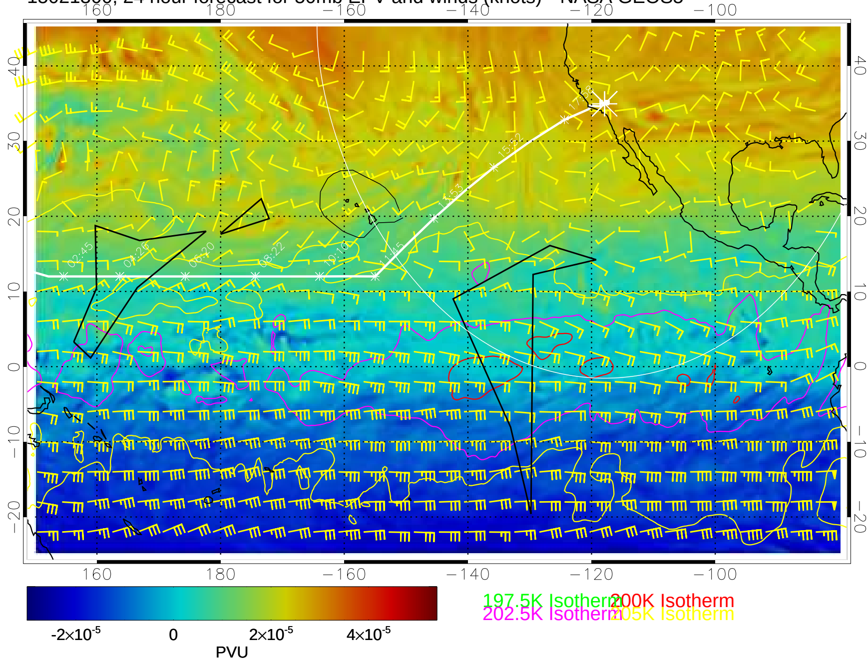
15021300, 24 hour forecast for 50mb EPV and winds (knots)-- NASA GEOS5
