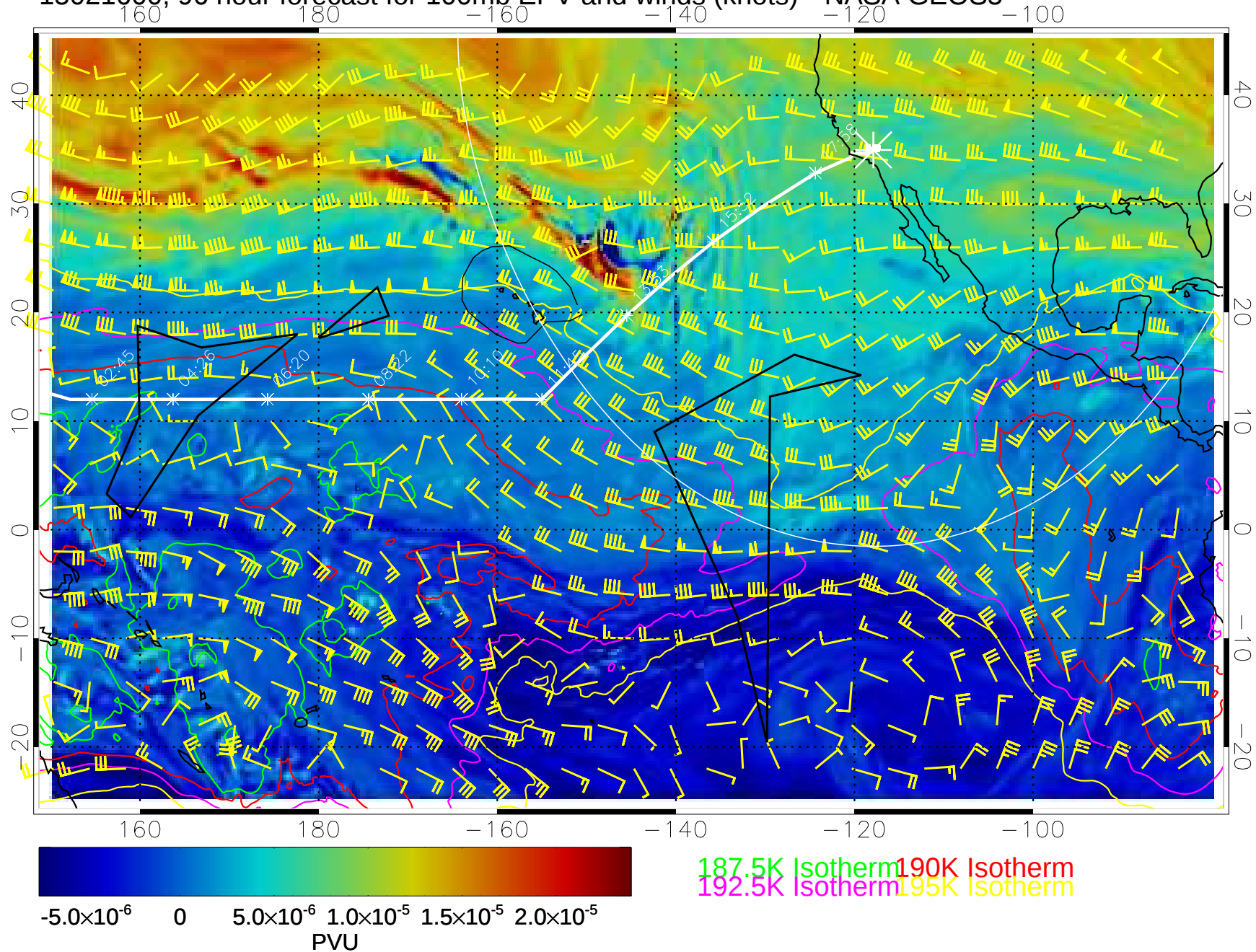
15021600, 96 hour forecast for 100mb EPV and winds (knots)-- NASA GEOS5
