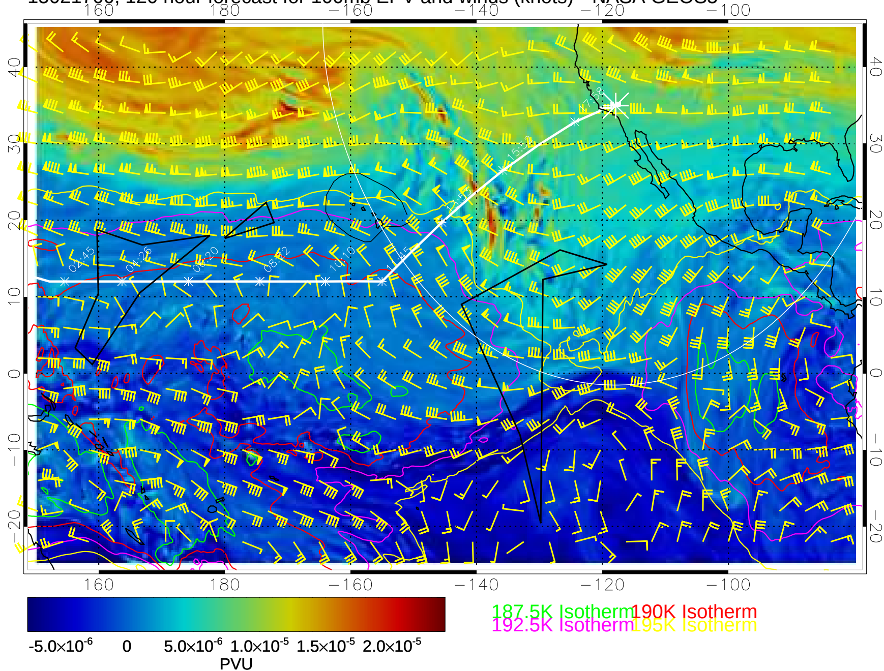
15021700, 120 hour forecast for 100mb EPV and winds (knots)-- NASA GEOS5
