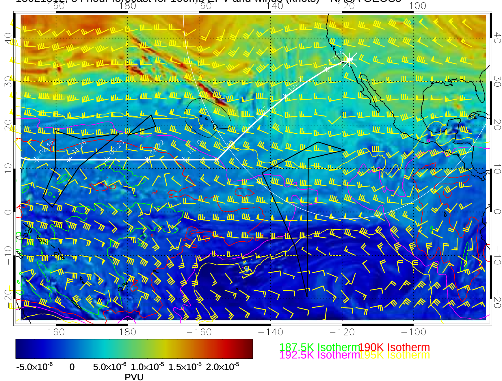
15021512, 84 hour forecast for 100mb EPV and winds (knots)-- NASA GEOS5
