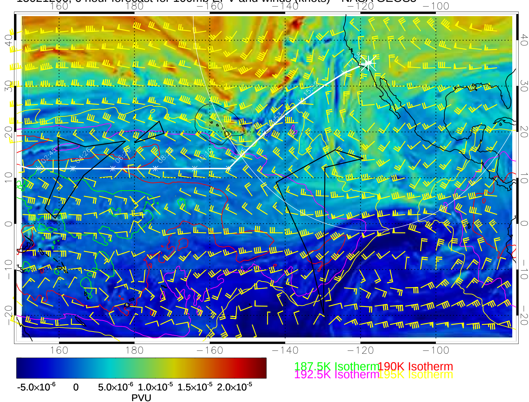
15021206, 6 hour forecast for 100mb EPV and winds (knots)-- NASA GEOS5
