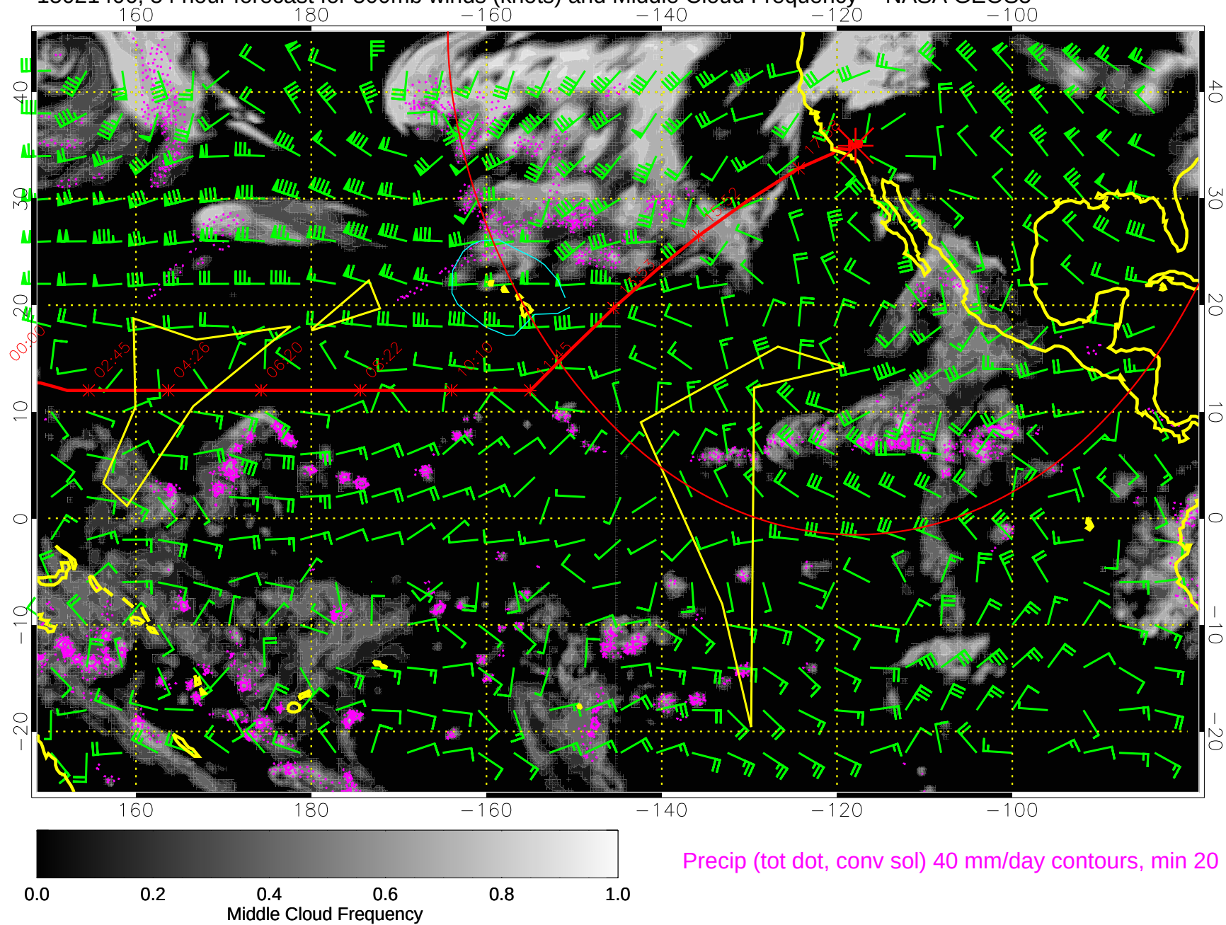
15021406, 54 hour forecast for 500mb winds (knots) and Middle Cloud Frequency -- NASA GEOS5
