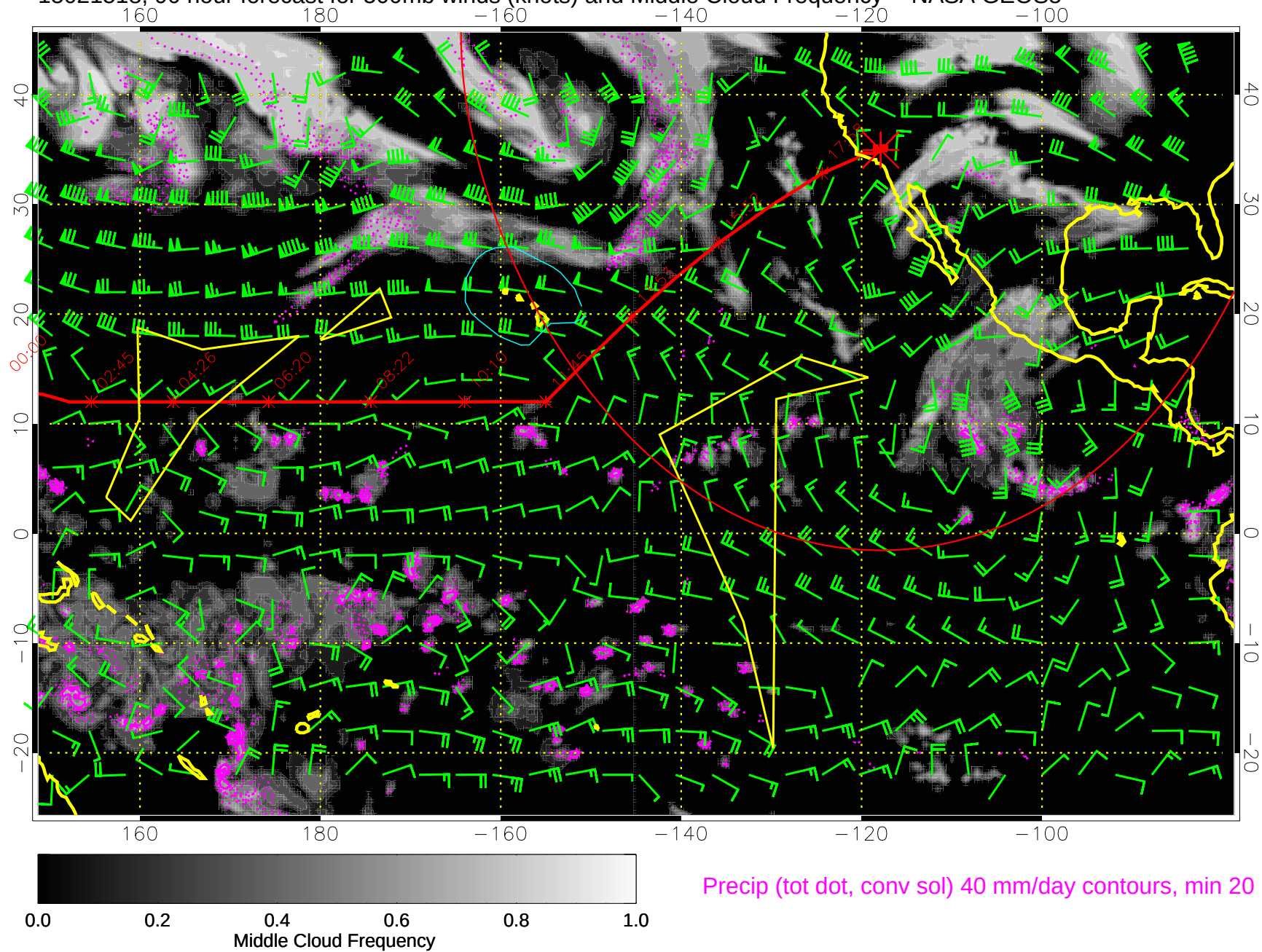
15021518, 90 hour forecast for 500mb winds (knots) and Middle Cloud Frequency -- NASA GEOS5
