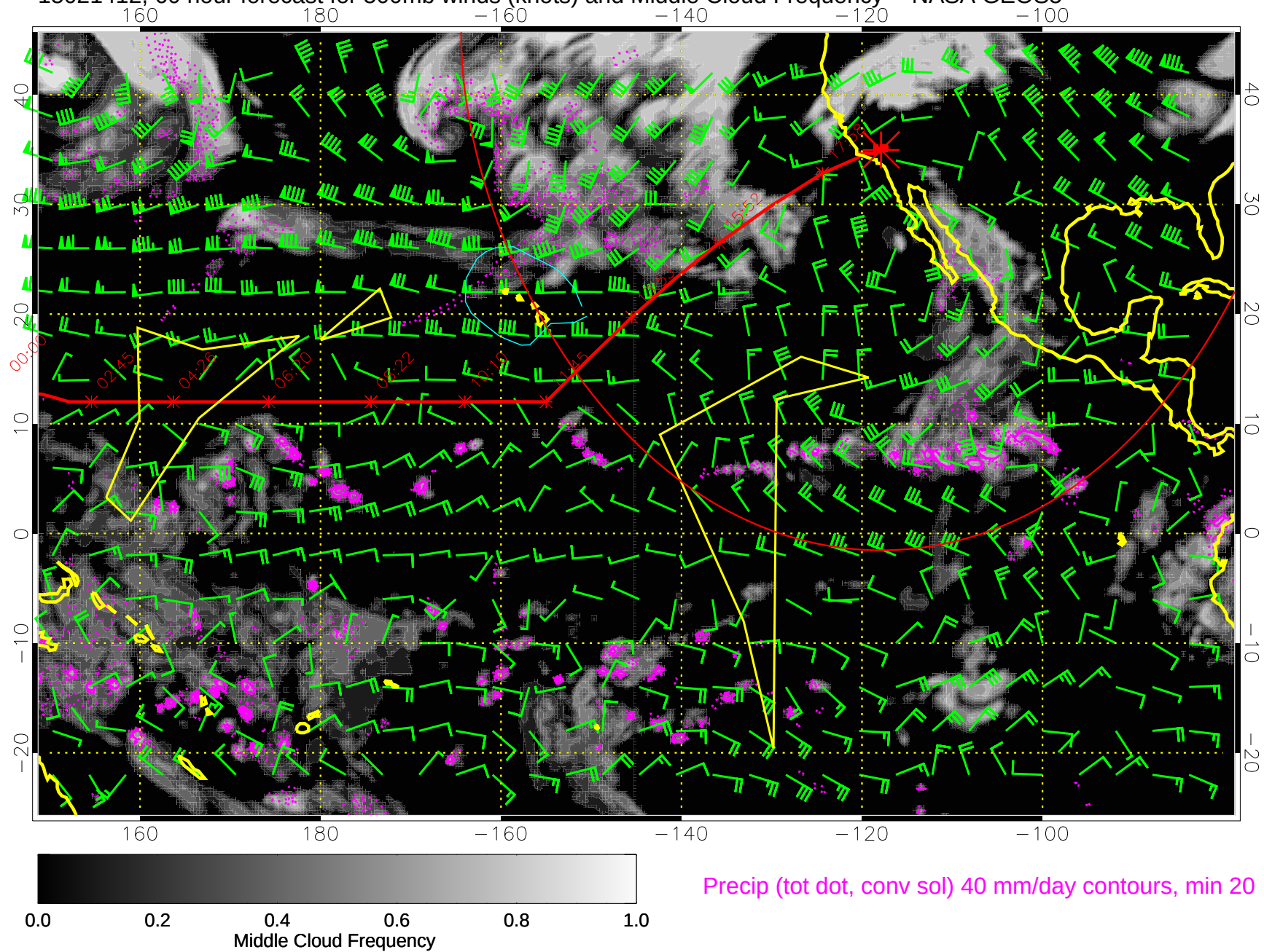
15021412, 60 hour forecast for 500mb winds (knots) and Middle Cloud Frequency -- NASA GEOS5
