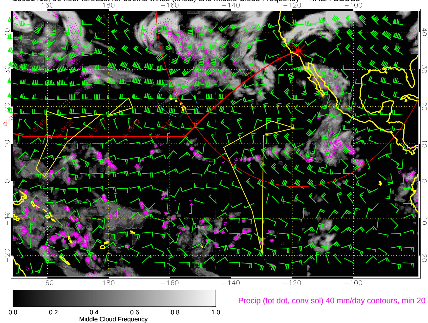
15021418, 66 hour forecast for 500mb winds (knots) and Middle Cloud Frequency -- NASA GEOS5
