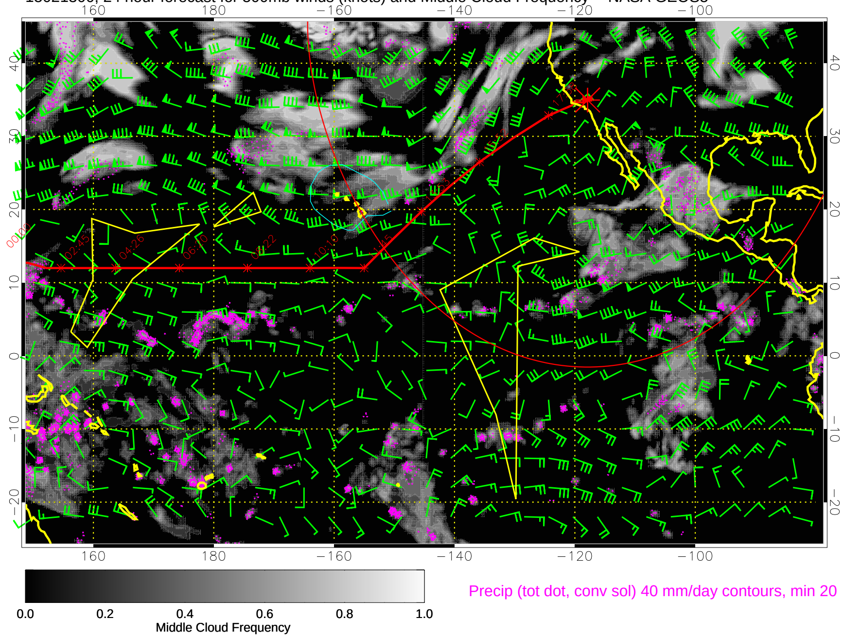
15021300, 24 hour forecast for 500mb winds (knots) and Middle Cloud Frequency -- NASA GEOS5
