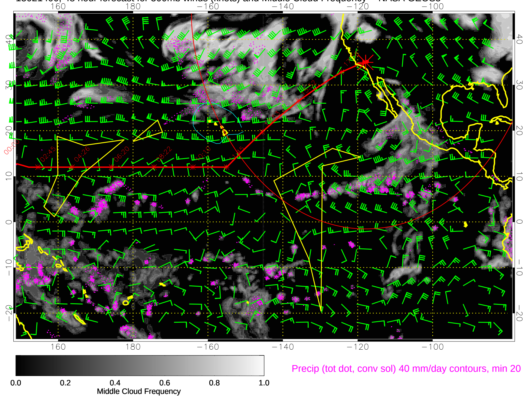
15021400, 48 hour forecast for 500mb winds (knots) and Middle Cloud Frequency -- NASA GEOS5
