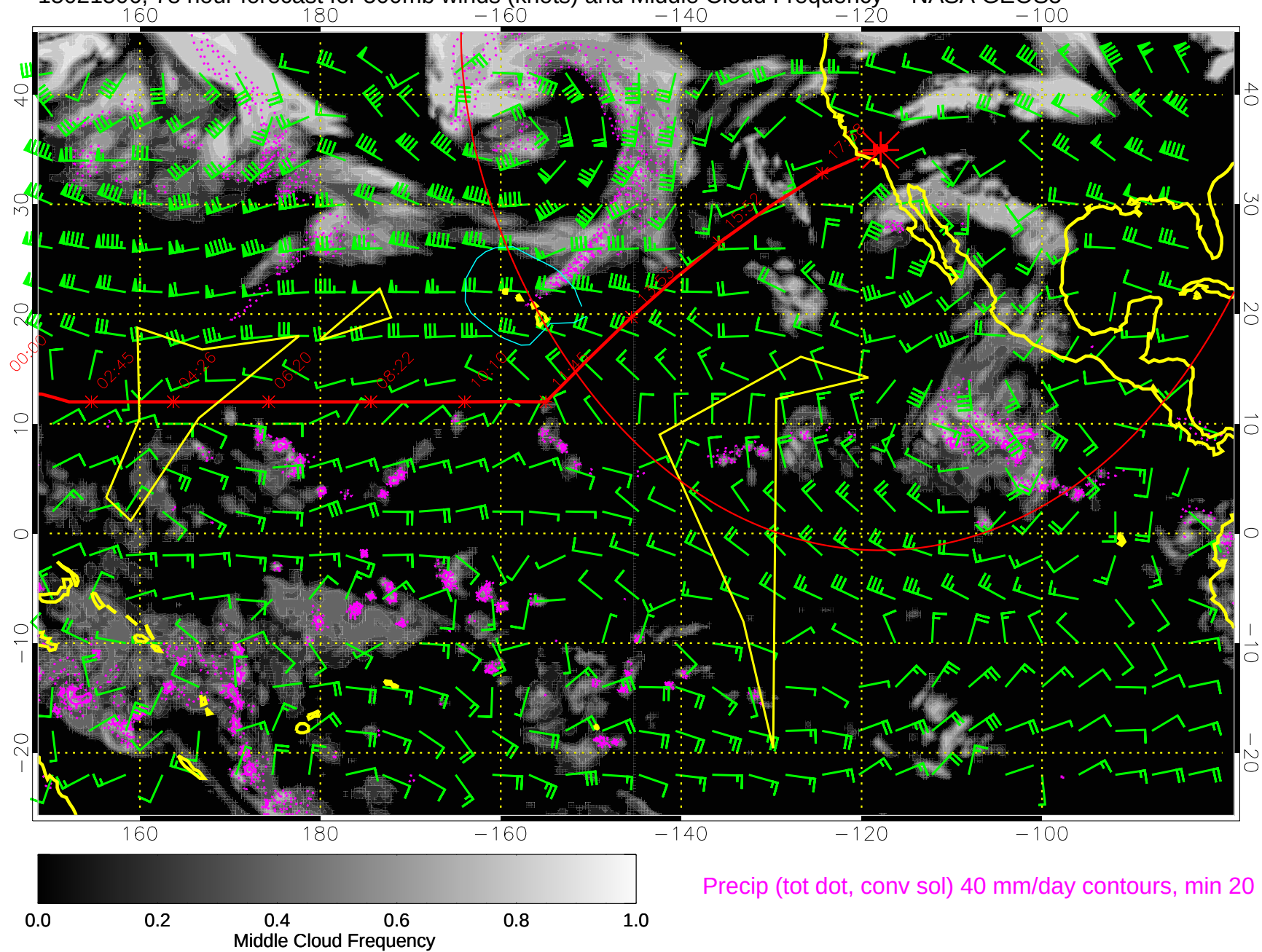
15021506, 78 hour forecast for 500mb winds (knots) and Middle Cloud Frequency -- NASA GEOS5
