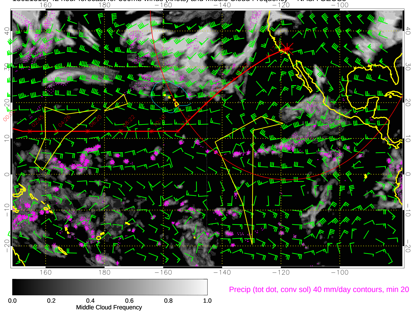
15021318, 42 hour forecast for 500mb winds (knots) and Middle Cloud Frequency -- NASA GEOS5
