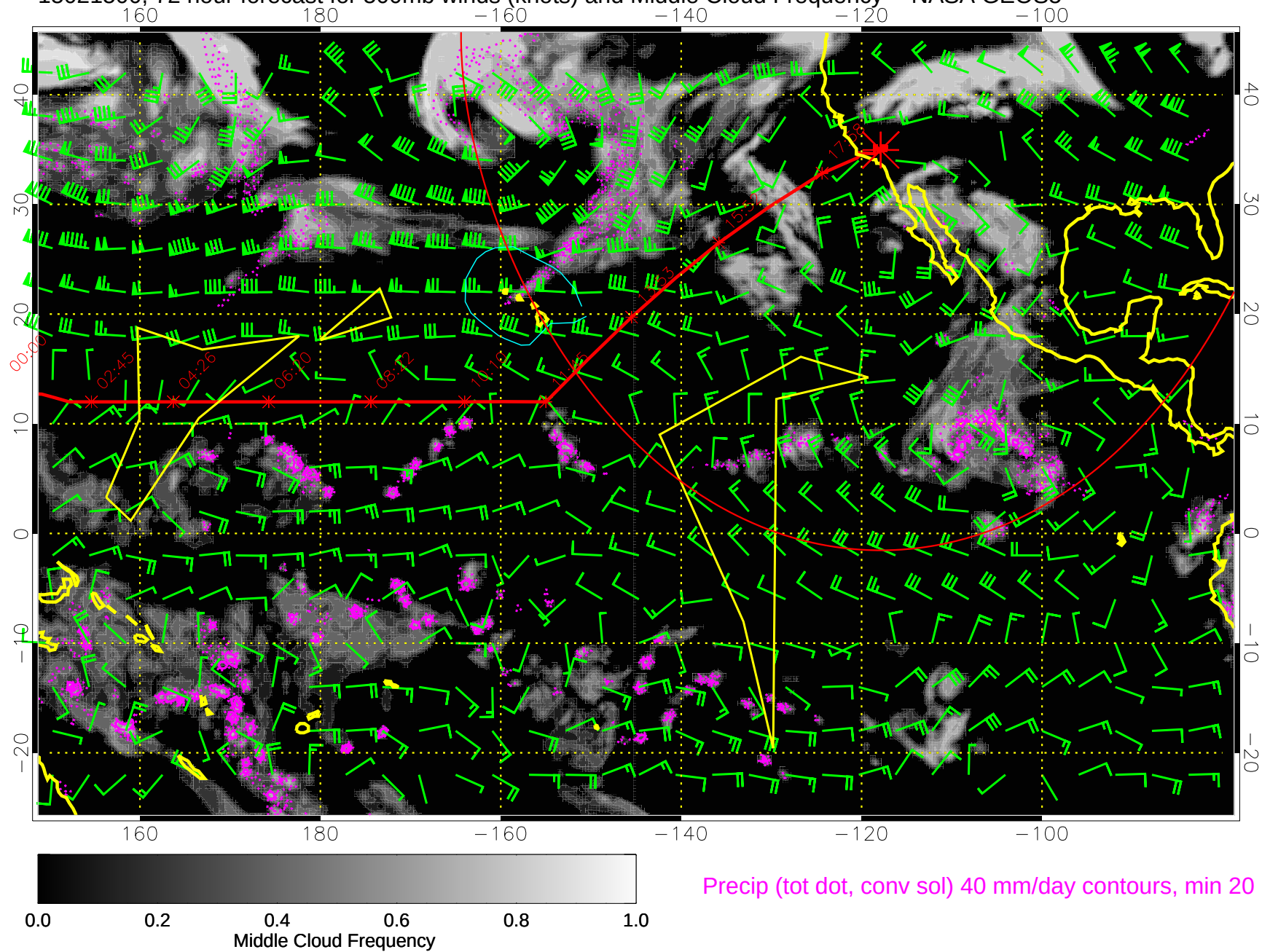
15021500, 72 hour forecast for 500mb winds (knots) and Middle Cloud Frequency -- NASA GEOS5
