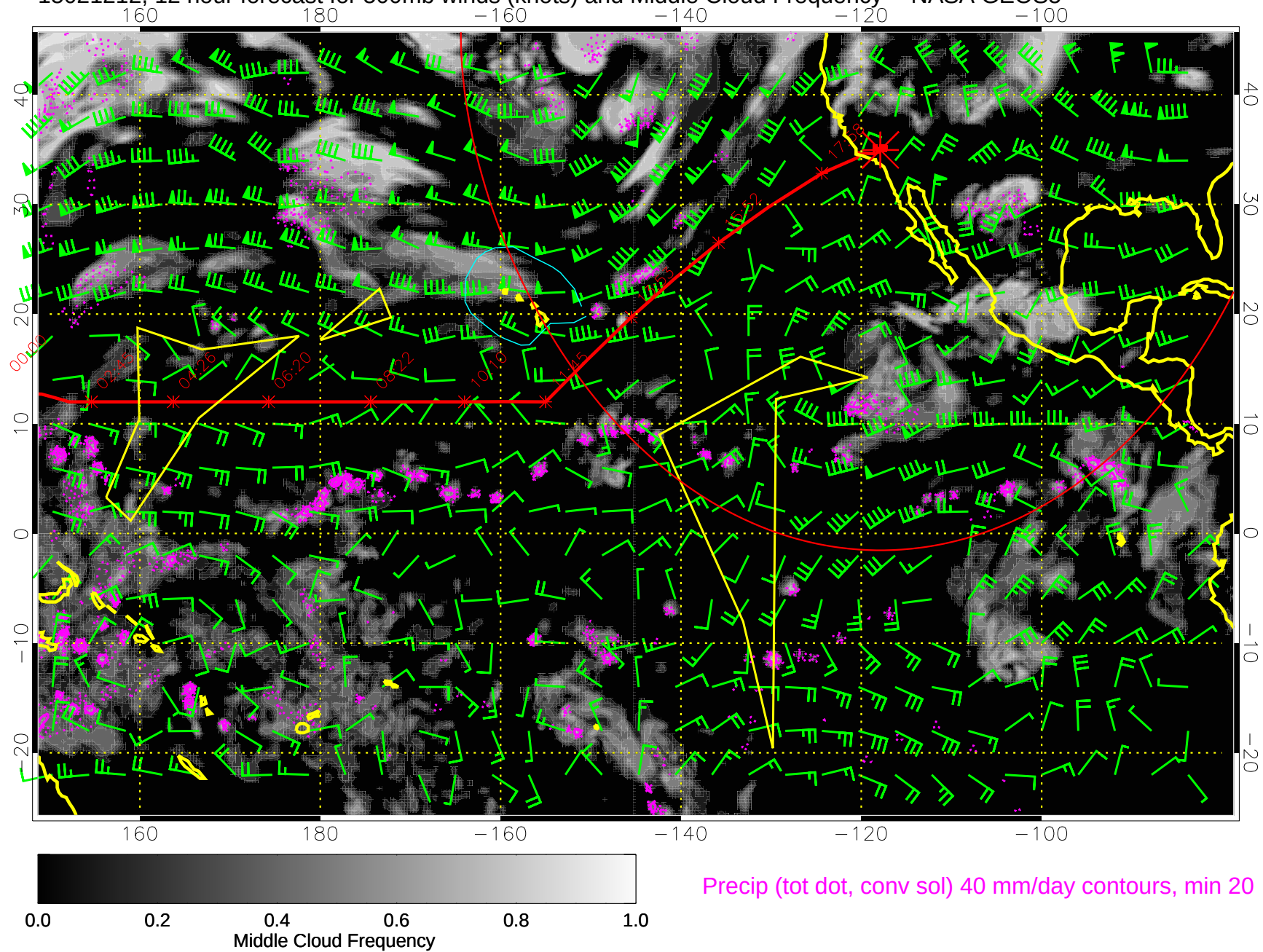
15021212, 12 hour forecast for 500mb winds (knots) and Middle Cloud Frequency -- NASA GEOS5
