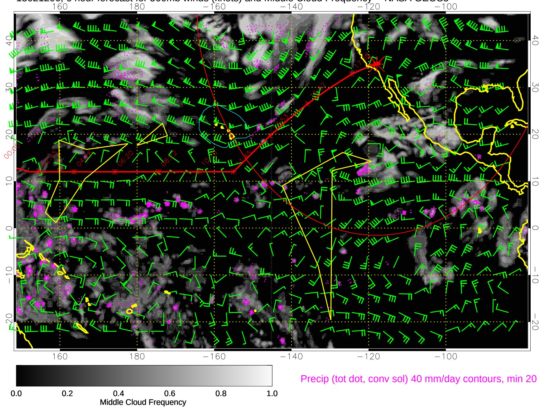
15021206, 6 hour forecast for 500mb winds (knots) and Middle Cloud Frequency -- NASA GEOS5
