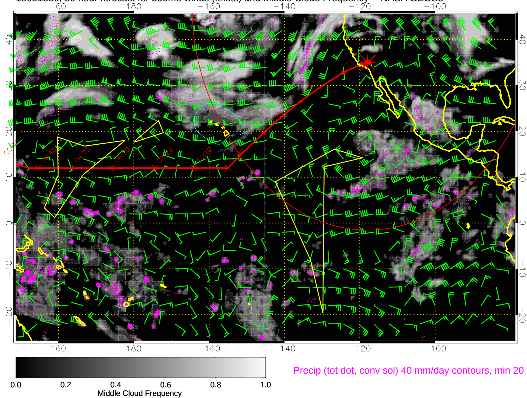
15021306, 30 hour forecast for 500mb winds (knots) and Middle Cloud Frequency -- NASA GEOS5
