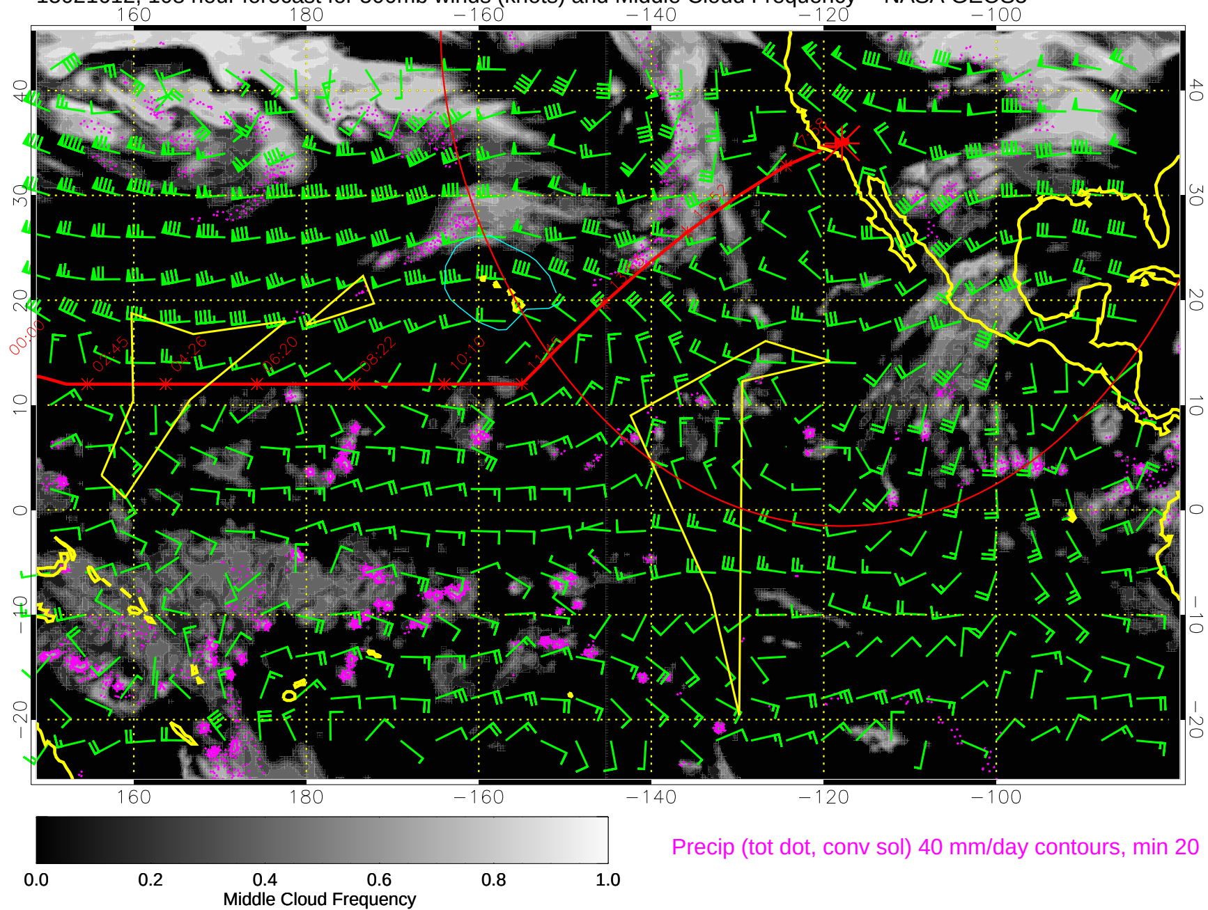
15021612, 108 hour forecast for 500mb winds (knots) and Middle Cloud Frequency -- NASA GEOS5
