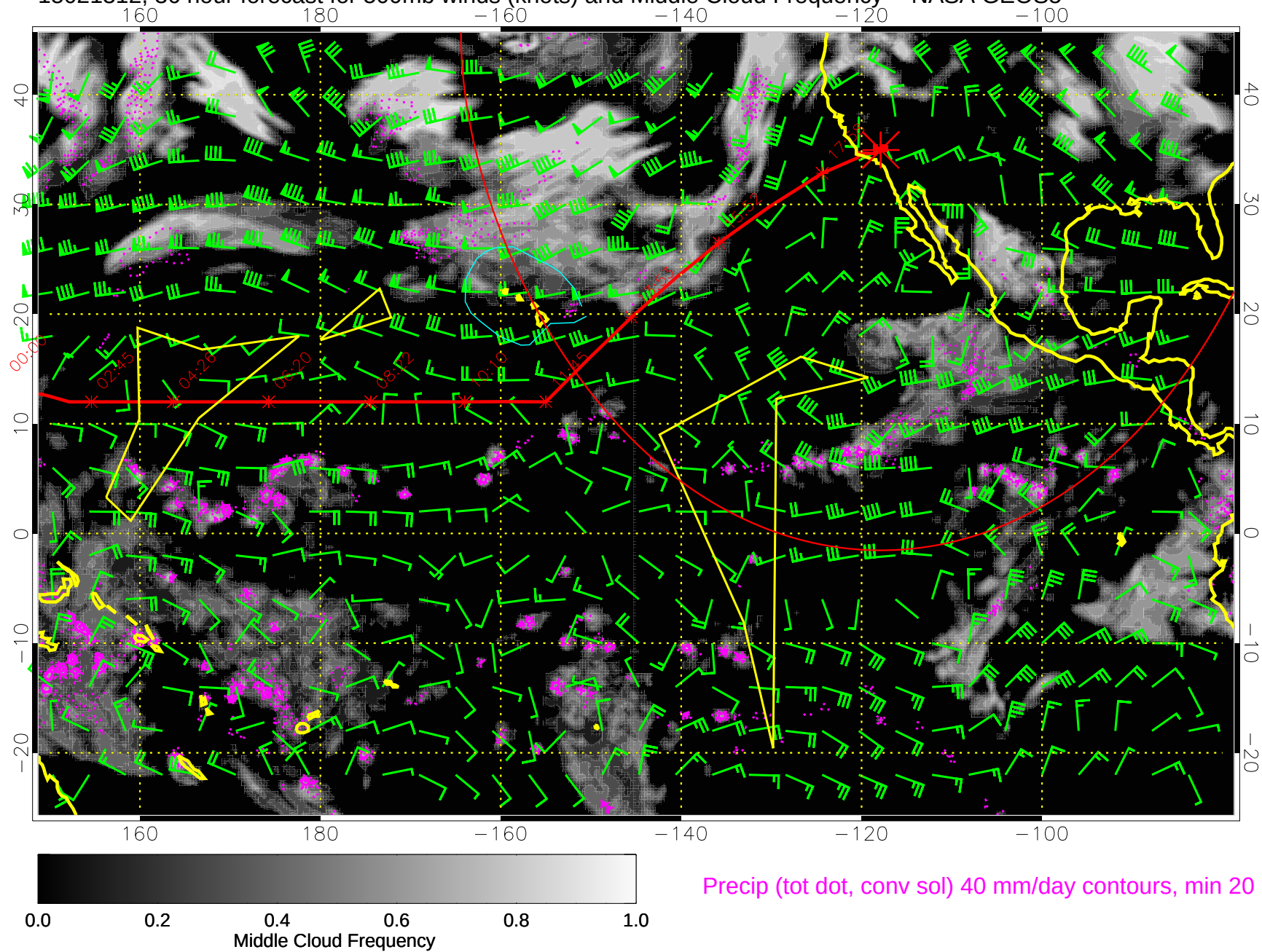
15021312, 36 hour forecast for 500mb winds (knots) and Middle Cloud Frequency -- NASA GEOS5
