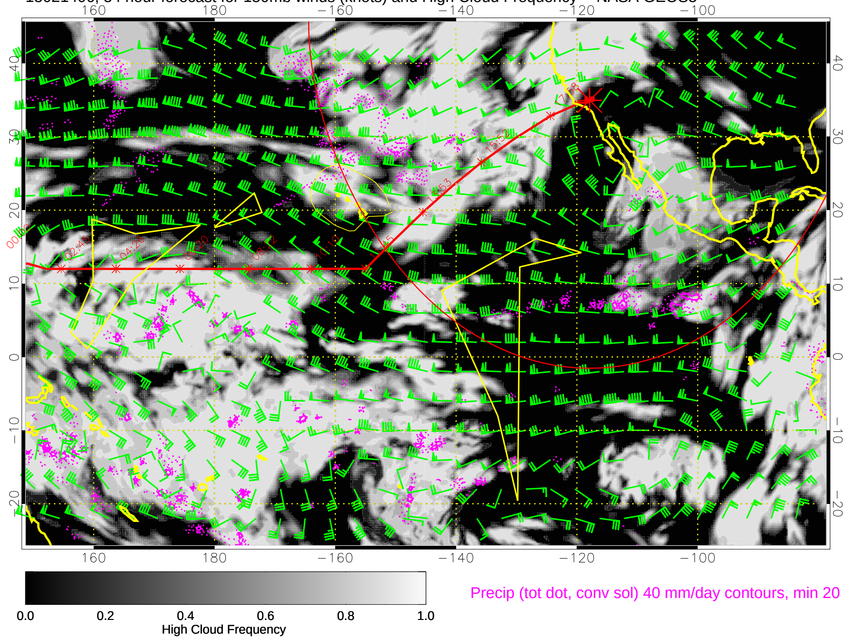
15021406, 54 hour forecast for 150mb winds (knots) and High Cloud Frequency -- NASA GEOS5
