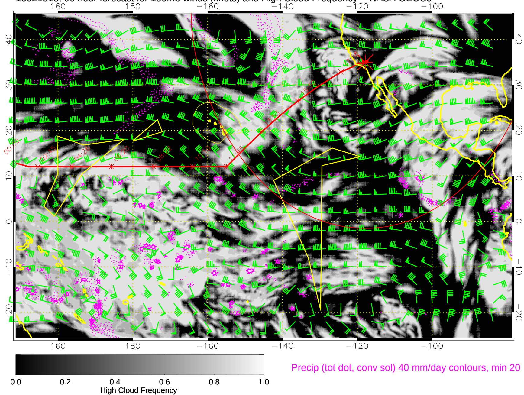
15021518, 90 hour forecast for 150mb winds (knots) and High Cloud Frequency -- NASA GEOS5
