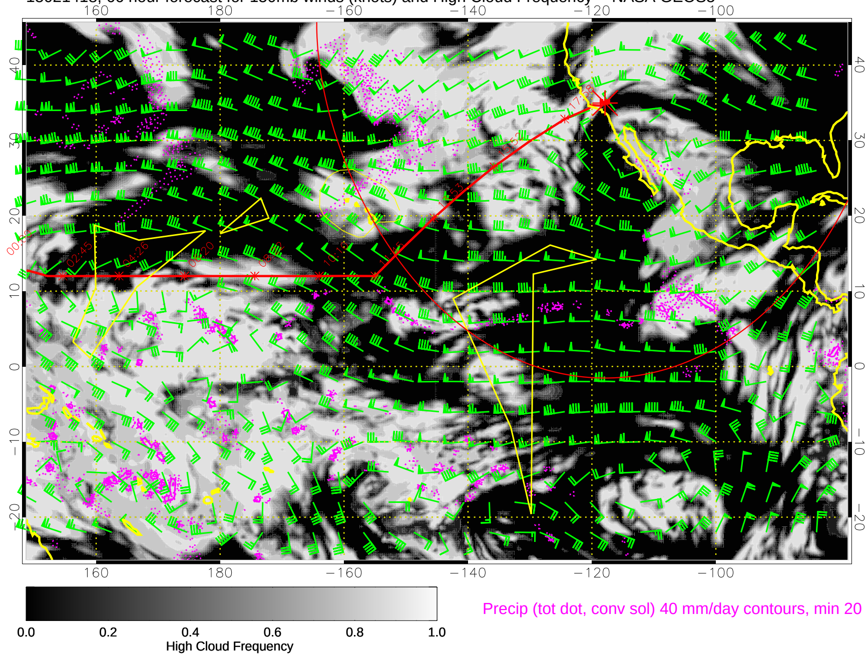
15021418, 66 hour forecast for 150mb winds (knots) and High Cloud Frequency -- NASA GEOS5
