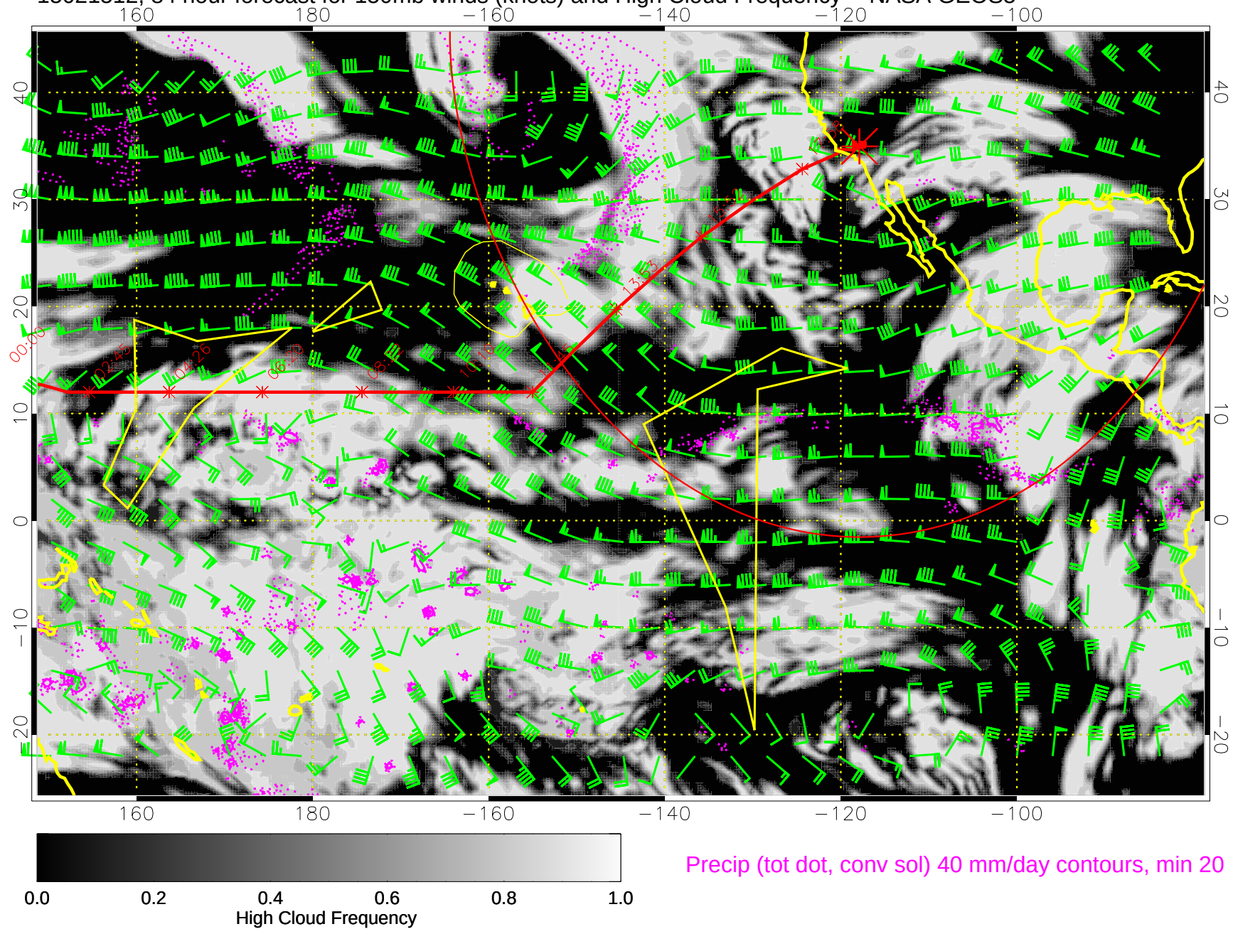
15021512, 84 hour forecast for 150mb winds (knots) and High Cloud Frequency -- NASA GEOS5
