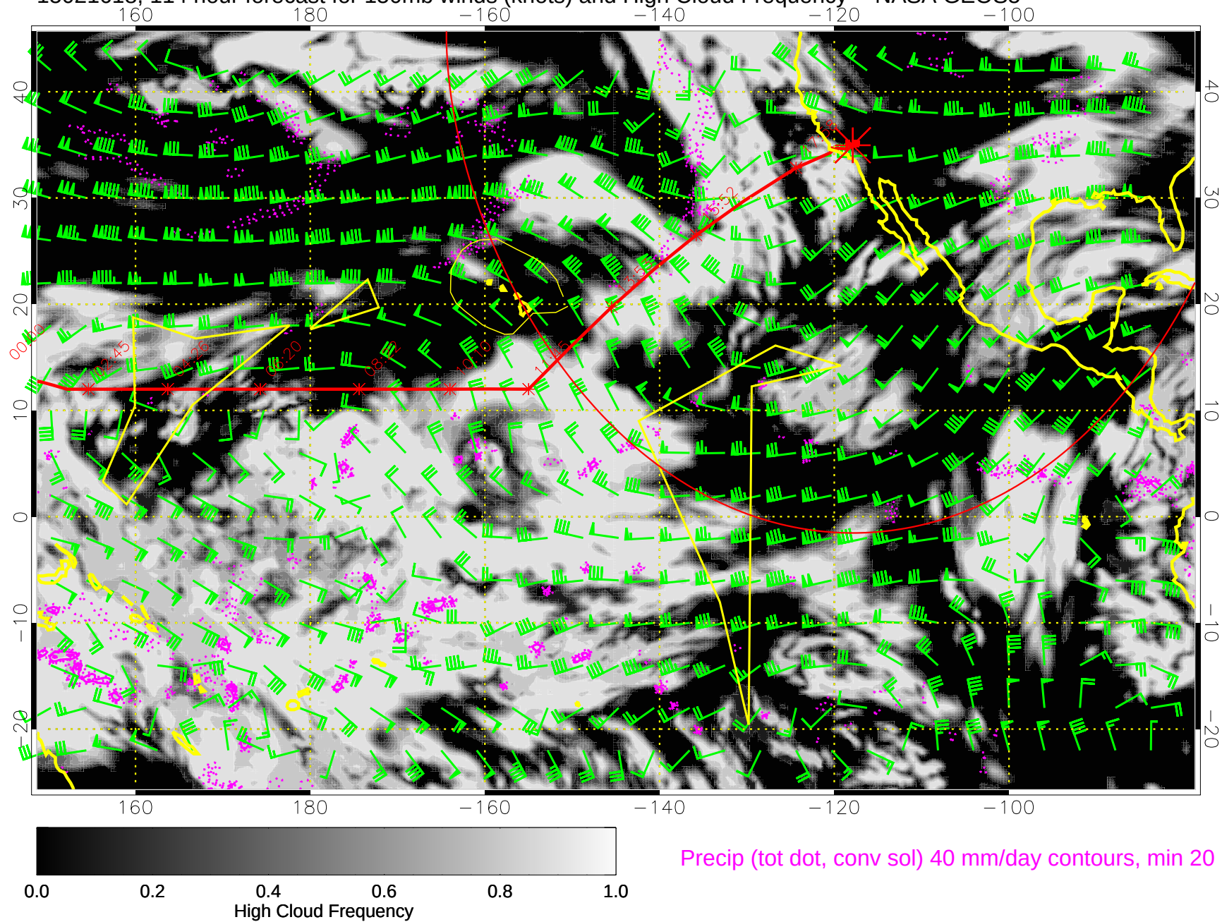
15021618, 114 hour forecast for 150mb winds (knots) and High Cloud Frequency -- NASA GEOS5
