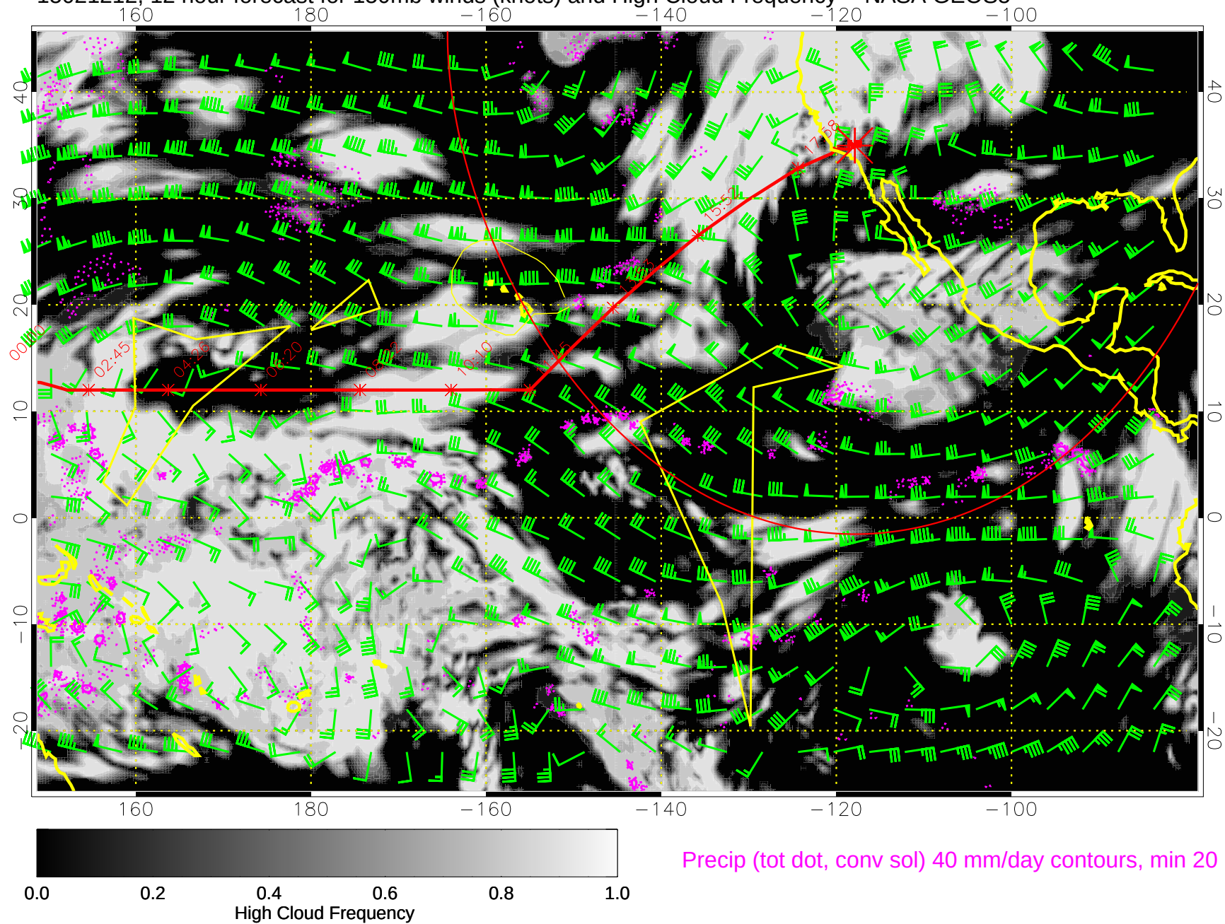
15021212, 12 hour forecast for 150mb winds (knots) and High Cloud Frequency -- NASA GEOS5
