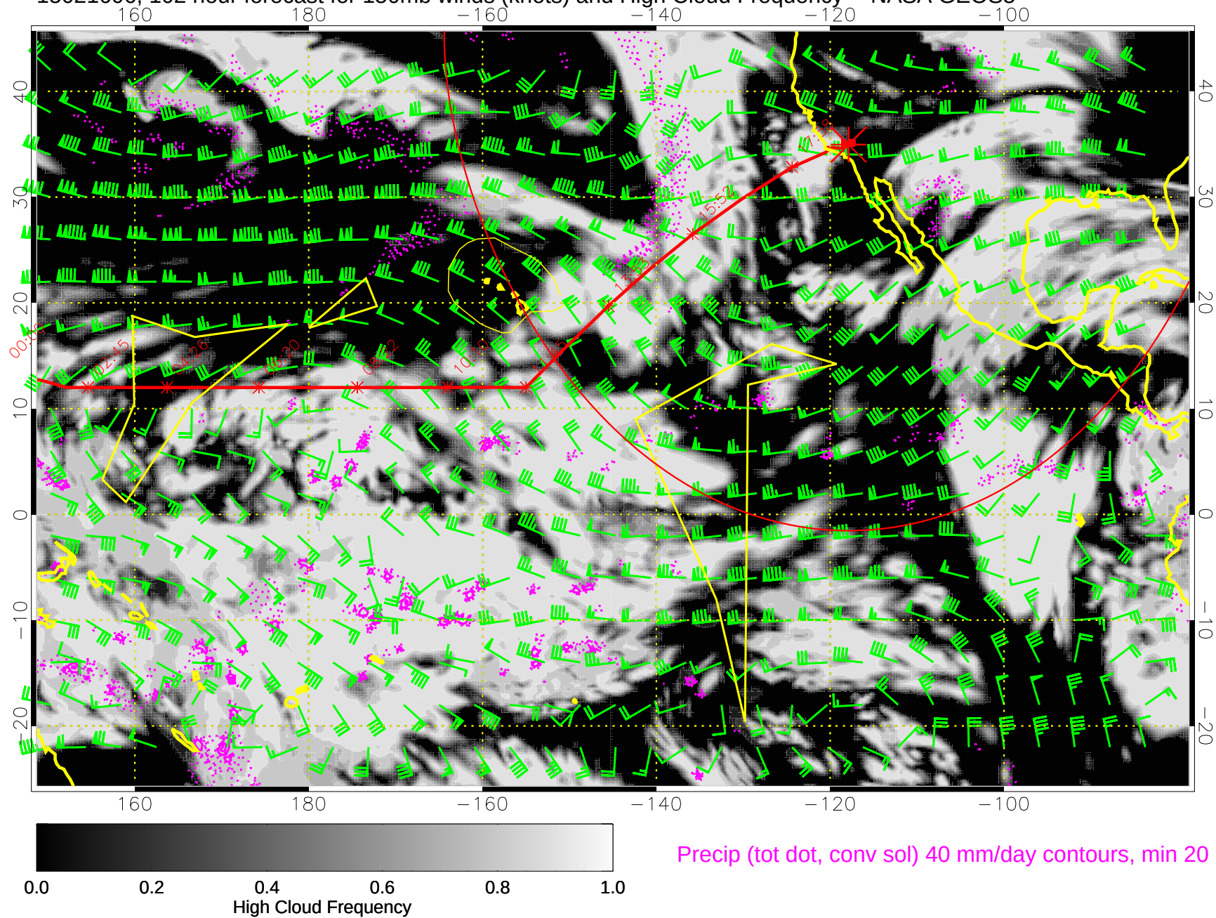
15021606, 102 hour forecast for 150mb winds (knots) and High Cloud Frequency -- NASA GEOS5
