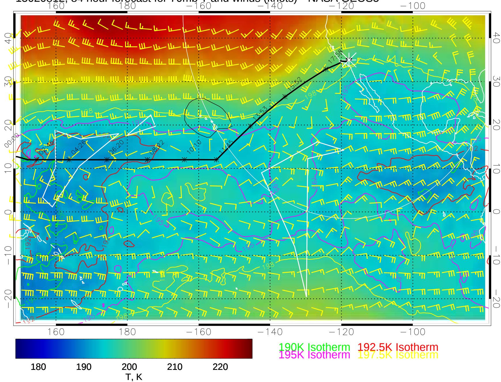
15020812, 84 hour forecast for 70mb T and winds (knots)-- NASA GEOS5
