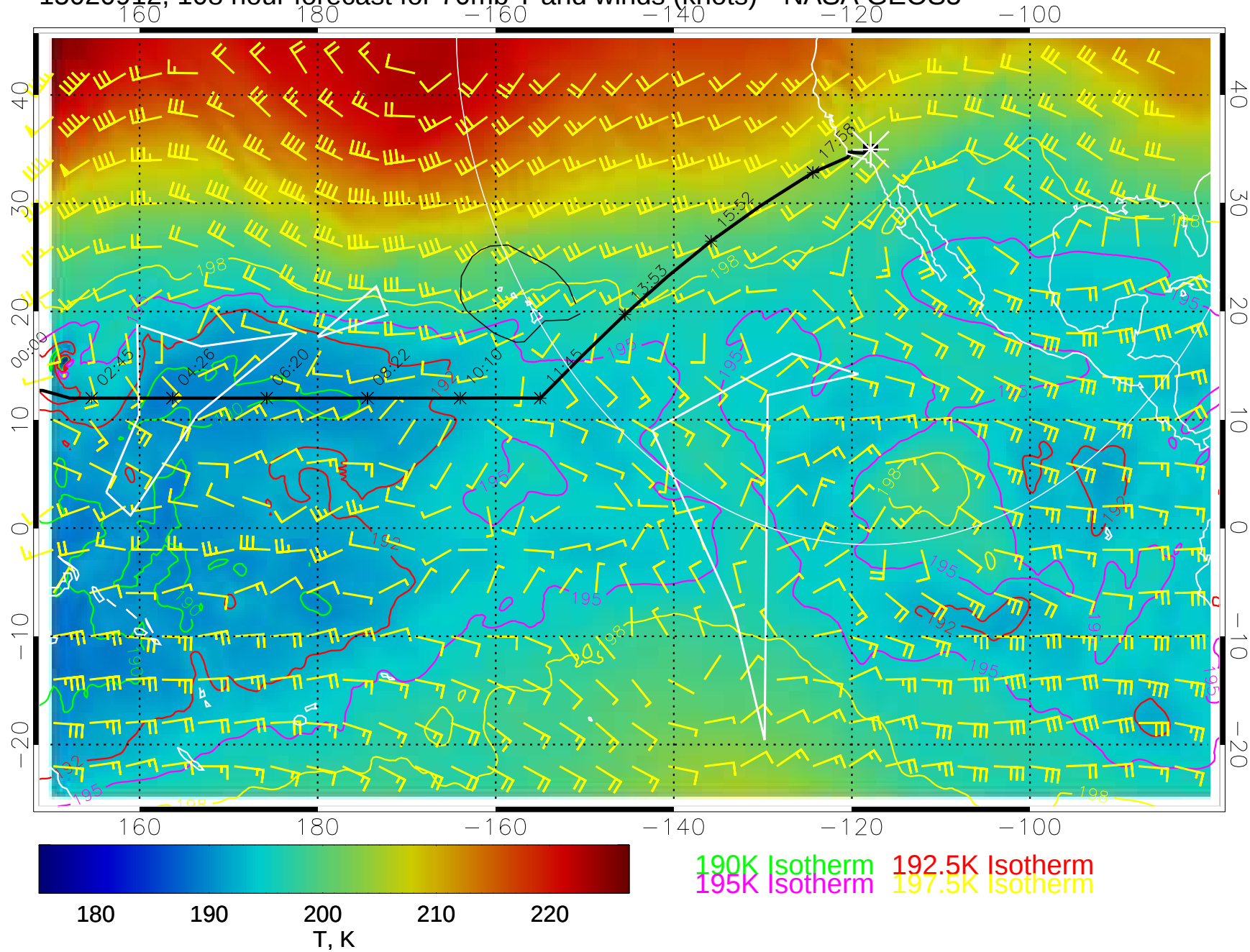
15020912, 108 hour forecast for 70mb T and winds (knots)-- NASA GEOS5
