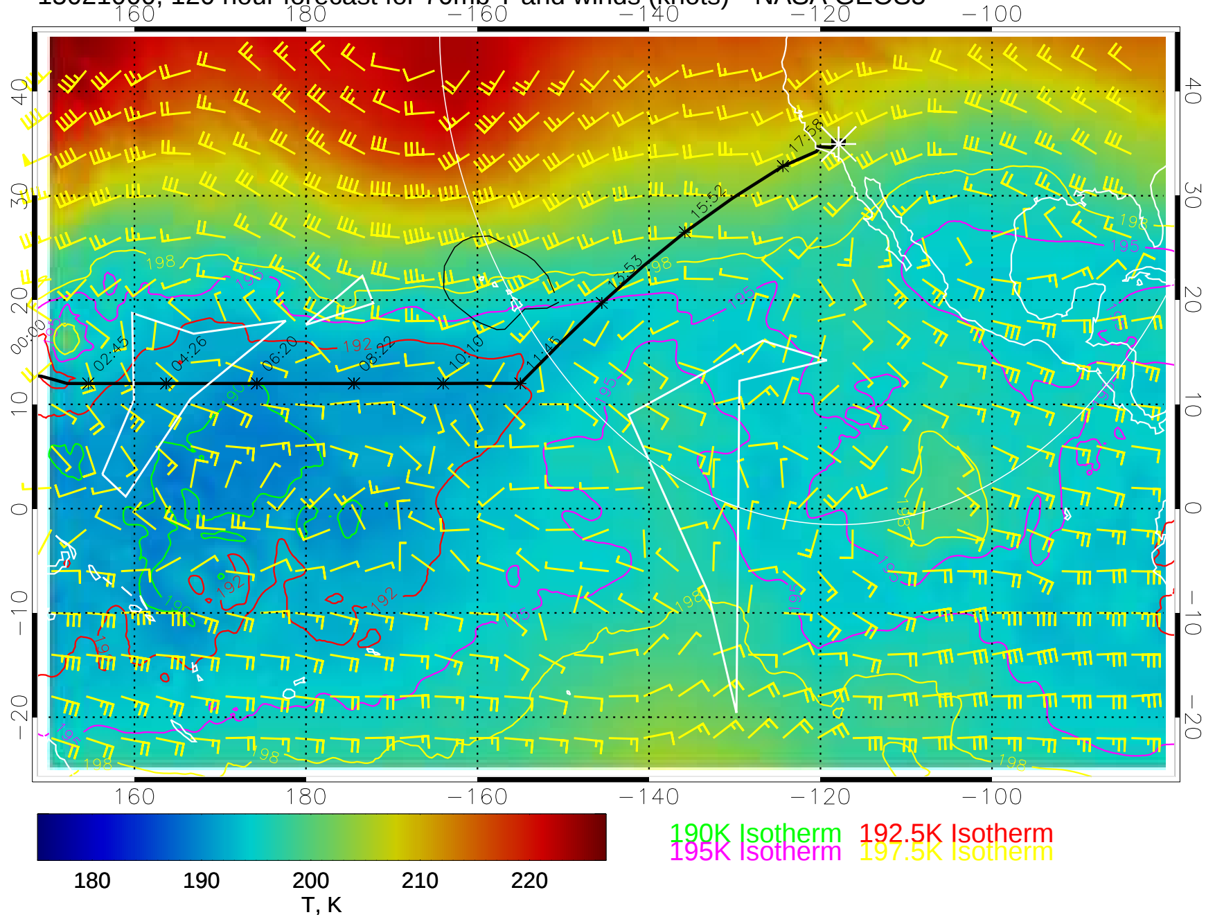
15021000, 120 hour forecast for 70mb T and winds (knots)-- NASA GEOS5
