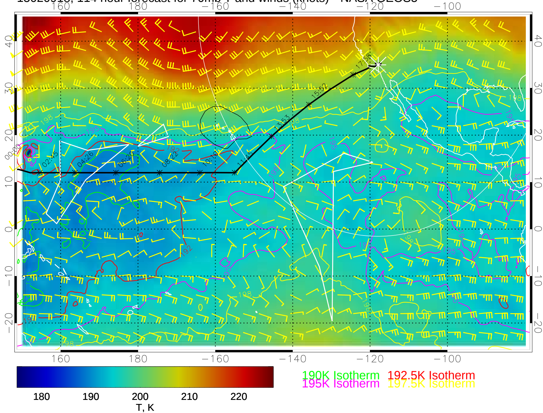
15020918, 114 hour forecast for 70mb T and winds (knots)-- NASA GEOS5
