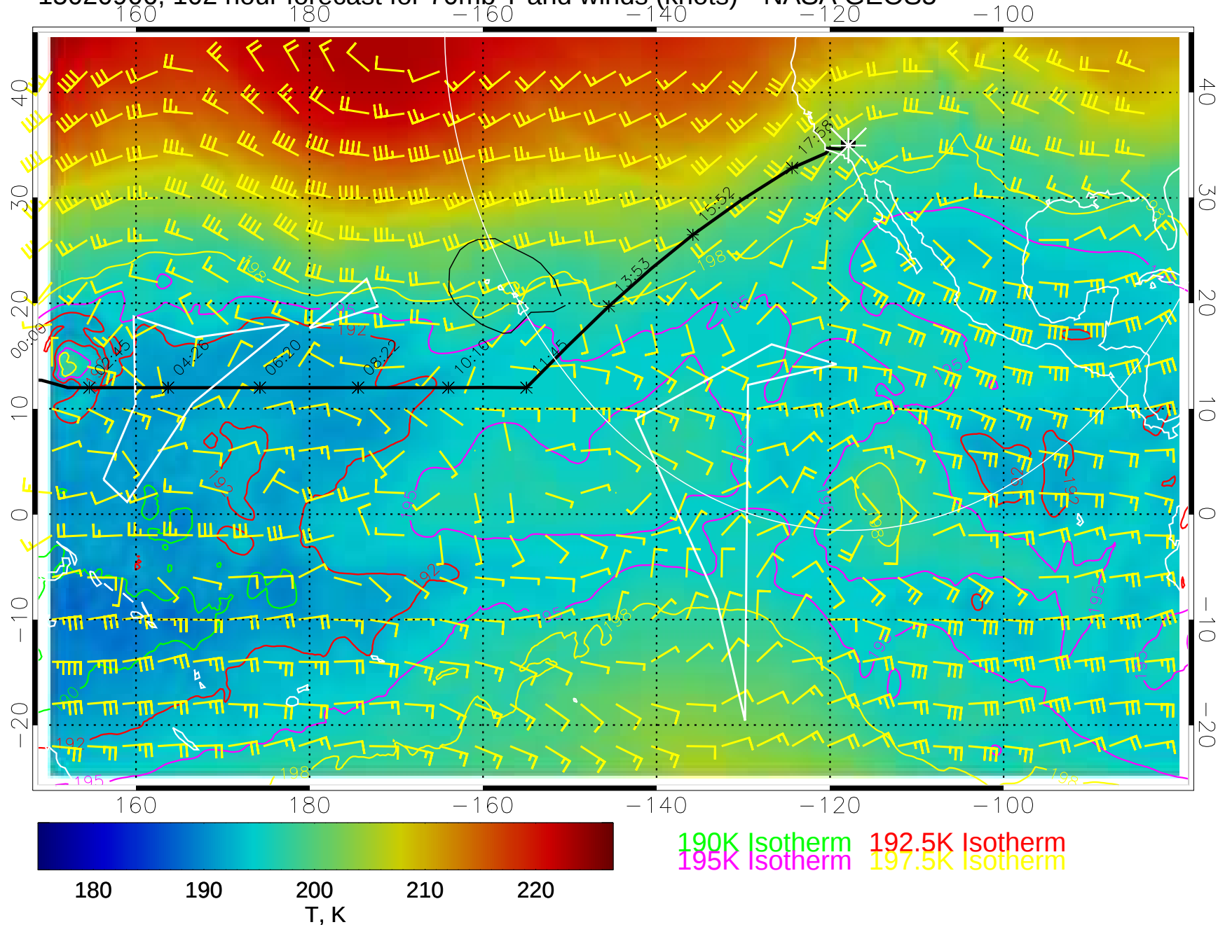
15020906, 102 hour forecast for 70mb T and winds (knots)-- NASA GEOS5
