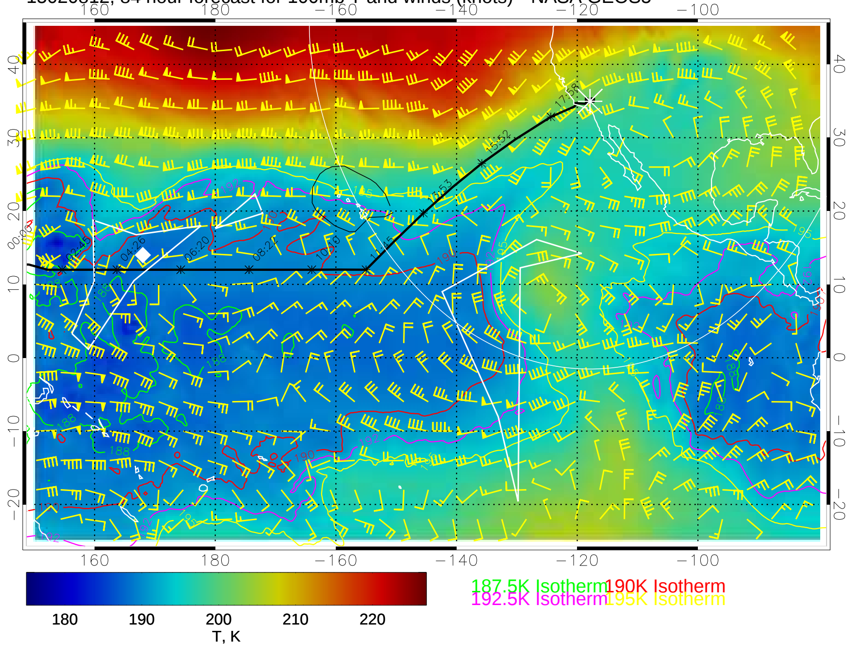
15020812, 84 hour forecast for 100mb T and winds (knots)-- NASA GEOS5
