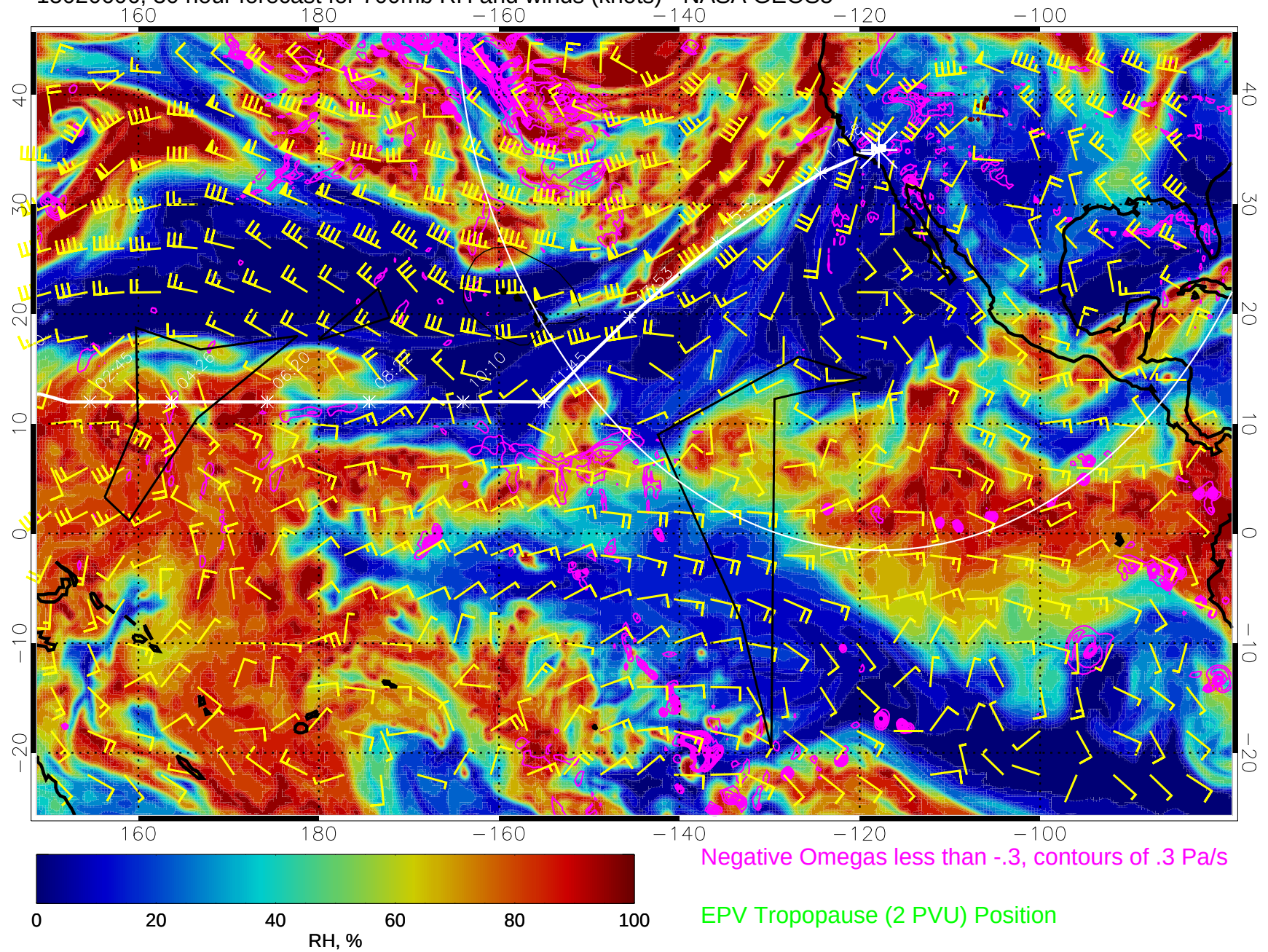
15020606, 30 hour forecast for 700mb RH and winds (knots) - NASA GEOS5
