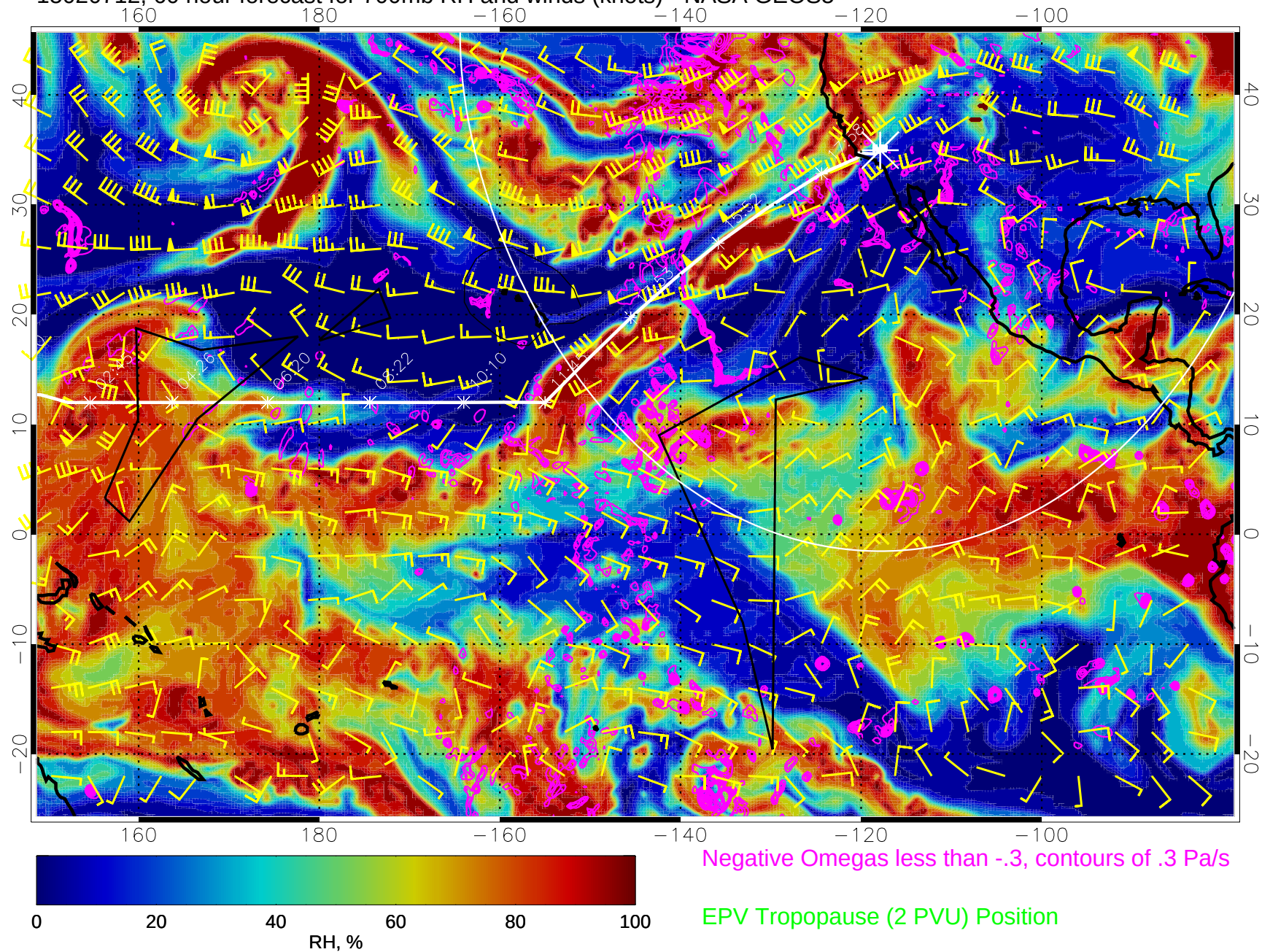
15020712, 60 hour forecast for 700mb RH and winds (knots) - NASA GEOS5
