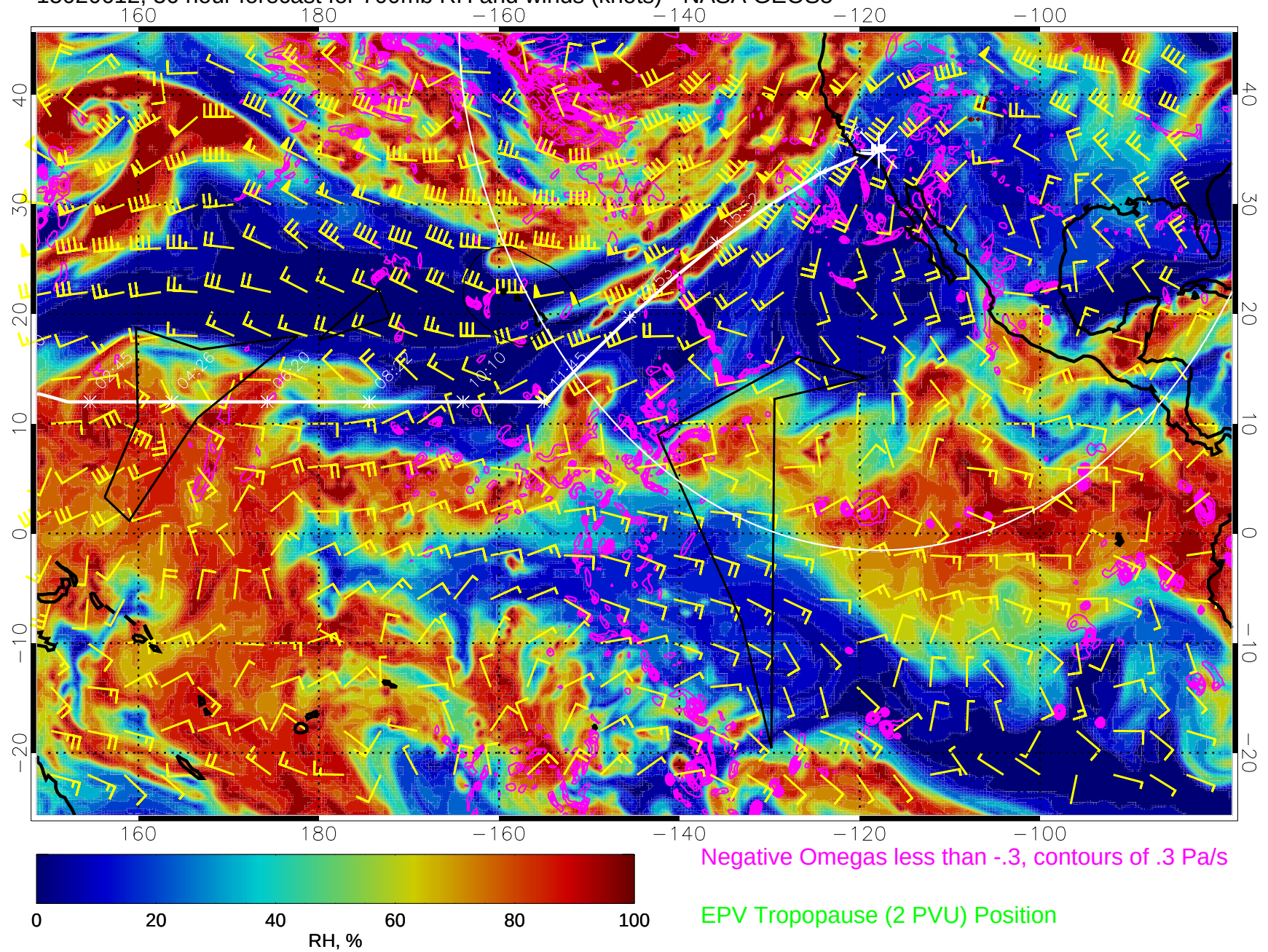
15020612, 36 hour forecast for 700mb RH and winds (knots) - NASA GEOS5
