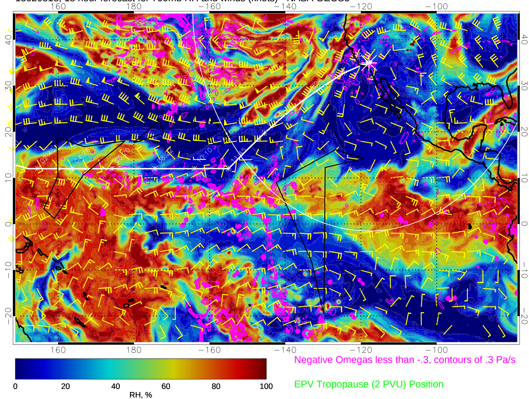
15020518, 18 hour forecast for 700mb RH and winds (knots) - NASA GEOS5
