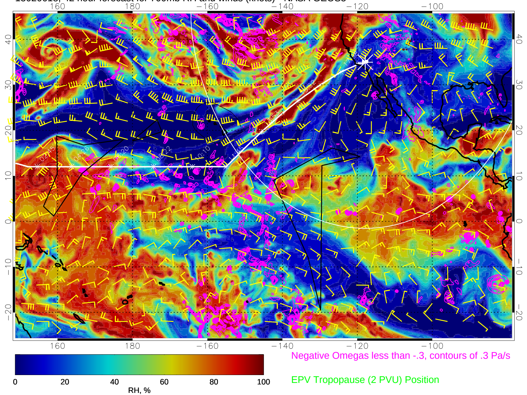
15020618, 42 hour forecast for 700mb RH and winds (knots) - NASA GEOS5
