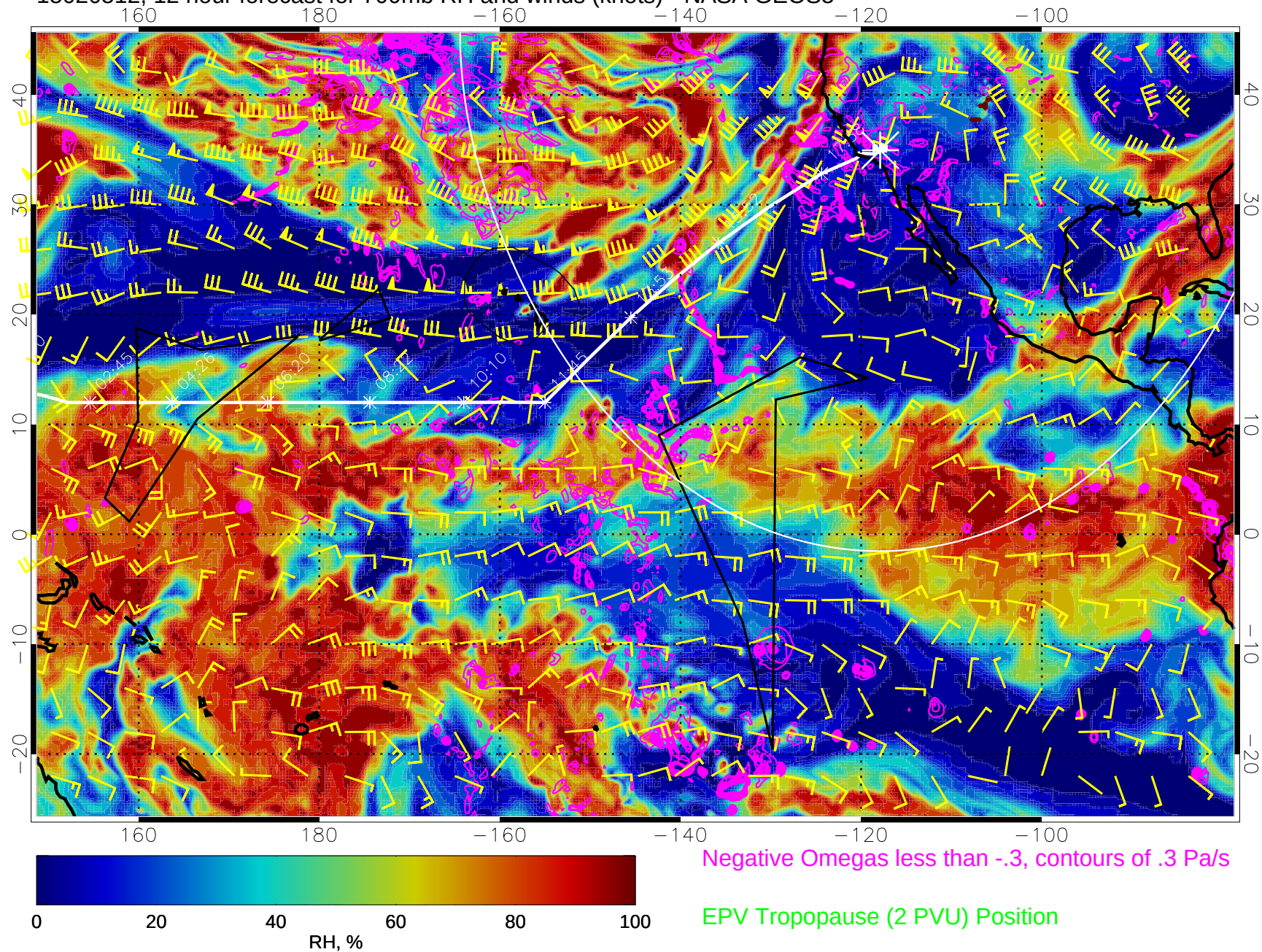
15020512, 12 hour forecast for 700mb RH and winds (knots) - NASA GEOS5
