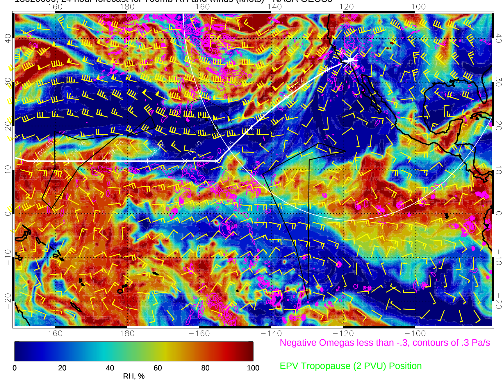
15020600, 24 hour forecast for 700mb RH and winds (knots) - NASA GEOS5
