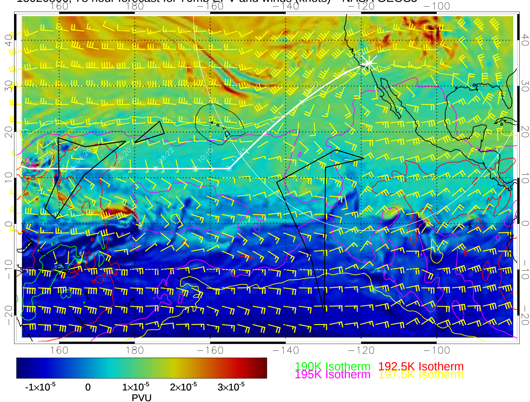
15020806, 78 hour forecast for 70mb EPV and winds (knots)-- NASA GEOS5
