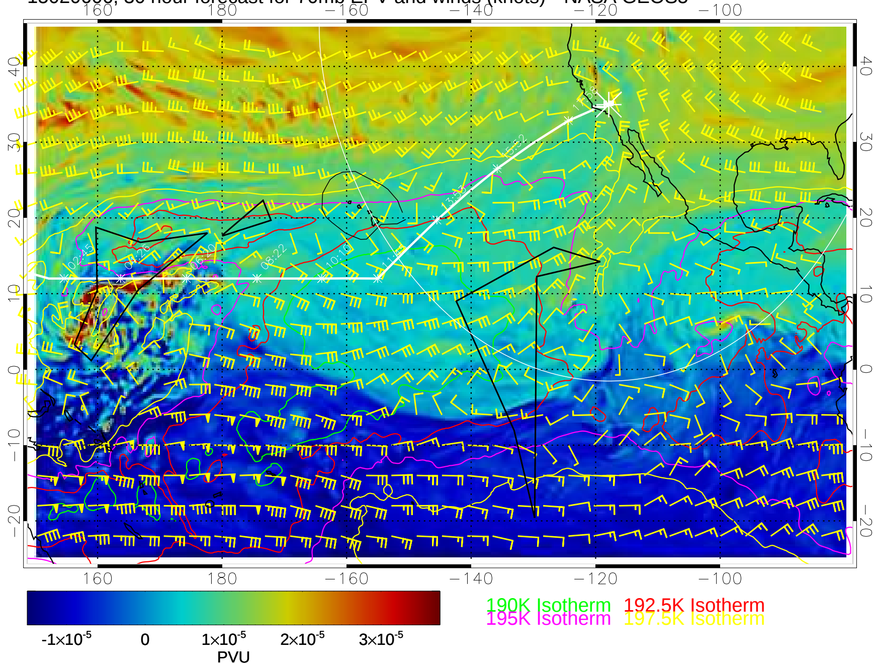
15020606, 30 hour forecast for 70mb EPV and winds (knots)-- NASA GEOS5
