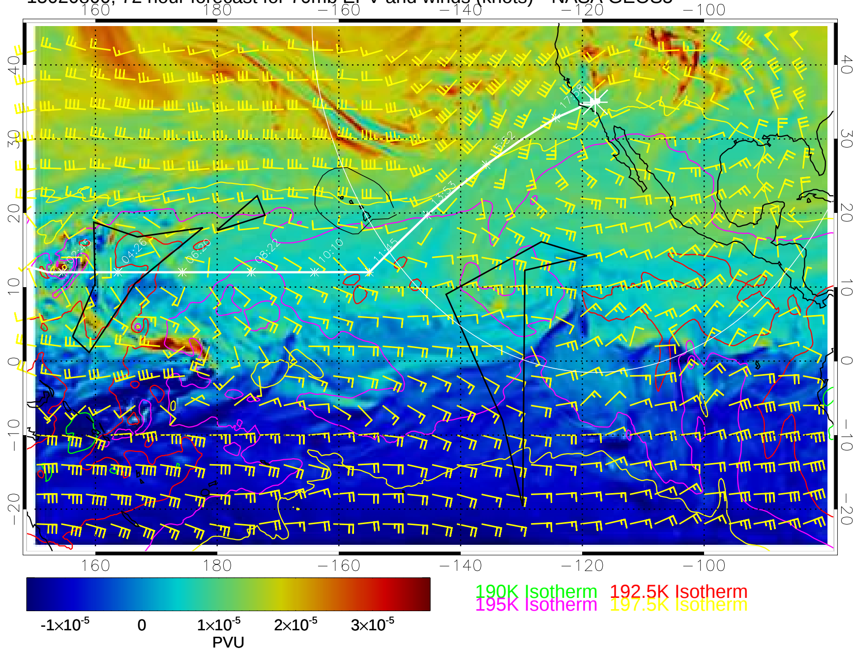
15020800, 72 hour forecast for 70mb EPV and winds (knots)-- NASA GEOS5
