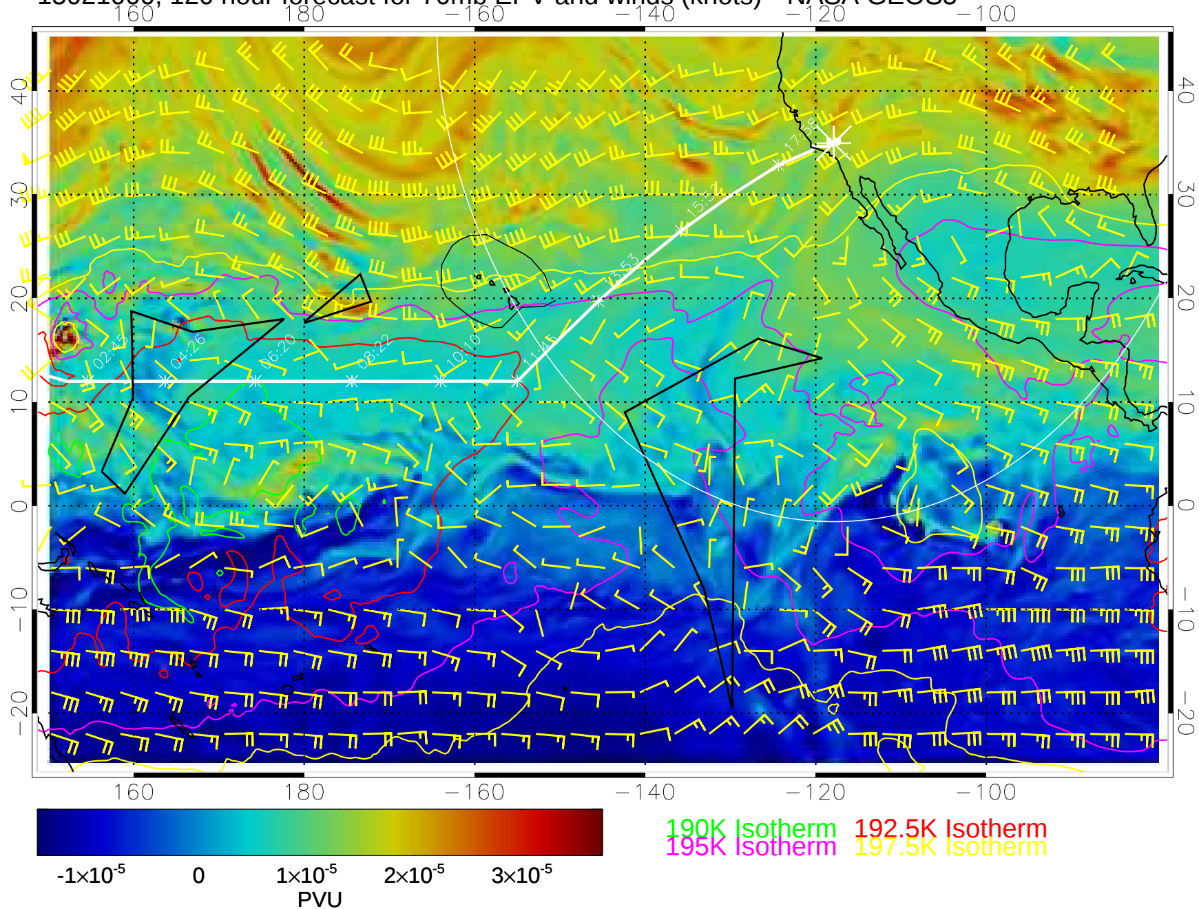
15021000, 120 hour forecast for 70mb EPV and winds (knots)-- NASA GEOS5
