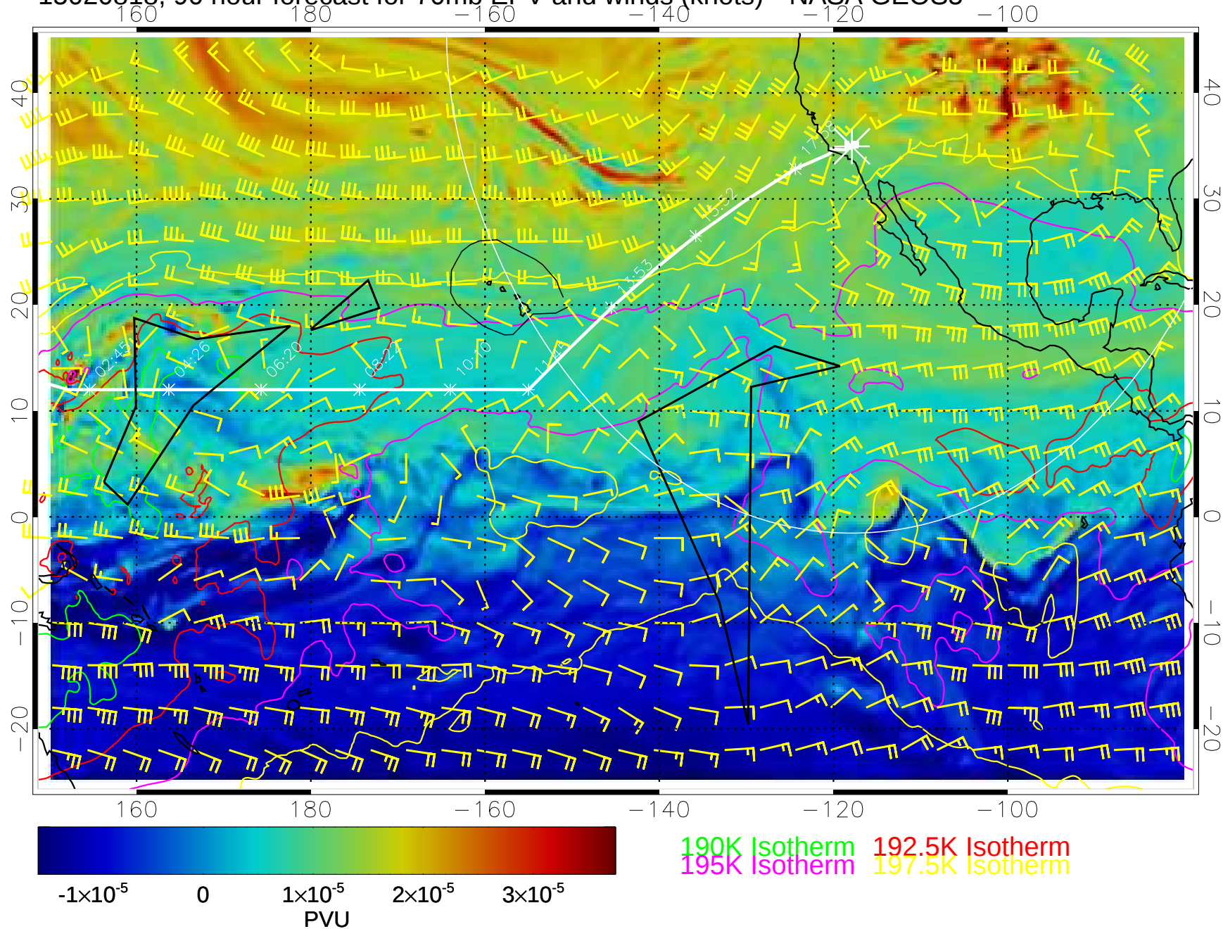
15020818, 90 hour forecast for 70mb EPV and winds (knots)-- NASA GEOS5
