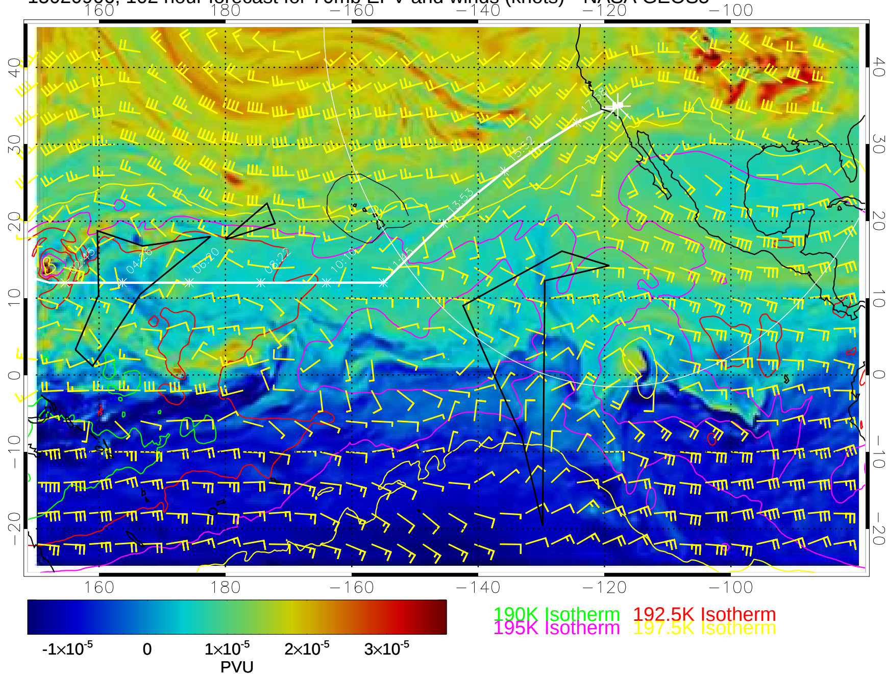
15020906, 102 hour forecast for 70mb EPV and winds (knots)-- NASA GEOS5
