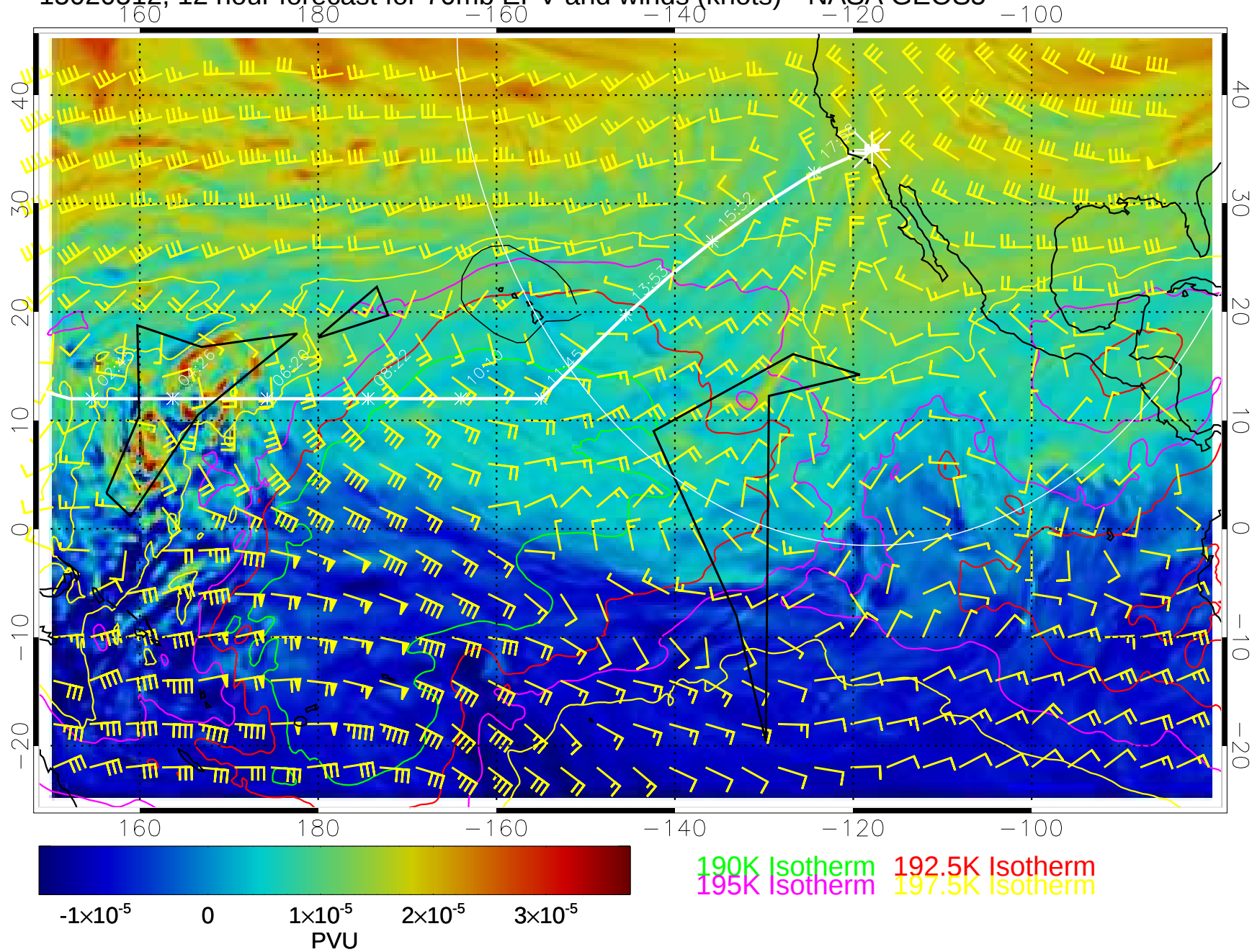
15020512, 12 hour forecast for 70mb EPV and winds (knots)-- NASA GEOS5
