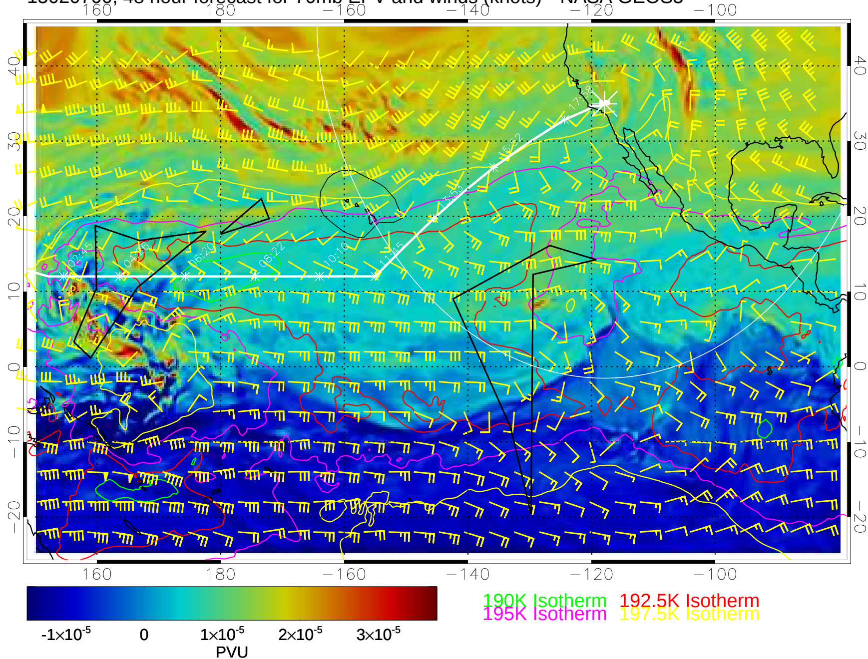
15020700, 48 hour forecast for 70mb EPV and winds (knots)-- NASA GEOS5
