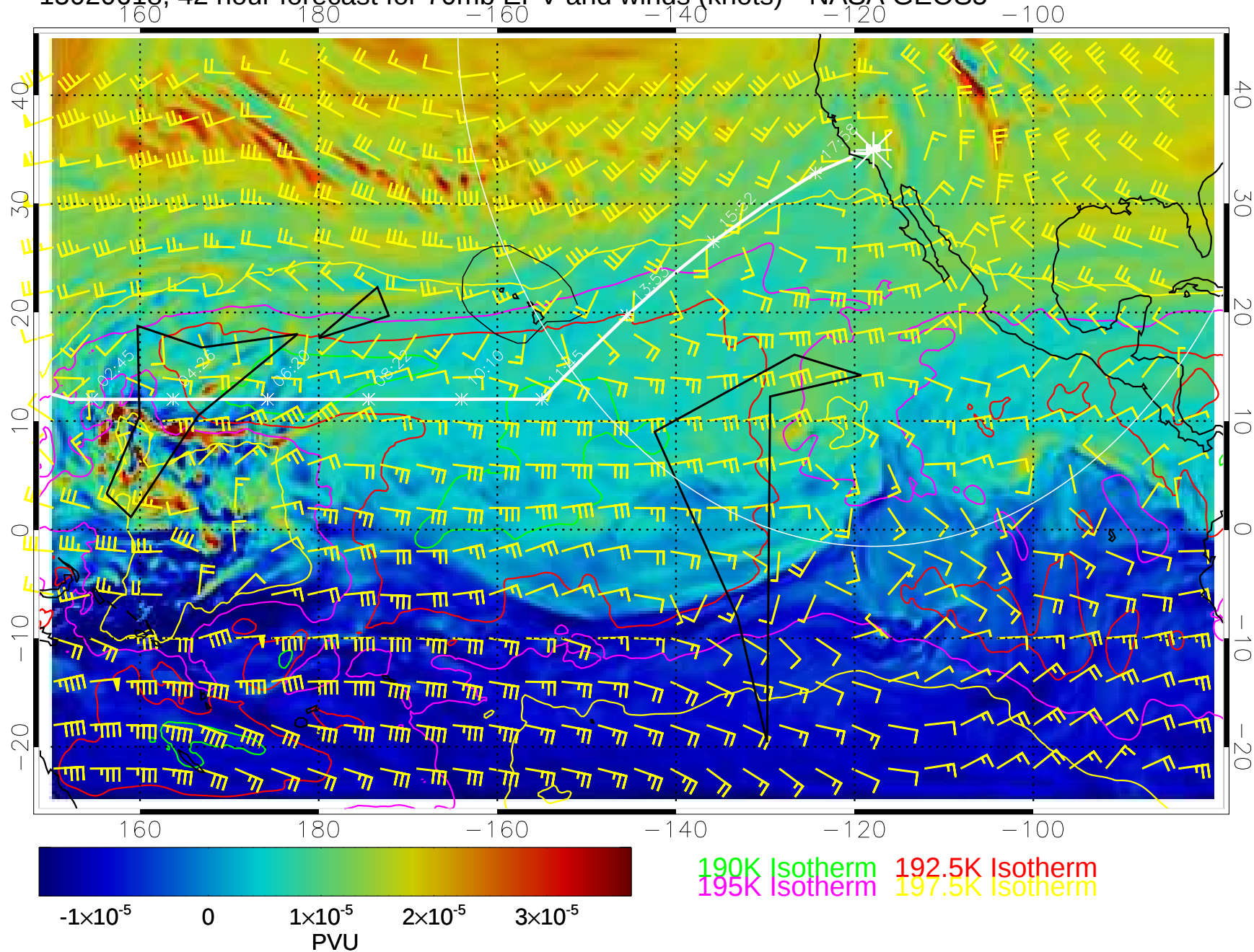
15020618, 42 hour forecast for 70mb EPV and winds (knots)-- NASA GEOS5
