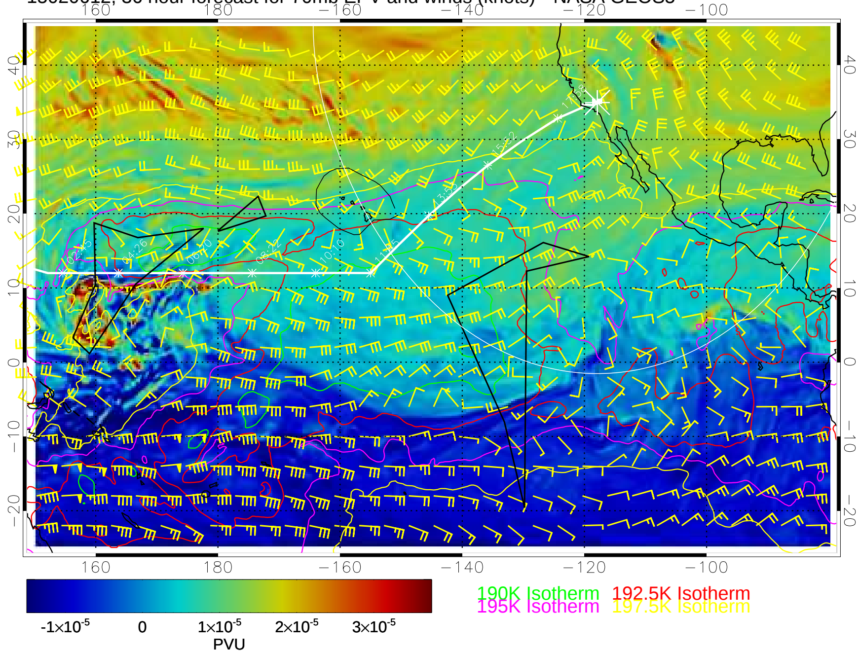
15020612, 36 hour forecast for 70mb EPV and winds (knots)-- NASA GEOS5
