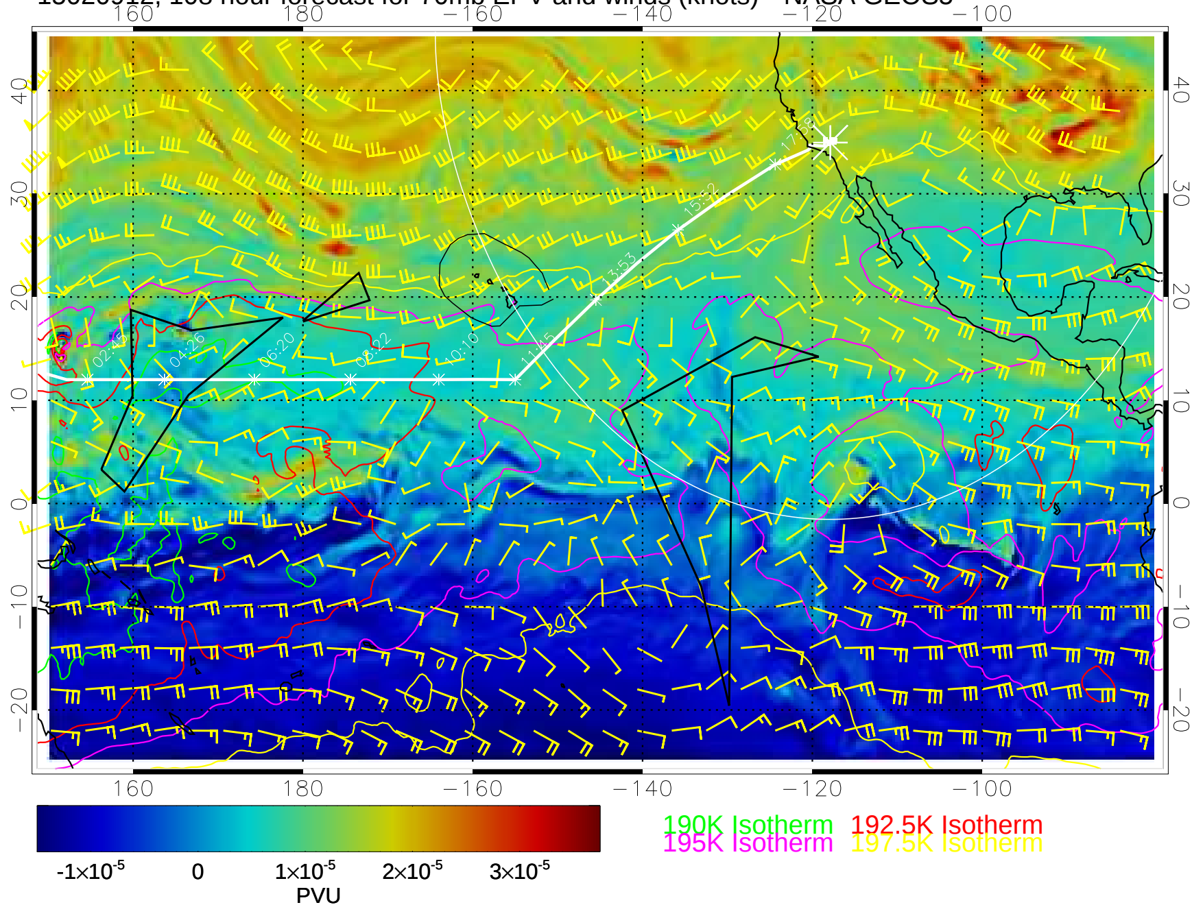
15020912, 108 hour forecast for 70mb EPV and winds (knots)-- NASA GEOS5
