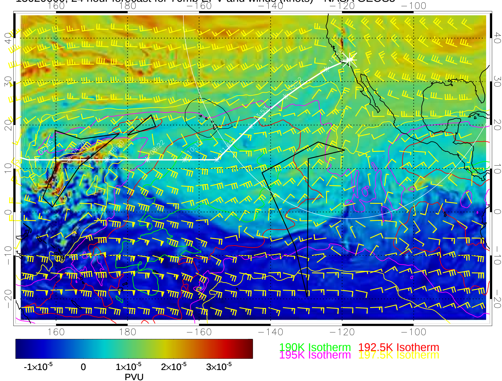
15020600, 24 hour forecast for 70mb EPV and winds (knots)-- NASA GEOS5
