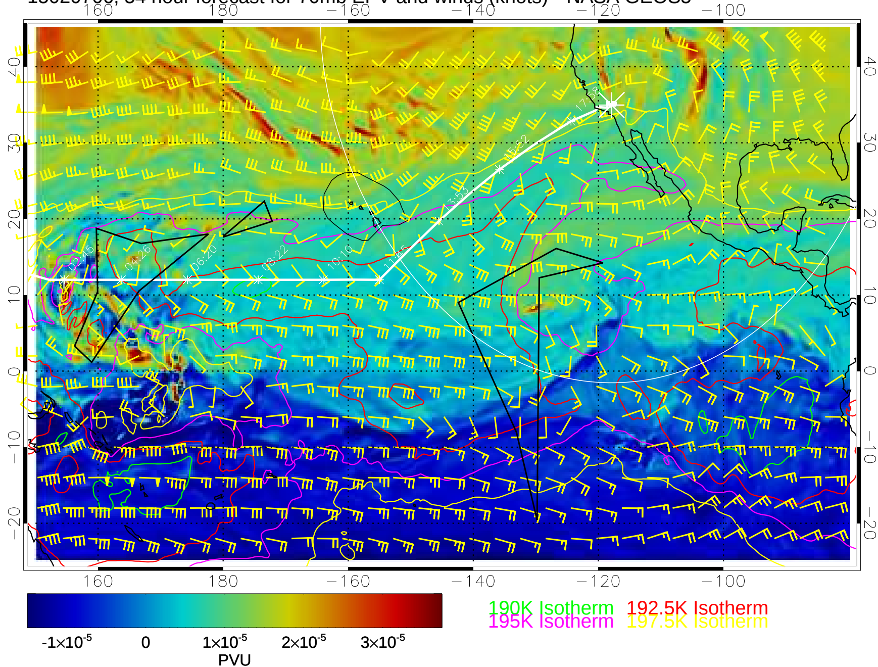
15020706, 54 hour forecast for 70mb EPV and winds (knots)-- NASA GEOS5
