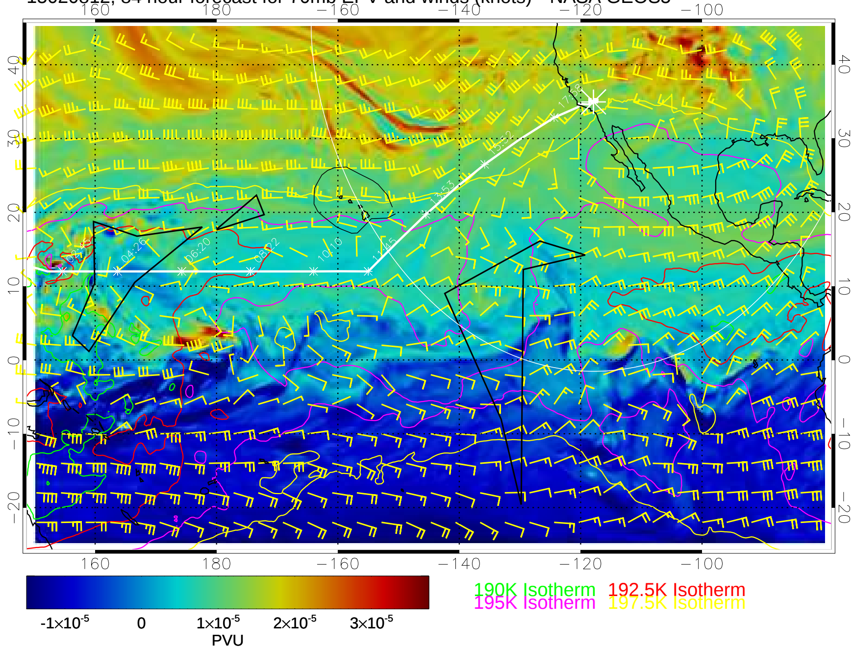
15020812, 84 hour forecast for 70mb EPV and winds (knots)-- NASA GEOS5
