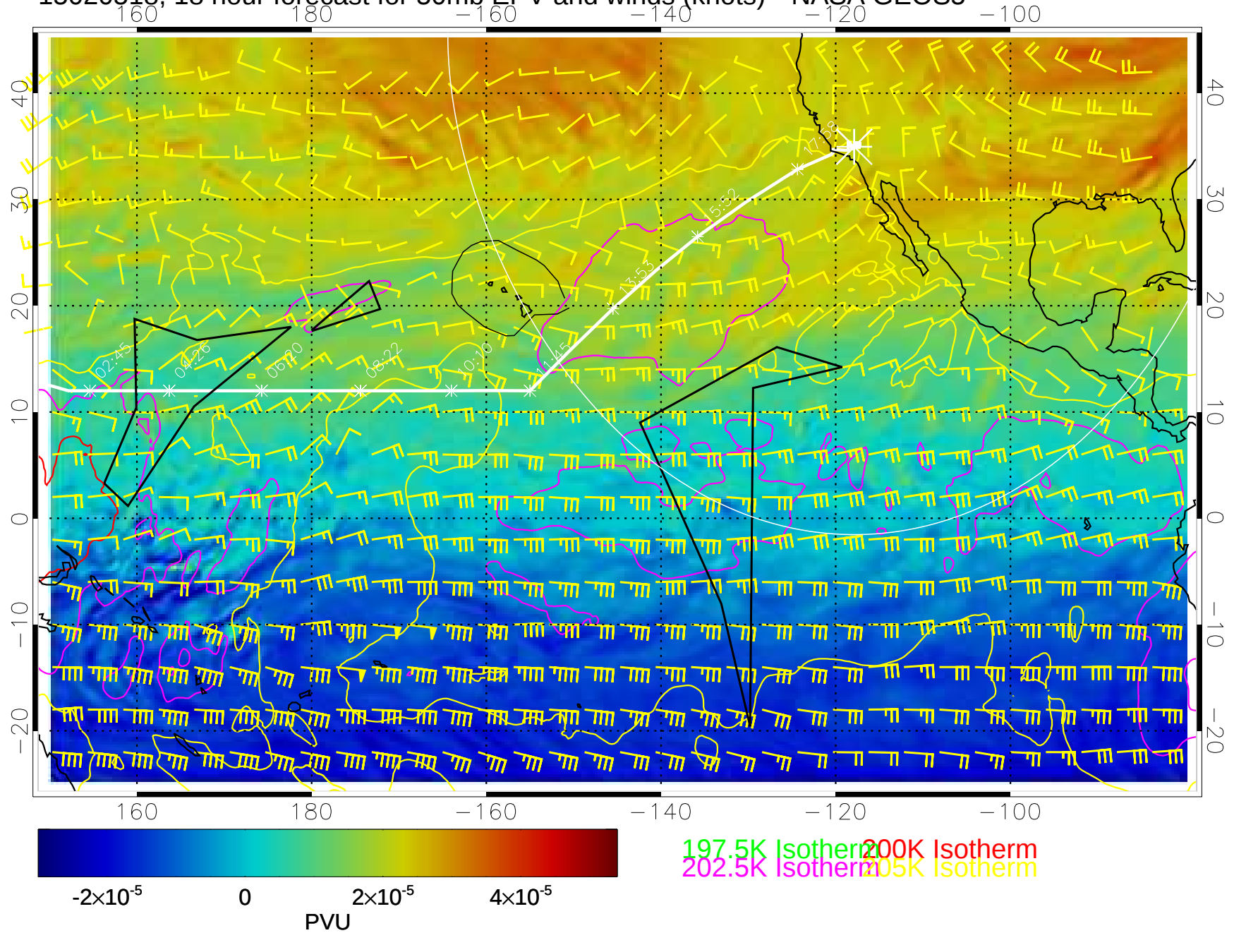
15020518, 18 hour forecast for 50mb EPV and winds (knots)-- NASA GEOS5
