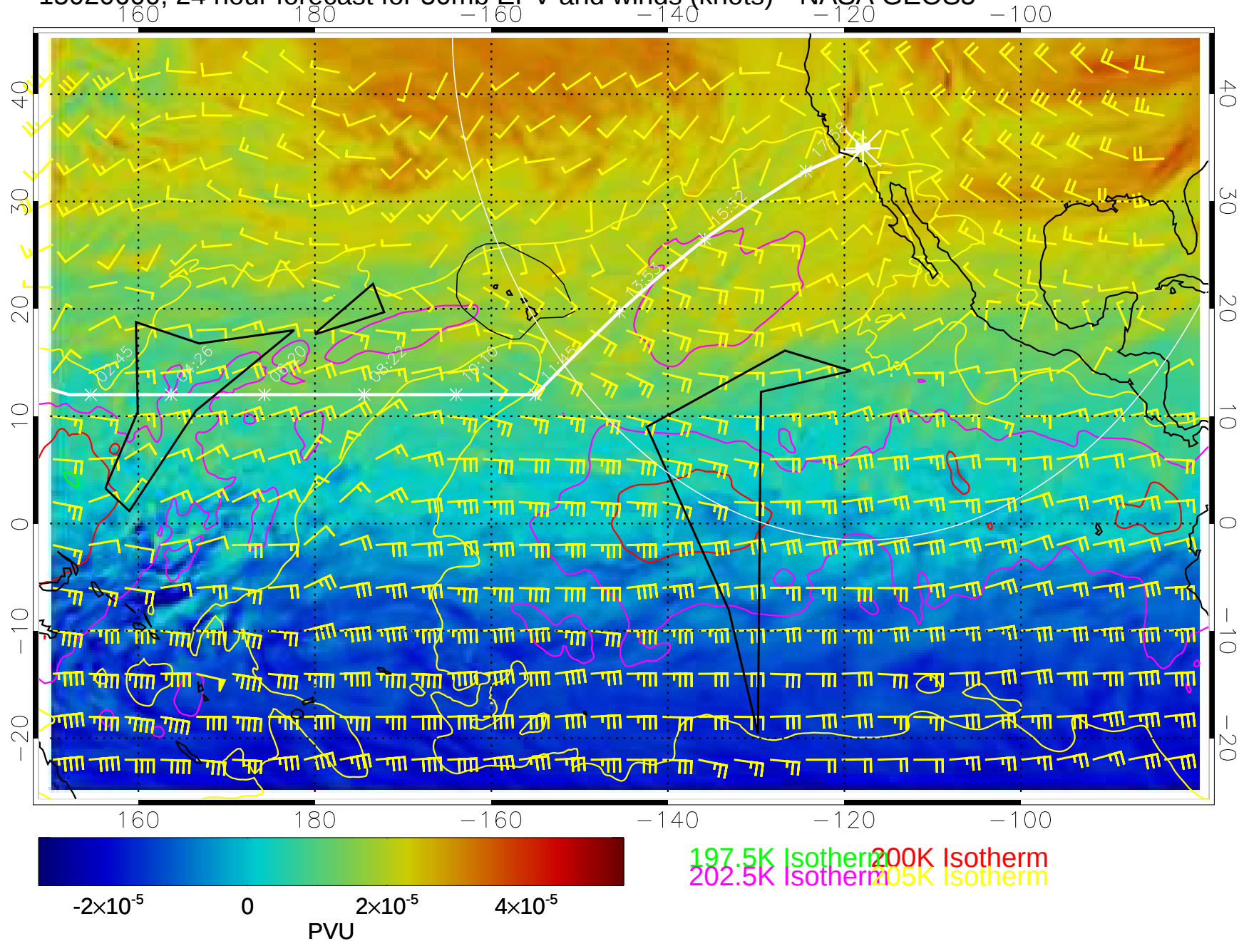
15020600, 24 hour forecast for 50mb EPV and winds (knots)-- NASA GEOS5
