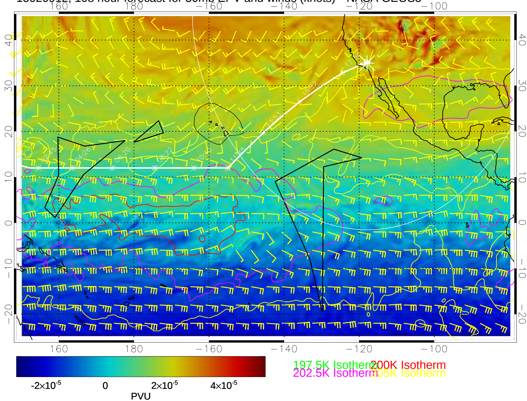
15020912, 108 hour forecast for 50mb EPV and winds (knots)-- NASA GEOS5
