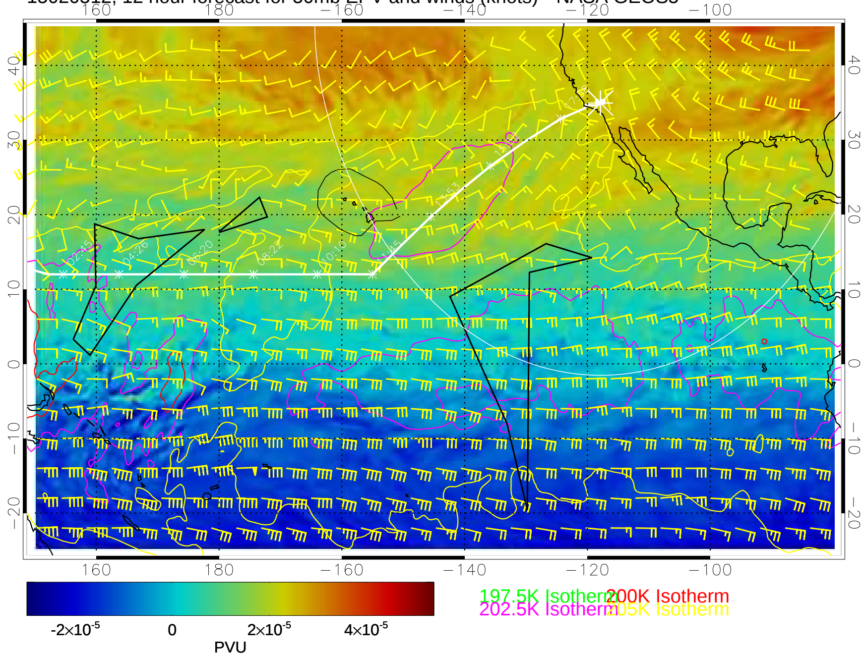
15020512, 12 hour forecast for 50mb EPV and winds (knots)-- NASA GEOS5
