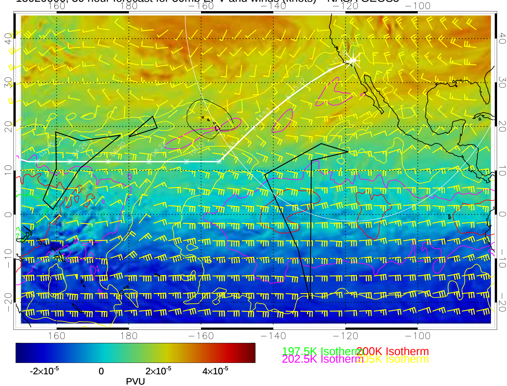
15020606, 30 hour forecast for 50mb EPV and winds (knots)-- NASA GEOS5
