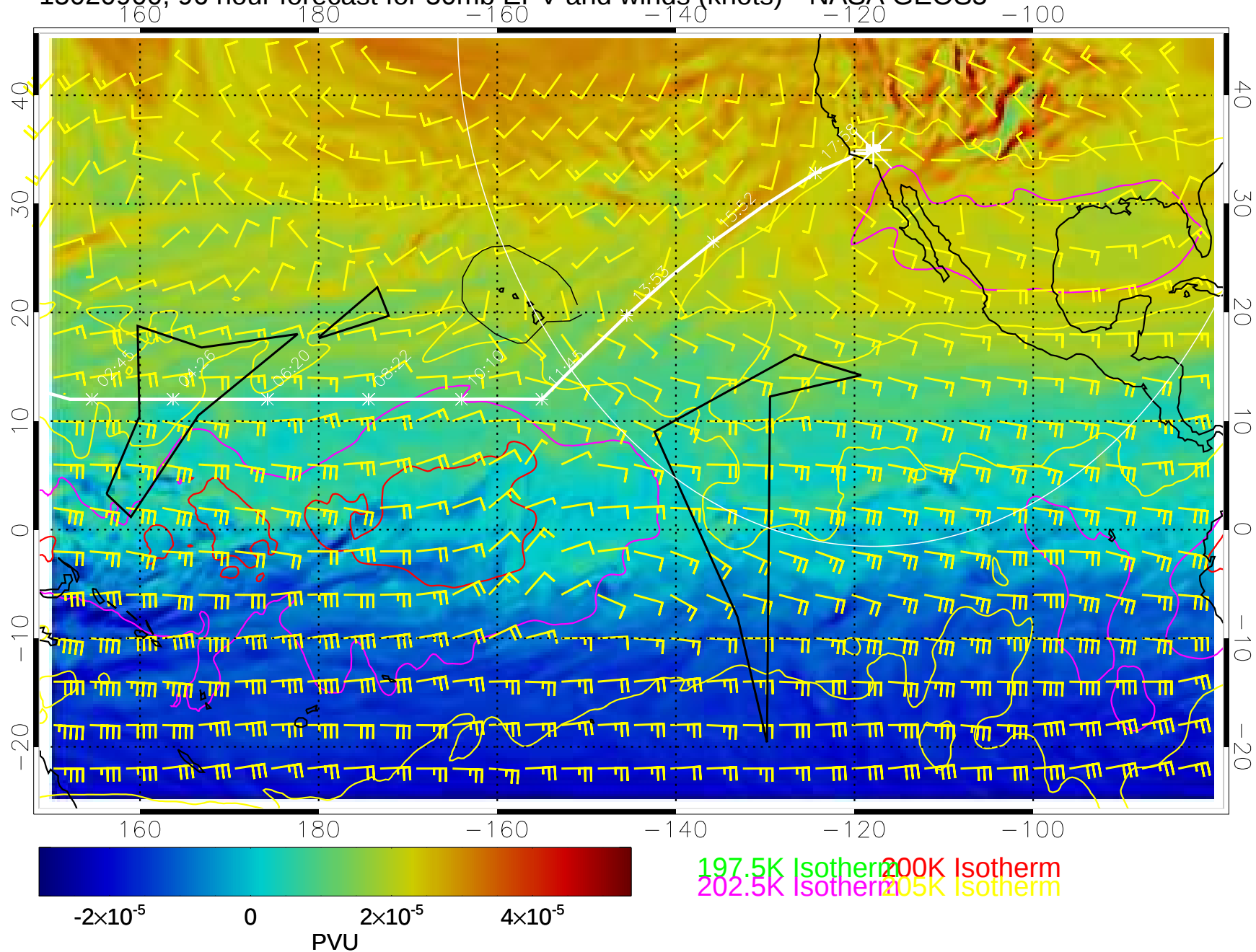
15020900, 96 hour forecast for 50mb EPV and winds (knots)-- NASA GEOS5
