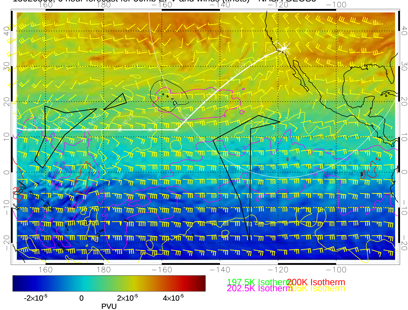
15020506, 6 hour forecast for 50mb EPV and winds (knots)-- NASA GEOS5
