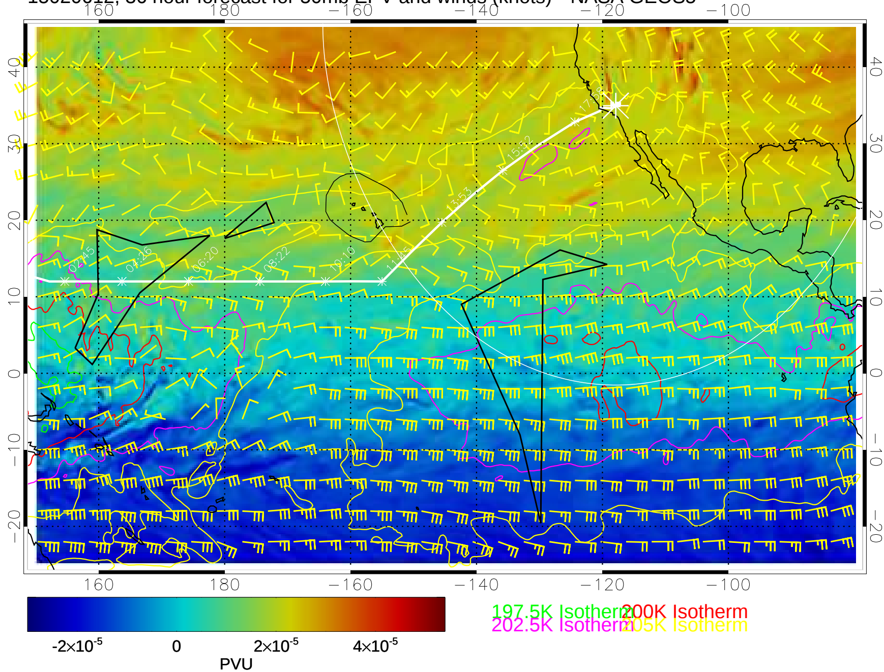
15020612, 36 hour forecast for 50mb EPV and winds (knots)-- NASA GEOS5
