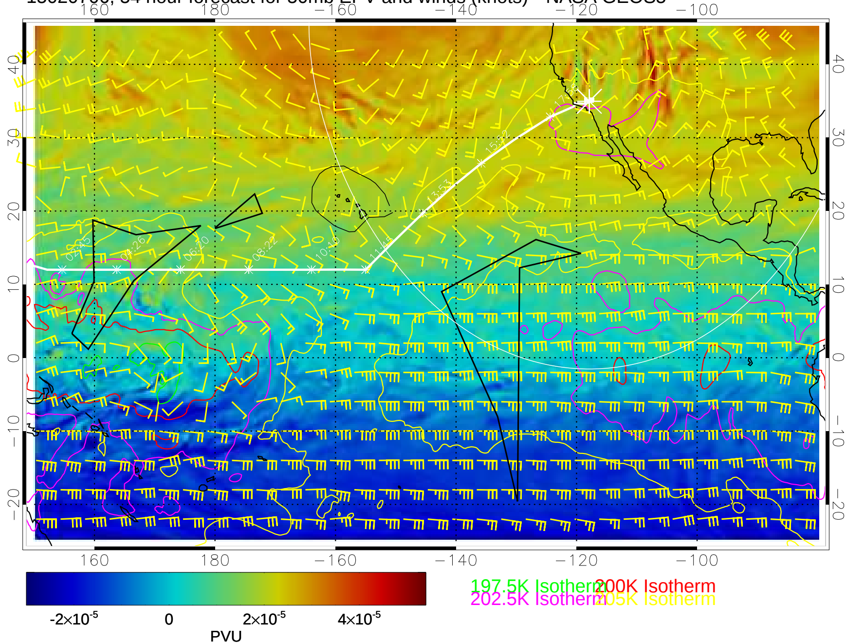
15020706, 54 hour forecast for 50mb EPV and winds (knots)-- NASA GEOS5
