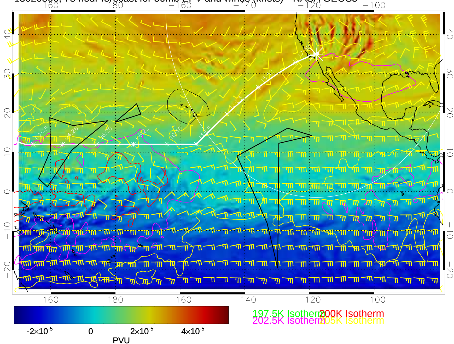
15020806, 78 hour forecast for 50mb EPV and winds (knots)-- NASA GEOS5
