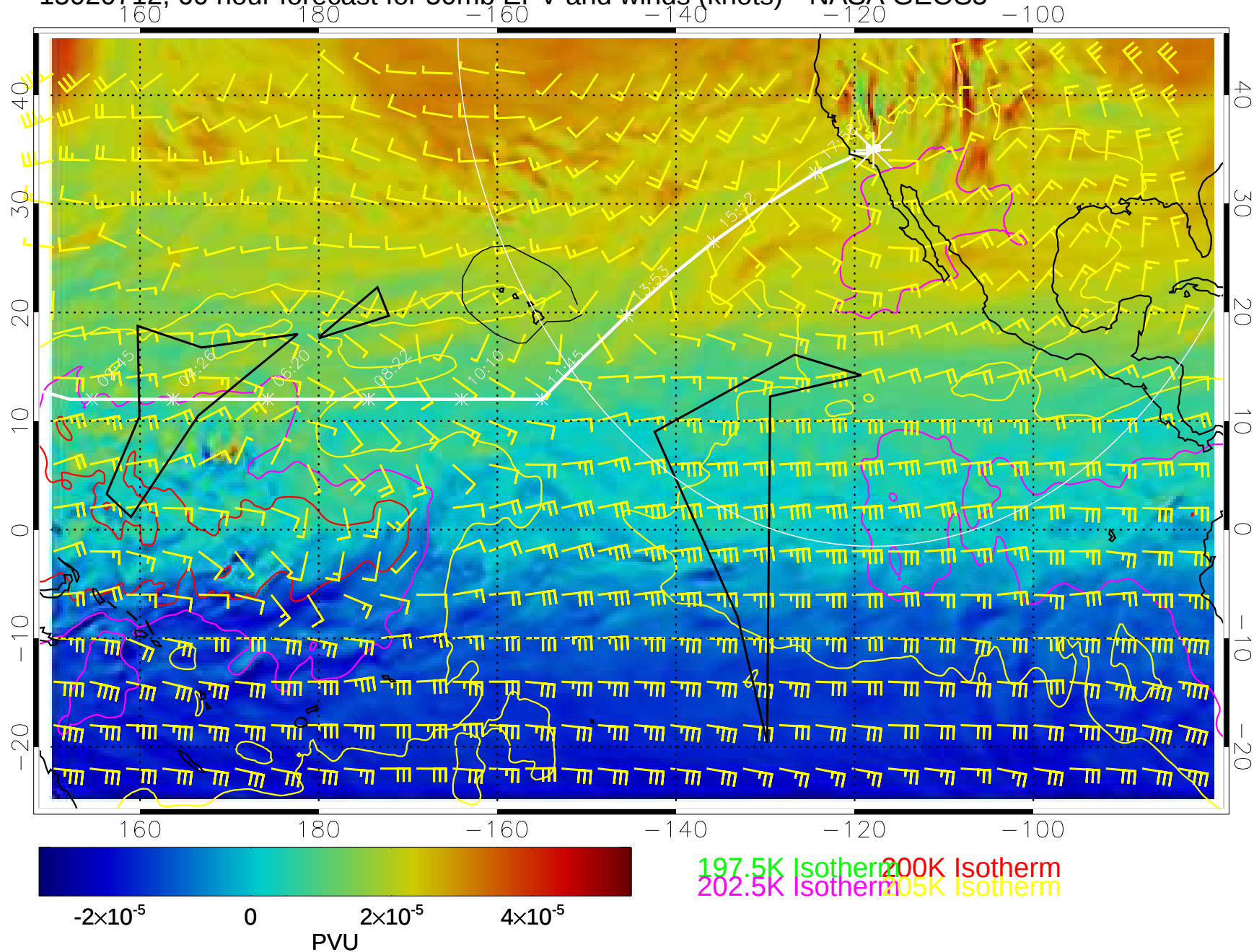
15020712, 60 hour forecast for 50mb EPV and winds (knots)-- NASA GEOS5
