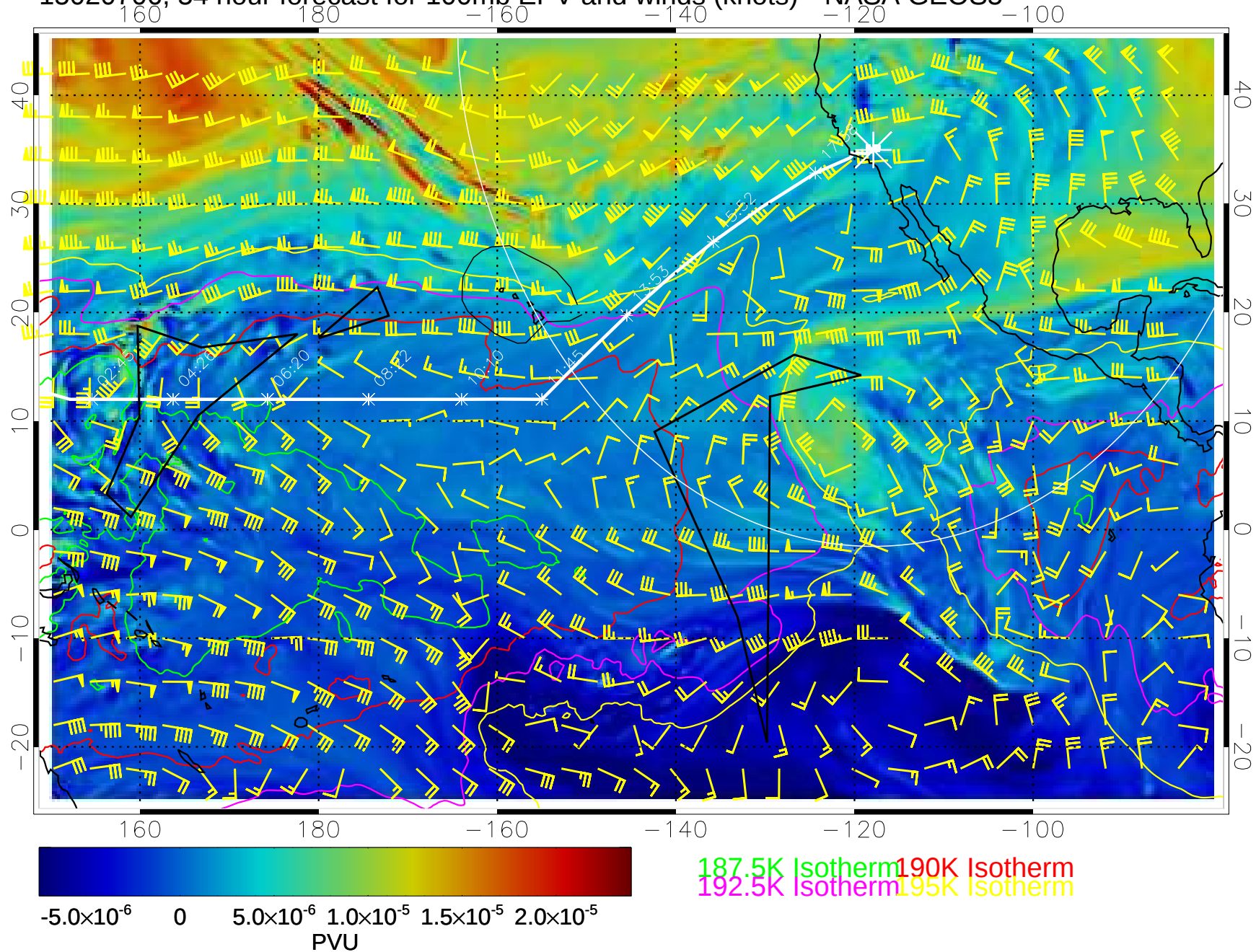
15020706, 54 hour forecast for 100mb EPV and winds (knots)-- NASA GEOS5
