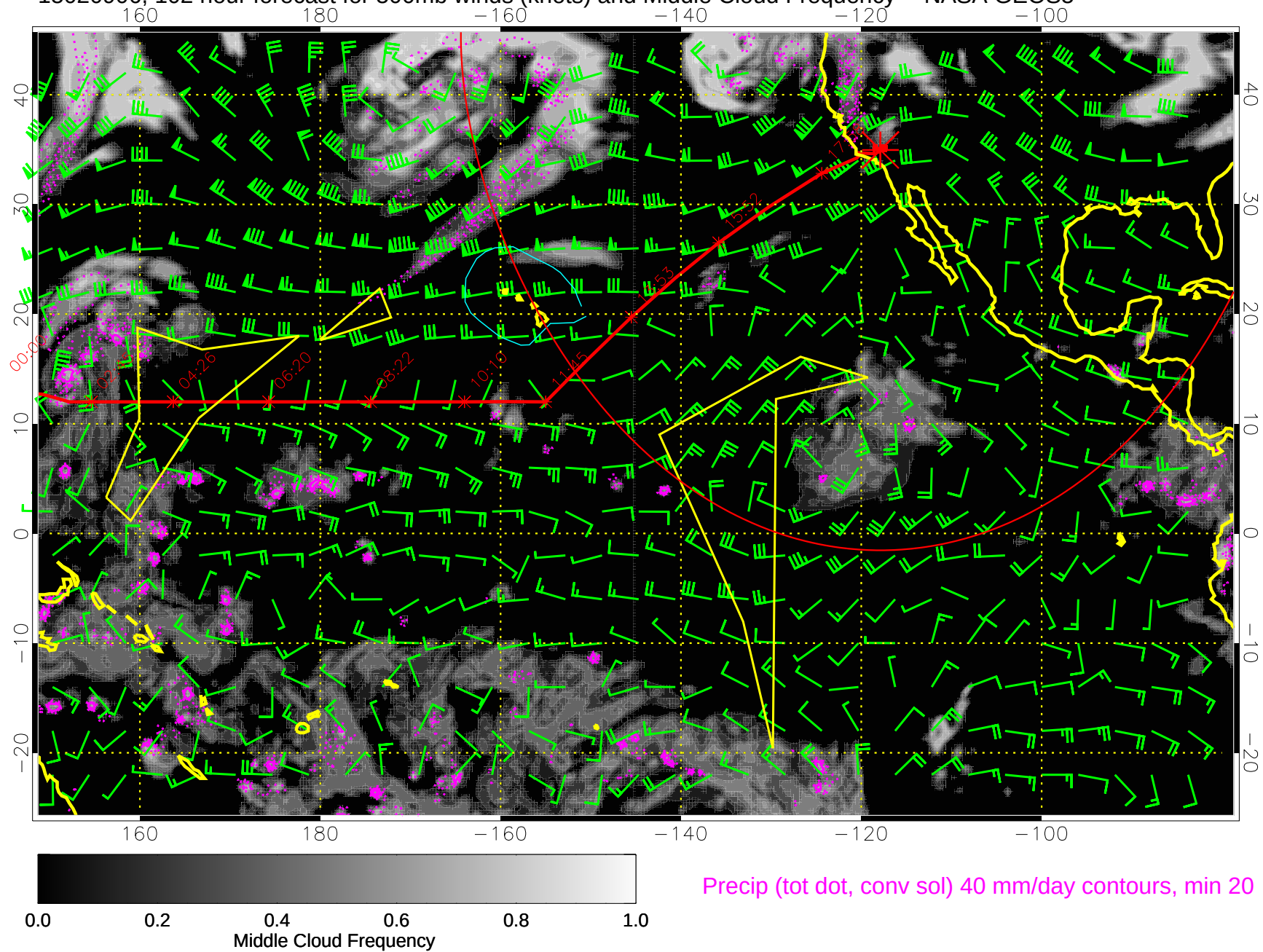
15020906, 102 hour forecast for 500mb winds (knots) and Middle Cloud Frequency -- NASA GEOS5
