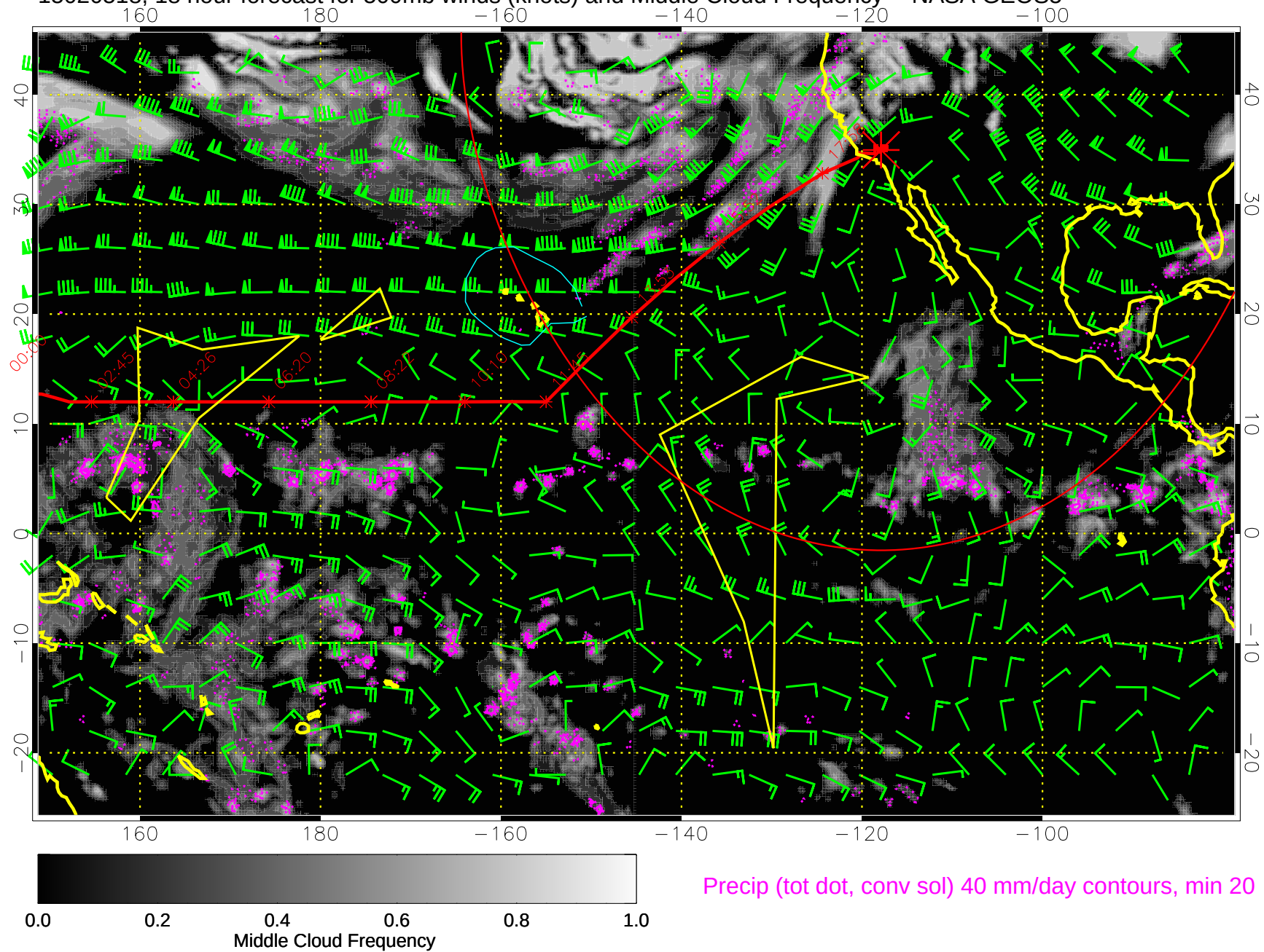
15020518, 18 hour forecast for 500mb winds (knots) and Middle Cloud Frequency -- NASA GEOS5
