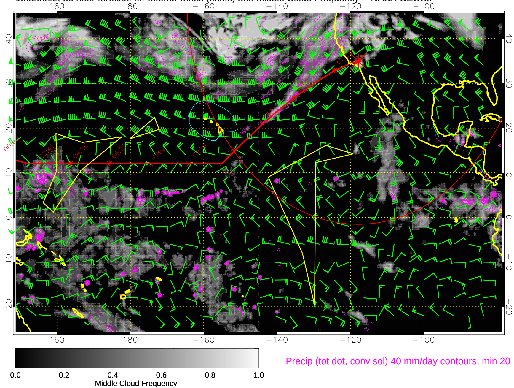
15020612, 36 hour forecast for 500mb winds (knots) and Middle Cloud Frequency -- NASA GEOS5
