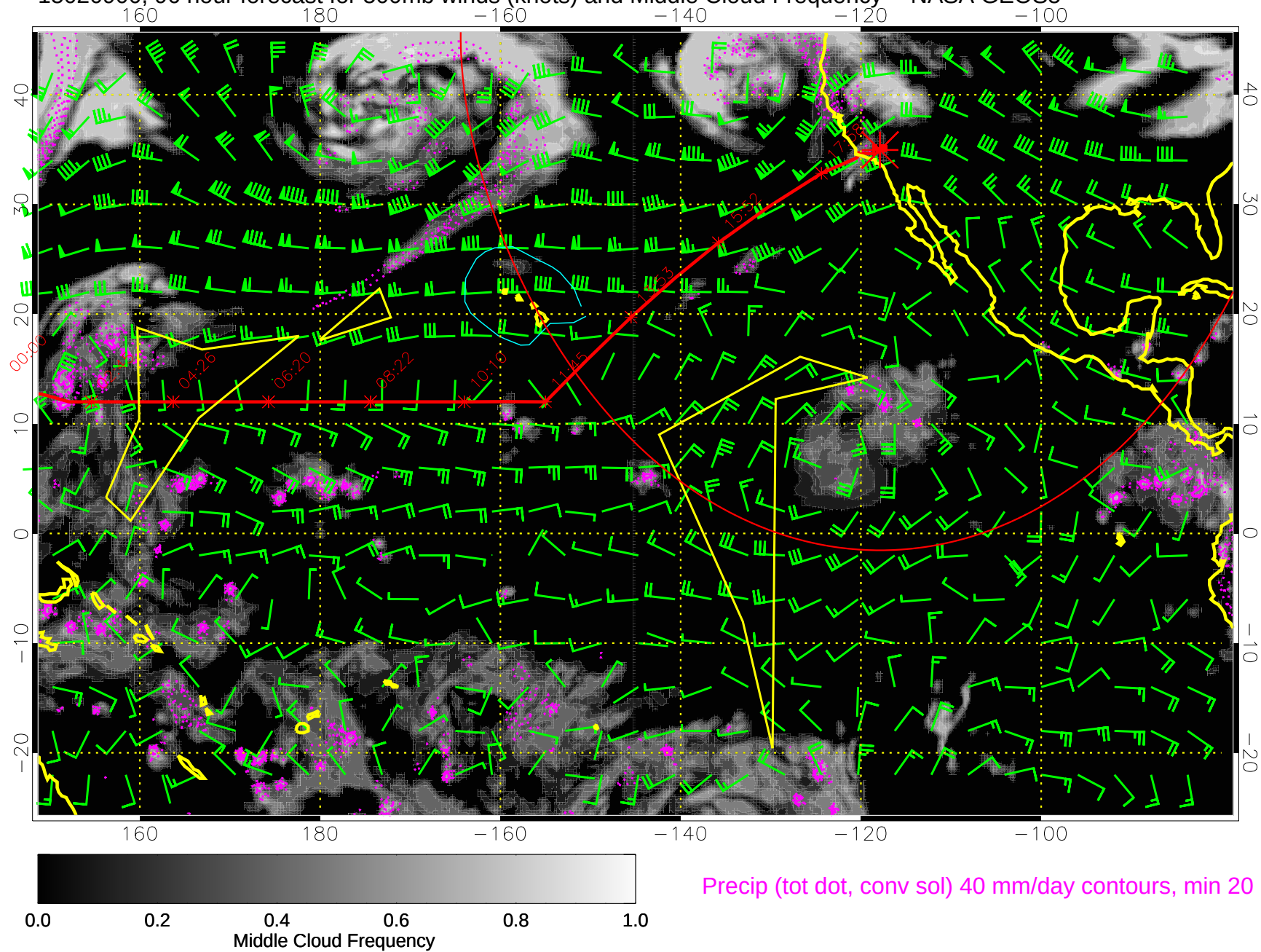
15020900, 96 hour forecast for 500mb winds (knots) and Middle Cloud Frequency -- NASA GEOS5
