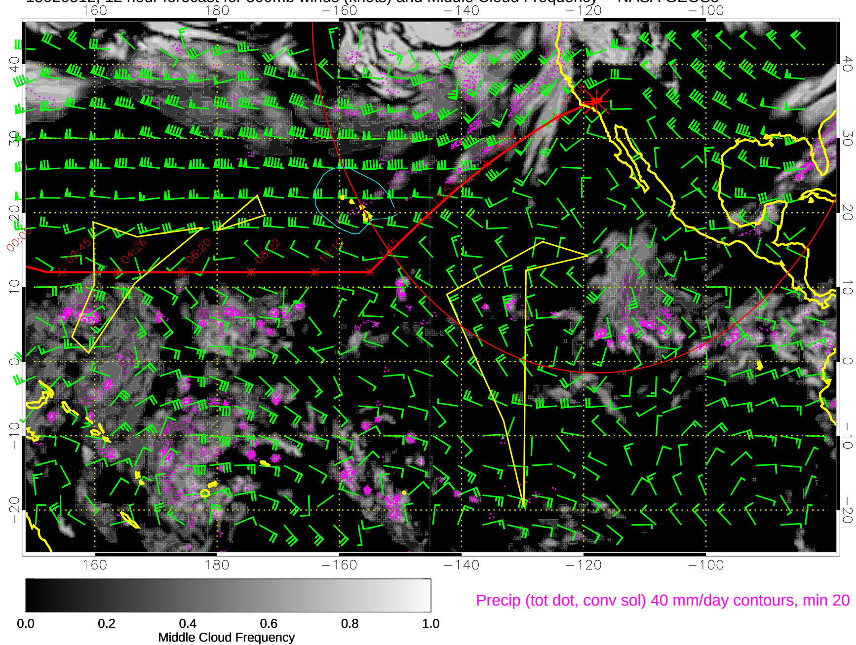
15020512, 12 hour forecast for 500mb winds (knots) and Middle Cloud Frequency -- NASA GEOS5
