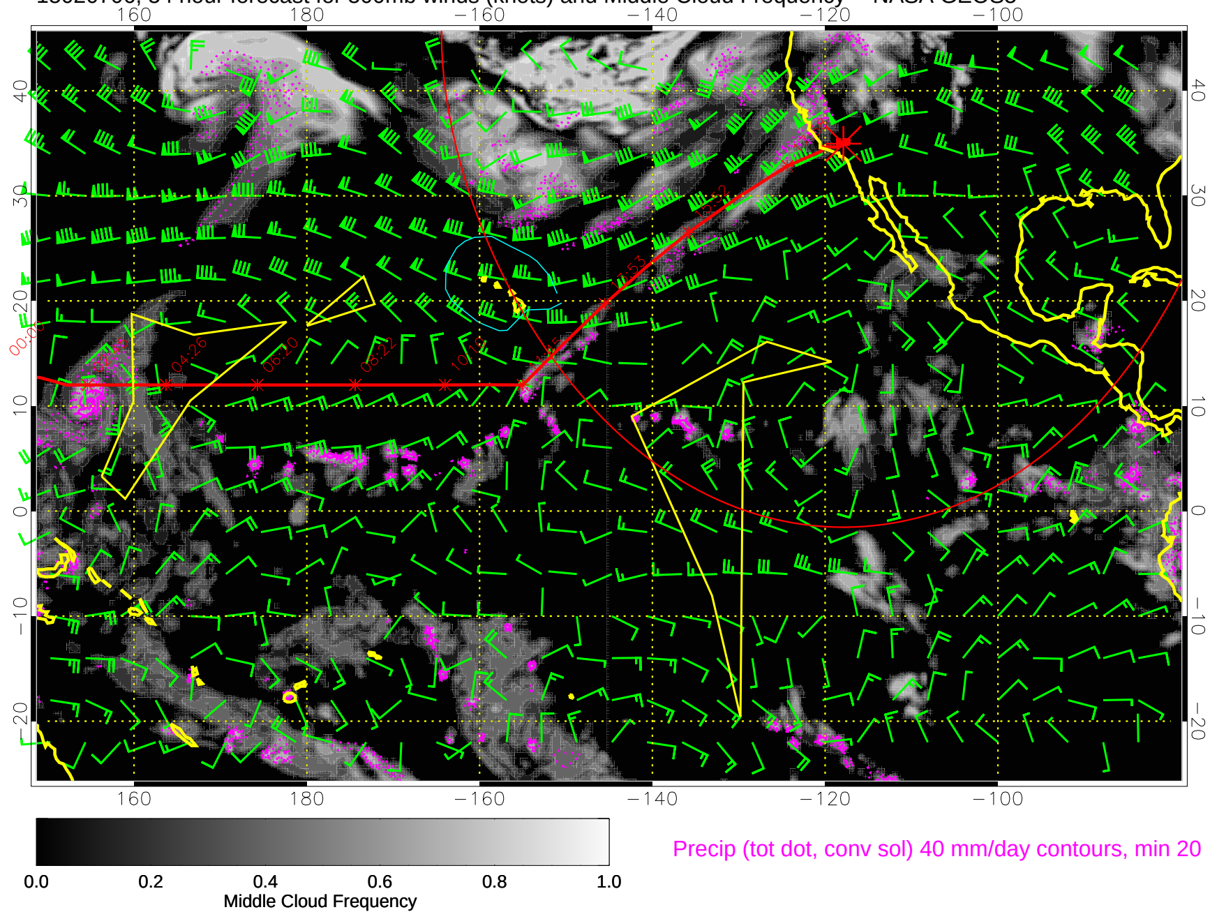
15020706, 54 hour forecast for 500mb winds (knots) and Middle Cloud Frequency -- NASA GEOS5
