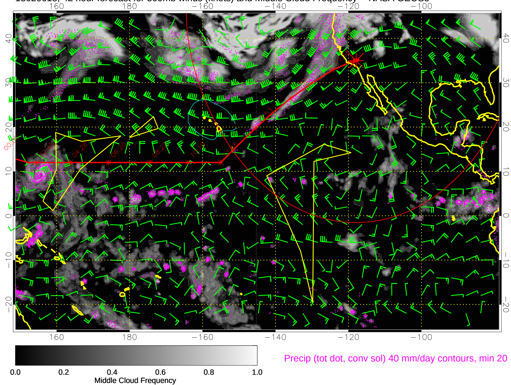
15020618, 42 hour forecast for 500mb winds (knots) and Middle Cloud Frequency -- NASA GEOS5
