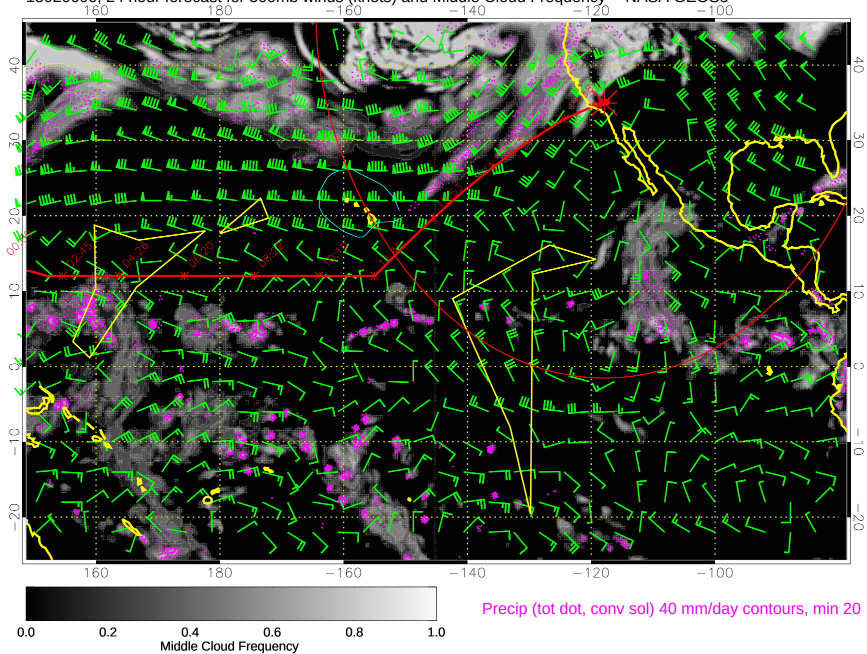
15020600, 24 hour forecast for 500mb winds (knots) and Middle Cloud Frequency -- NASA GEOS5
