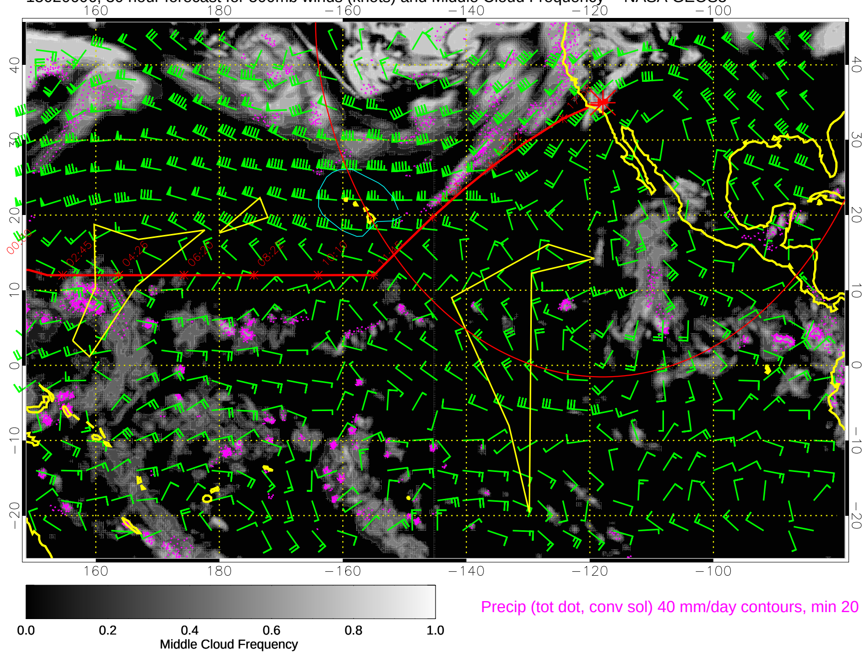
15020606, 30 hour forecast for 500mb winds (knots) and Middle Cloud Frequency -- NASA GEOS5
