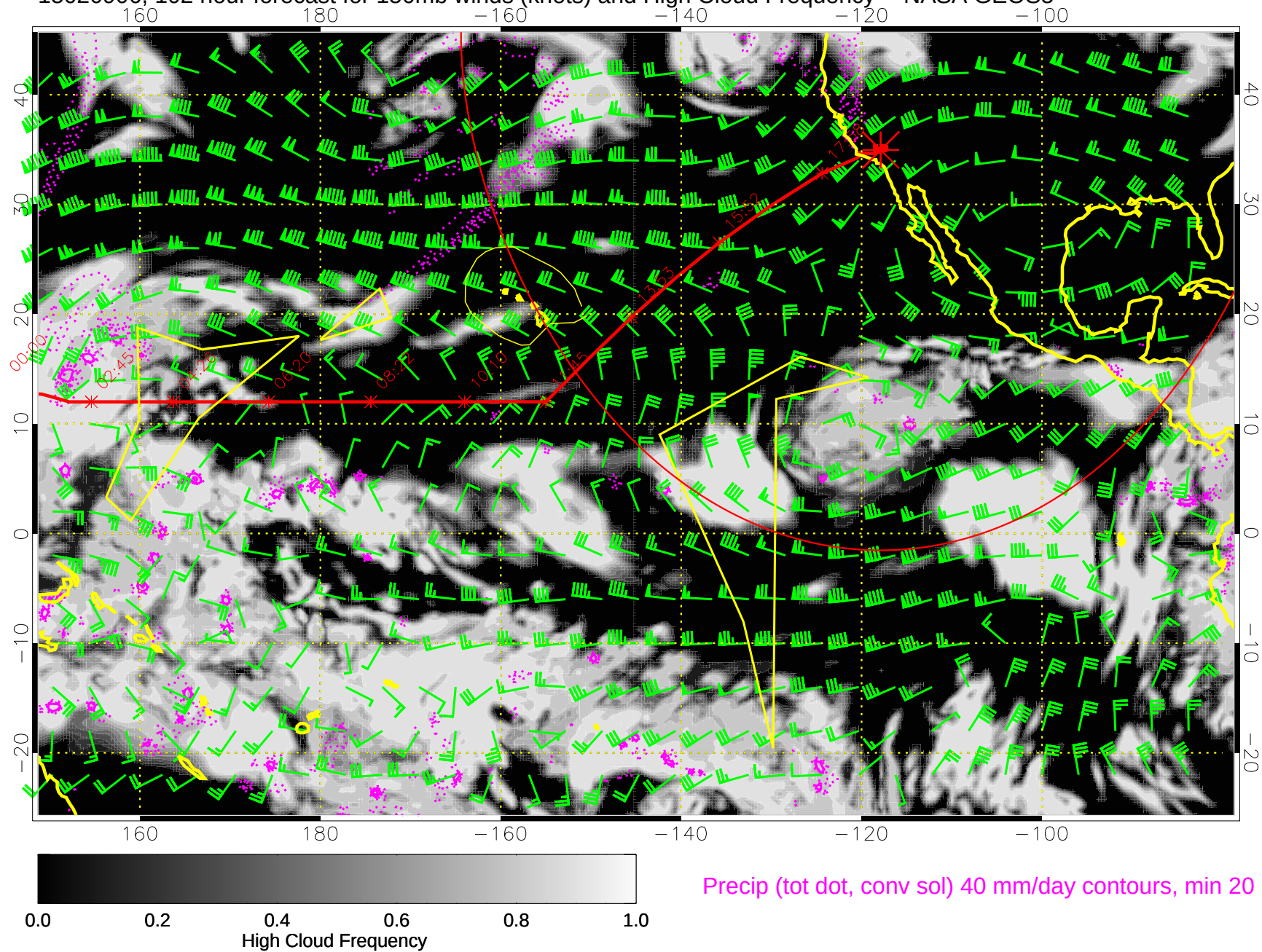
15020906, 102 hour forecast for 150mb winds (knots) and High Cloud Frequency -- NASA GEOS5
