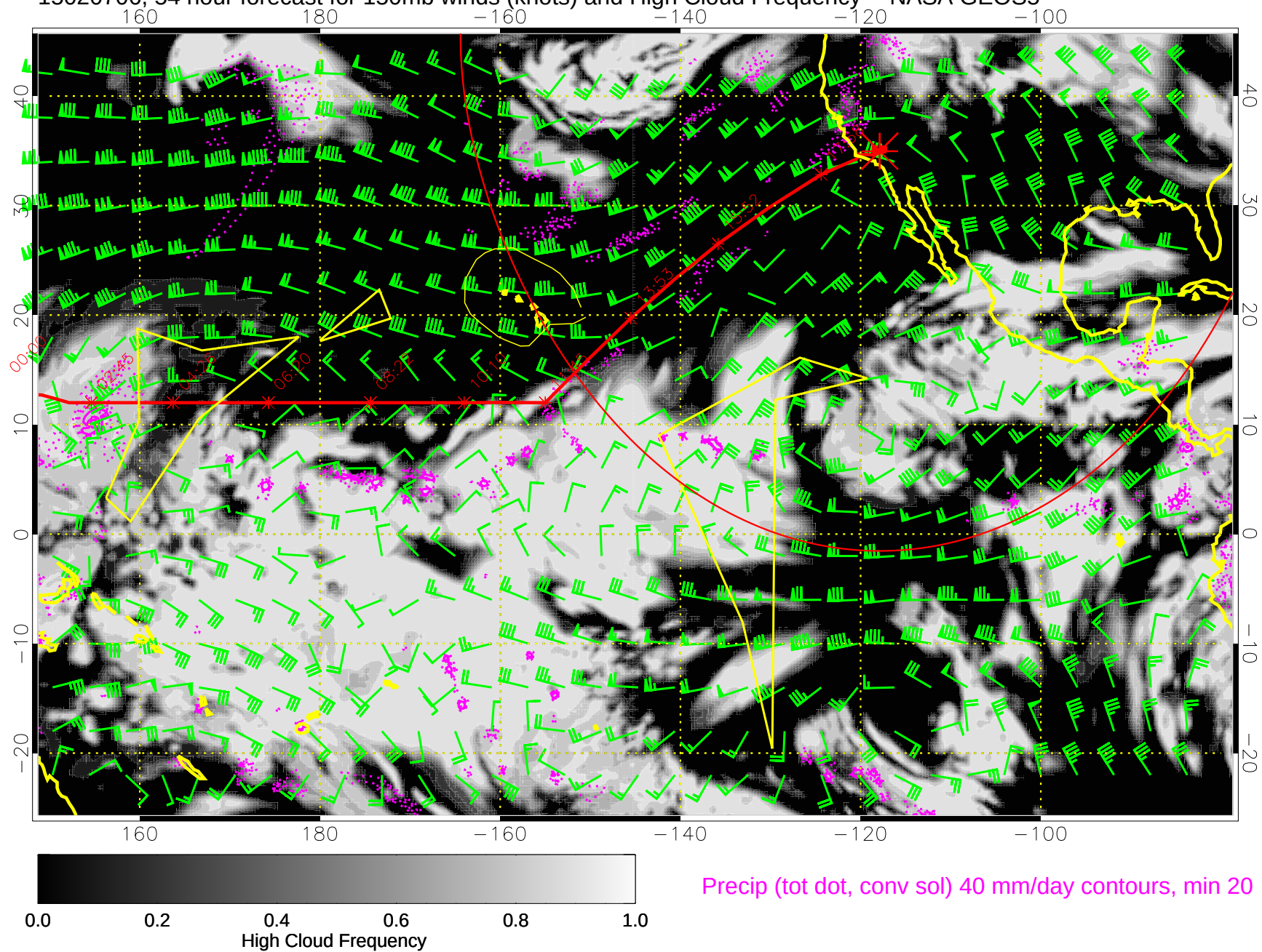
15020706, 54 hour forecast for 150mb winds (knots) and High Cloud Frequency -- NASA GEOS5
