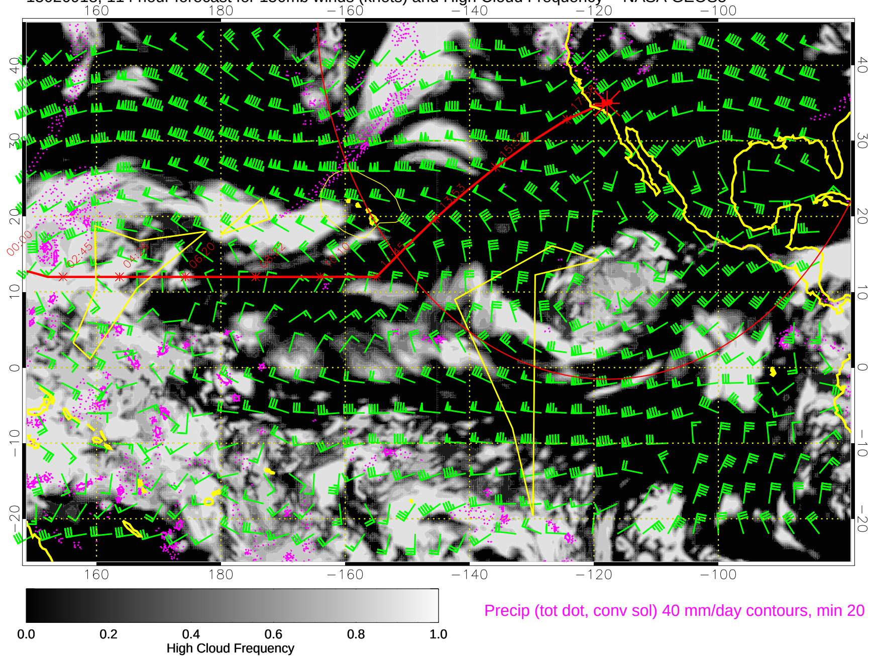
15020918, 114 hour forecast for 150mb winds (knots) and High Cloud Frequency -- NASA GEOS5
