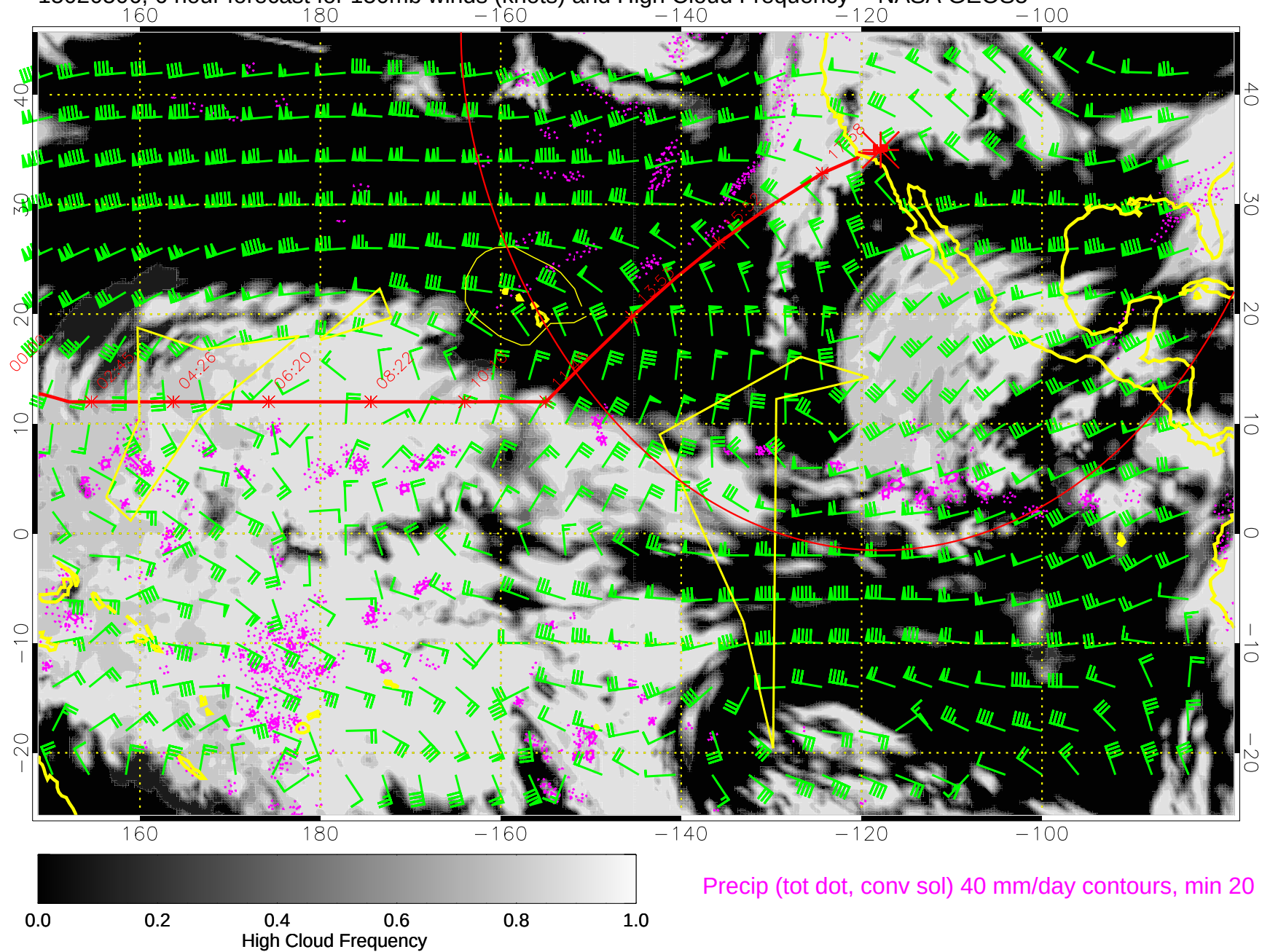
15020506, 6 hour forecast for 150mb winds (knots) and High Cloud Frequency -- NASA GEOS5
