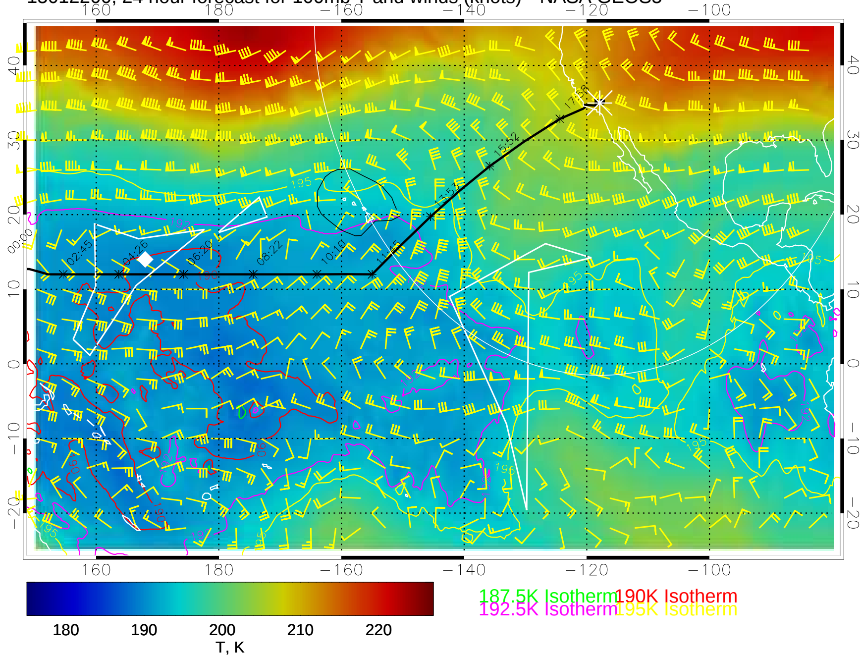
15012200, 24 hour forecast for 100mb T and winds (knots)-- NASA GEOS5
