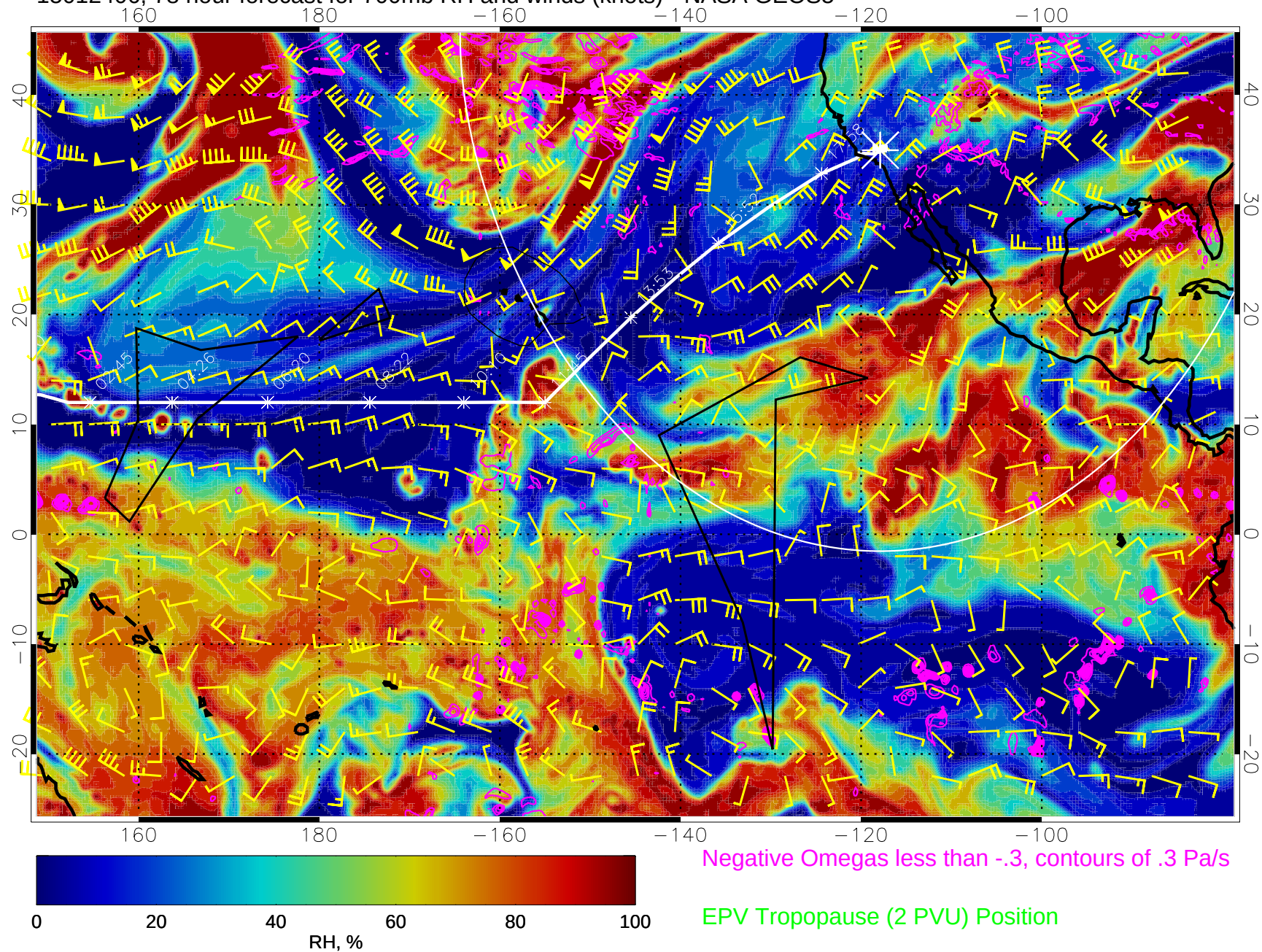
15012406, 78 hour forecast for 700mb RH and winds (knots) - NASA GEOS5
