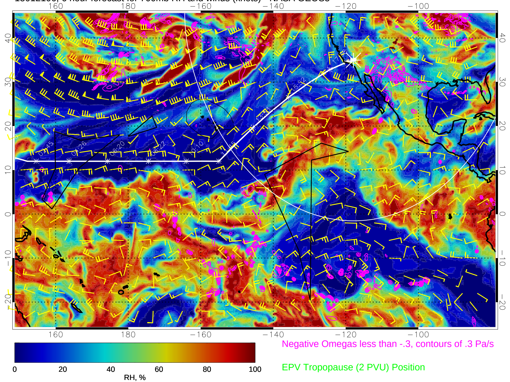
15012106, 6 hour forecast for 700mb RH and winds (knots) - NASA GEOS5
