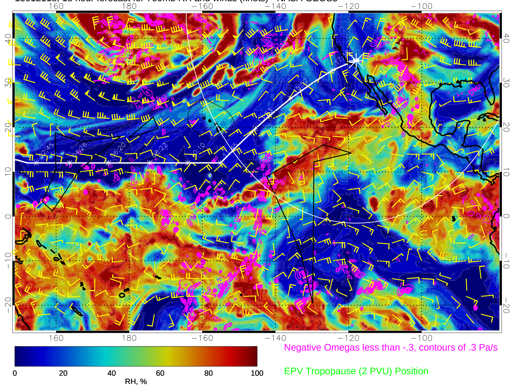
15012118, 18 hour forecast for 700mb RH and winds (knots) - NASA GEOS5
