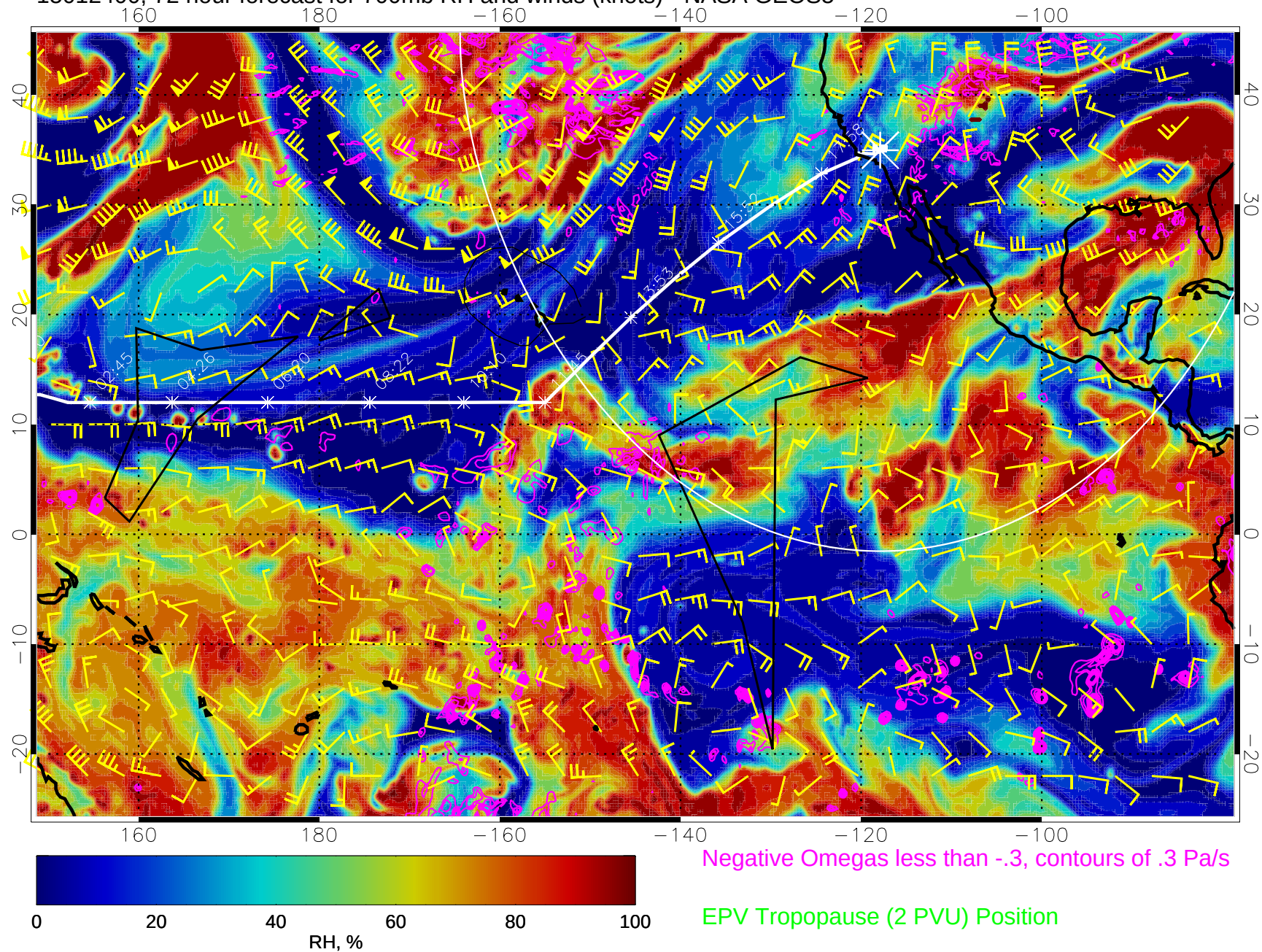
15012400, 72 hour forecast for 700mb RH and winds (knots) - NASA GEOS5
