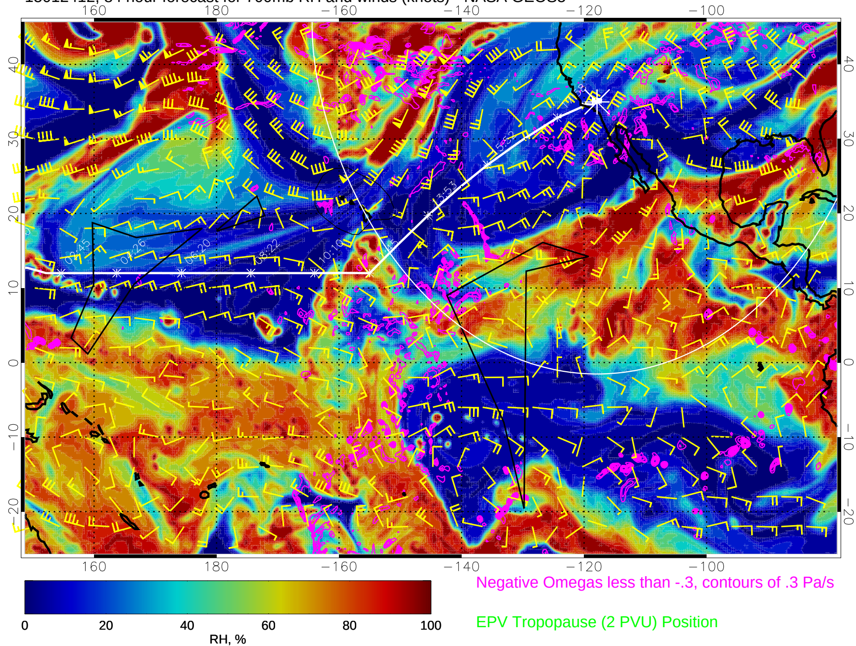
15012412, 84 hour forecast for 700mb RH and winds (knots) - NASA GEOS5
