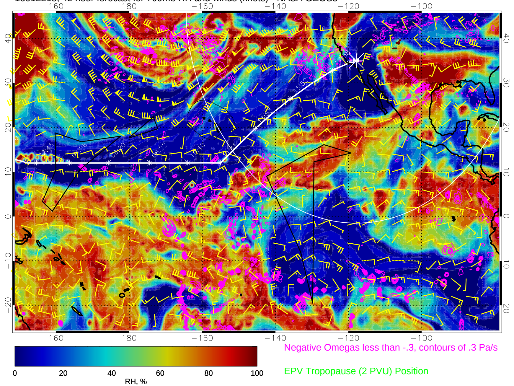
15012218, 42 hour forecast for 700mb RH and winds (knots) - NASA GEOS5
