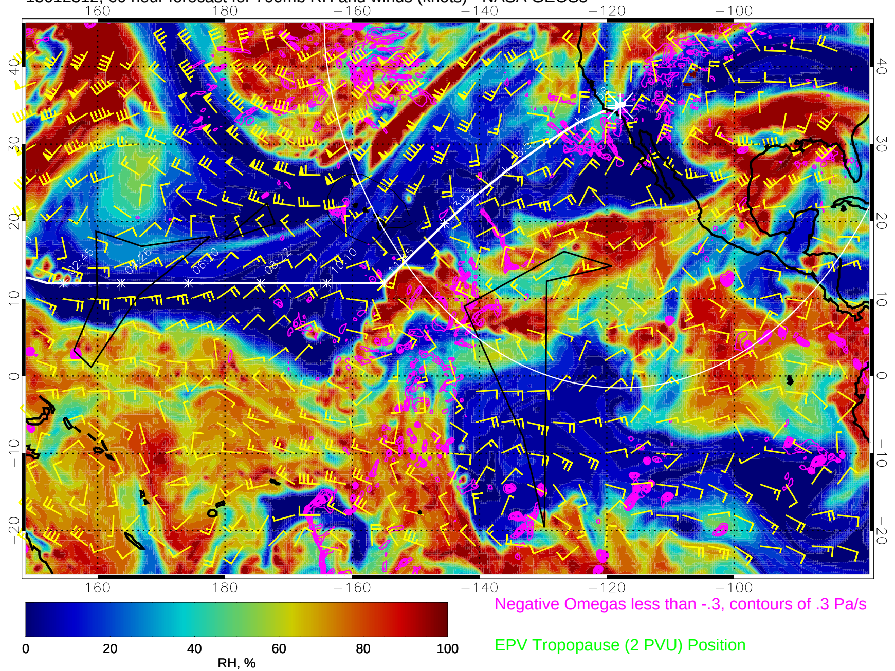
15012312, 60 hour forecast for 700mb RH and winds (knots) - NASA GEOS5
