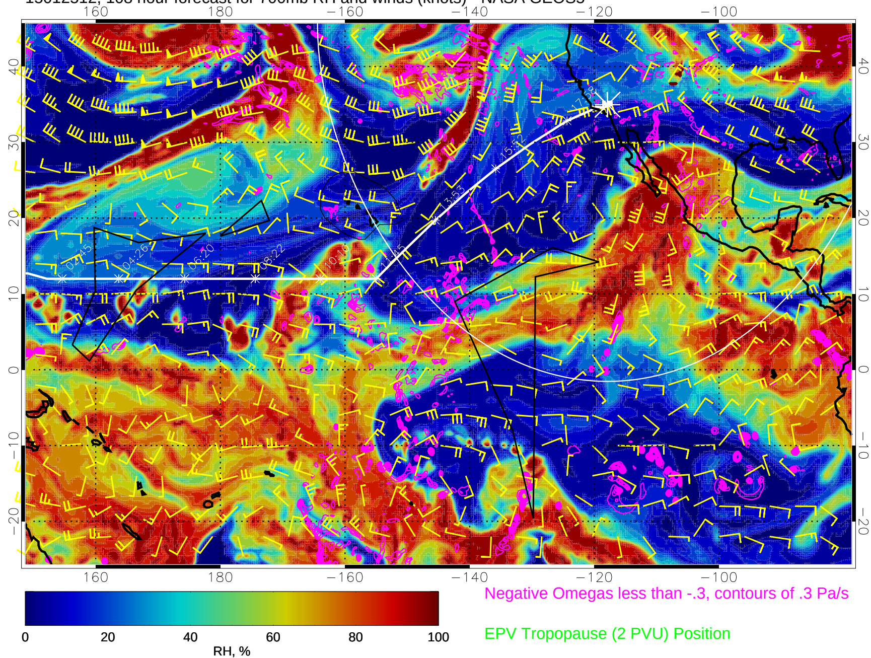
15012512, 108 hour forecast for 700mb RH and winds (knots) - NASA GEOS5
