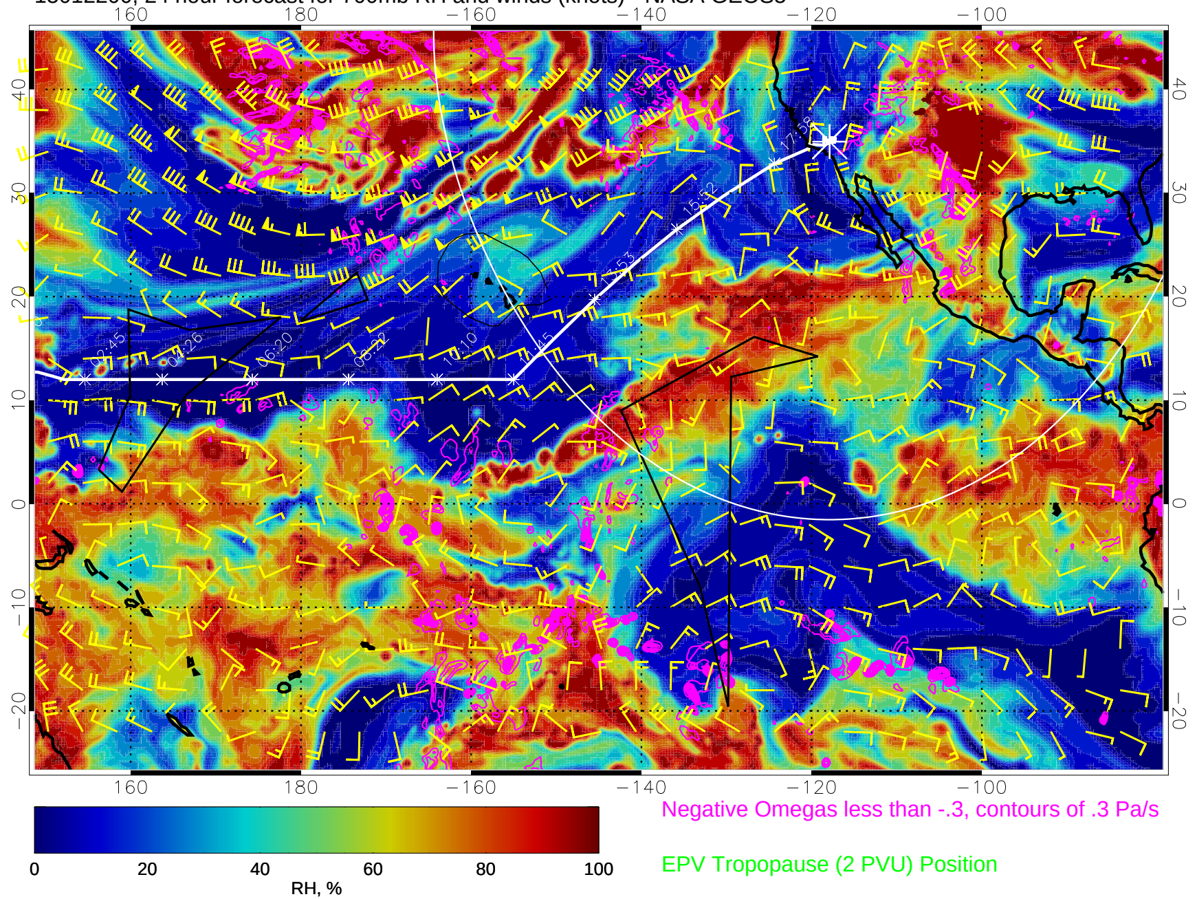
15012200, 24 hour forecast for 700mb RH and winds (knots) - NASA GEOS5
