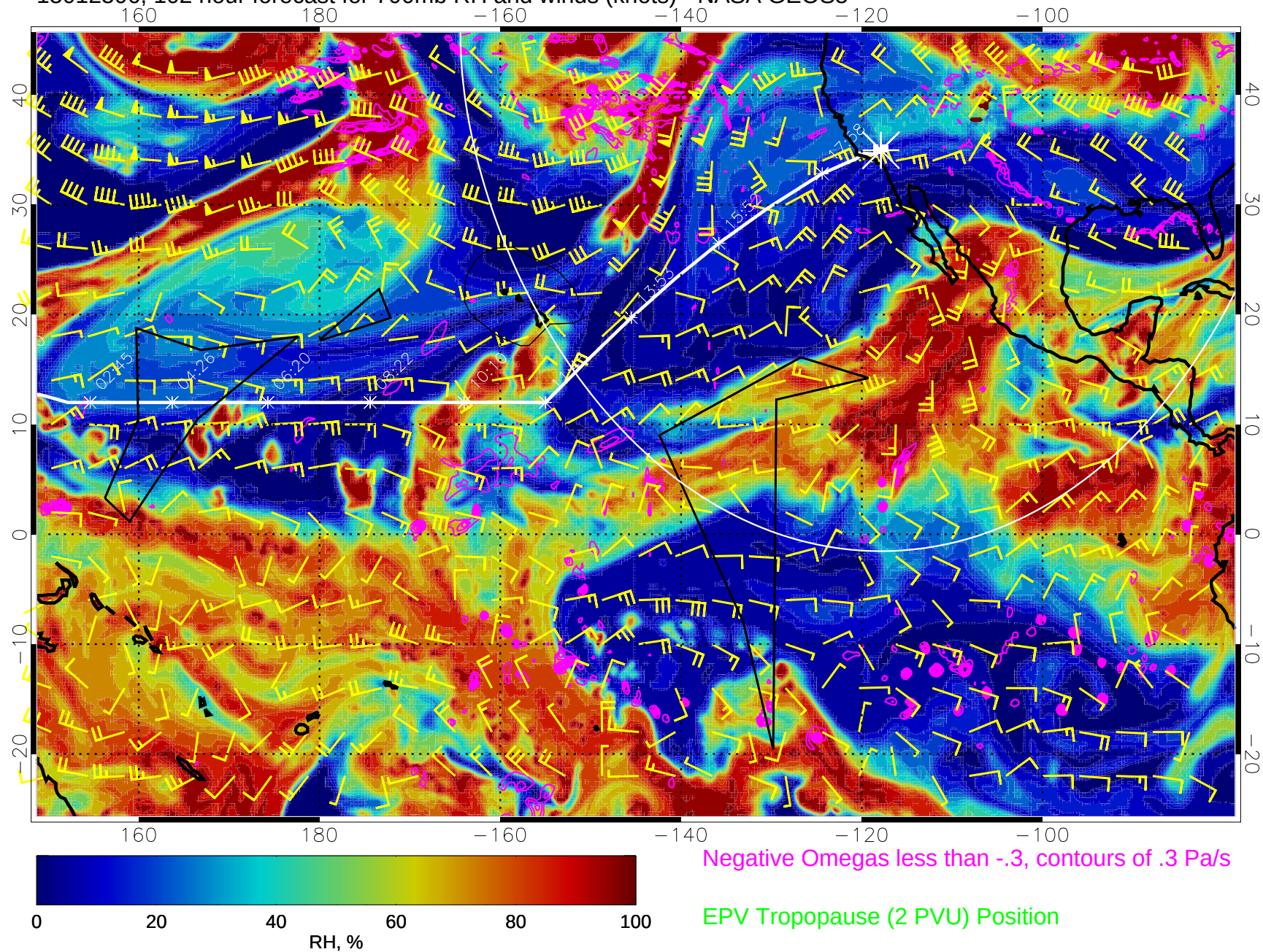
15012506, 102 hour forecast for 700mb RH and winds (knots) - NASA GEOS5
