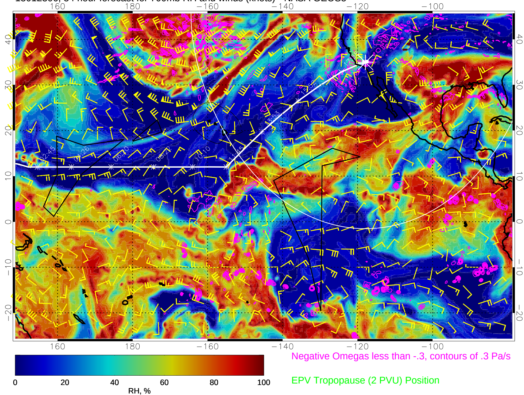
15012306, 54 hour forecast for 700mb RH and winds (knots) - NASA GEOS5
