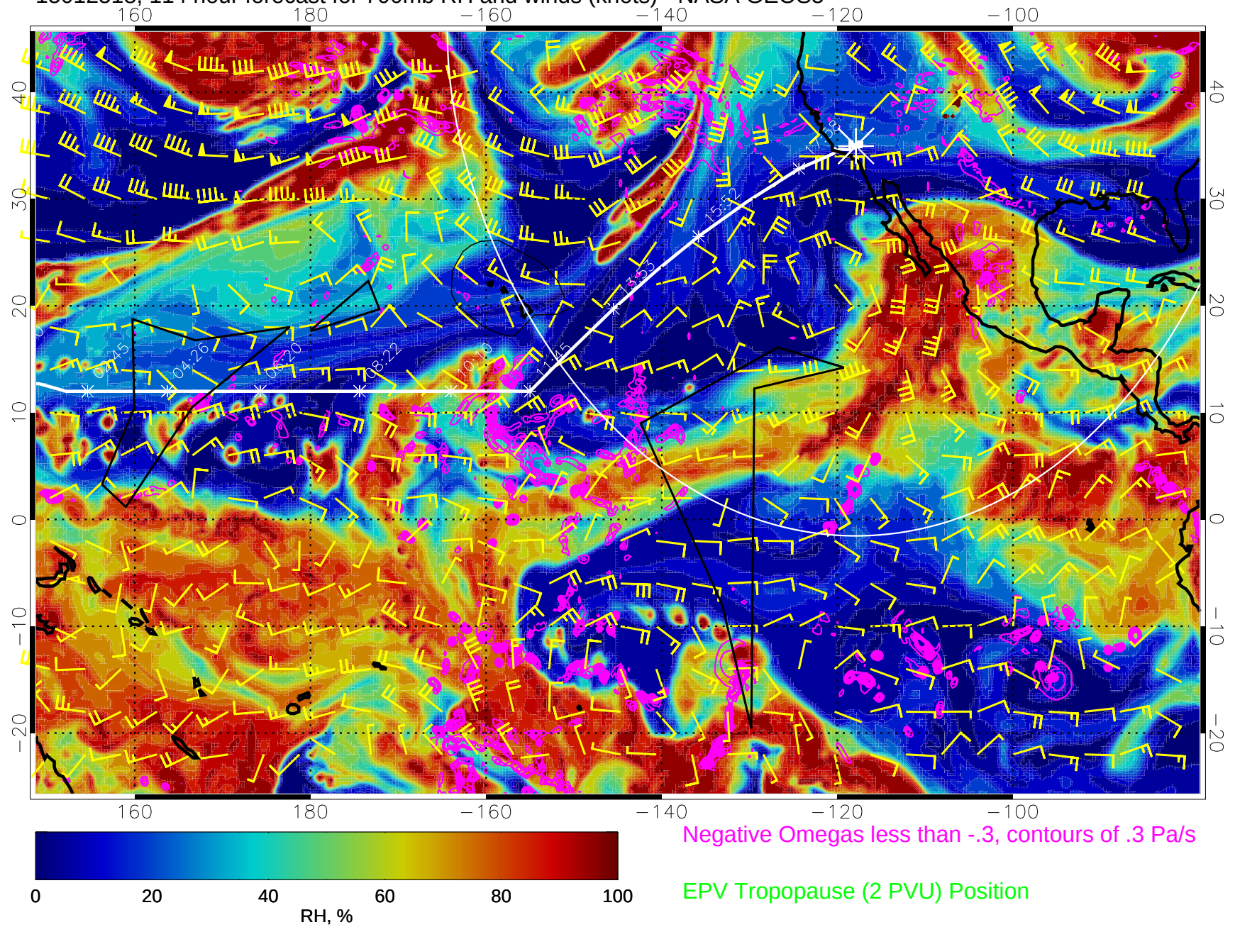
15012518, 114 hour forecast for 700mb RH and winds (knots) - NASA GEOS5
