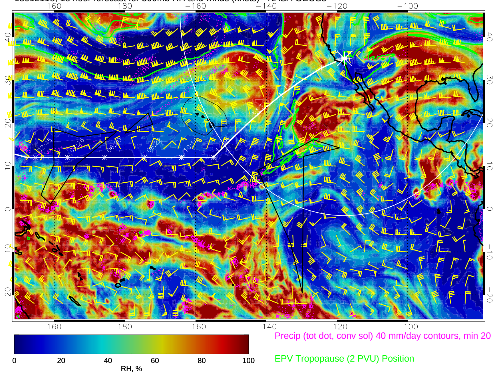
15012118, 18 hour forecast for 300mb RH and winds (knots) - NASA GEOS5
