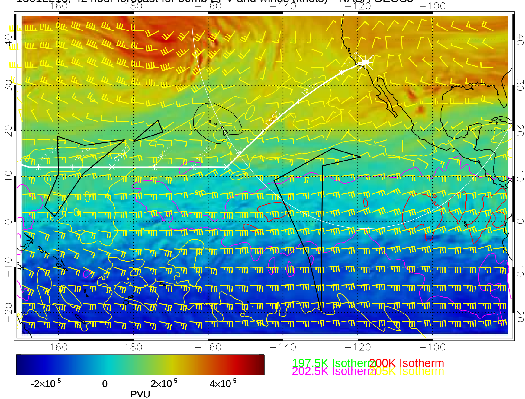
15012218, 42 hour forecast for 50mb EPV and winds (knots)-- NASA GEOS5
