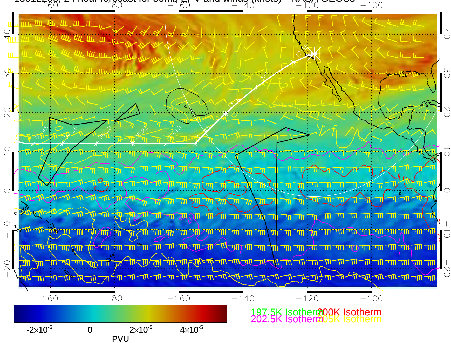
15012200, 24 hour forecast for 50mb EPV and winds (knots)-- NASA GEOS5
