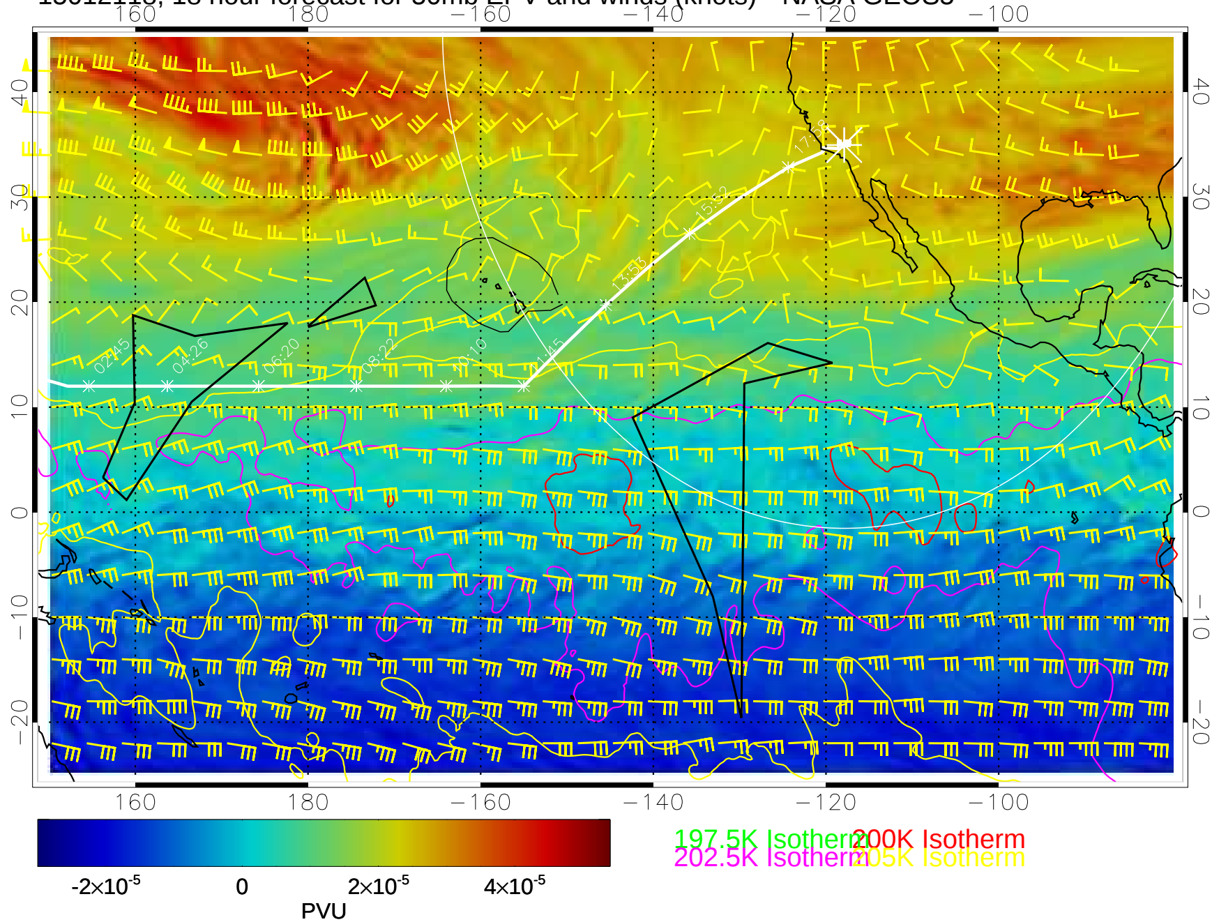
15012118, 18 hour forecast for 50mb EPV and winds (knots)-- NASA GEOS5
