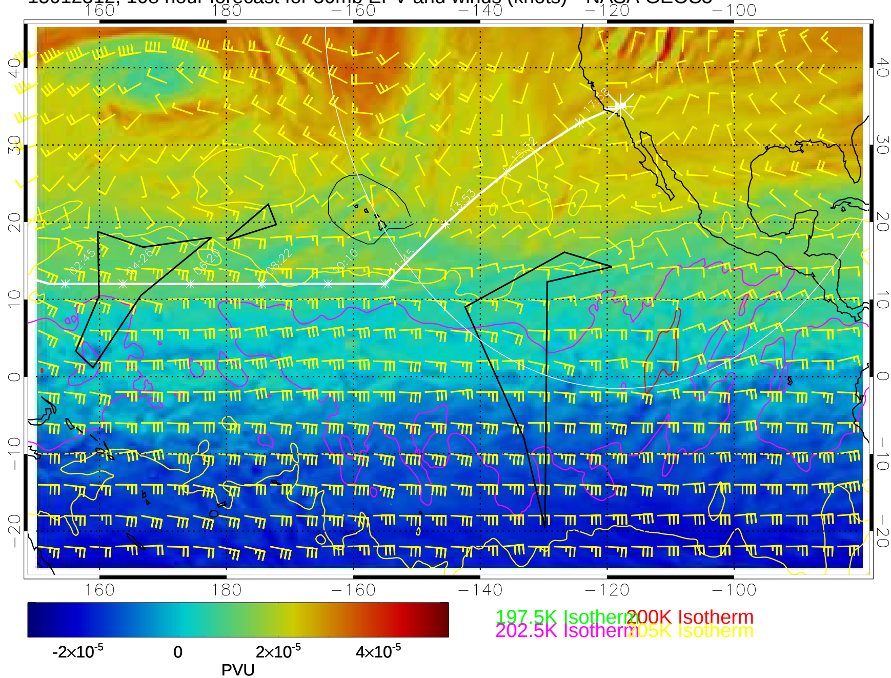
15012512, 108 hour forecast for 50mb EPV and winds (knots)-- NASA GEOS5
