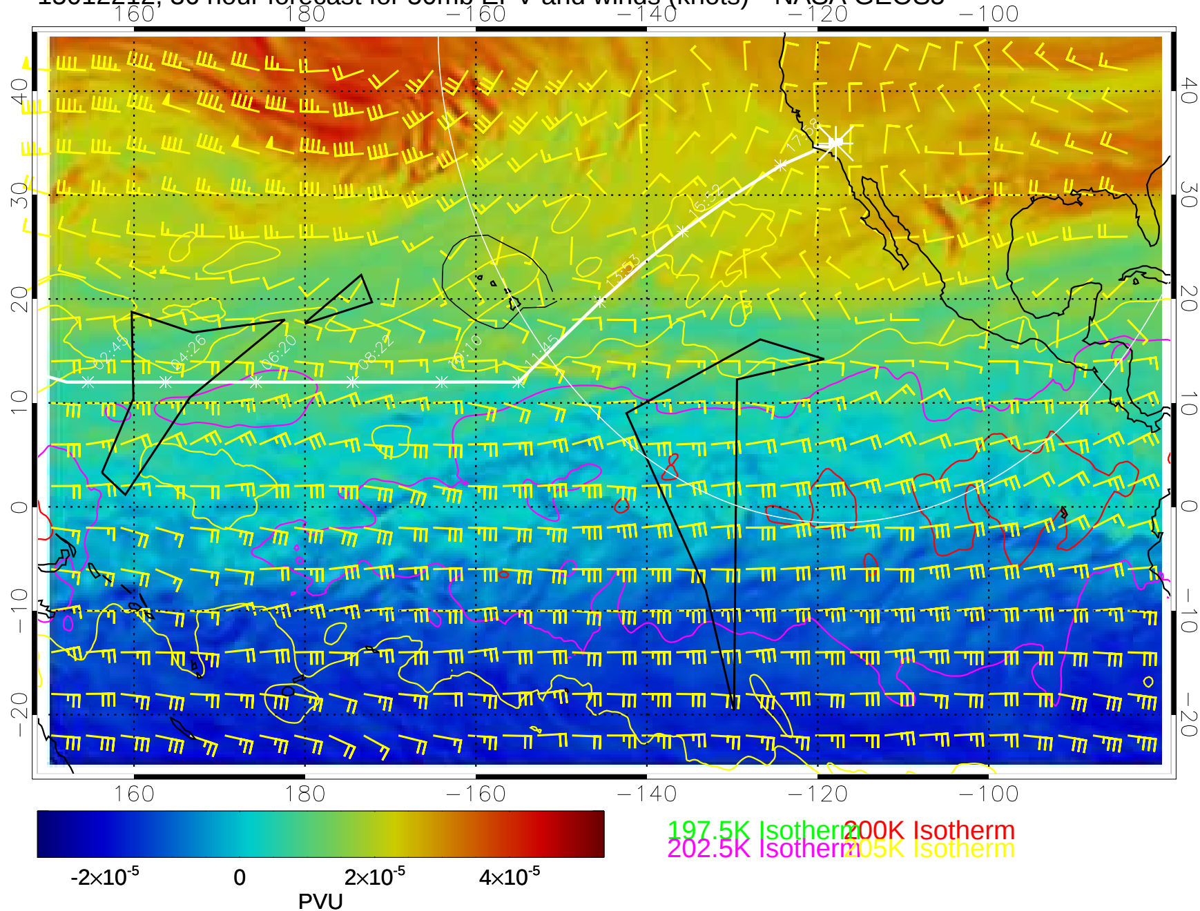
15012212, 36 hour forecast for 50mb EPV and winds (knots)-- NASA GEOS5
