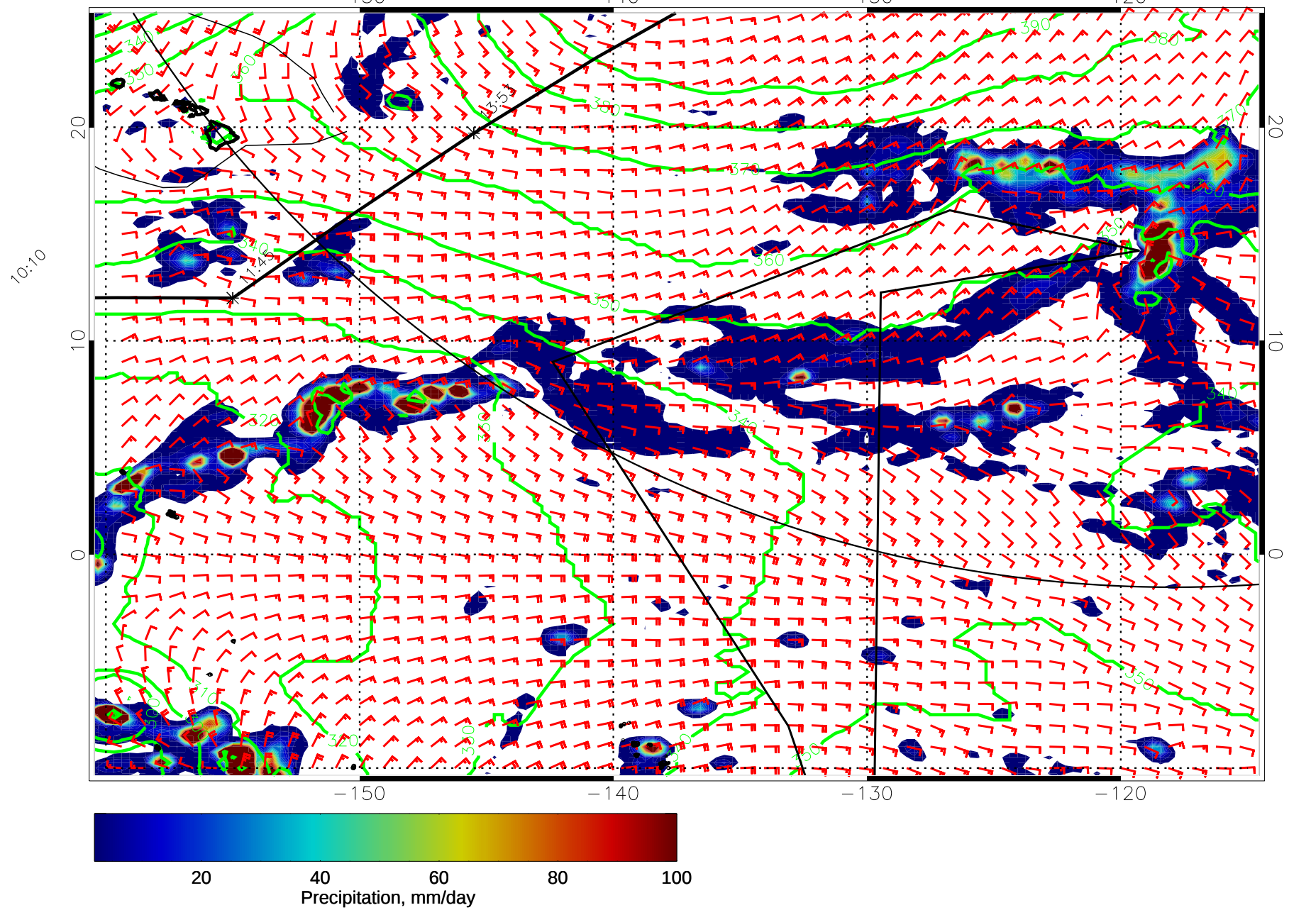
15012218, 66 hour forecast for 975mb Z, Precip., and Surface Winds (knots) -- NASA GEOS5
