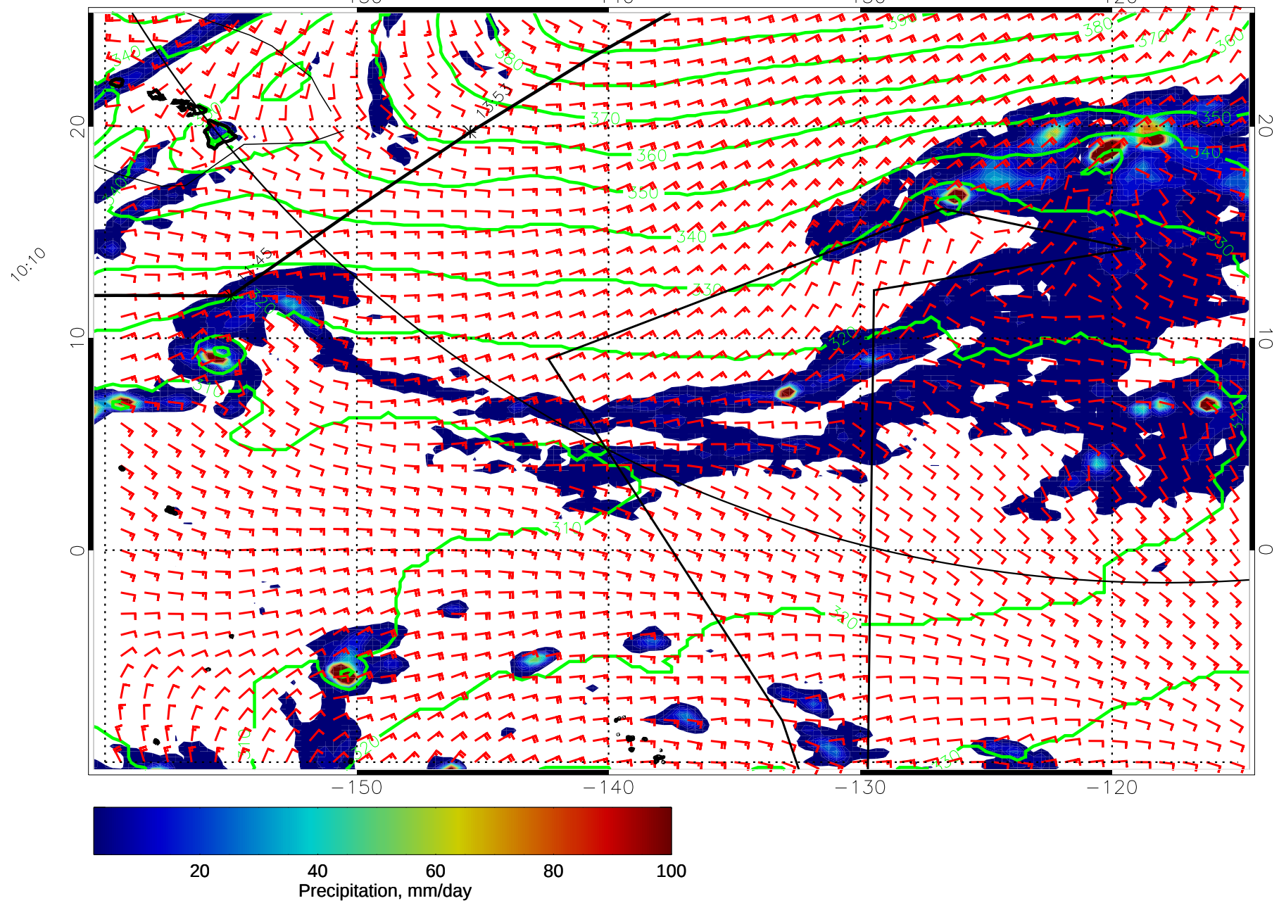
15012400, 96 hour forecast for 975mb Z, Precip., and Surface Winds (knots) -- NASA GEOS5
