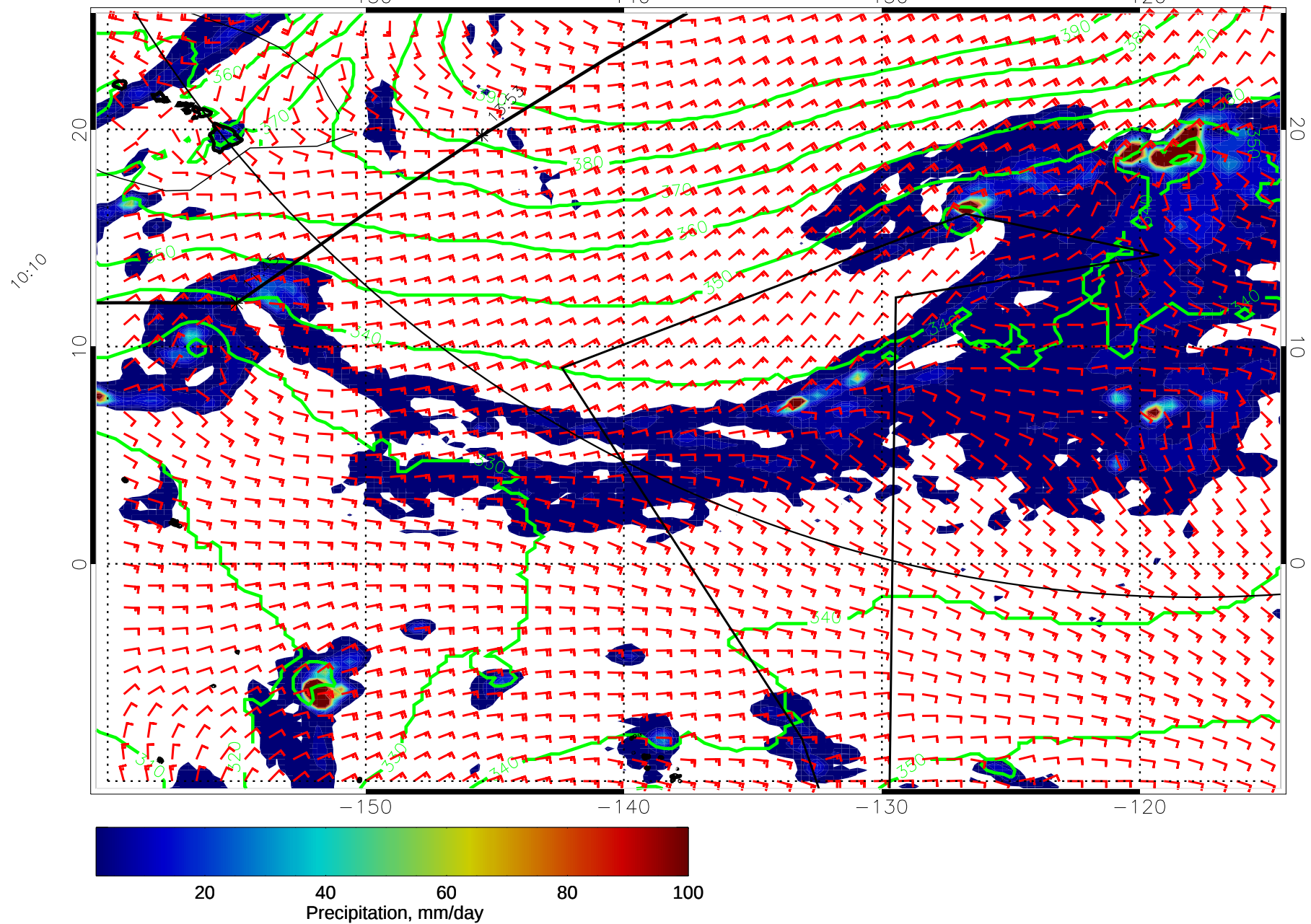
15012406, 102 hour forecast for 975mb Z, Precip., and Surface Winds (knots) -- NASA GEOS5
