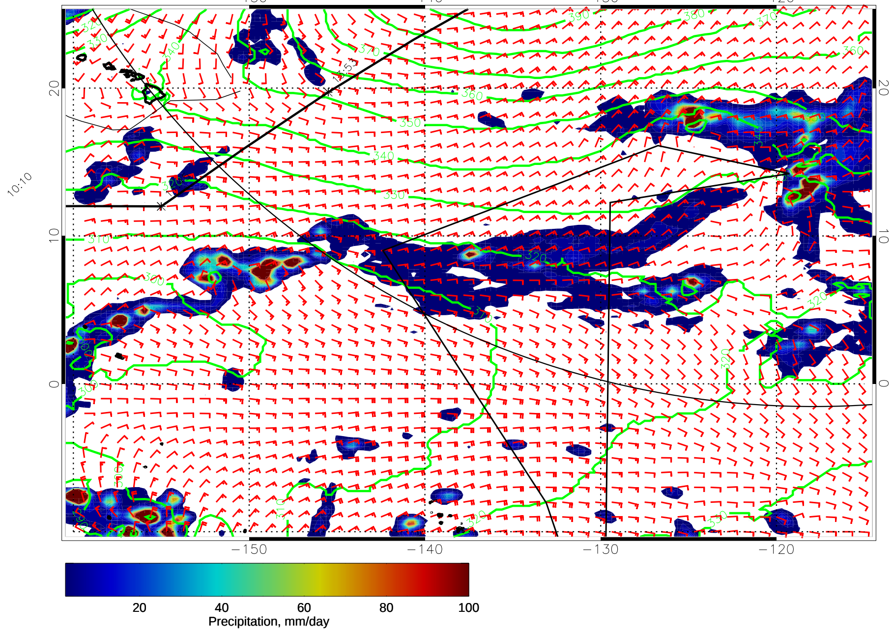
15012300, 72 hour forecast for 975mb Z, Precip., and Surface Winds (knots) -- NASA GEOS5
