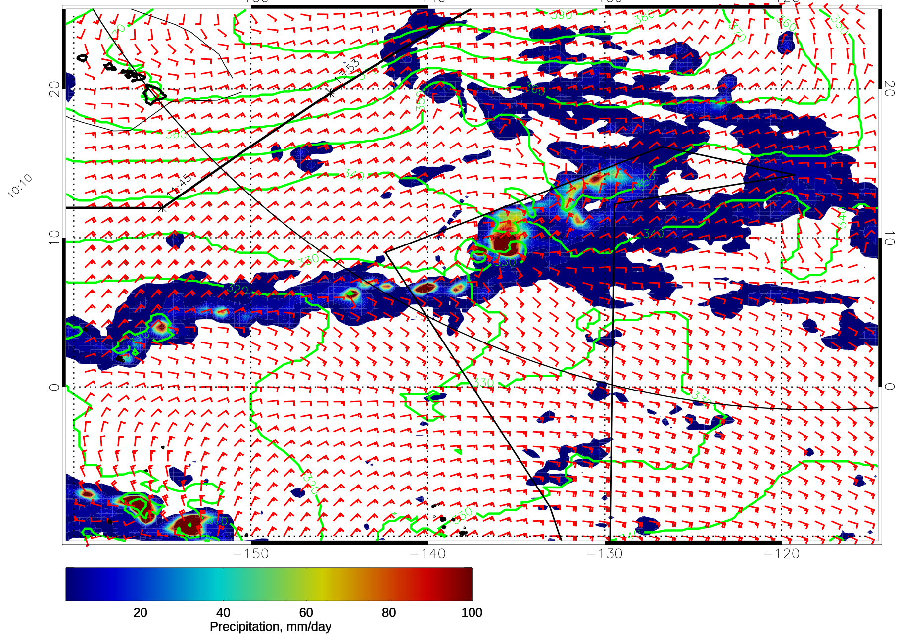
15012106, 30 hour forecast for 975mb Z, Precip., and Surface Winds (knots) -- NASA GEOS5
