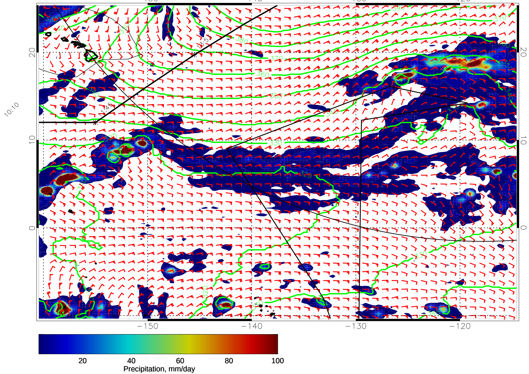
15012312, 84 hour forecast for 975mb Z, Precip., and Surface Winds (knots) -- NASA GEOS5
