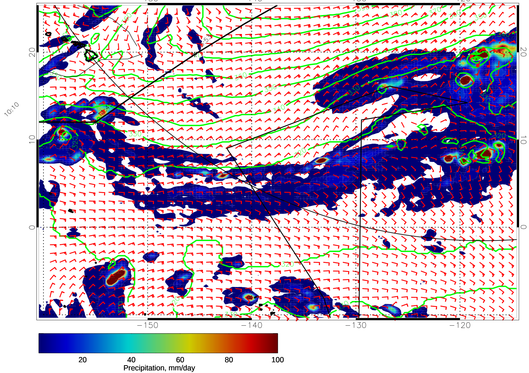
15012412, 108 hour forecast for 975mb Z, Precip., and Surface Winds (knots) -- NASA GEOS5
