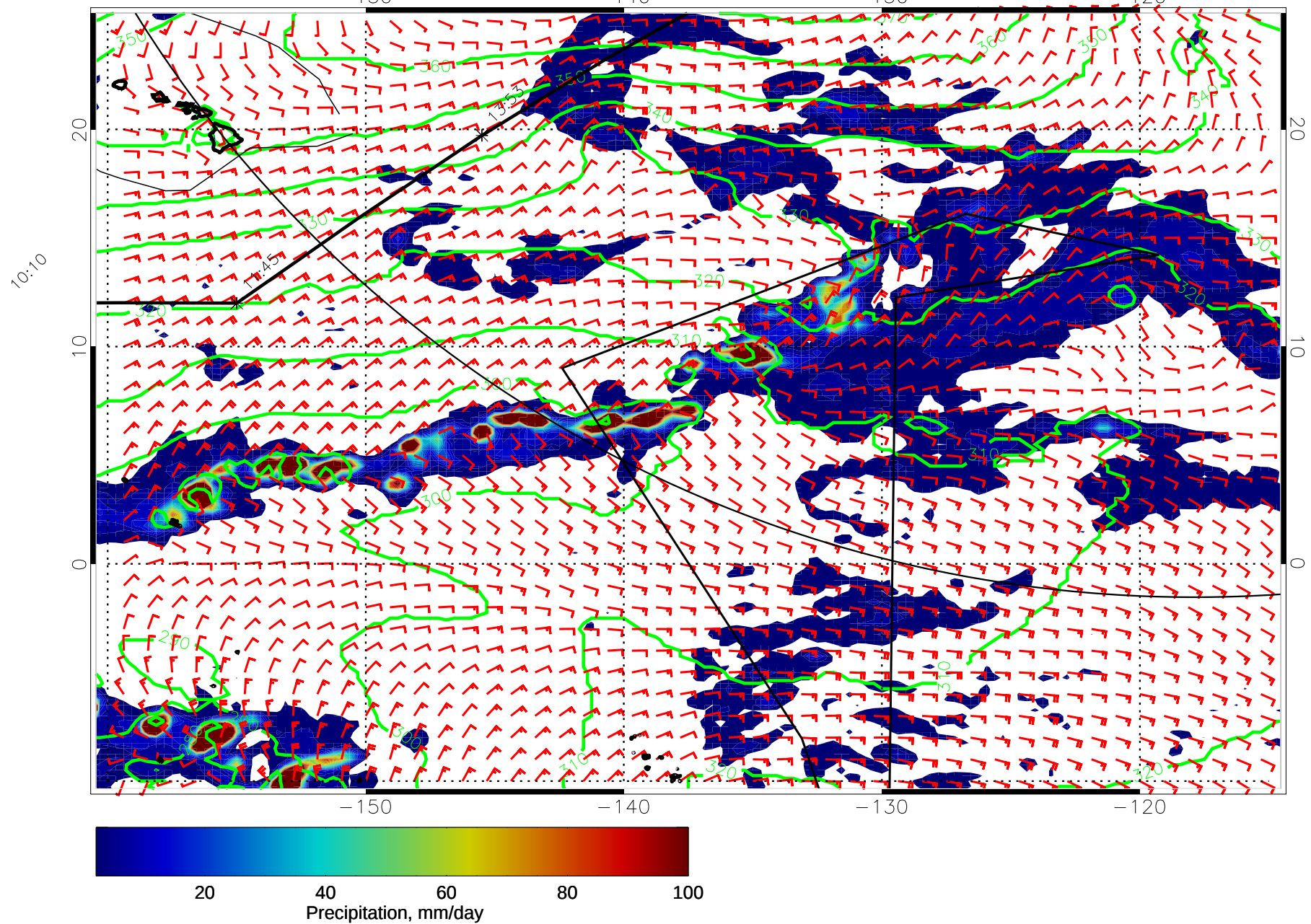
15012112, 36 hour forecast for 975mb Z, Precip., and Surface Winds (knots) -- NASA GEOS5
