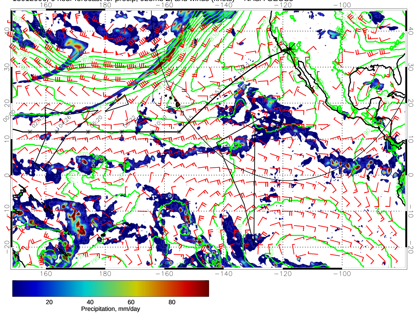
15012006, 6 hour forecast for precip, 925mb Z, and winds (knots) -- NASA GEOS5
