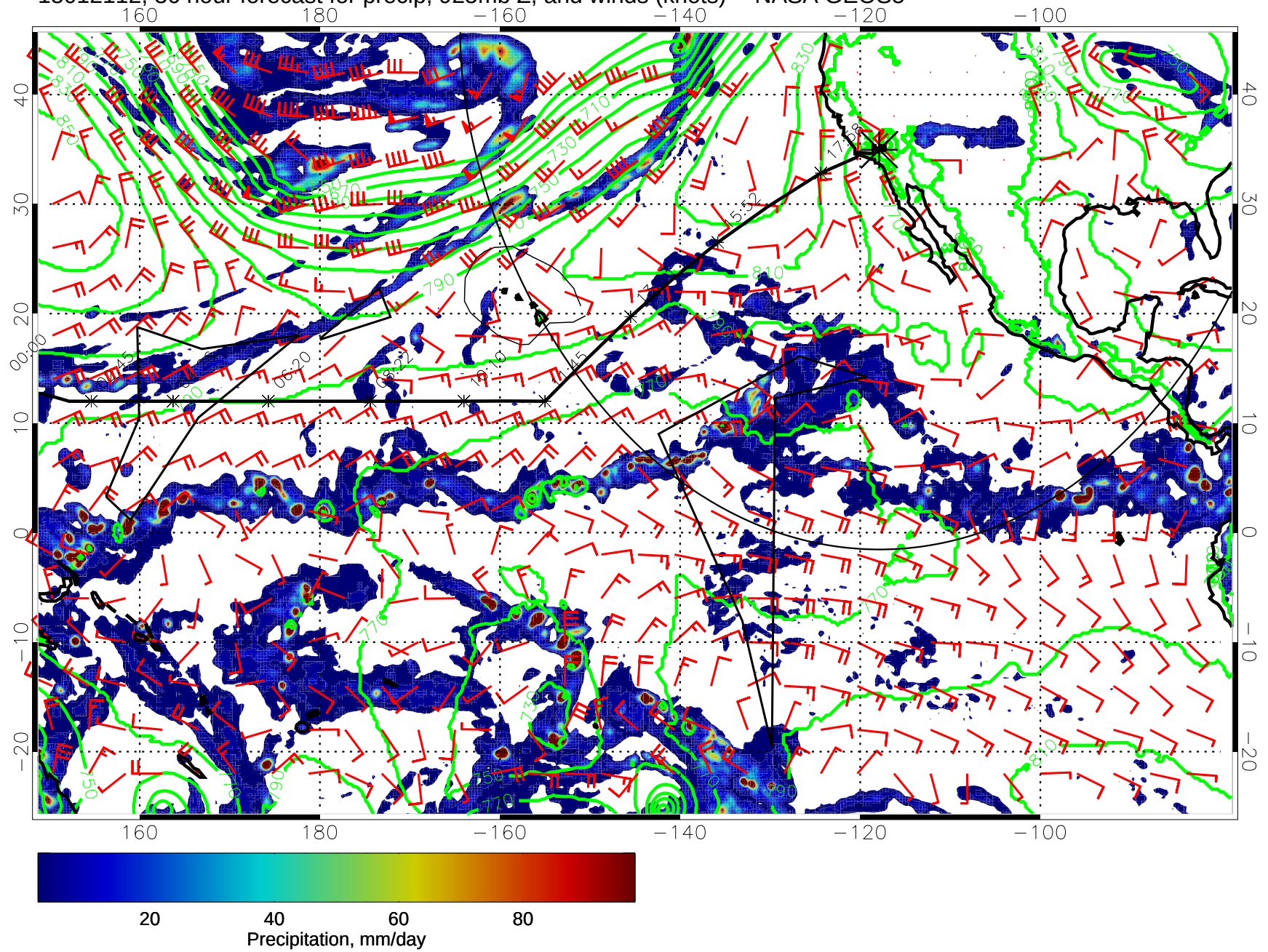
15012112, 36 hour forecast for precip, 925mb Z, and winds (knots) -- NASA GEOS5
