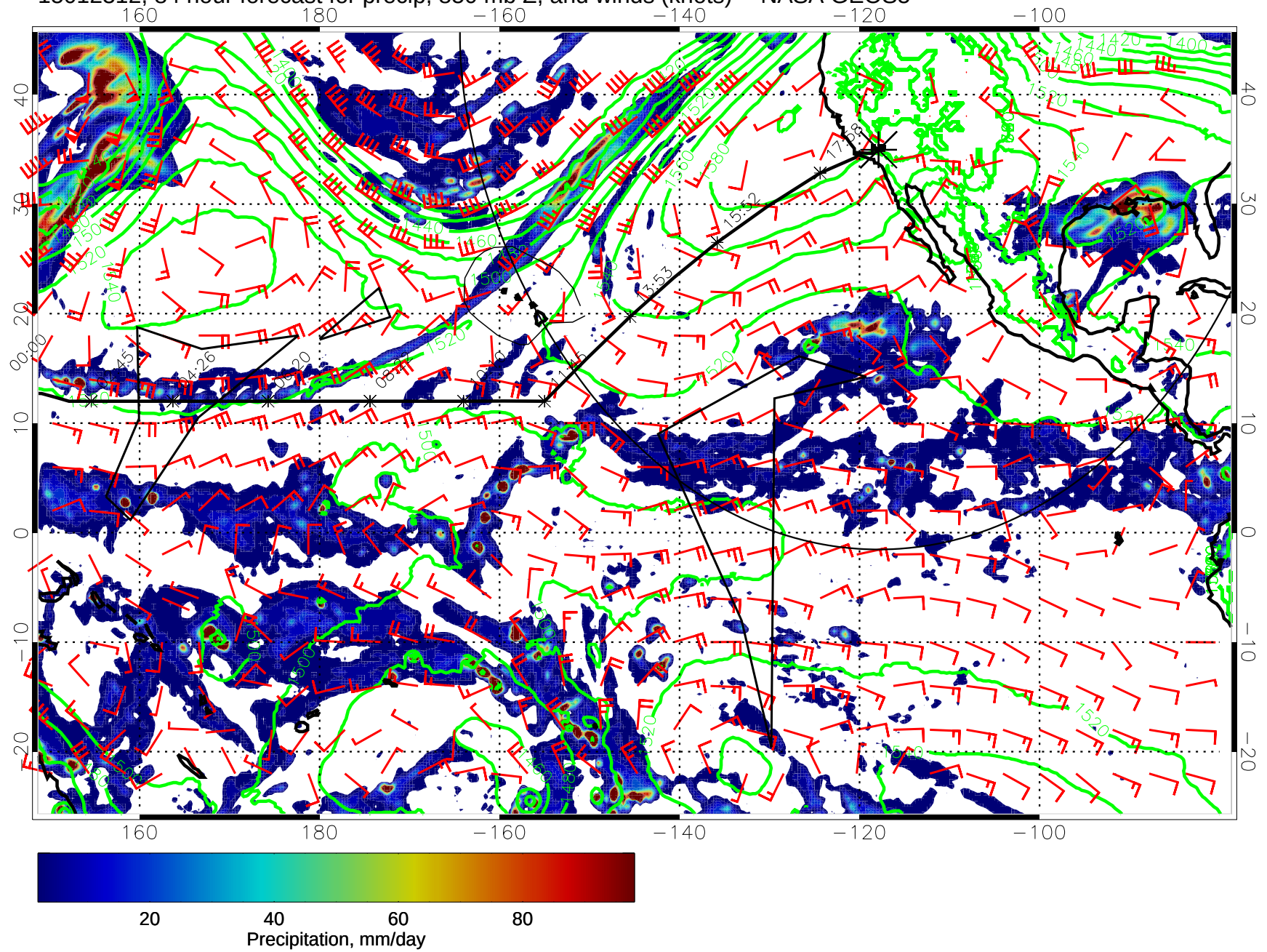
15012312, 84 hour forecast for precip, 850 mb Z, and winds (knots) -- NASA GEOS5
