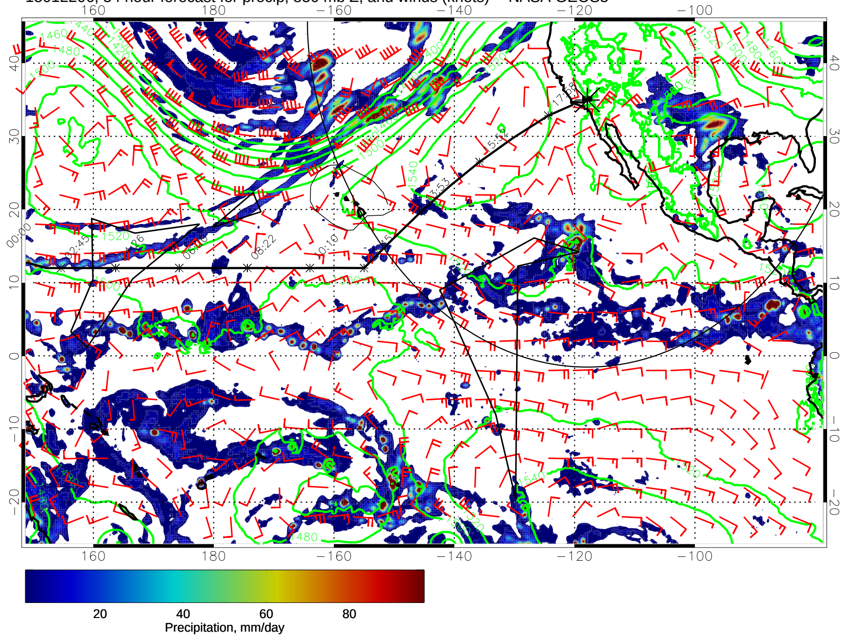
15012206, 54 hour forecast for precip, 850 mb Z, and winds (knots) -- NASA GEOS5
