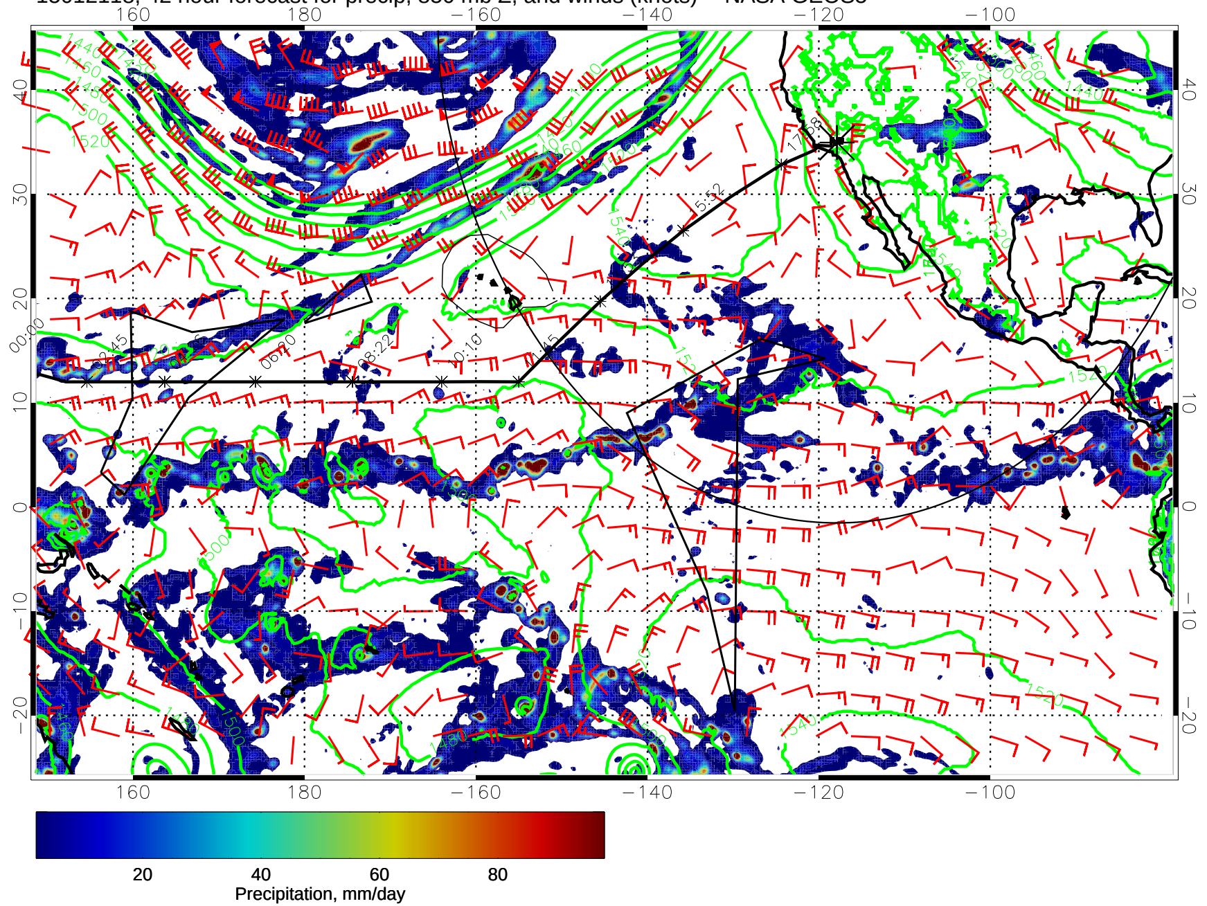
15012118, 42 hour forecast for precip, 850 mb Z, and winds (knots) -- NASA GEOS5
