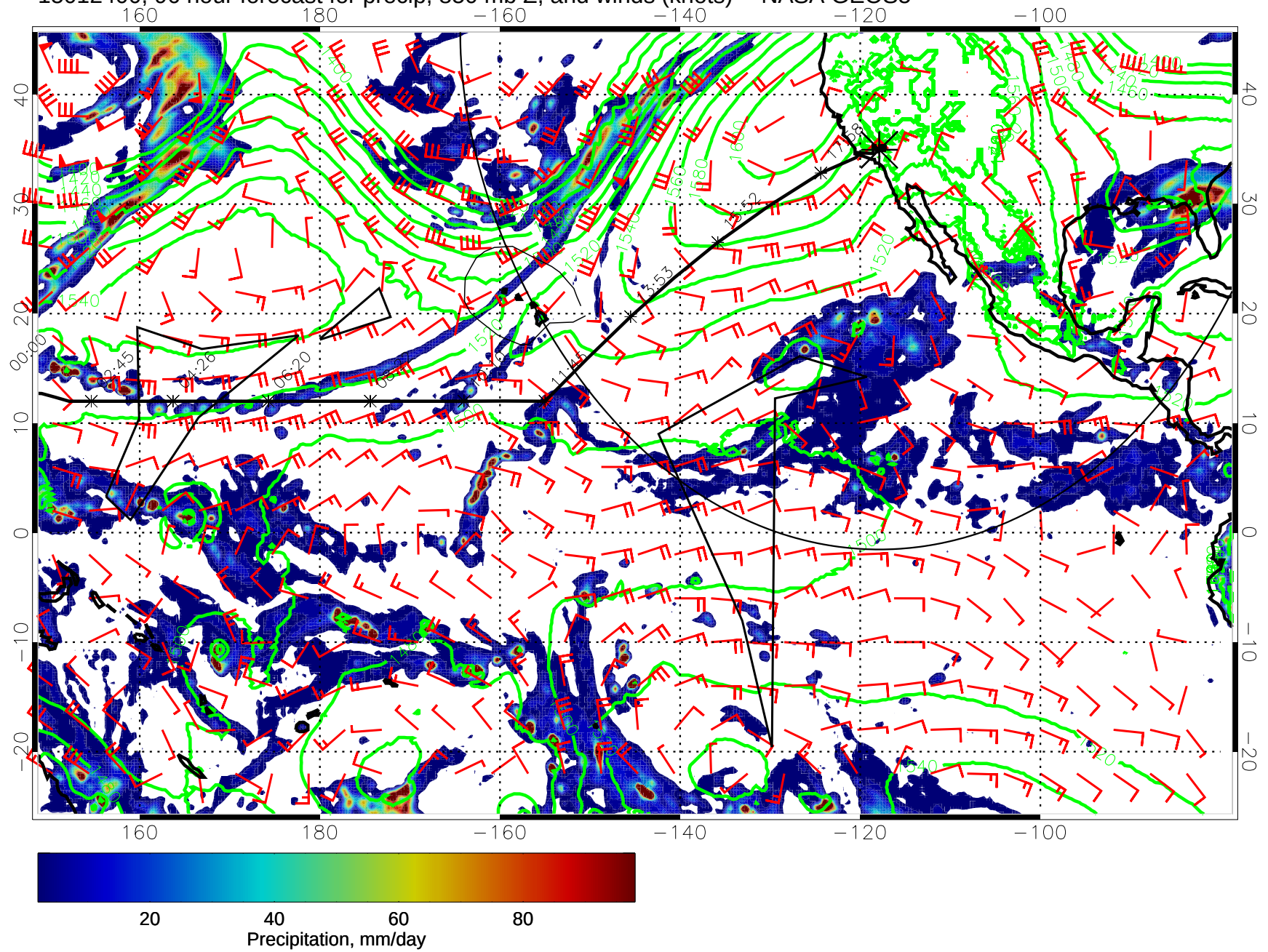
15012400, 96 hour forecast for precip, 850 mb Z, and winds (knots) -- NASA GEOS5
