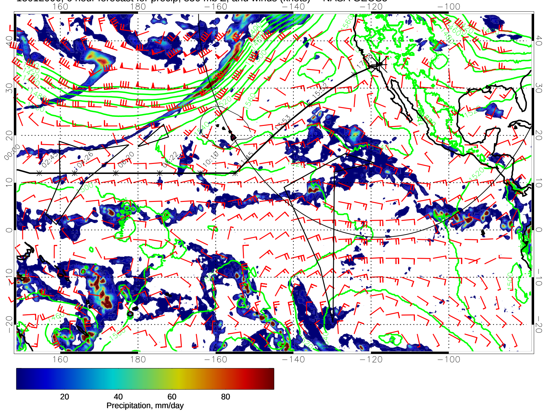
15012006, 6 hour forecast for precip, 850 mb Z, and winds (knots) -- NASA GEOS5
