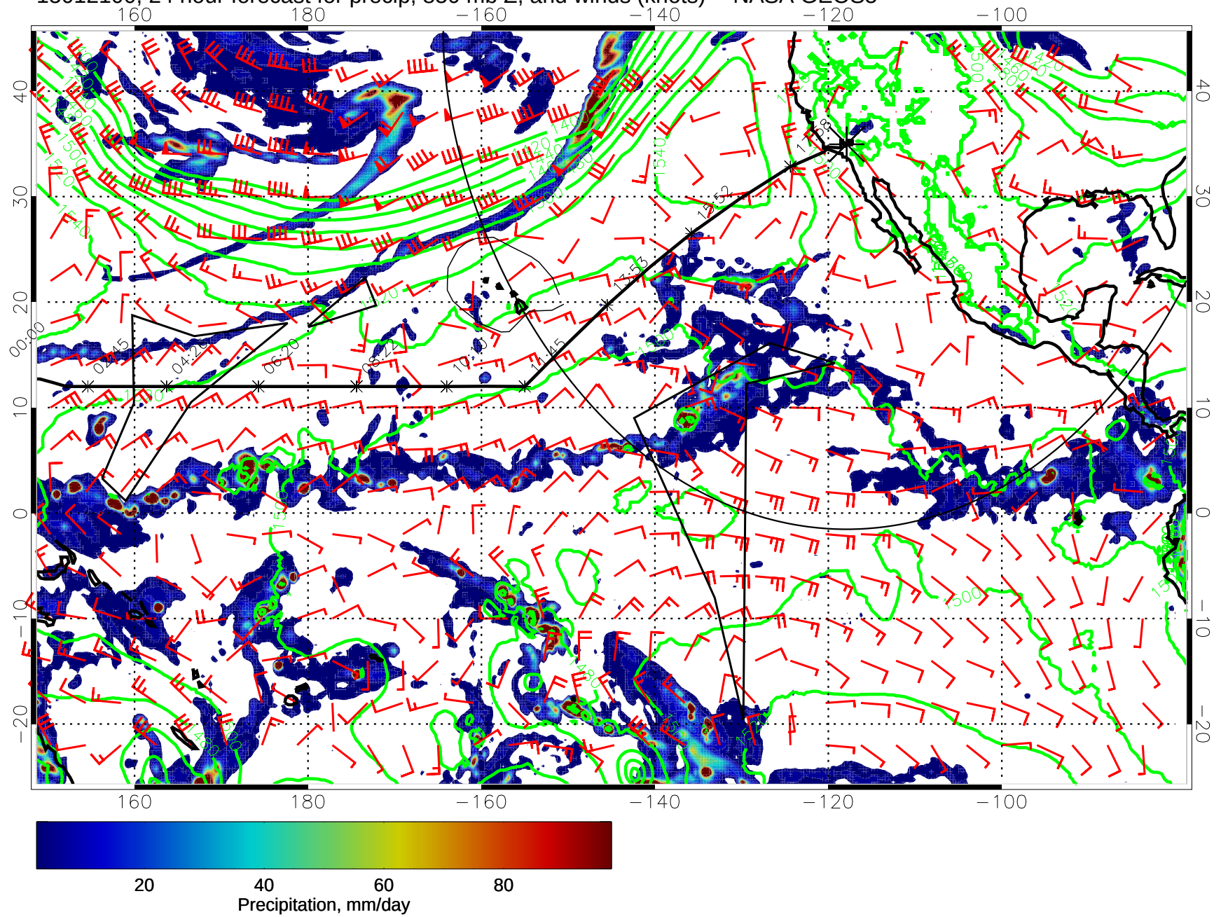
15012100, 24 hour forecast for precip, 850 mb Z, and winds (knots) -- NASA GEOS5
