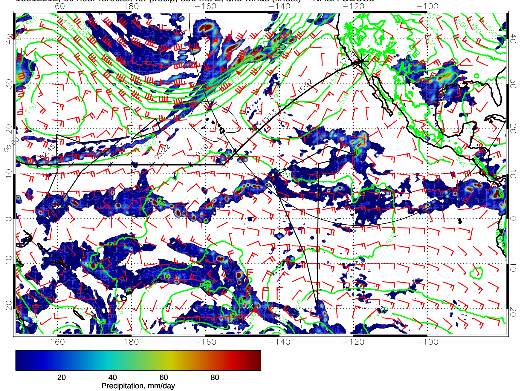
15012212, 60 hour forecast for precip, 850 mb Z, and winds (knots) -- NASA GEOS5
