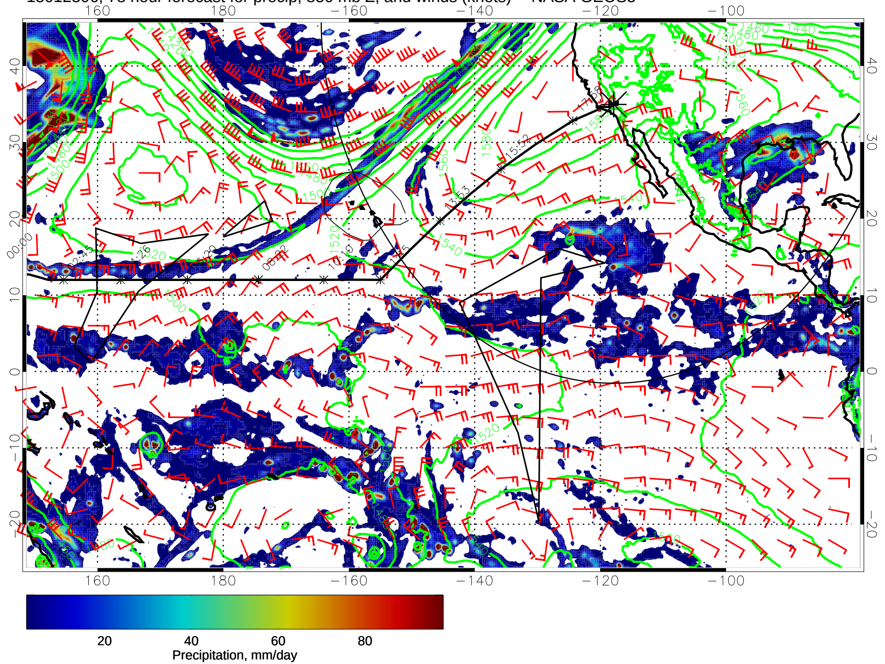
15012306, 78 hour forecast for precip, 850 mb Z, and winds (knots) -- NASA GEOS5
