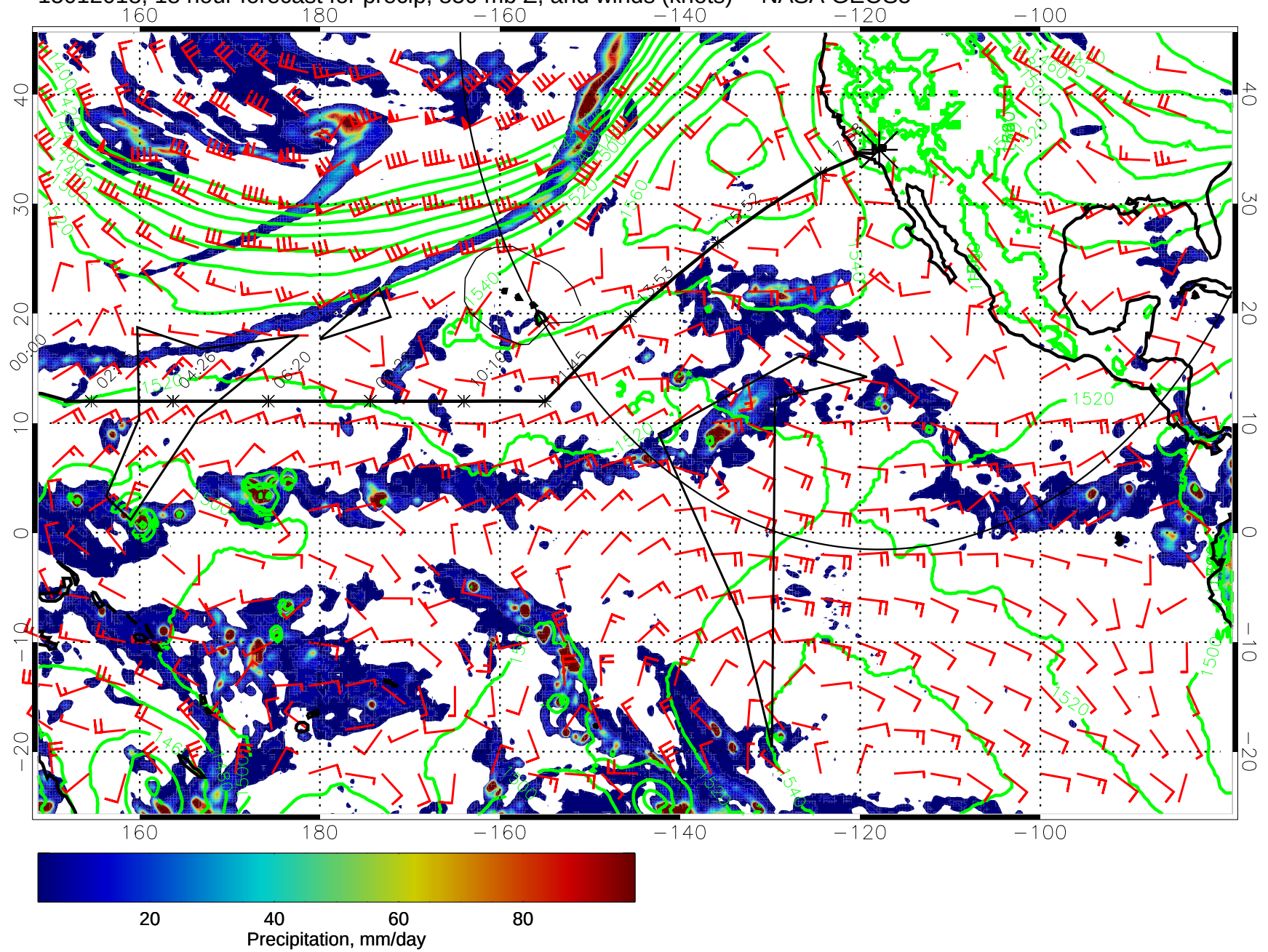
15012018, 18 hour forecast for precip, 850 mb Z, and winds (knots) -- NASA GEOS5
