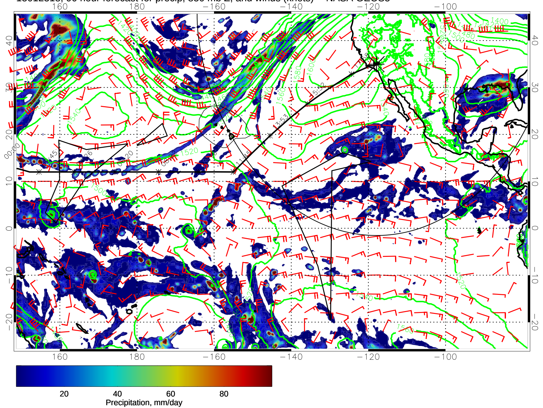
15012318, 90 hour forecast for precip, 850 mb Z, and winds (knots) -- NASA GEOS5
