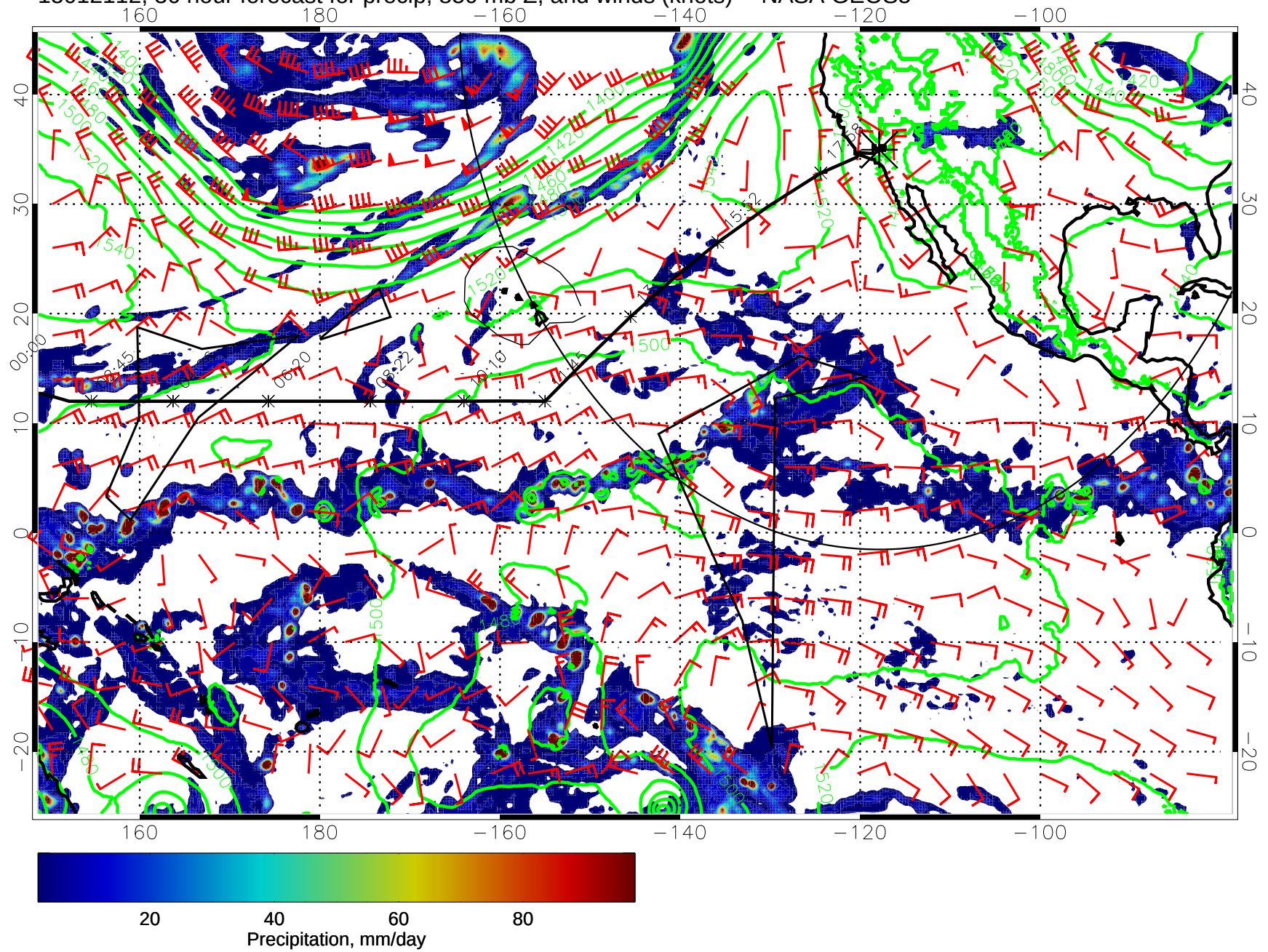
15012112, 36 hour forecast for precip, 850 mb Z, and winds (knots) -- NASA GEOS5
