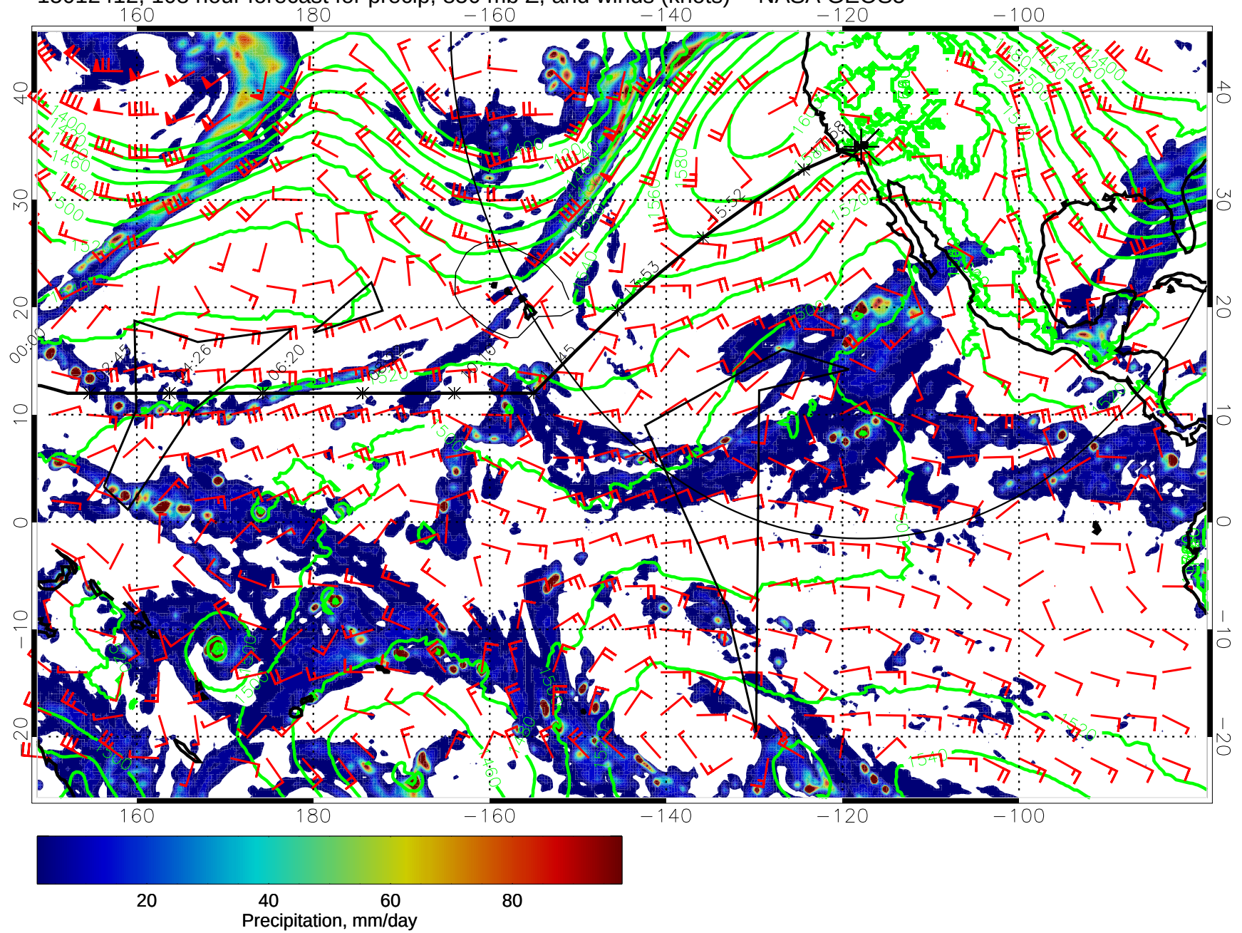
15012412, 108 hour forecast for precip, 850 mb Z, and winds (knots) -- NASA GEOS5
