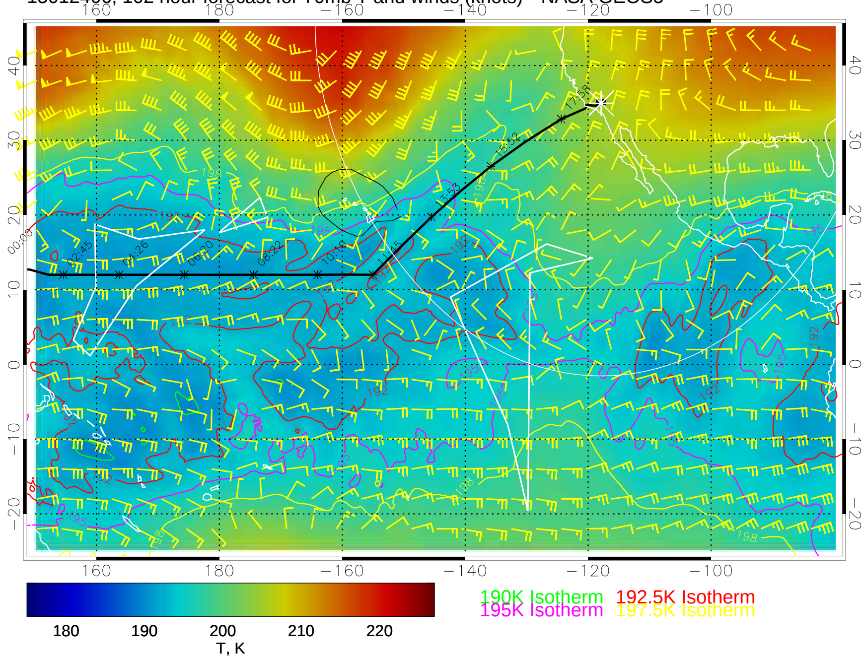
15012406, 102 hour forecast for 70mb T and winds (knots)-- NASA GEOS5
