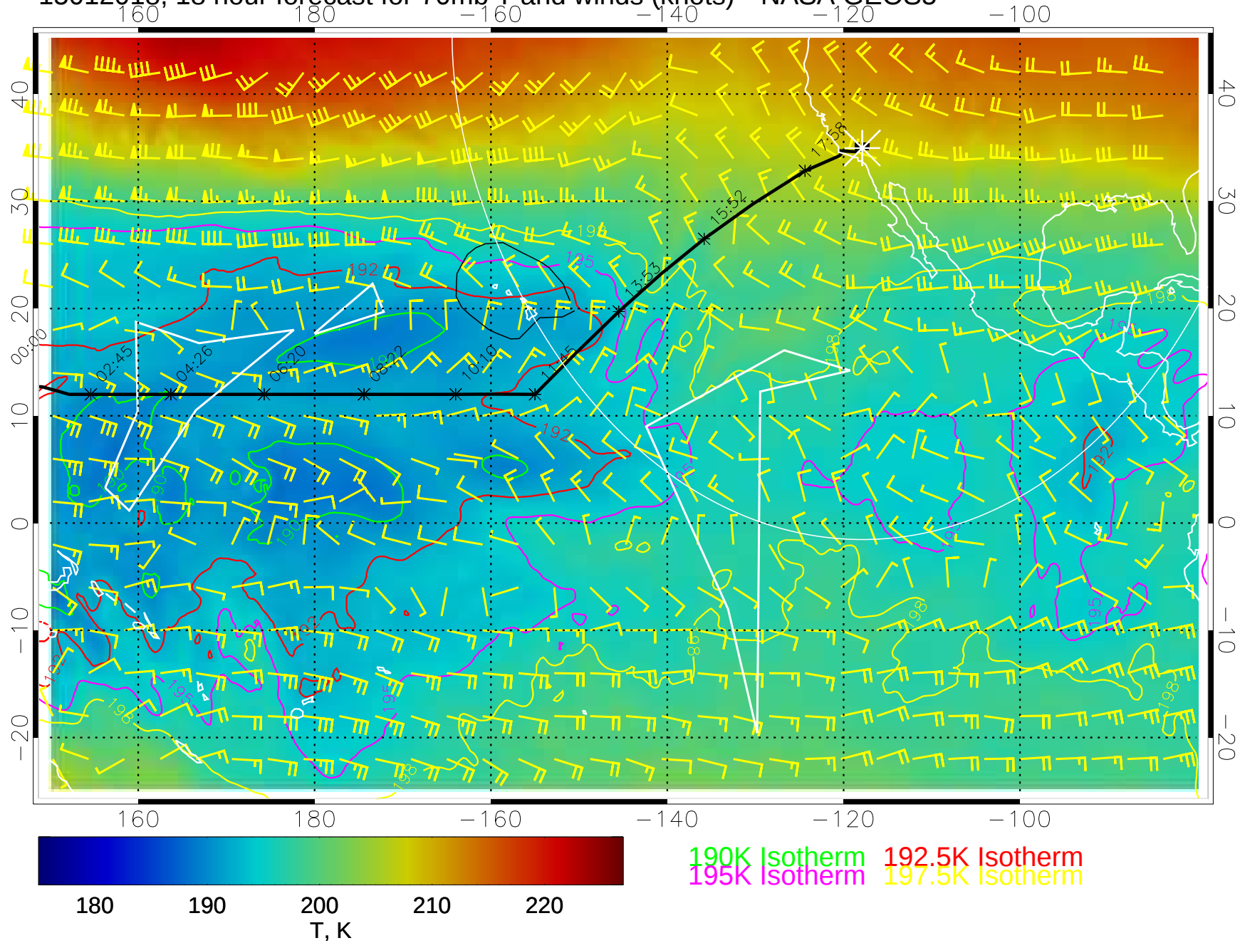
15012018, 18 hour forecast for 70mb T and winds (knots)-- NASA GEOS5
