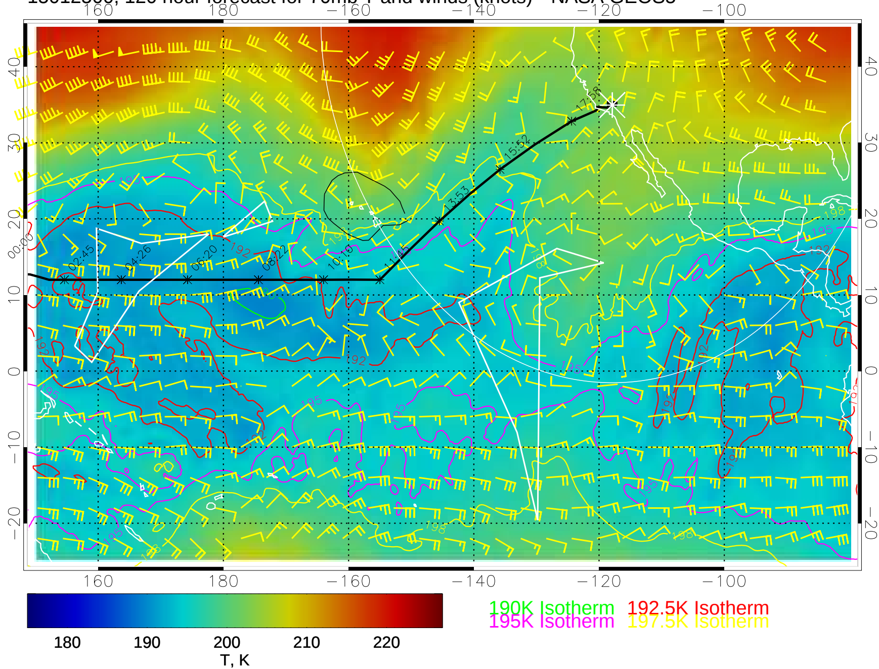
15012500, 120 hour forecast for 70mb T and winds (knots)-- NASA GEOS5
