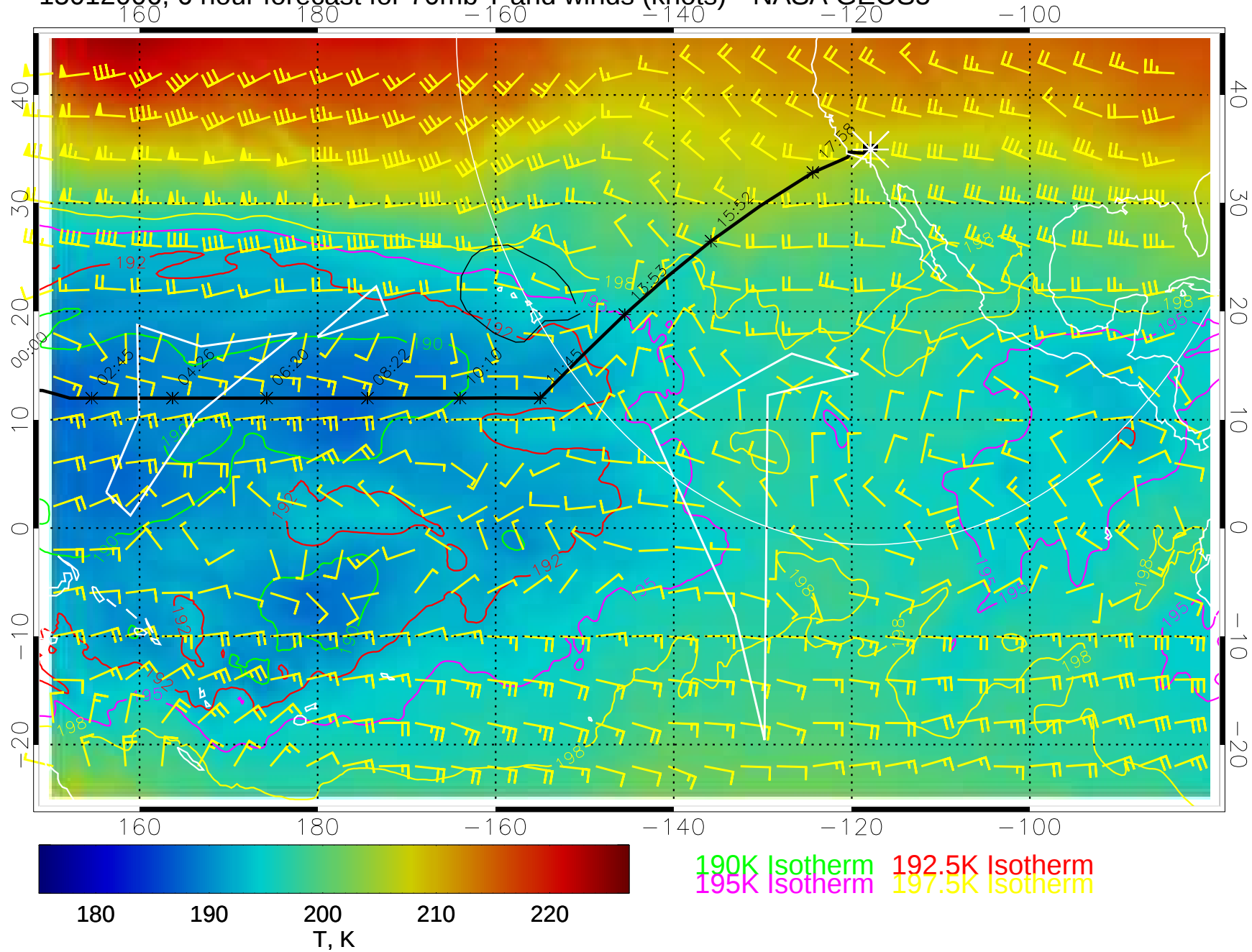
15012006, 6 hour forecast for 70mb T and winds (knots)-- NASA GEOS5
