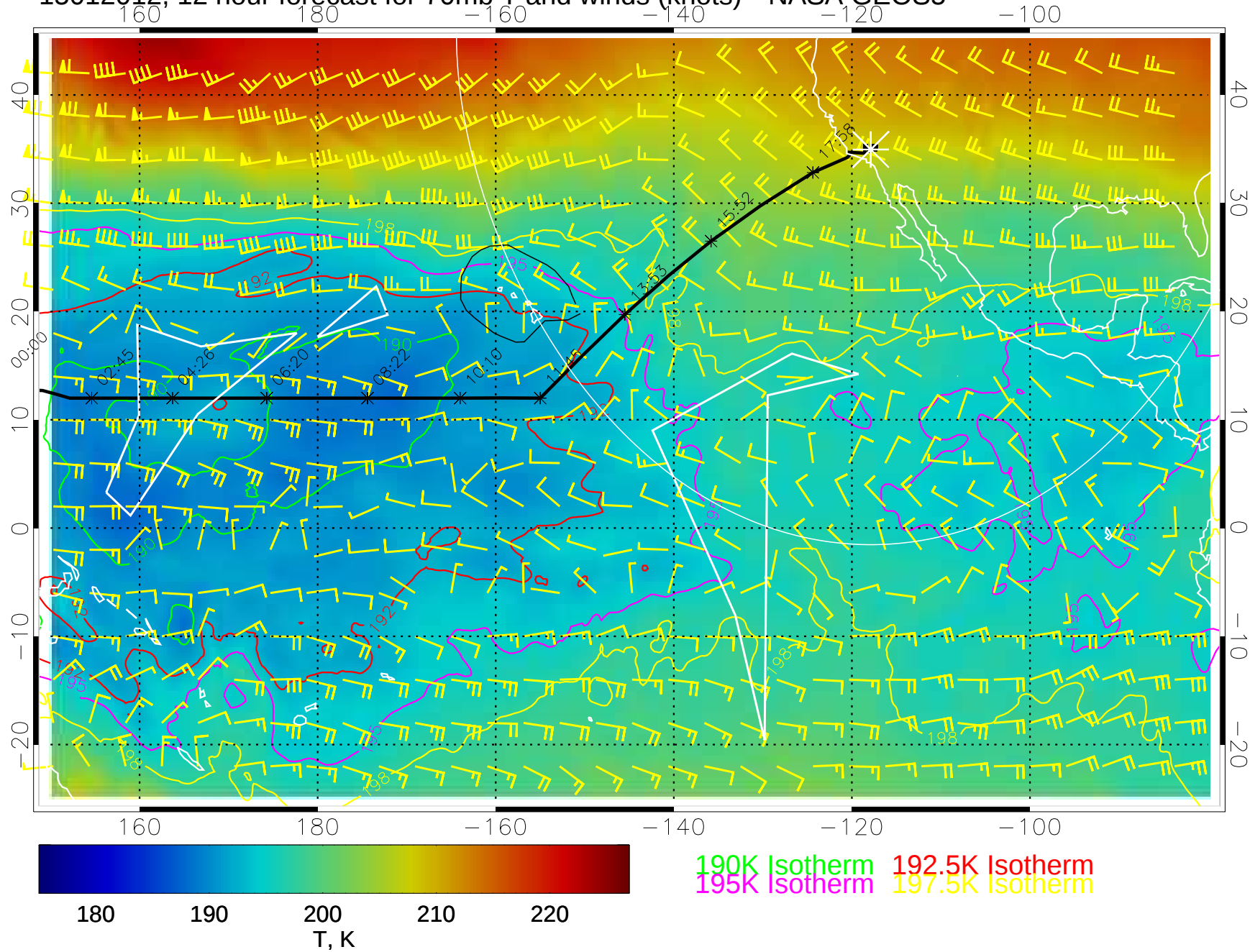
15012012, 12 hour forecast for 70mb T and winds (knots)-- NASA GEOS5
