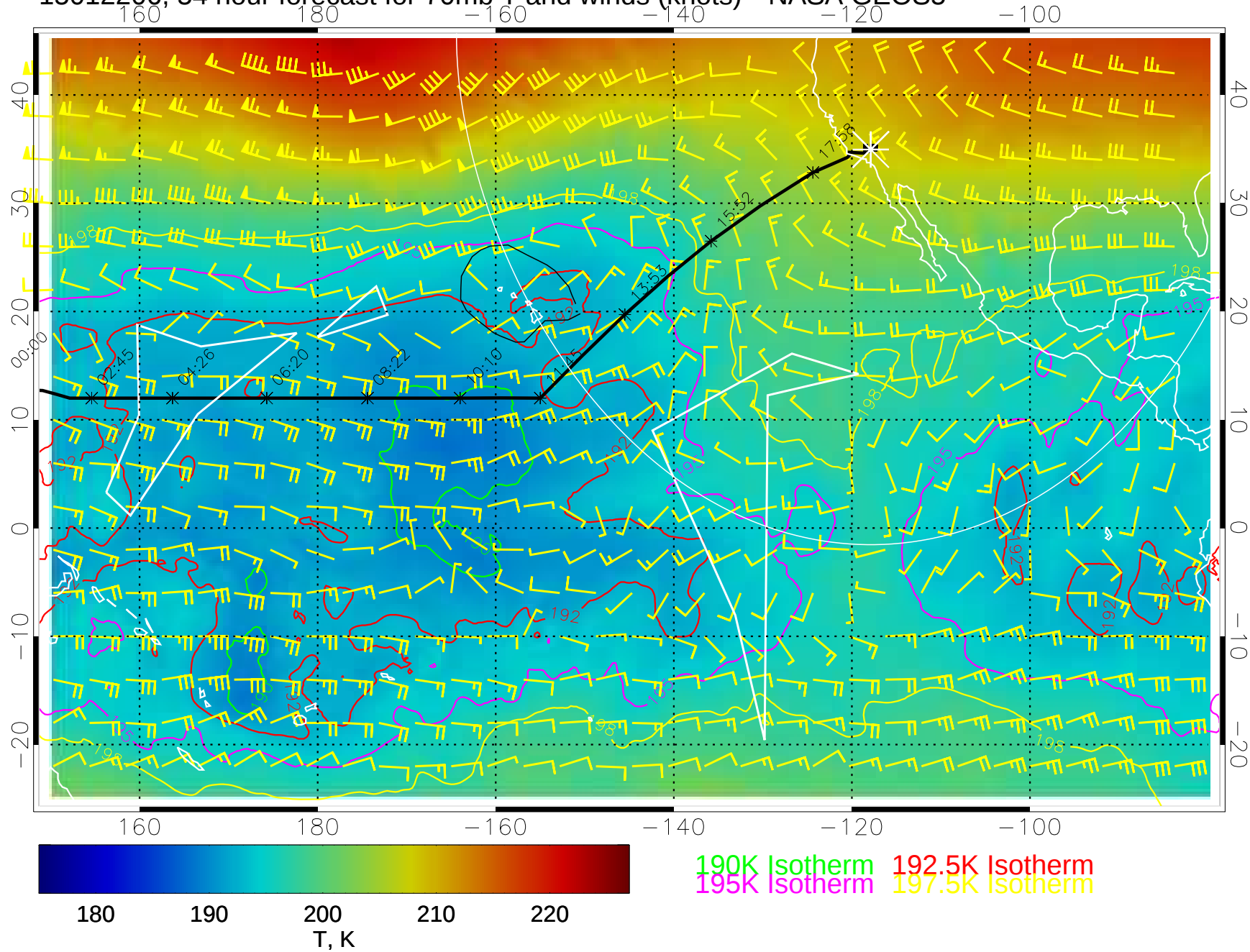
15012206, 54 hour forecast for 70mb T and winds (knots)-- NASA GEOS5
