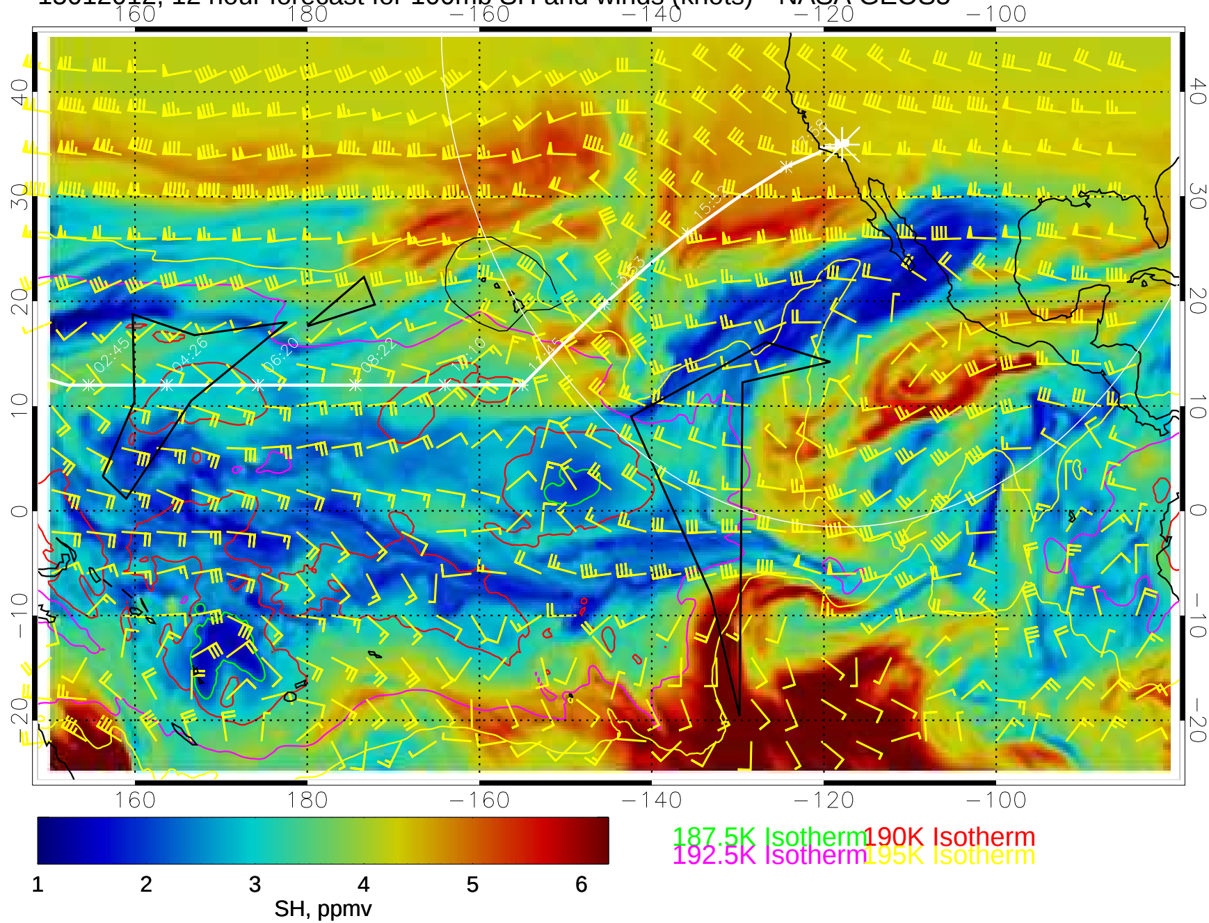
15012012, 12 hour forecast for 100mb SH and winds (knots)-- NASA GEOS5
