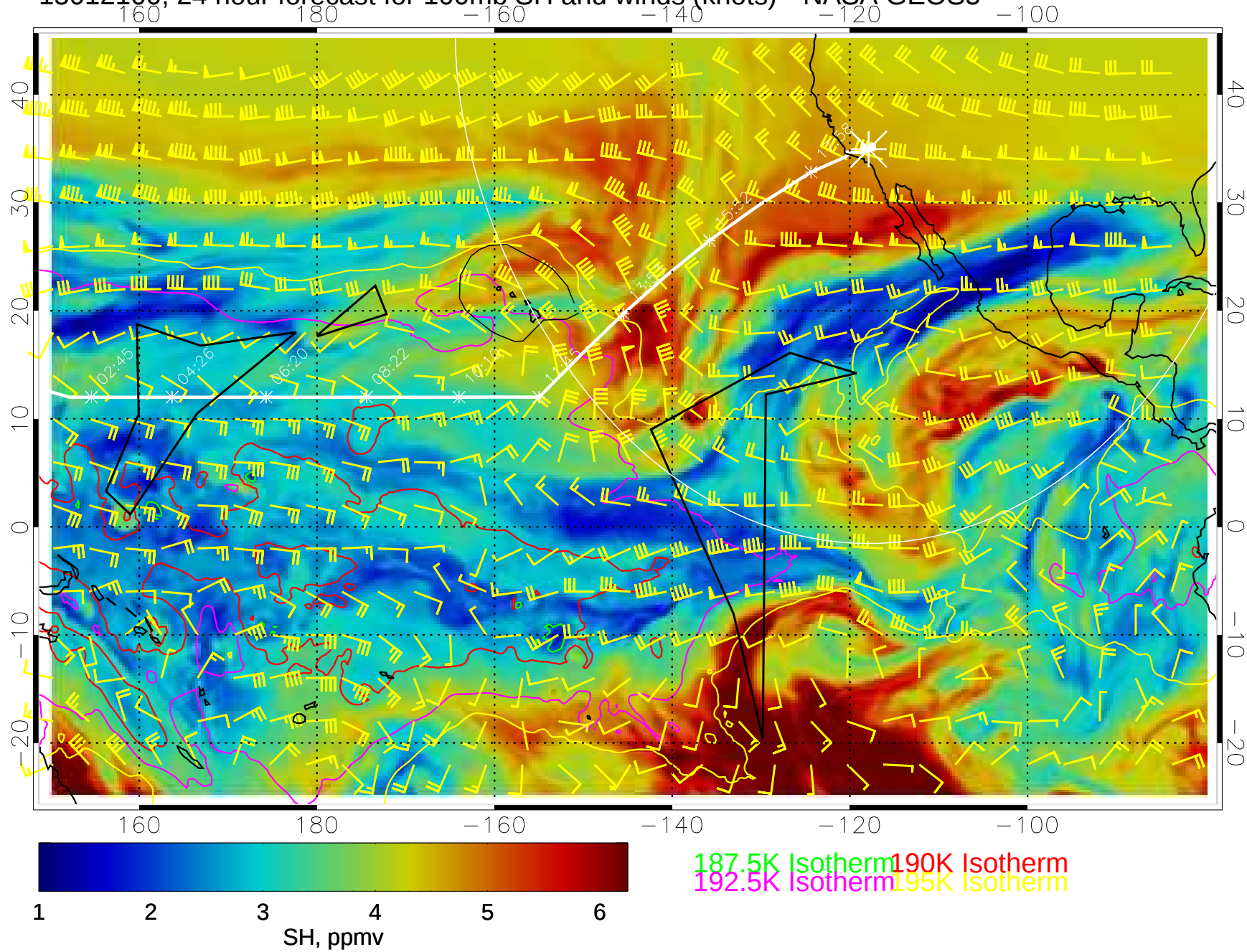
15012100, 24 hour forecast for 100mb SH and winds (knots)-- NASA GEOS5
