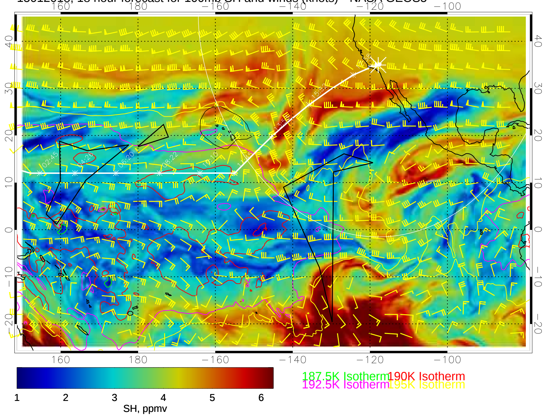
15012018, 18 hour forecast for 100mb SH and winds (knots)-- NASA GEOS5
