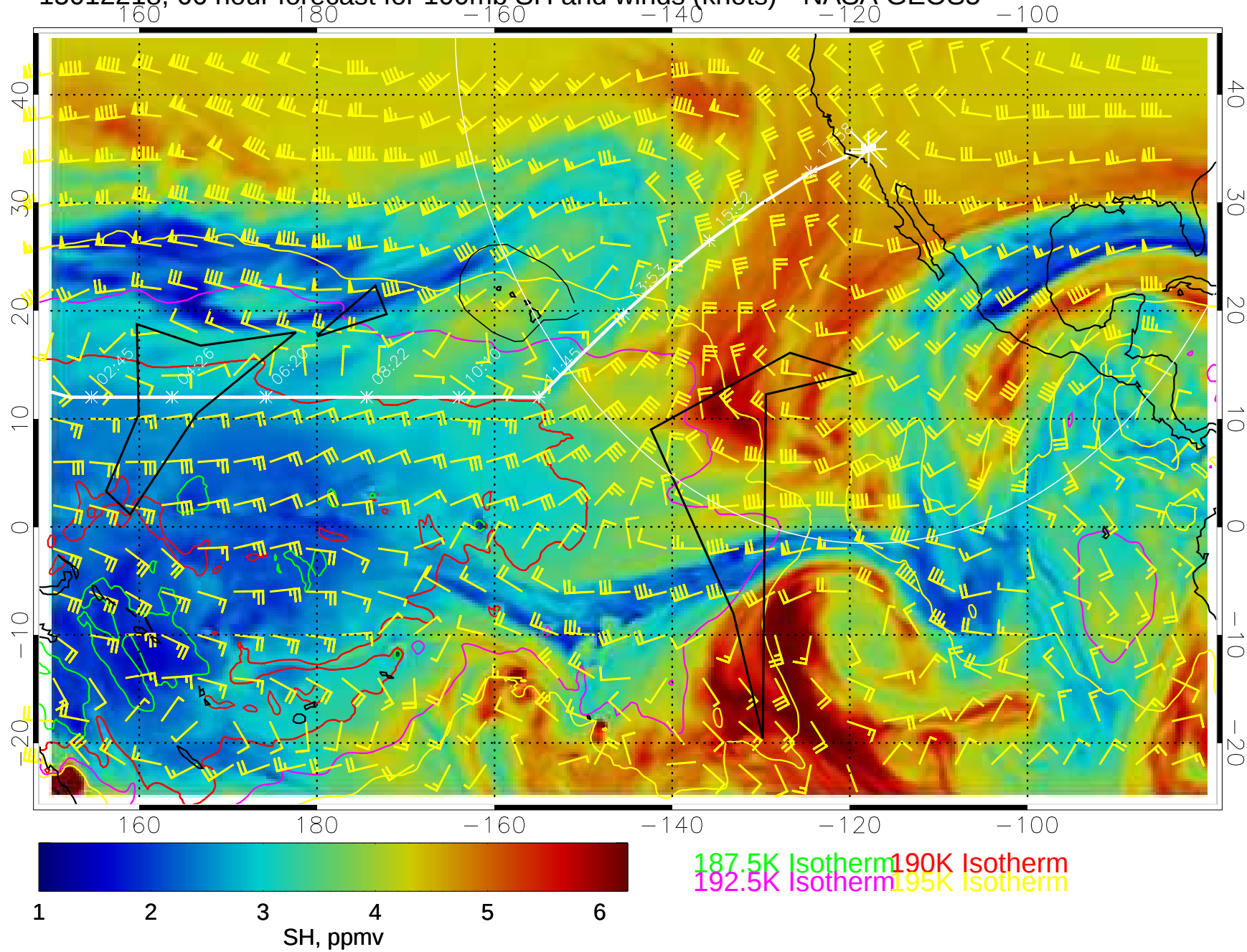
15012218, 66 hour forecast for 100mb SH and winds (knots)-- NASA GEOS5
