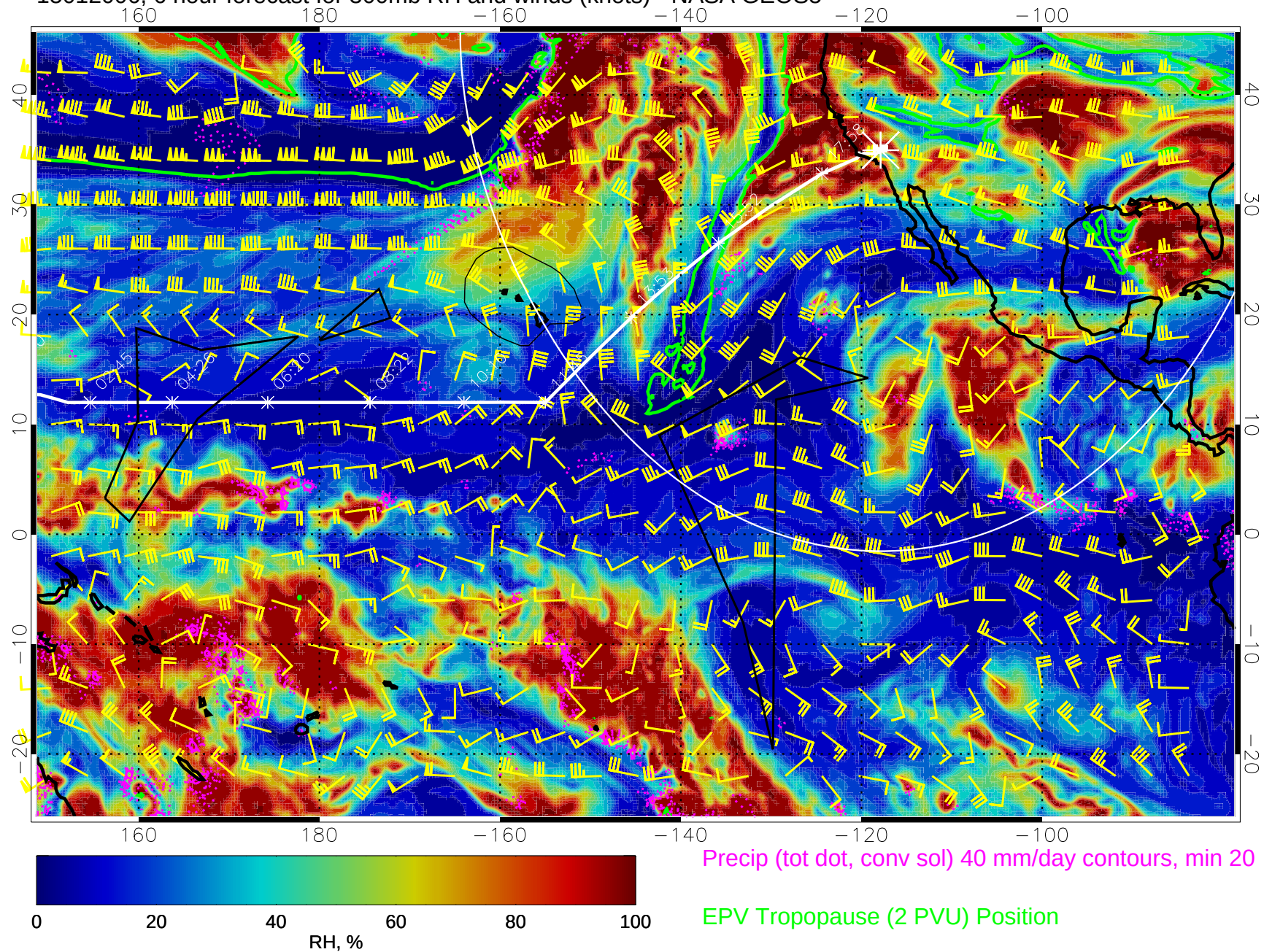
15012006, 6 hour forecast for 300mb RH and winds (knots) - NASA GEOS5
