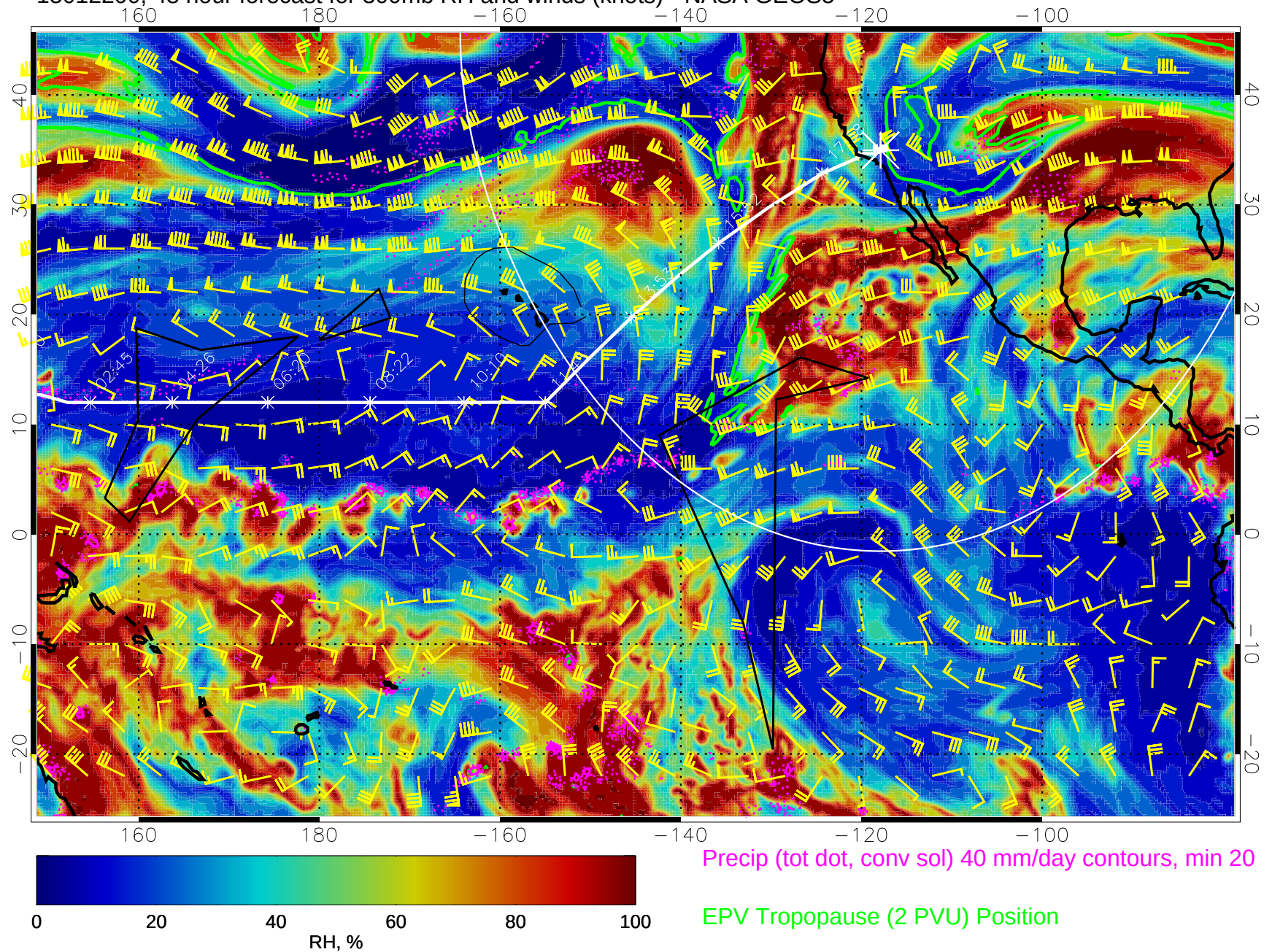
15012200, 48 hour forecast for 300mb RH and winds (knots) - NASA GEOS5
