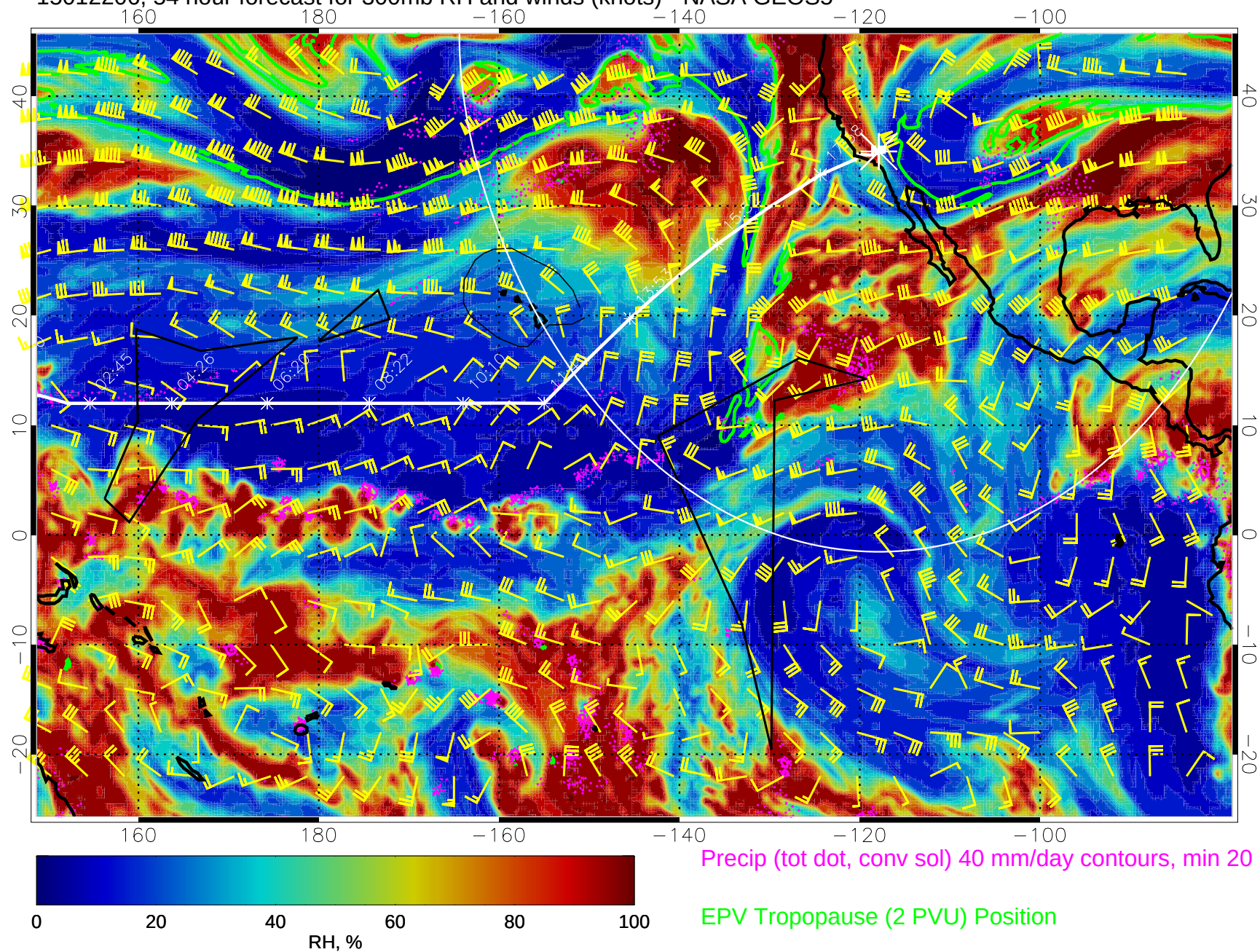
15012206, 54 hour forecast for 300mb RH and winds (knots) - NASA GEOS5
