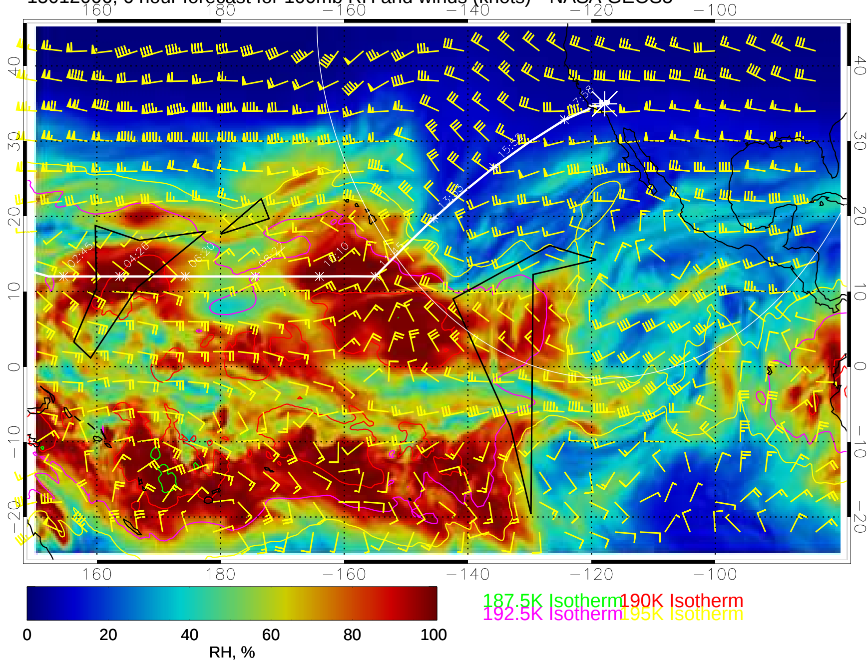
15012006, 6 hour forecast for 100mb RH and winds (knots)-- NASA GEOS5
