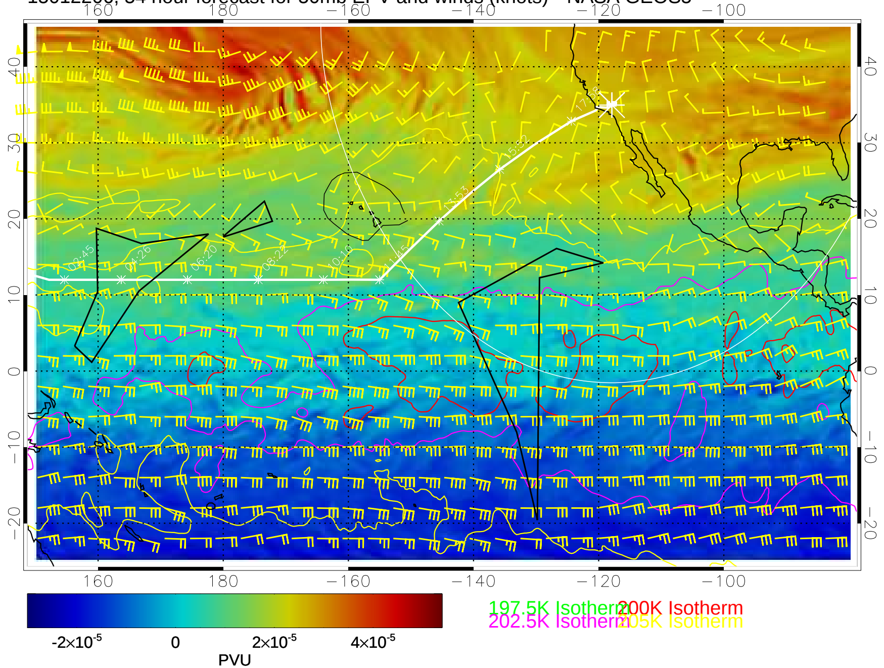
15012206, 54 hour forecast for 50mb EPV and winds (knots)-- NASA GEOS5
