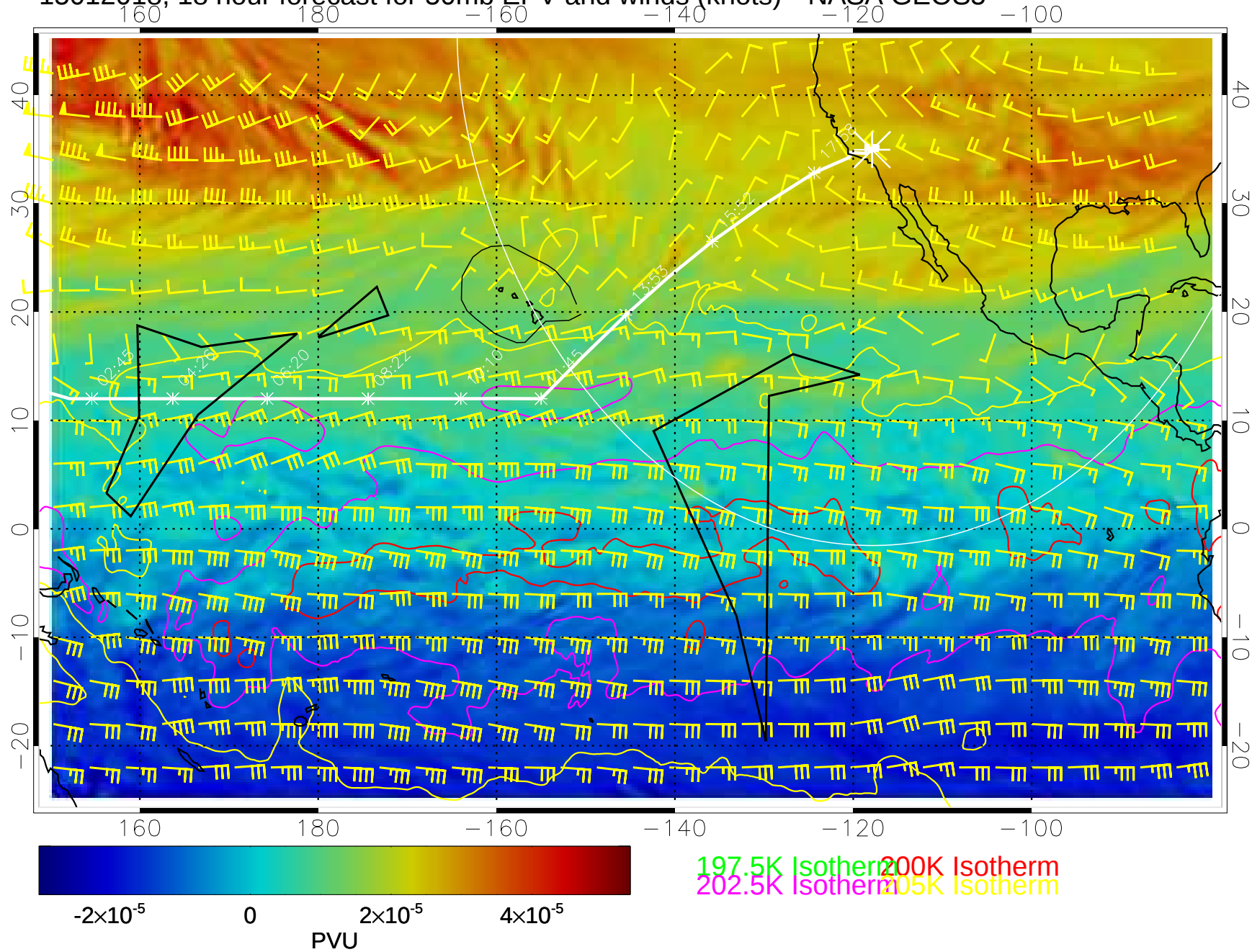
15012018, 18 hour forecast for 50mb EPV and winds (knots)-- NASA GEOS5
