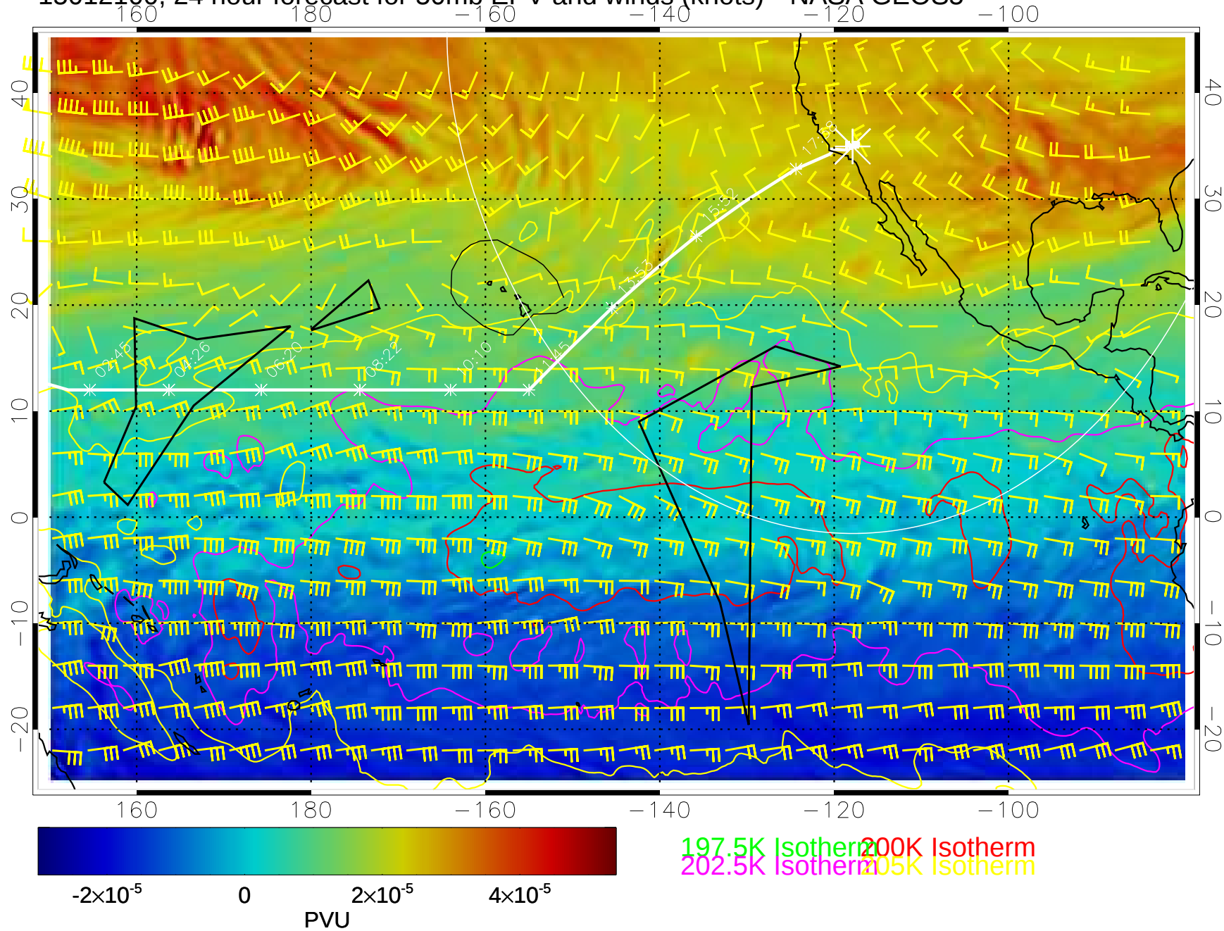
15012100, 24 hour forecast for 50mb EPV and winds (knots)-- NASA GEOS5
