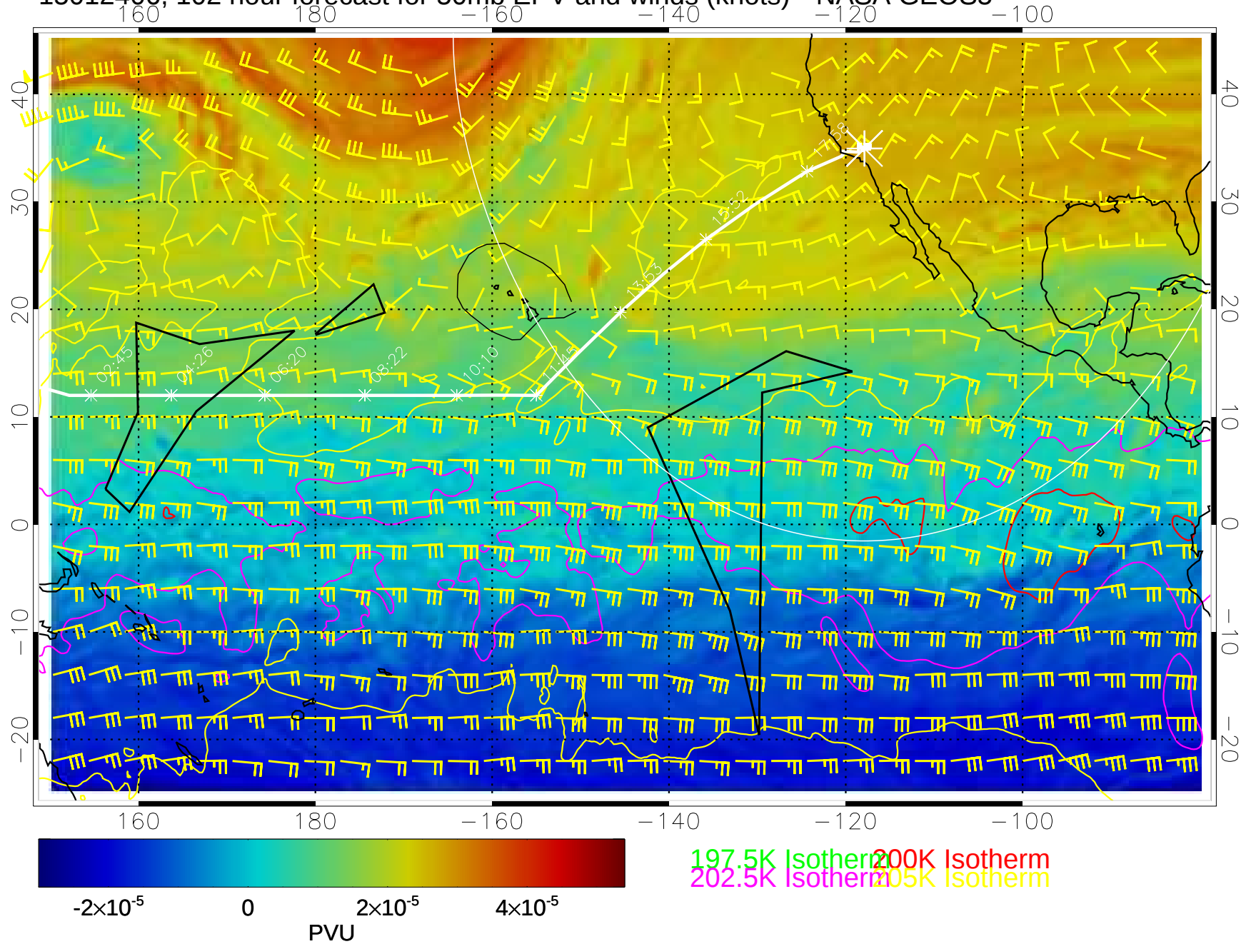
15012406, 102 hour forecast for 50mb EPV and winds (knots)-- NASA GEOS5
