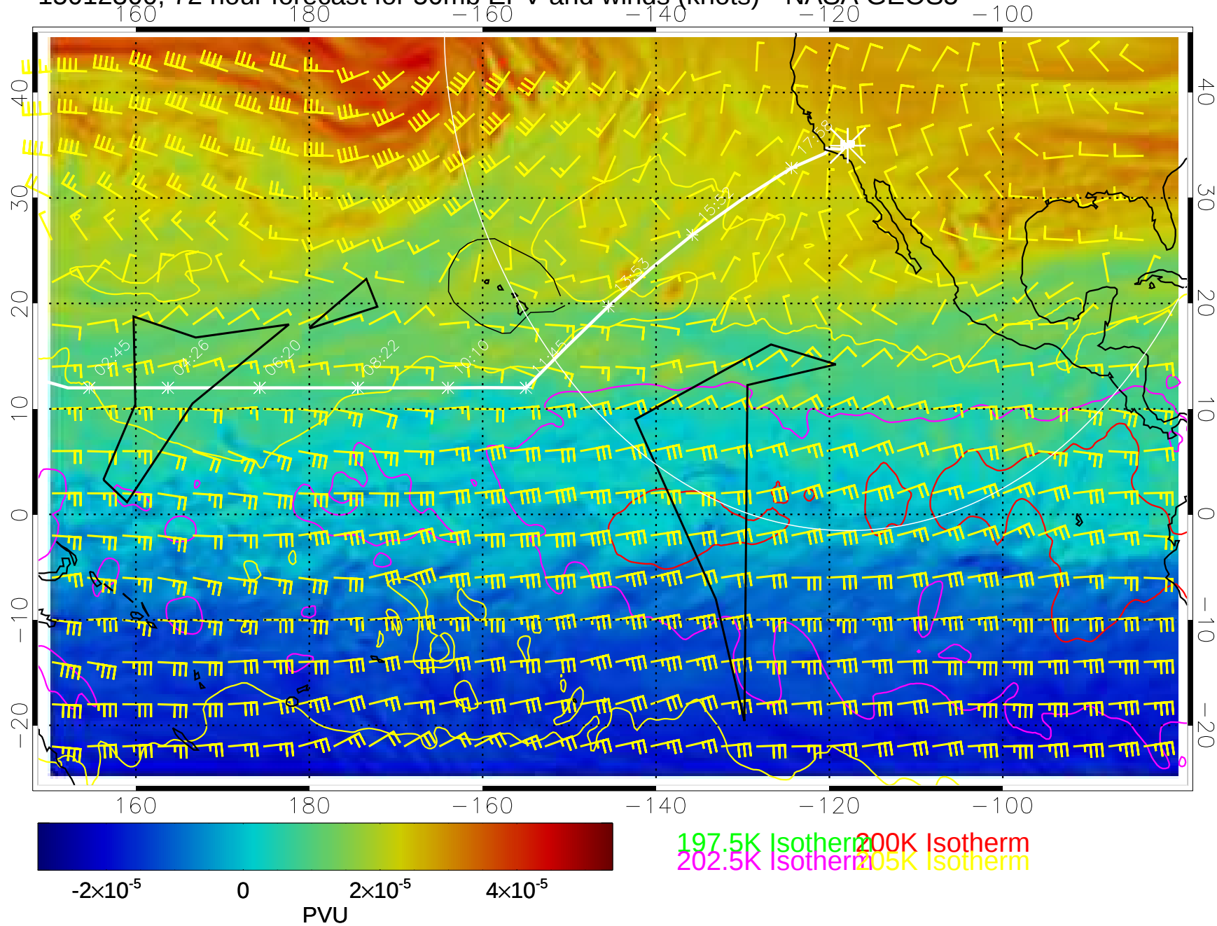
15012300, 72 hour forecast for 50mb EPV and winds (knots)-- NASA GEOS5
