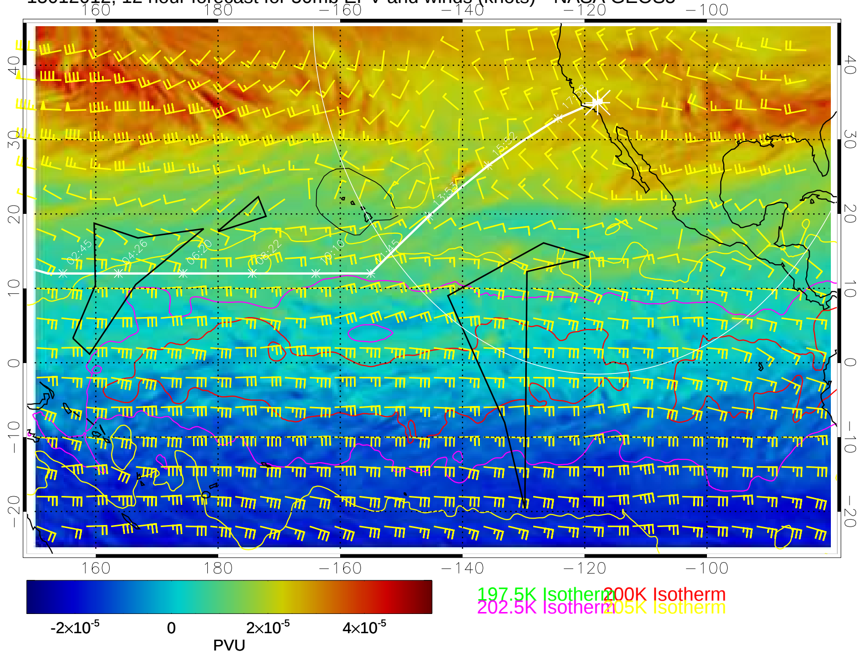
15012012, 12 hour forecast for 50mb EPV and winds (knots)-- NASA GEOS5
