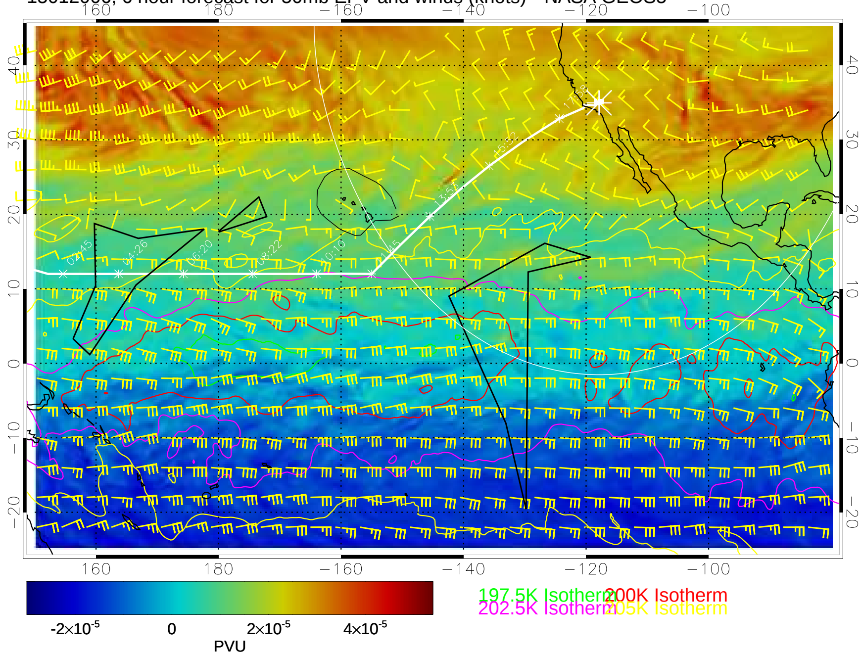
15012006, 6 hour forecast for 50mb EPV and winds (knots)-- NASA GEOS5
