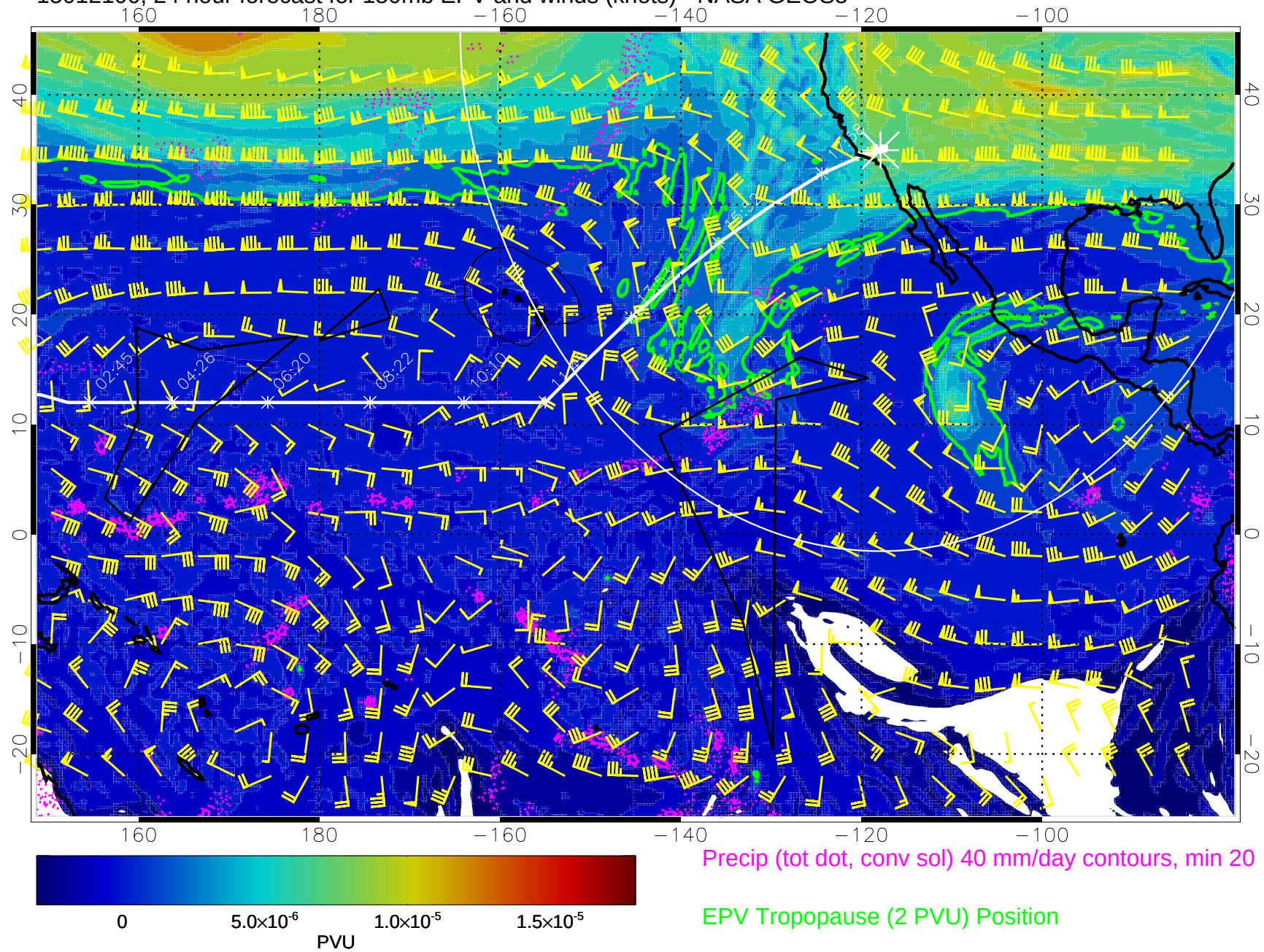
15012100, 24 hour forecast for 150mb EPV and winds (knots) - NASA GEOS5
