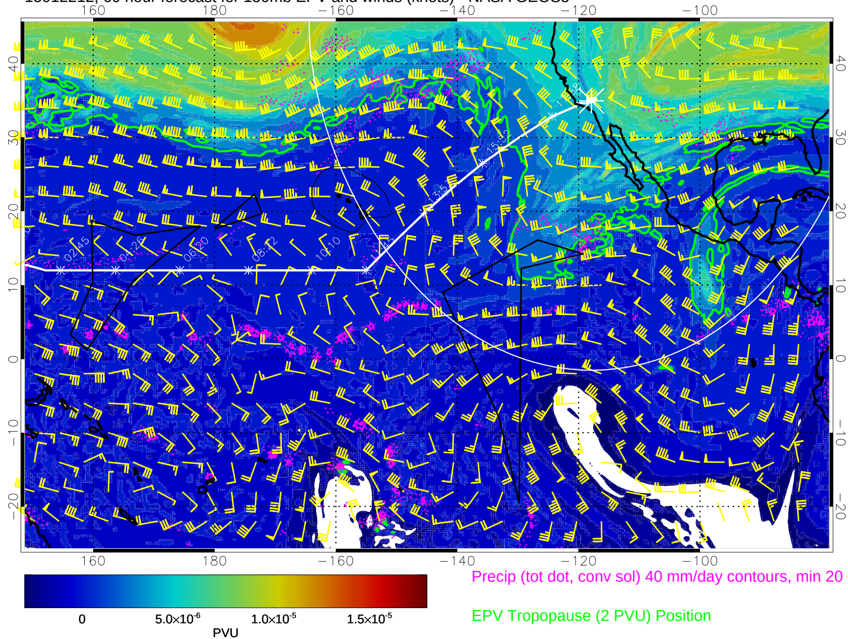
15012212, 60 hour forecast for 150mb EPV and winds (knots) - NASA GEOS5
