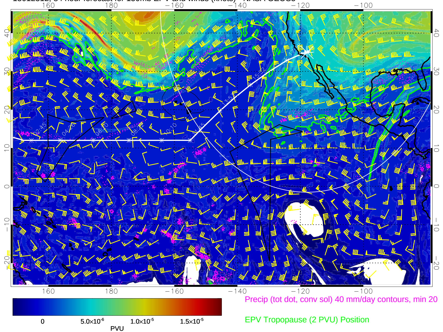
15012312, 84 hour forecast for 150mb EPV and winds (knots) - NASA GEOS5
