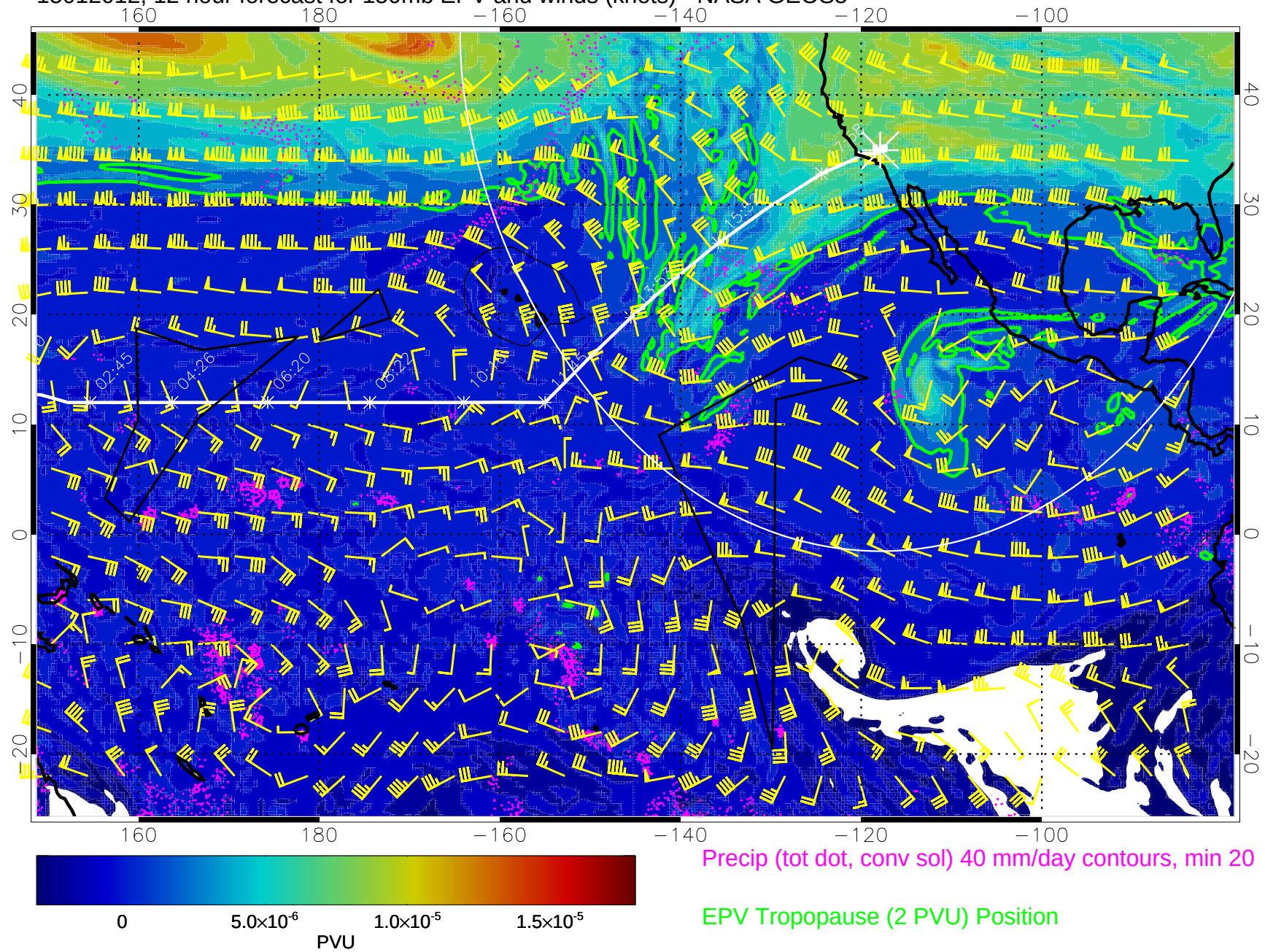
15012012, 12 hour forecast for 150mb EPV and winds (knots) - NASA GEOS5
