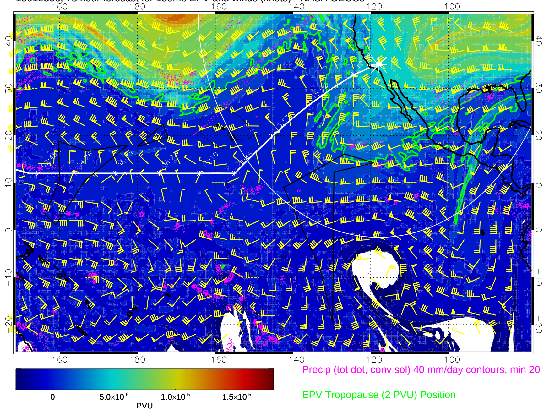
15012306, 78 hour forecast for 150mb EPV and winds (knots) - NASA GEOS5
