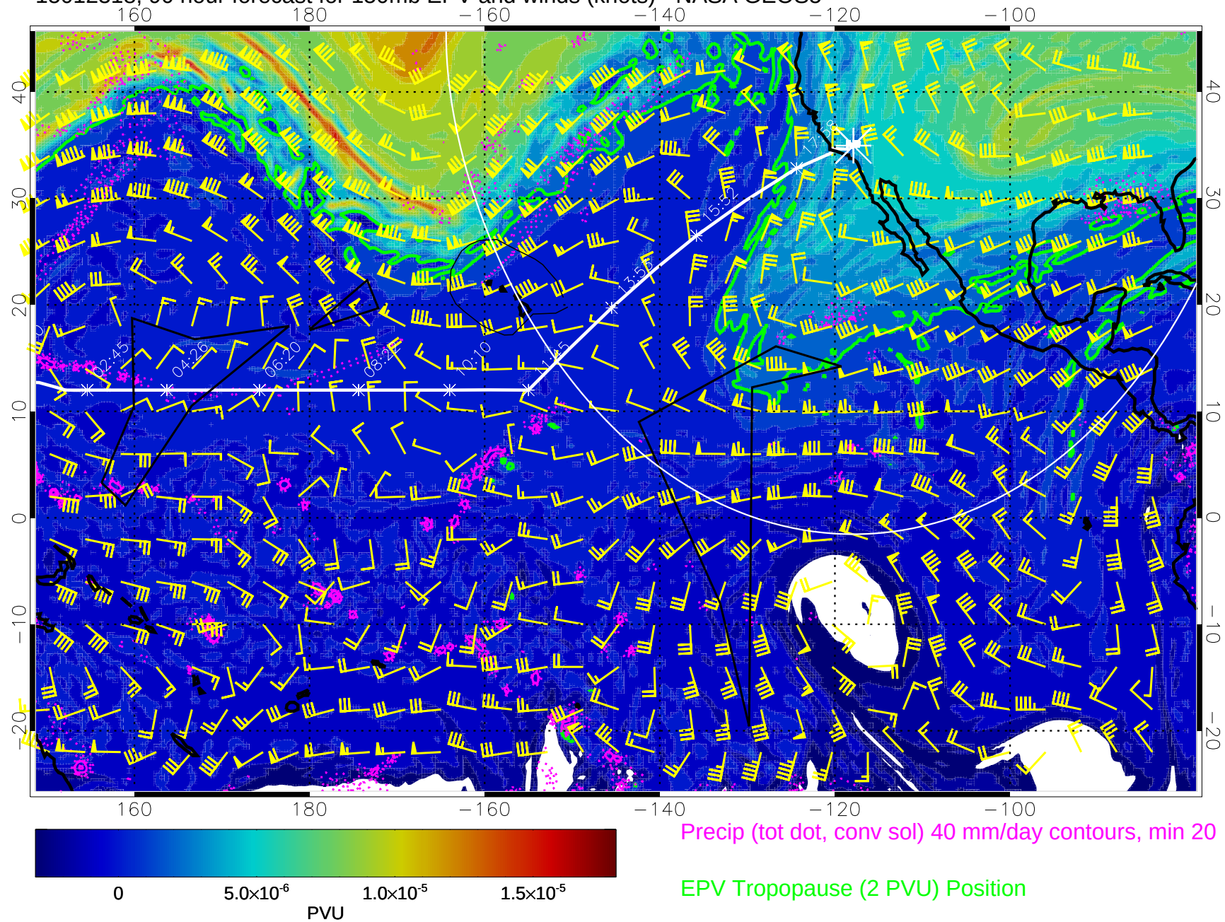
15012318, 90 hour forecast for 150mb EPV and winds (knots) - NASA GEOS5
