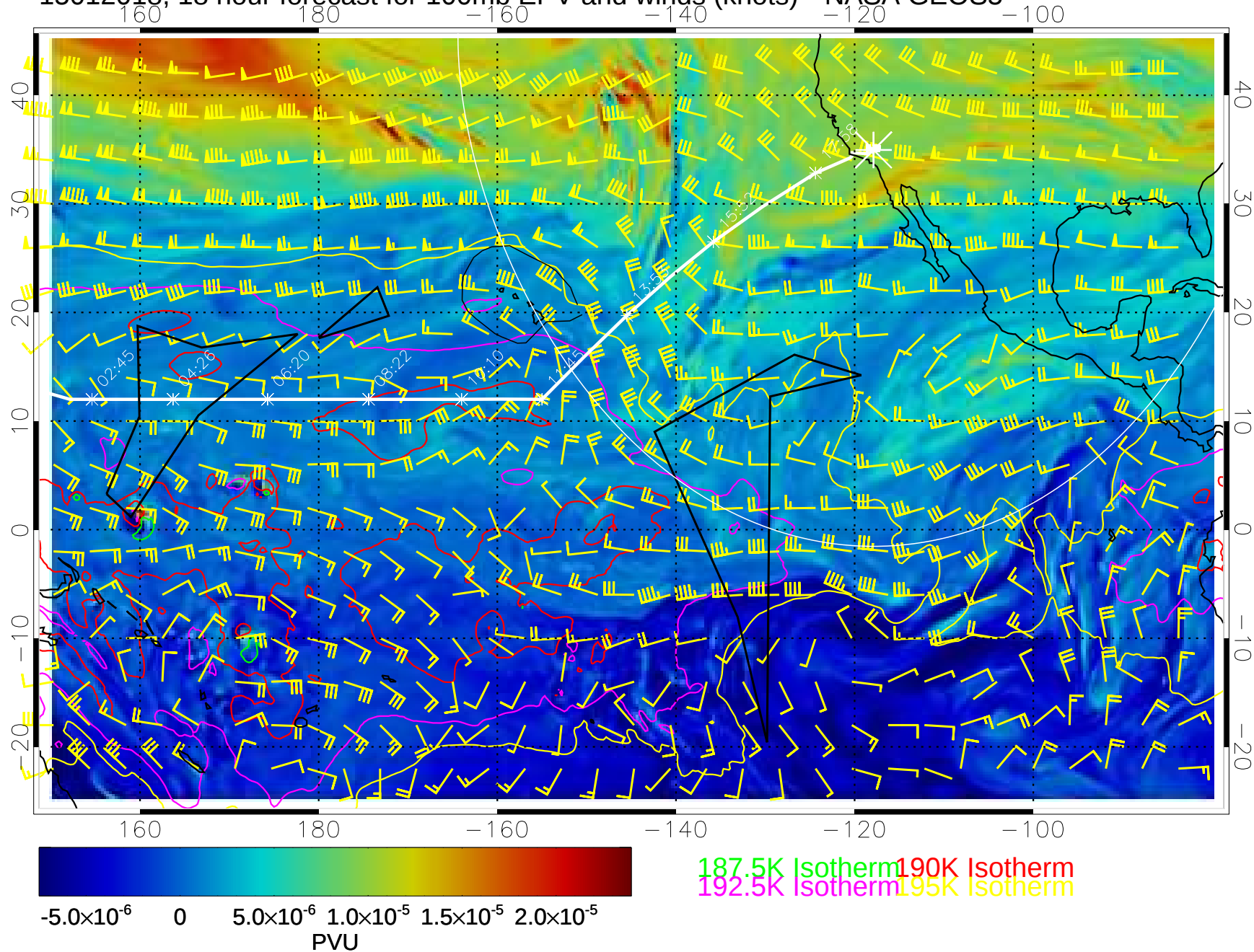
15012018, 18 hour forecast for 100mb EPV and winds (knots)-- NASA GEOS5
