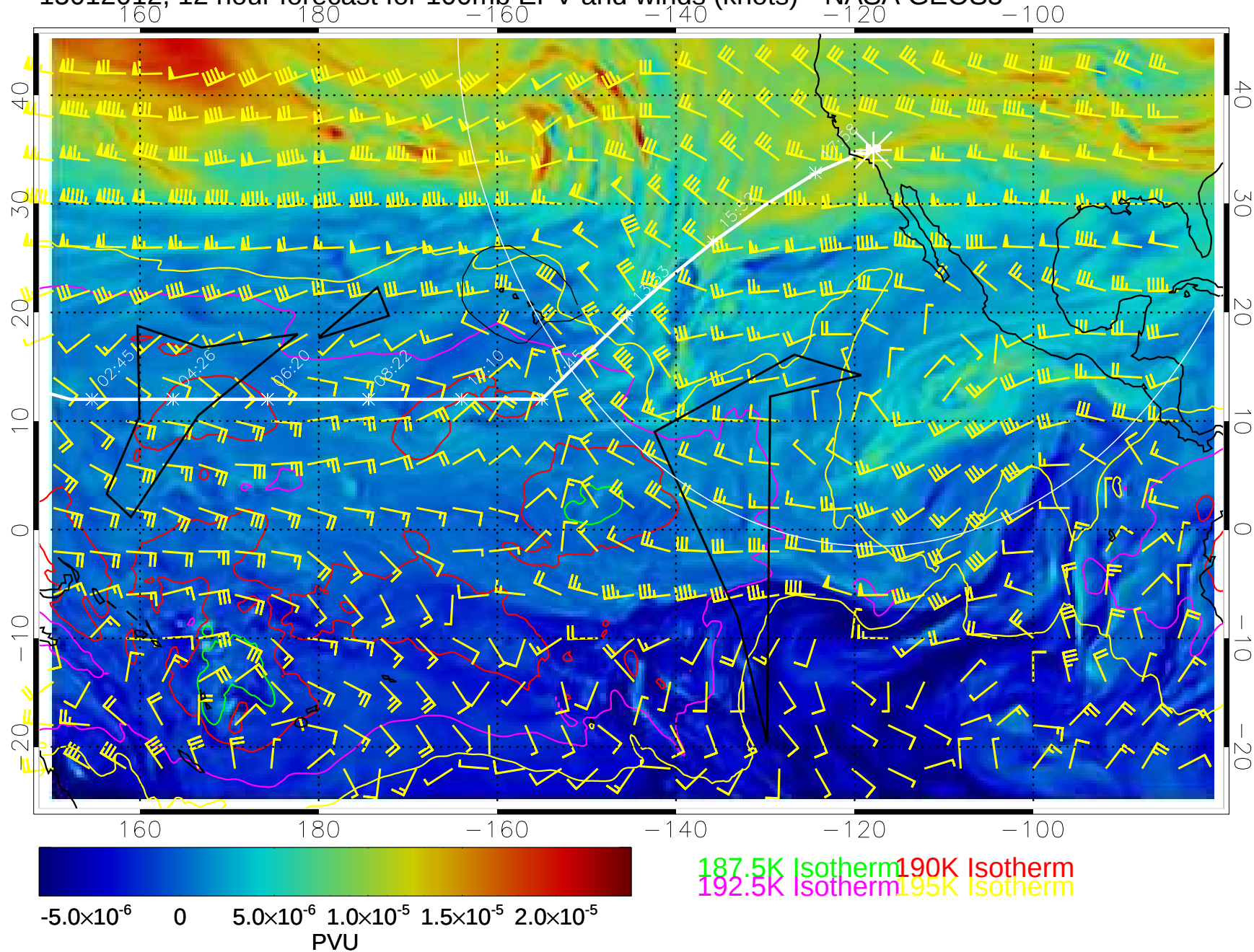
15012012, 12 hour forecast for 100mb EPV and winds (knots)-- NASA GEOS5
