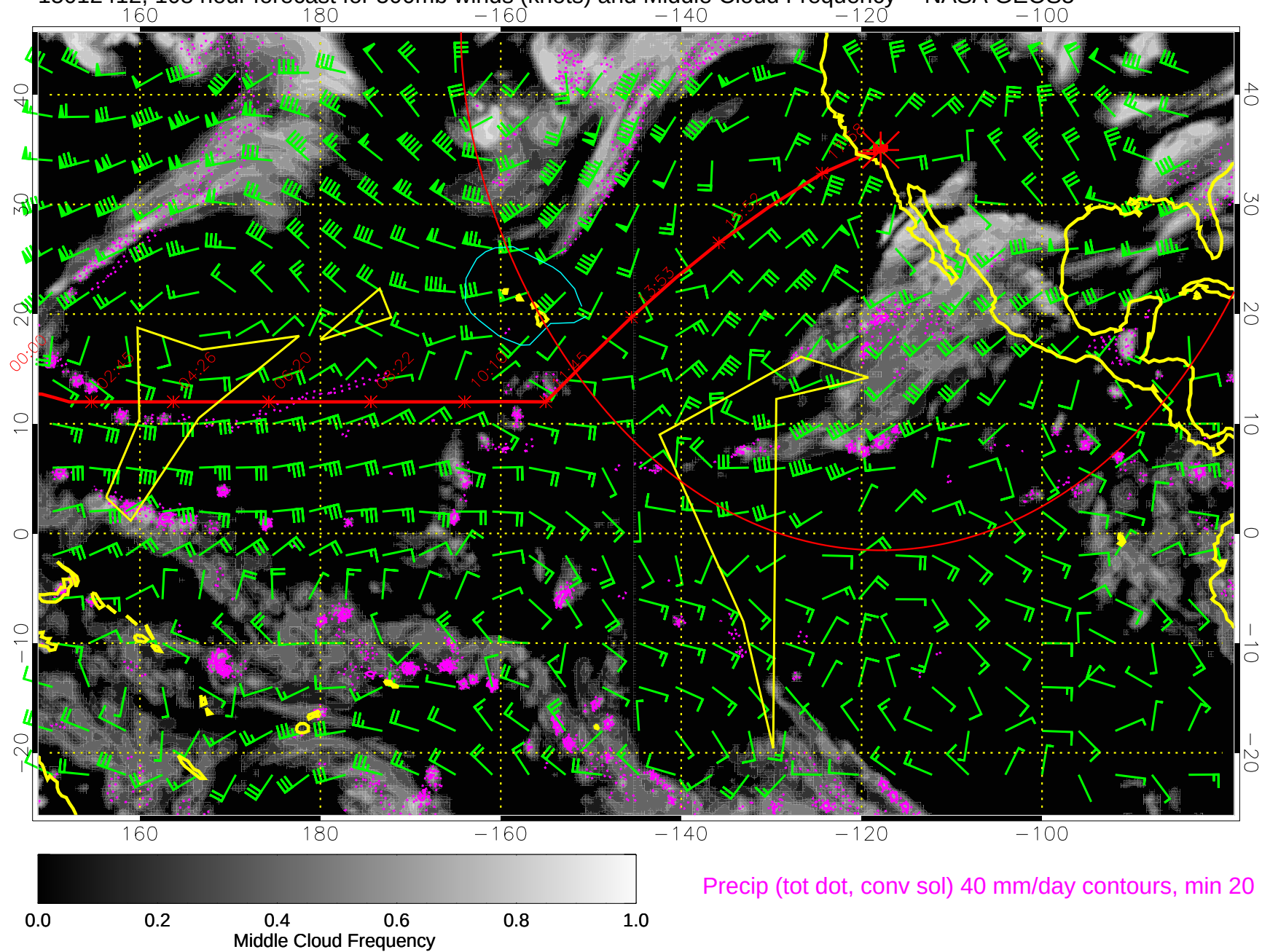
15012412, 108 hour forecast for 500mb winds (knots) and Middle Cloud Frequency -- NASA GEOS5
