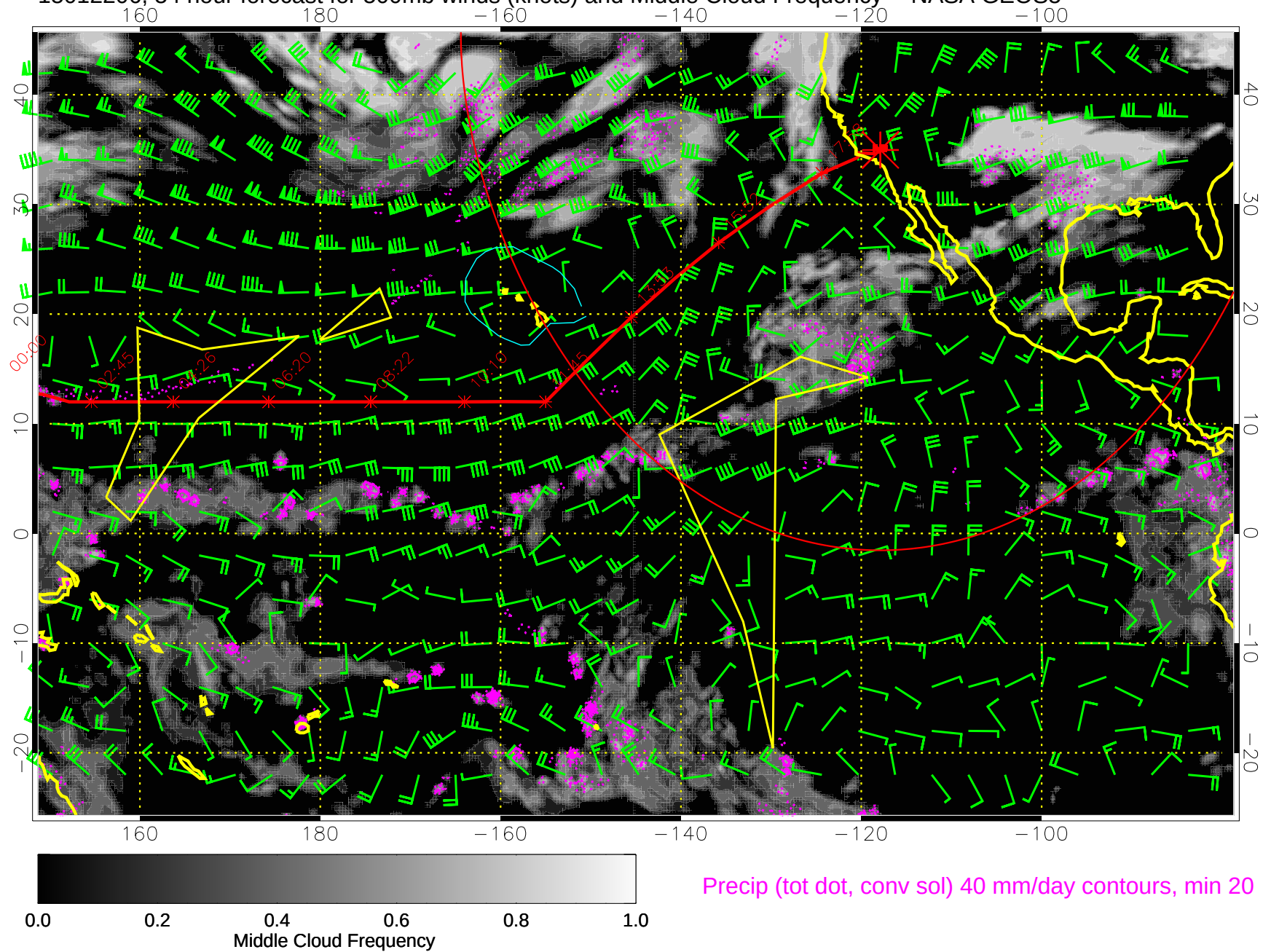
15012206, 54 hour forecast for 500mb winds (knots) and Middle Cloud Frequency -- NASA GEOS5
