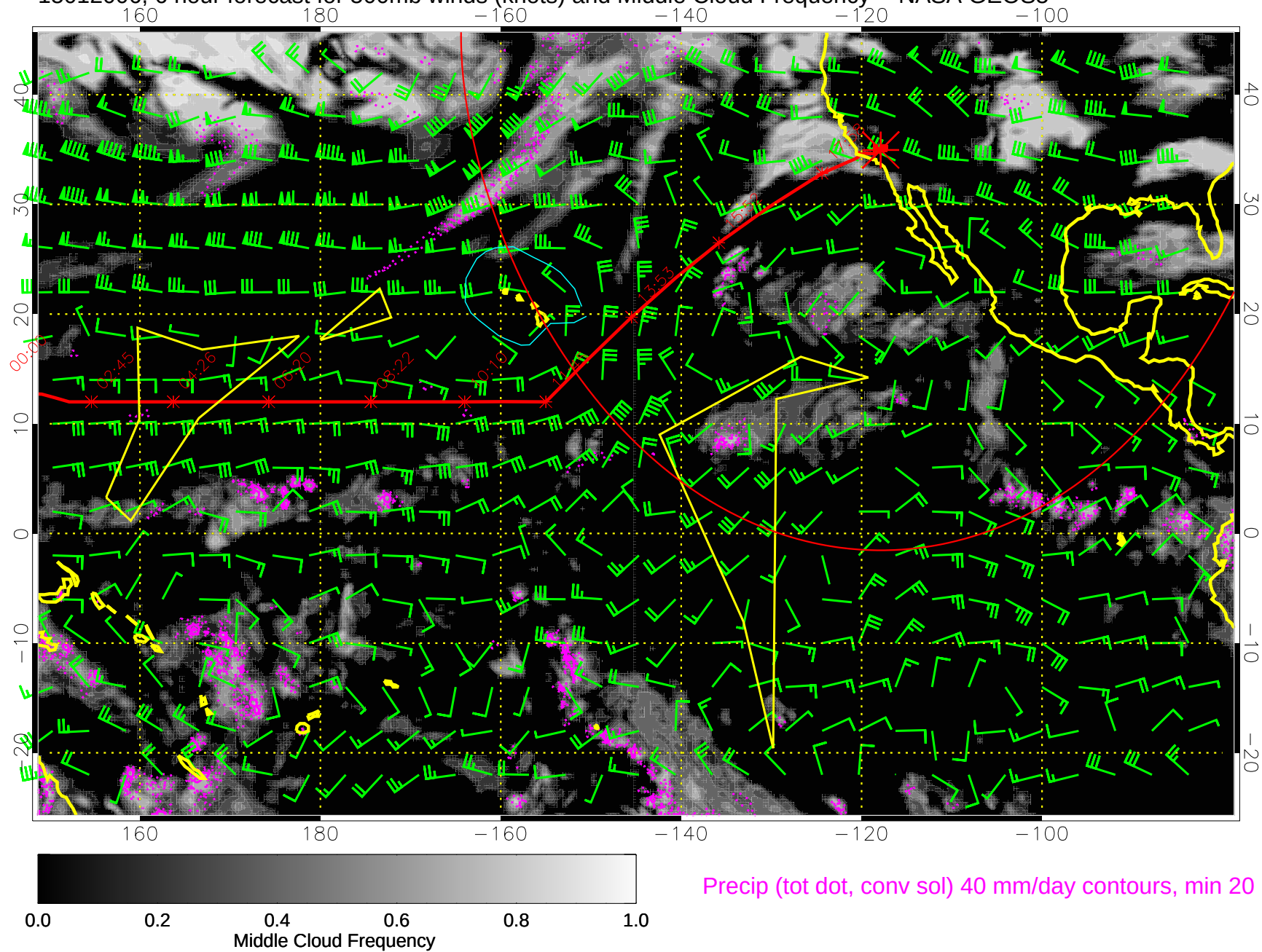
15012006, 6 hour forecast for 500mb winds (knots) and Middle Cloud Frequency -- NASA GEOS5
