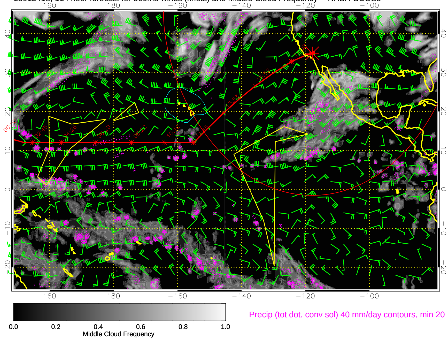
15012418, 114 hour forecast for 500mb winds (knots) and Middle Cloud Frequency -- NASA GEOS5
