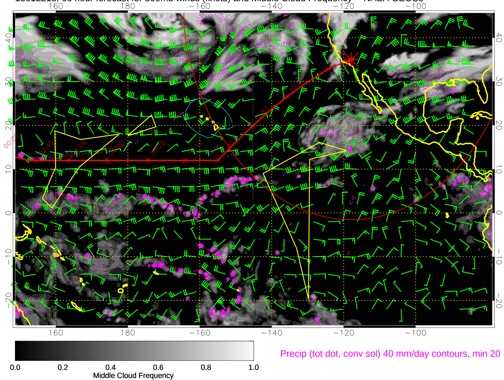
15012218, 66 hour forecast for 500mb winds (knots) and Middle Cloud Frequency -- NASA GEOS5
