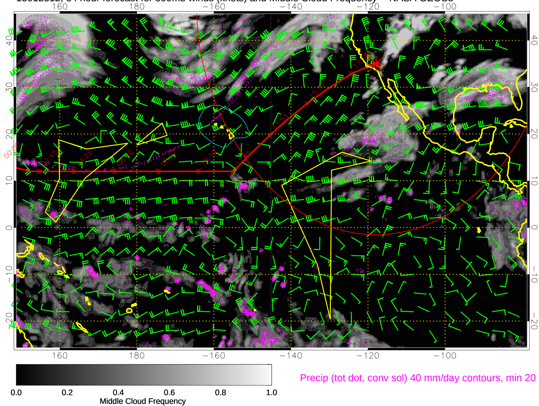
15012312, 84 hour forecast for 500mb winds (knots) and Middle Cloud Frequency -- NASA GEOS5
