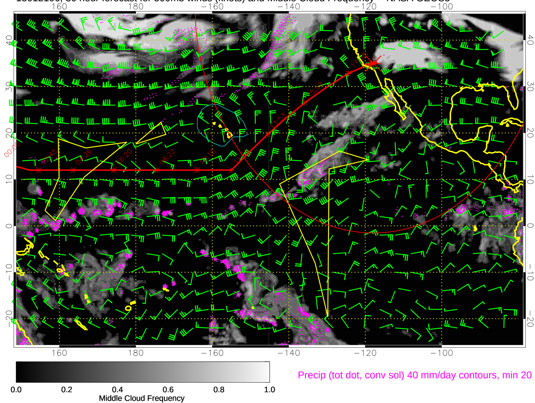
15012106, 30 hour forecast for 500mb winds (knots) and Middle Cloud Frequency -- NASA GEOS5
