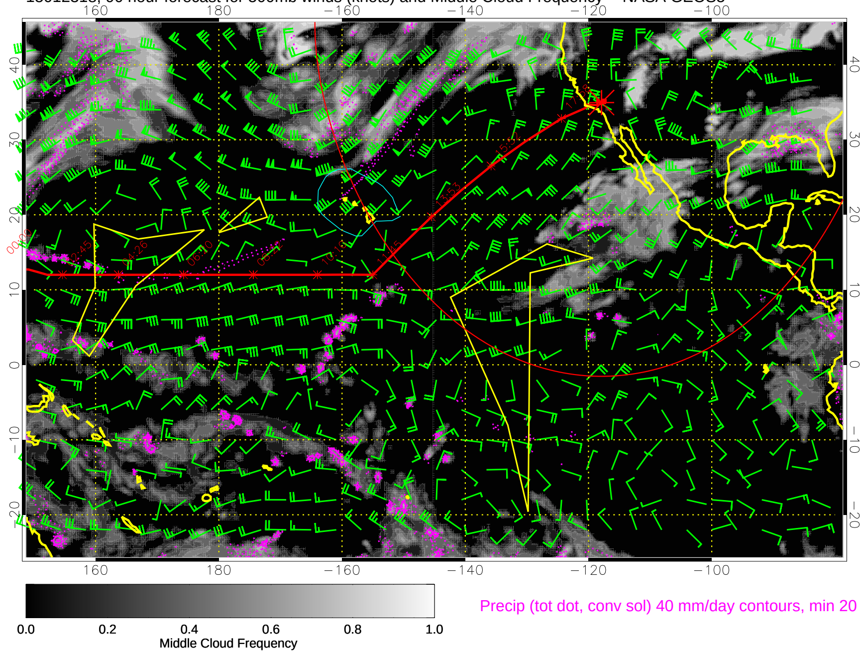
15012318, 90 hour forecast for 500mb winds (knots) and Middle Cloud Frequency -- NASA GEOS5
