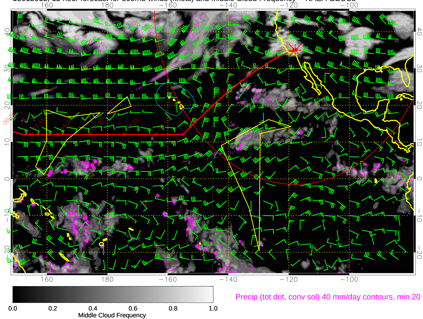
15012012, 12 hour forecast for 500mb winds (knots) and Middle Cloud Frequency -- NASA GEOS5
