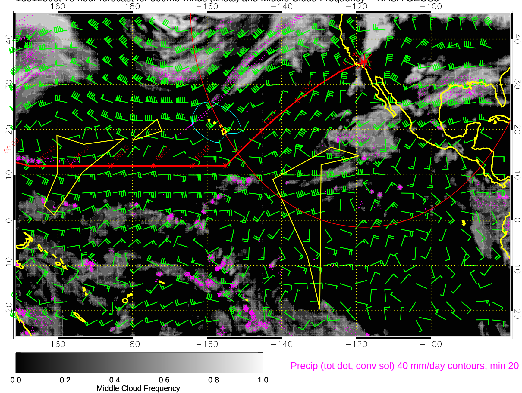
15012306, 78 hour forecast for 500mb winds (knots) and Middle Cloud Frequency -- NASA GEOS5
