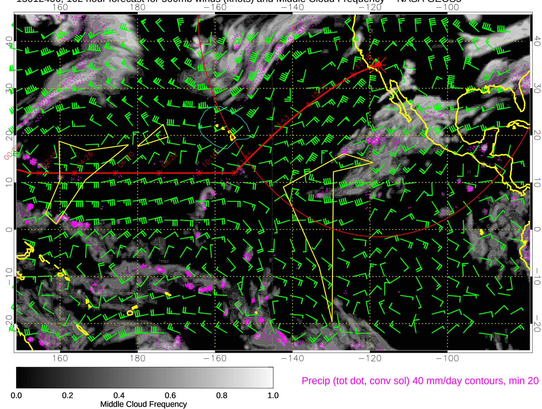
15012406, 102 hour forecast for 500mb winds (knots) and Middle Cloud Frequency -- NASA GEOS5
