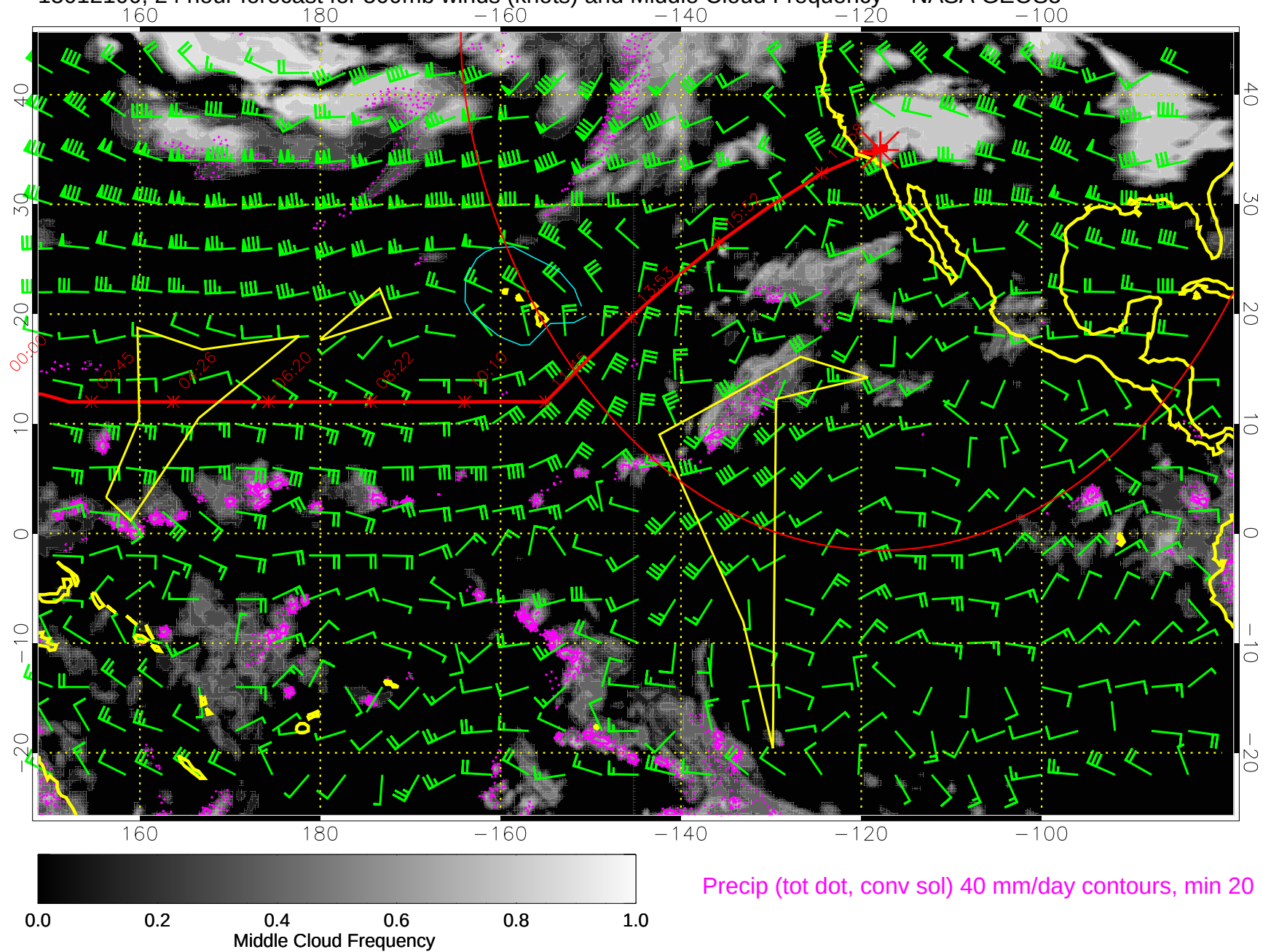
15012100, 24 hour forecast for 500mb winds (knots) and Middle Cloud Frequency -- NASA GEOS5
