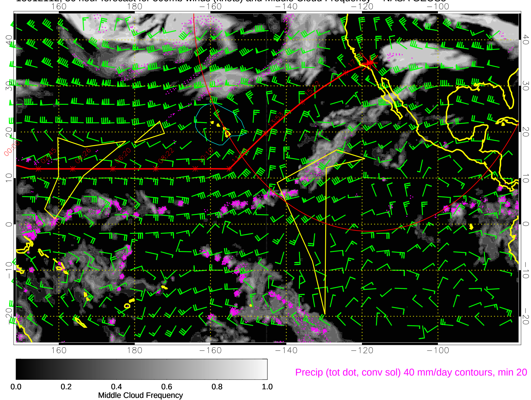
15012112, 36 hour forecast for 500mb winds (knots) and Middle Cloud Frequency -- NASA GEOS5
