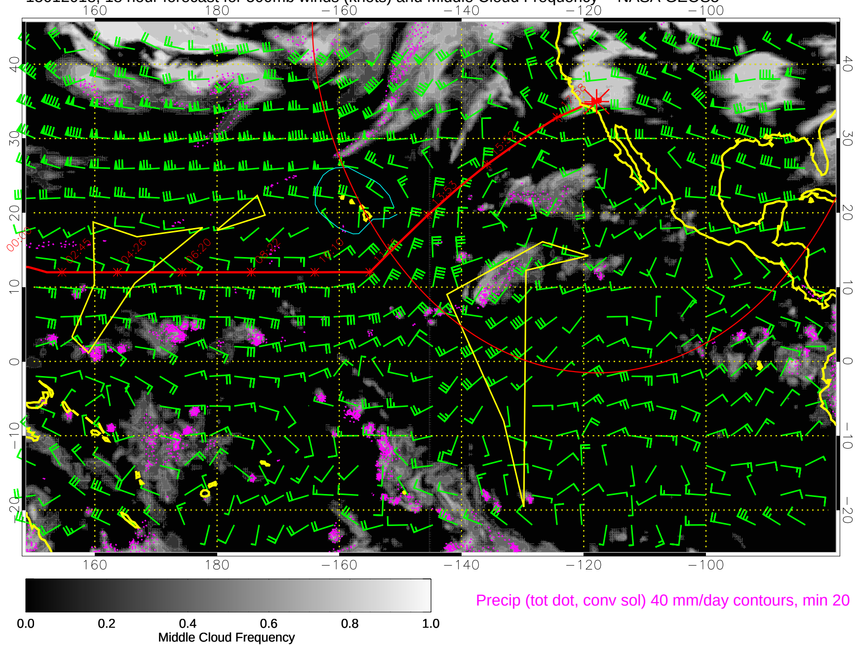
15012018, 18 hour forecast for 500mb winds (knots) and Middle Cloud Frequency -- NASA GEOS5
