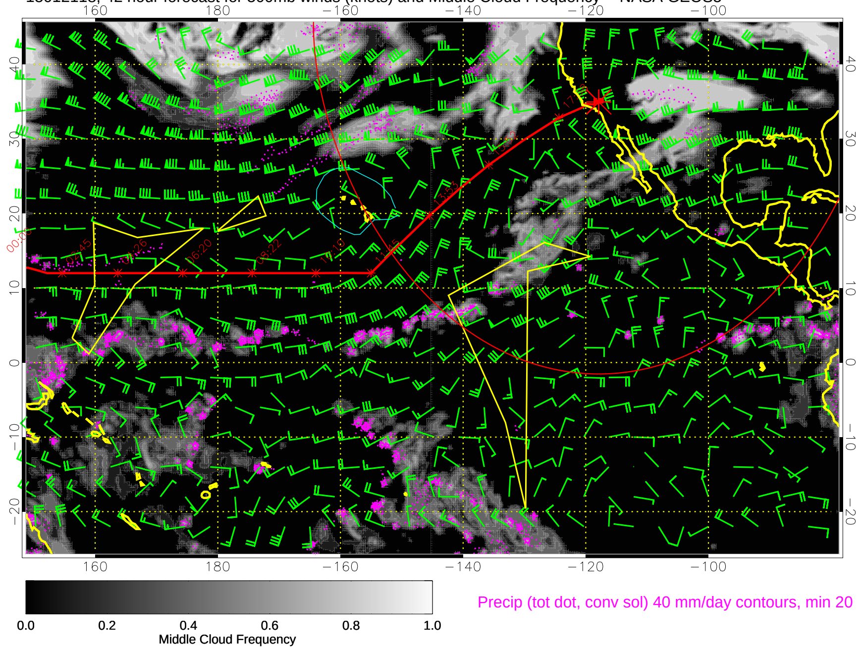
15012118, 42 hour forecast for 500mb winds (knots) and Middle Cloud Frequency -- NASA GEOS5
