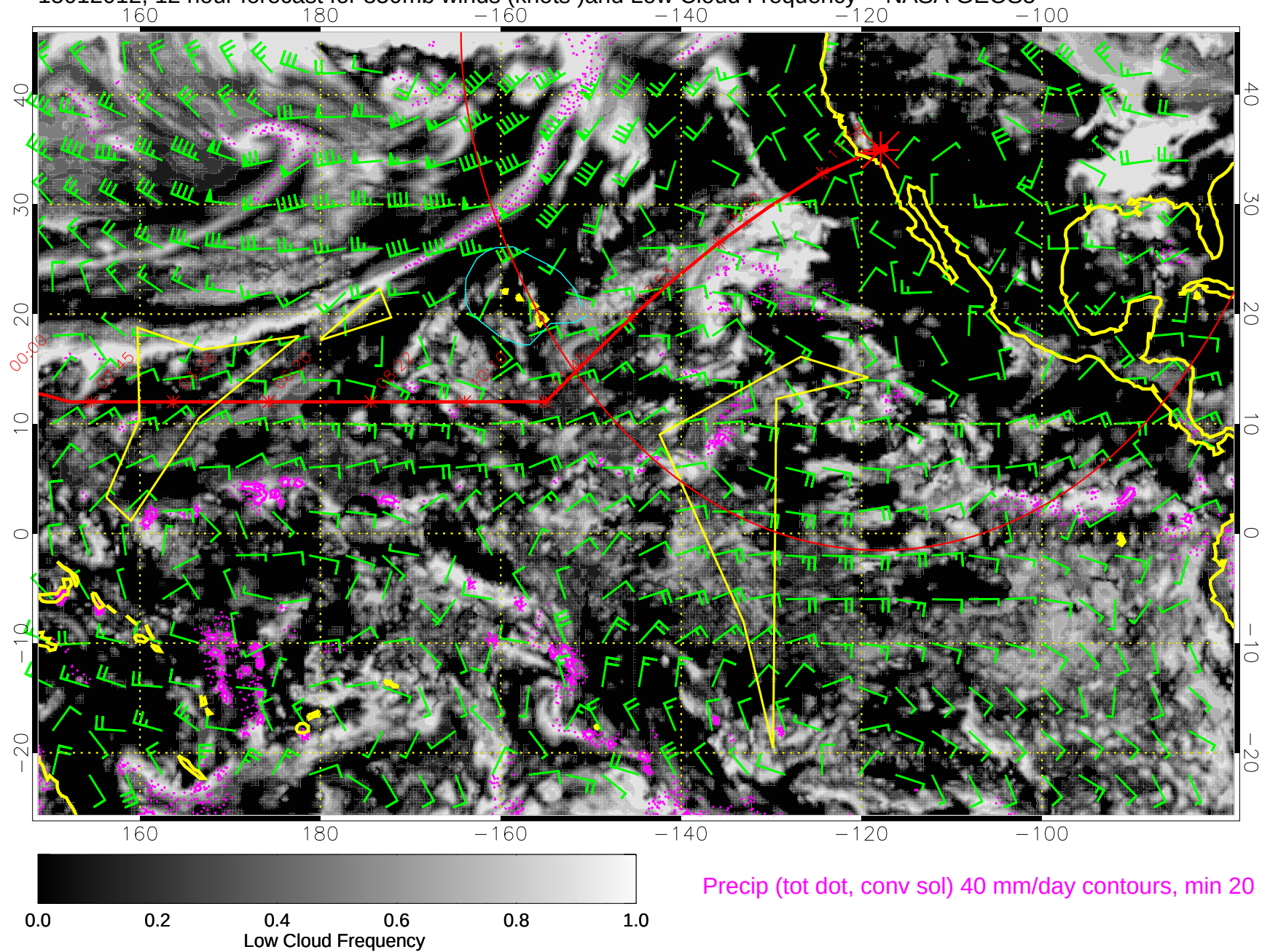
15012012, 12 hour forecast for 850mb winds (knots) and Low Cloud Frequency -- NASA GEOS5
