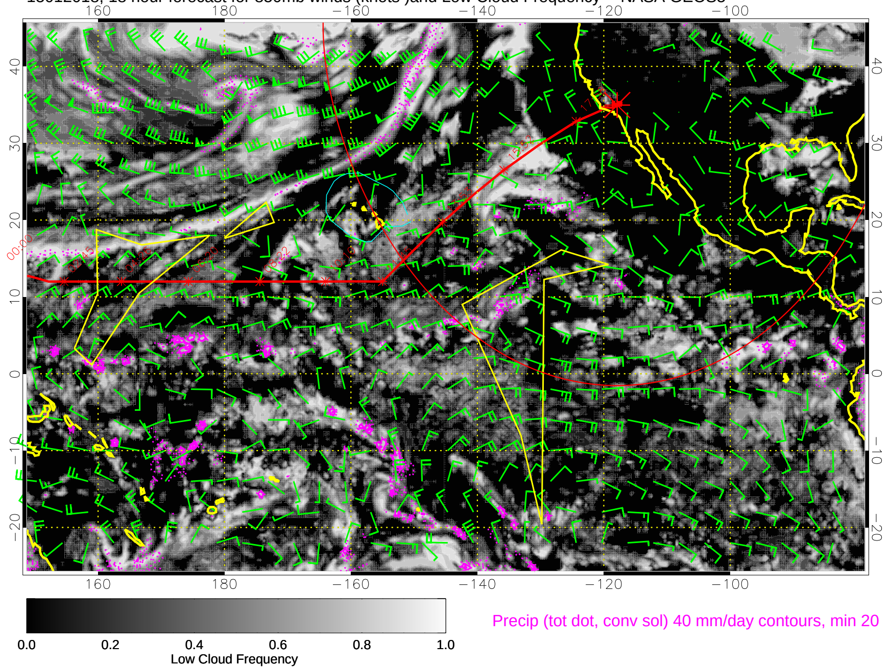
15012018, 18 hour forecast for 850mb winds (knots) and Low Cloud Frequency -- NASA GEOS5
