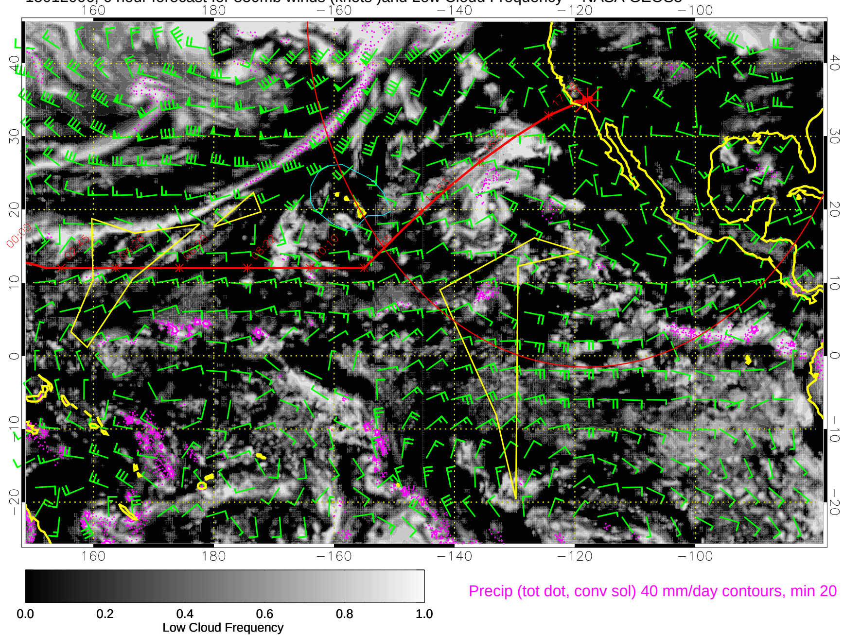
15012006, 6 hour forecast for 850mb winds (knots )and Low Cloud Frequency -- NASA GEOS5
