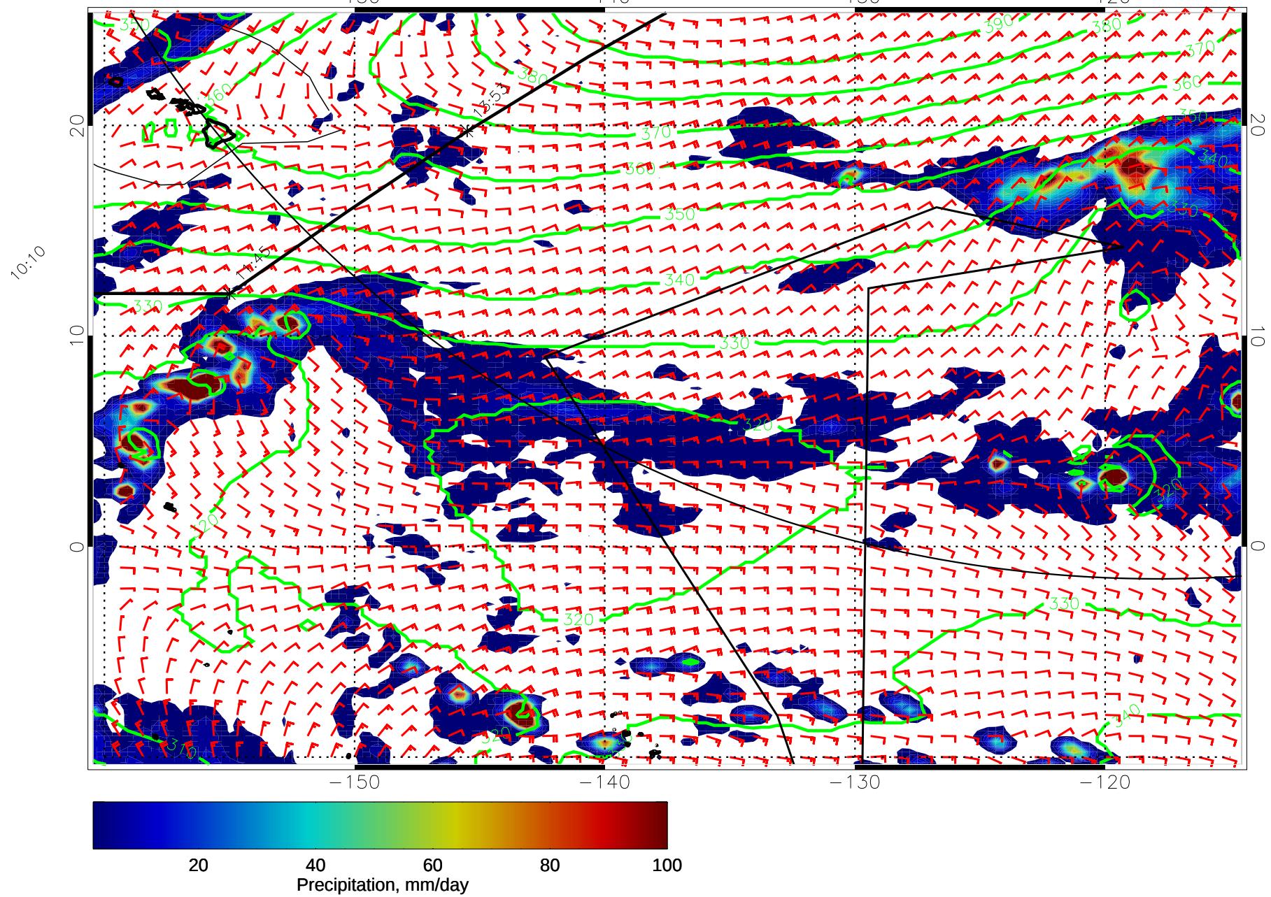
15012312, 108 hour forecast for 975mb Z, Precip., and Surface Winds (knots) -- NASA GEOS5
