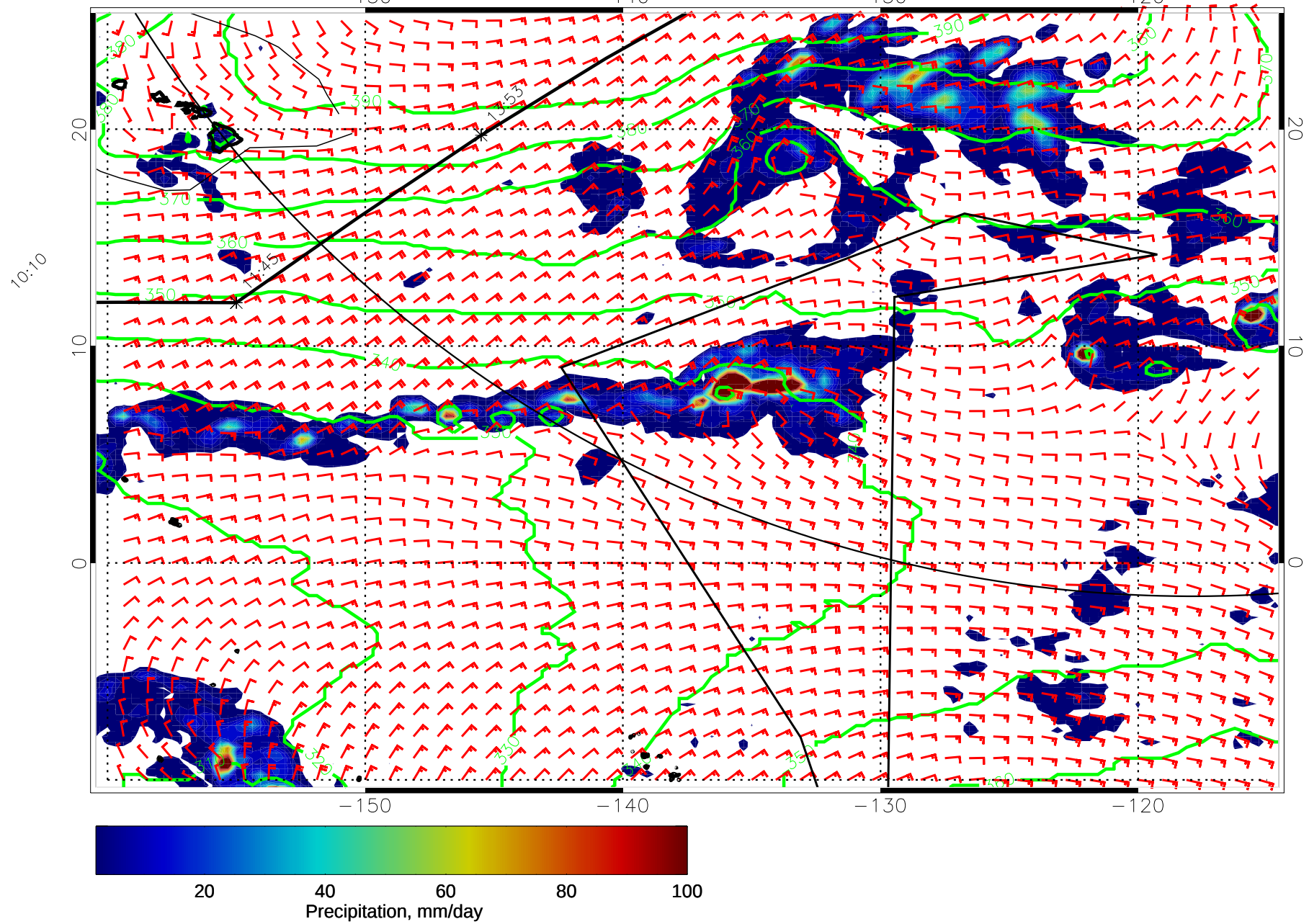
15012006, 30 hour forecast for 975mb Z, Precip., and Surface Winds (knots) -- NASA GEOS5
