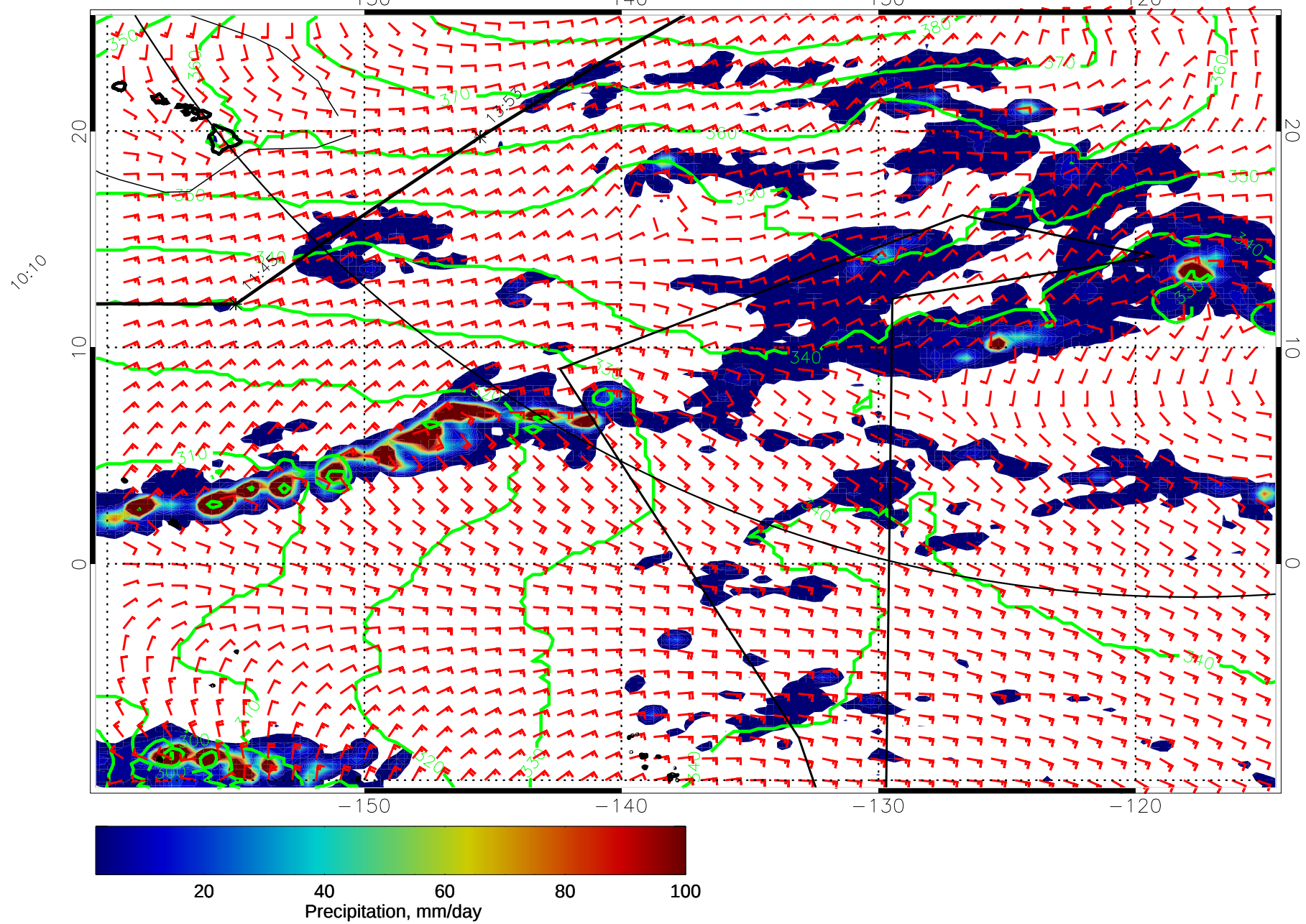
15012118, 66 hour forecast for 975mb Z, Precip., and Surface Winds (knots) -- NASA GEOS5
