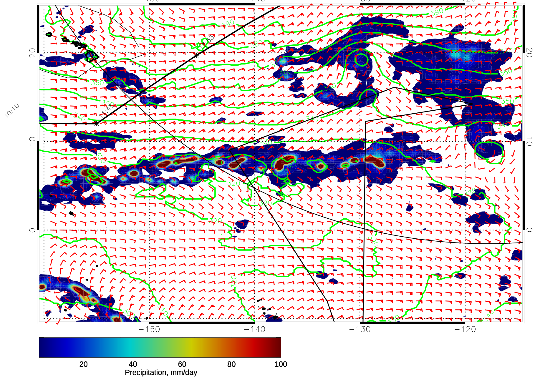
15011912, 12 hour forecast for 975mb Z, Precip., and Surface Winds (knots) -- NASA GEOS5
