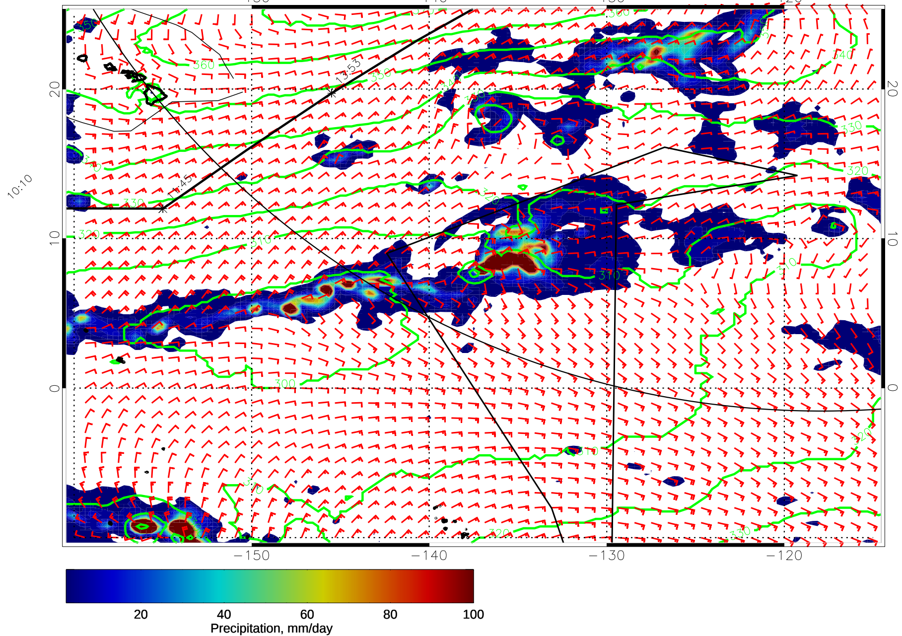
15012100, 48 hour forecast for 975mb Z, Precip., and Surface Winds (knots) -- NASA GEOS5
