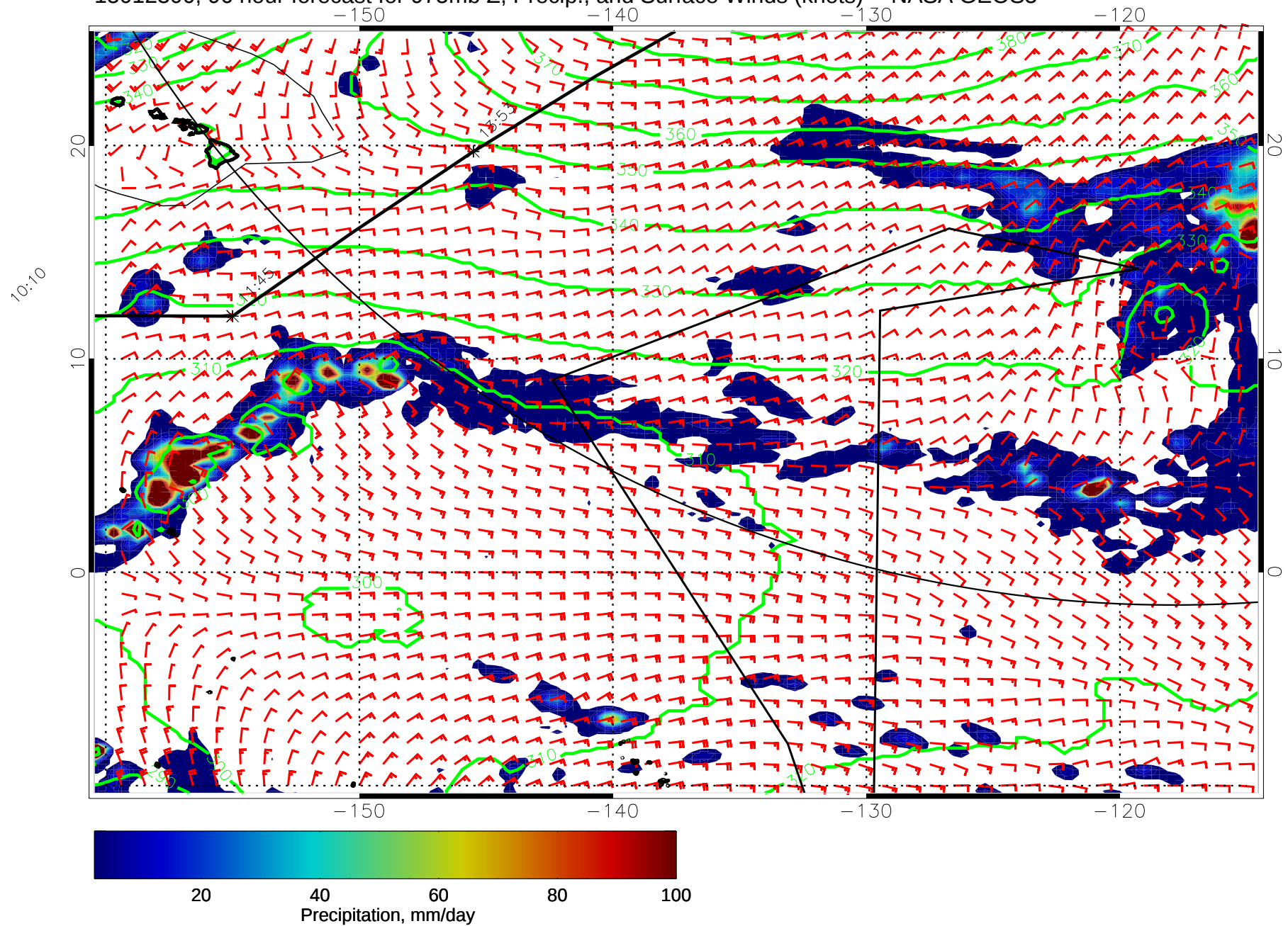
15012300, 96 hour forecast for 975mb Z, Precip., and Surface Winds (knots) -- NASA GEOS5
