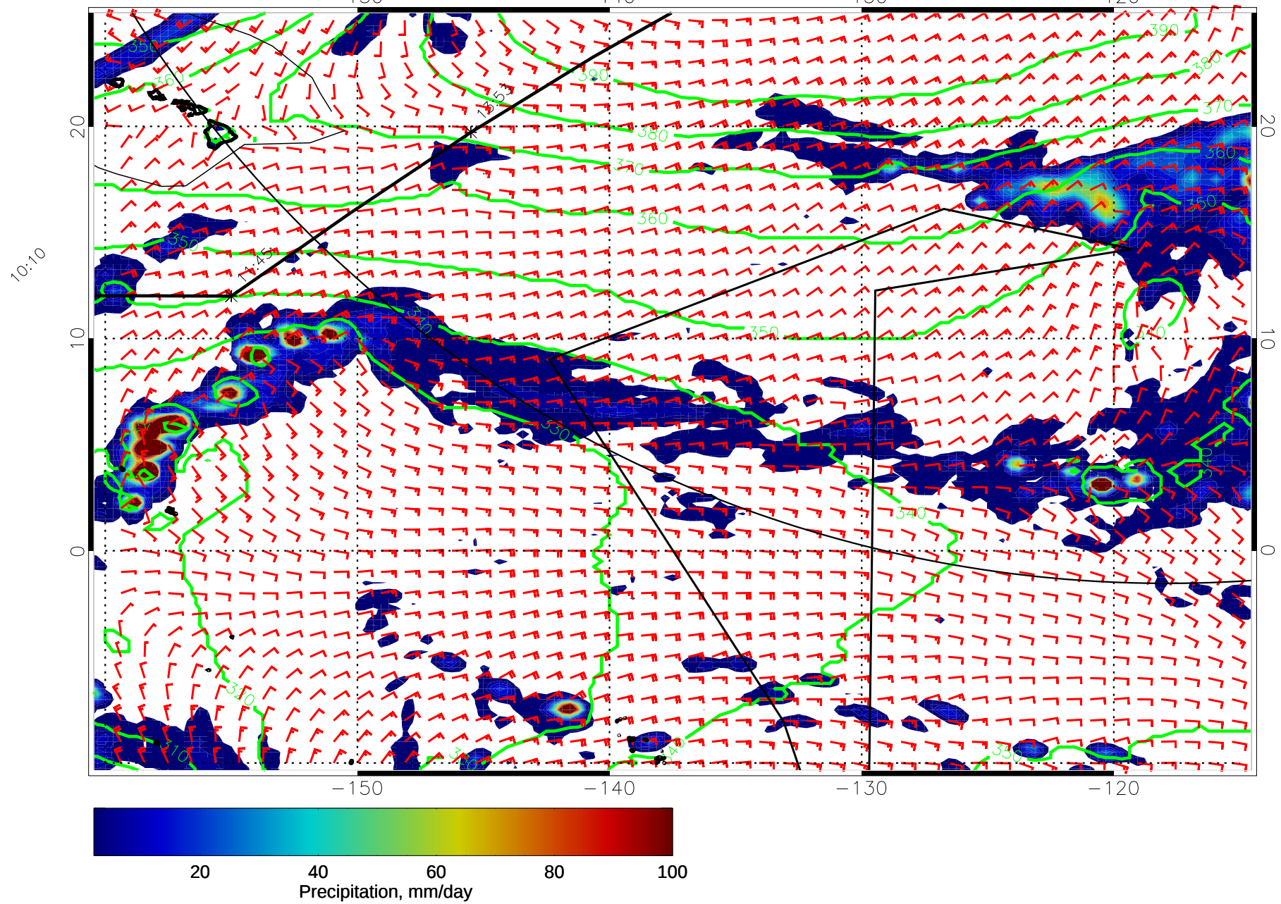
15012306, 102 hour forecast for 975mb Z, Precip., and Surface Winds (knots) -- NASA GEOS5
