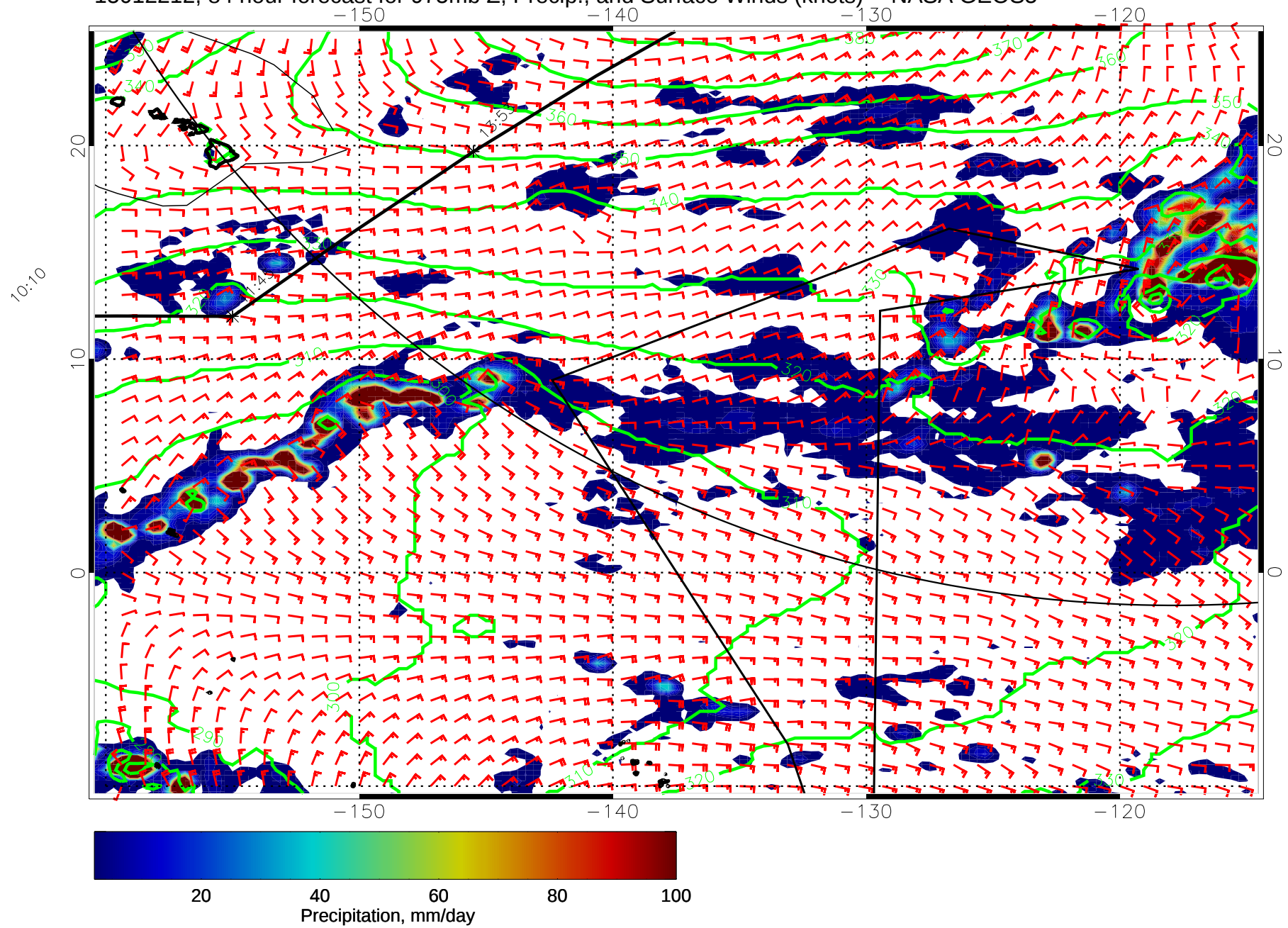
15012212, 84 hour forecast for 975mb Z, Precip., and Surface Winds (knots) -- NASA GEOS5
