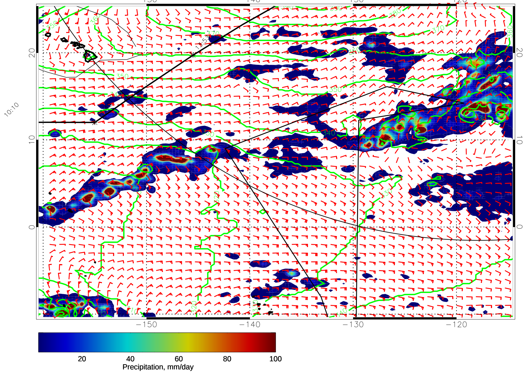
15012206, 78 hour forecast for 975mb Z, Precip., and Surface Winds (knots) -- NASA GEOS5
