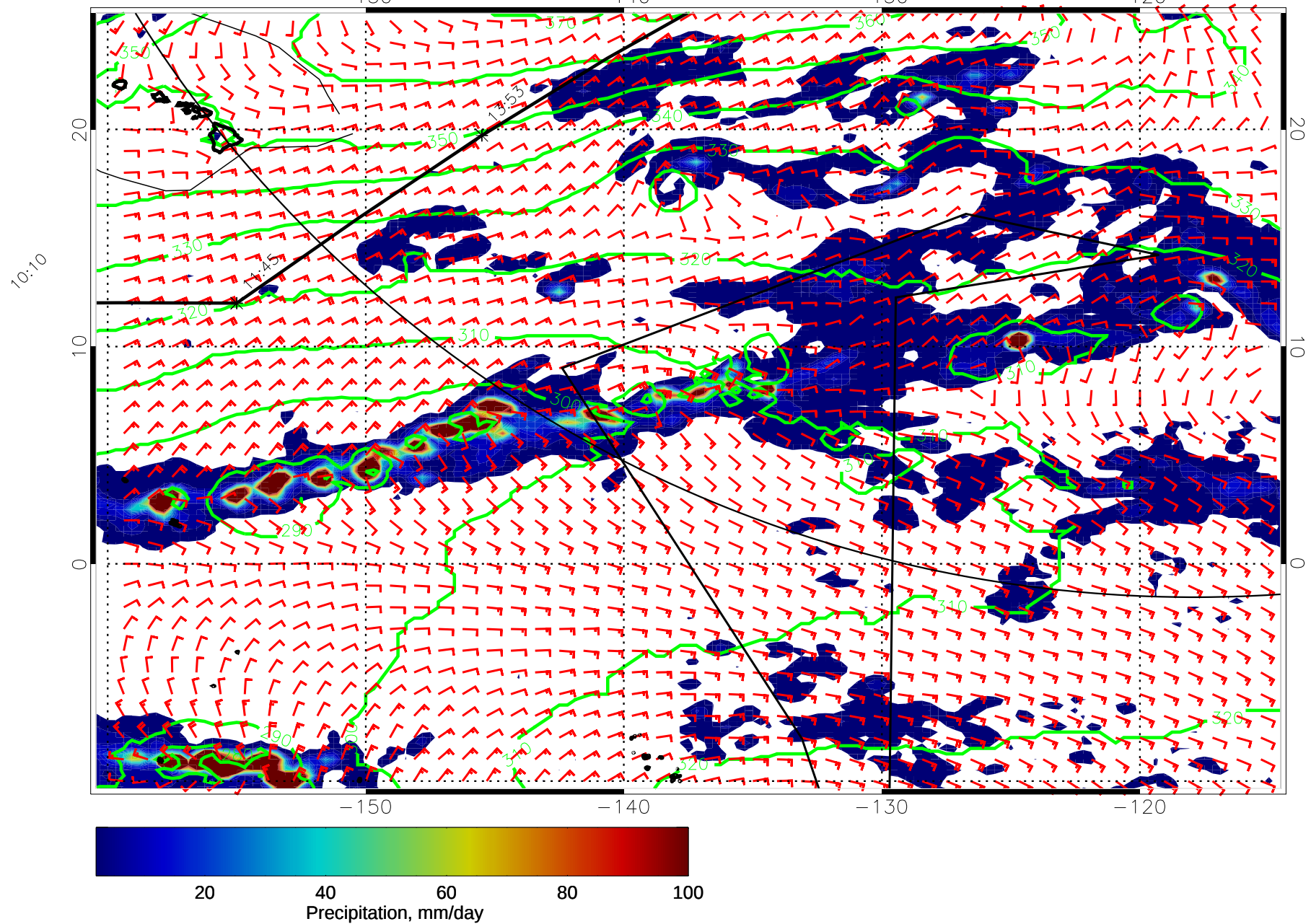
15012112, 60 hour forecast for 975mb Z, Precip., and Surface Winds (knots) -- NASA GEOS5
