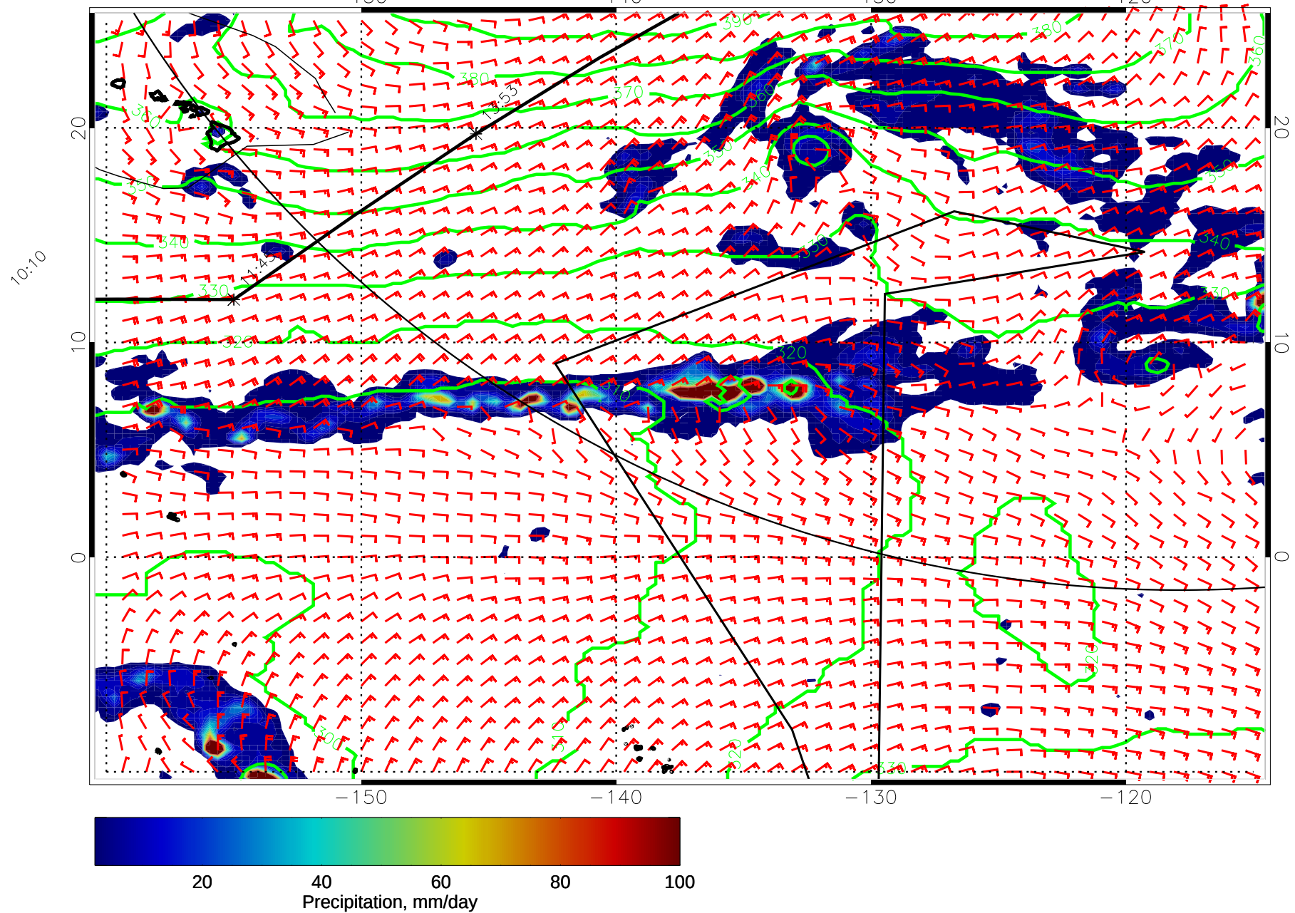
15012000, 24 hour forecast for 975mb Z, Precip., and Surface Winds (knots) -- NASA GEOS5
