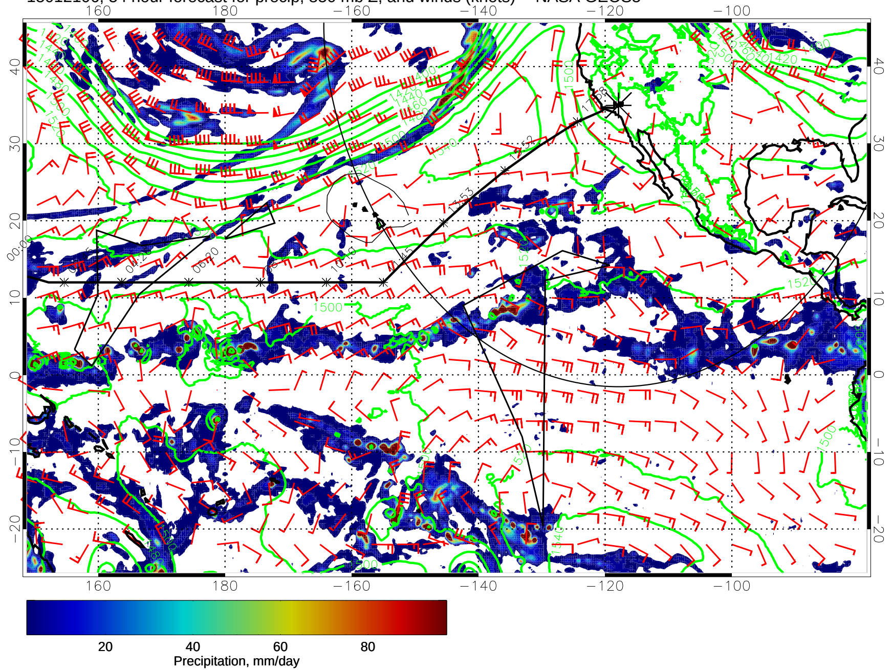
15012106, 54 hour forecast for precip, 850 mb Z, and winds (knots) -- NASA GEOS5
