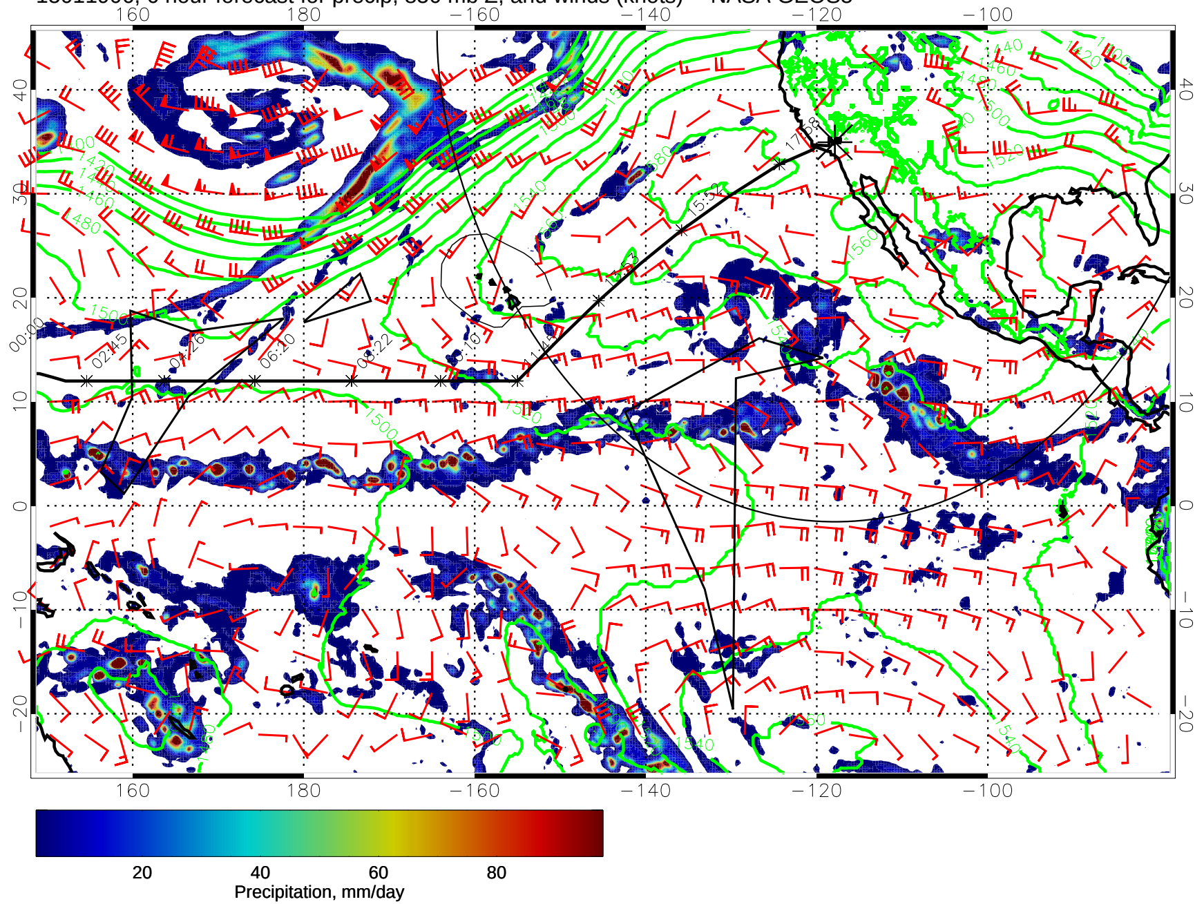
15011906, 6 hour forecast for precip, 850 mb Z, and winds (knots) -- NASA GEOS5
