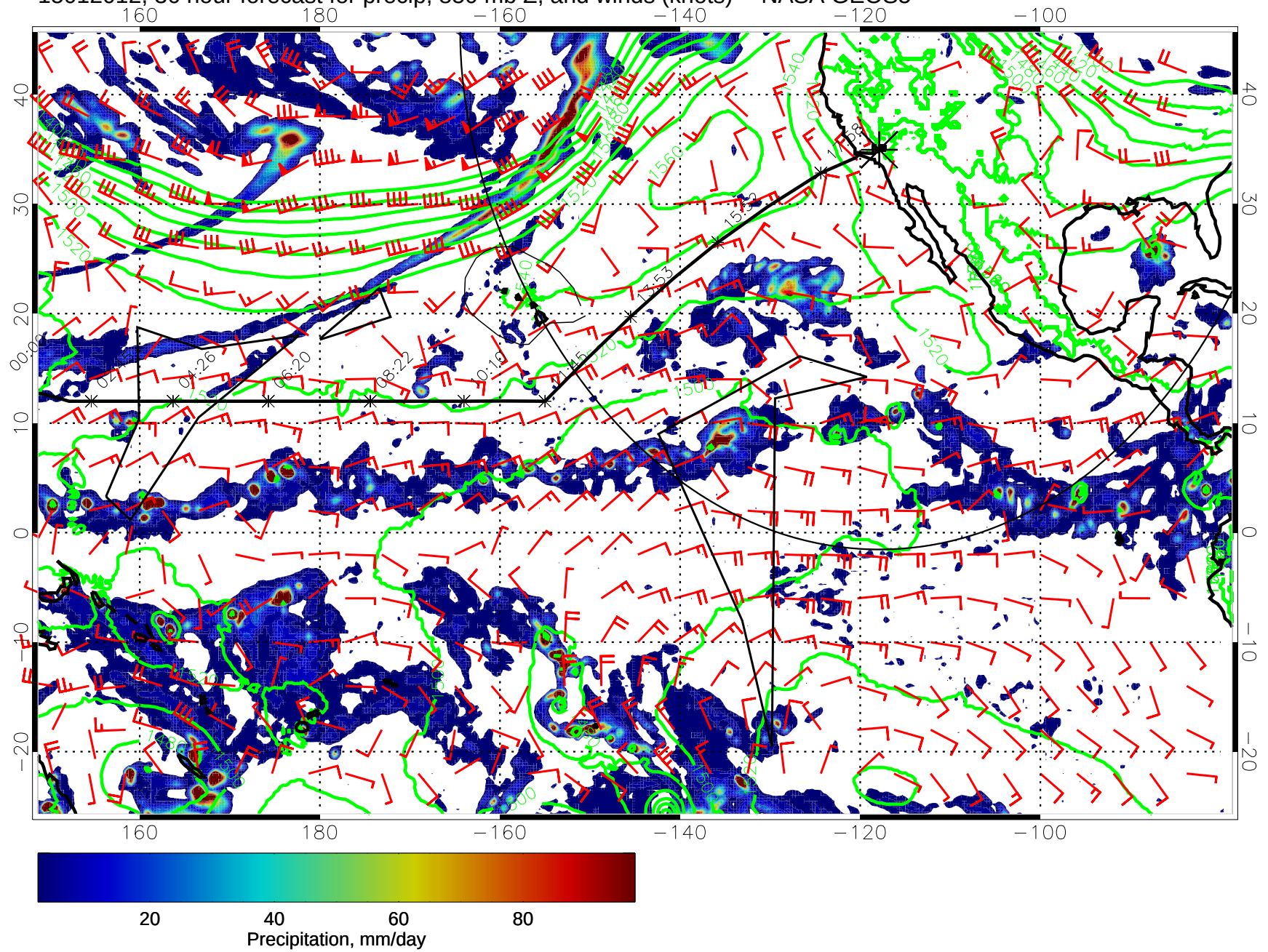
15012012, 36 hour forecast for precip, 850 mb Z, and winds (knots) -- NASA GEOS5
