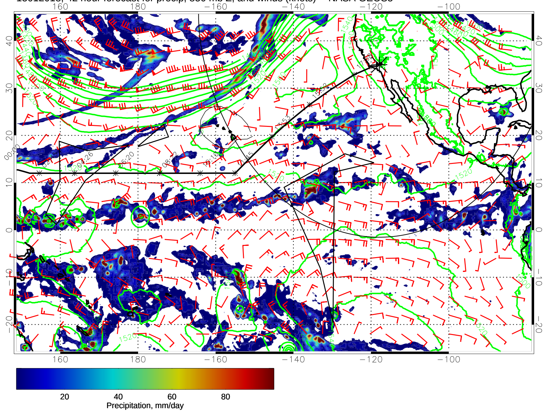
15012018, 42 hour forecast for precip, 850 mb Z, and winds (knots) -- NASA GEOS5
