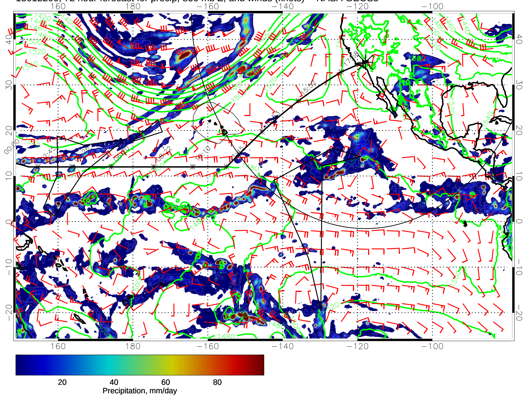
15012200, 72 hour forecast for precip, 850 mb Z, and winds (knots) -- NASA GEOS5
