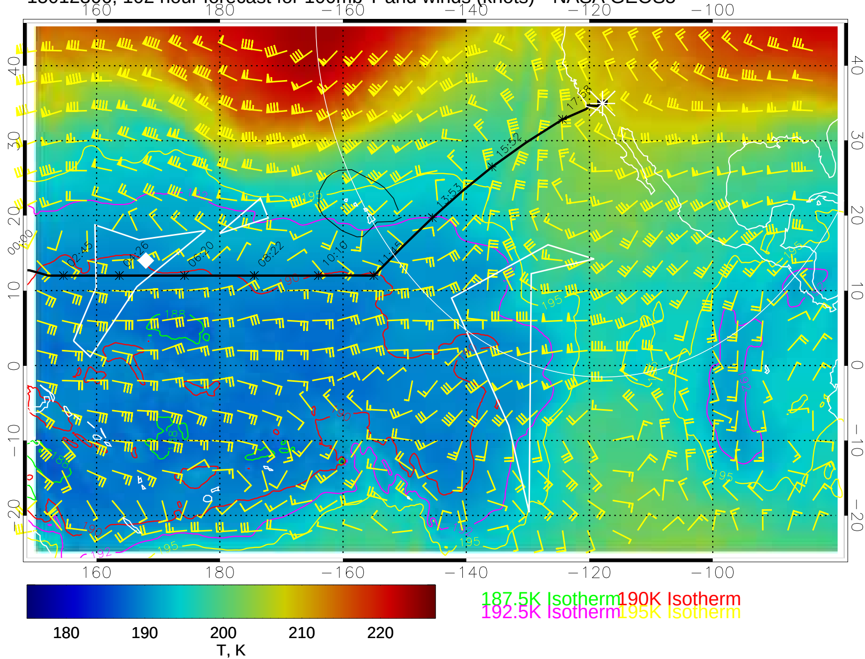
15012306, 102 hour forecast for 100mb T and winds (knots)-- NASA GEOS5
