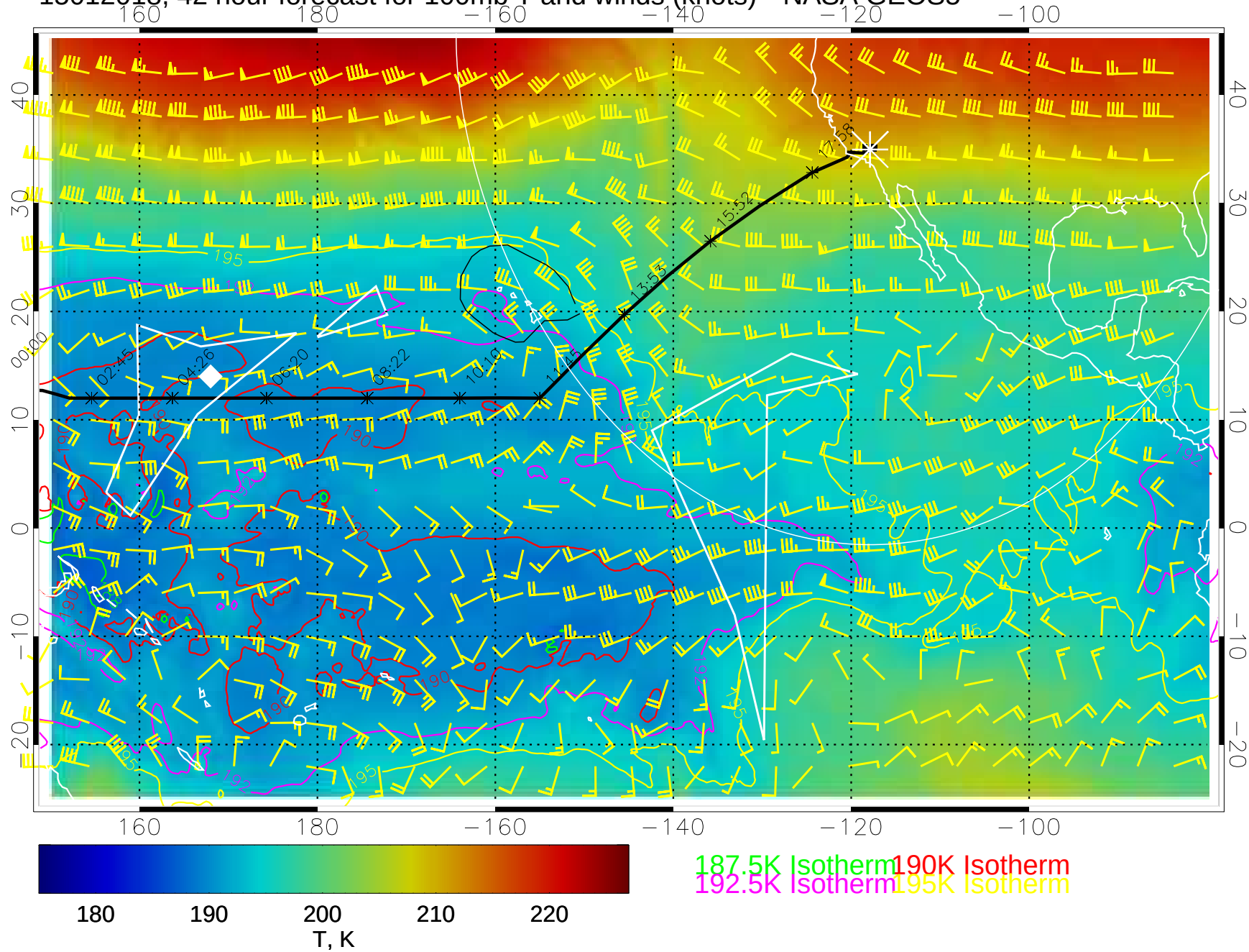
15012018, 42 hour forecast for 100mb T and winds (knots)-- NASA GEOS5
