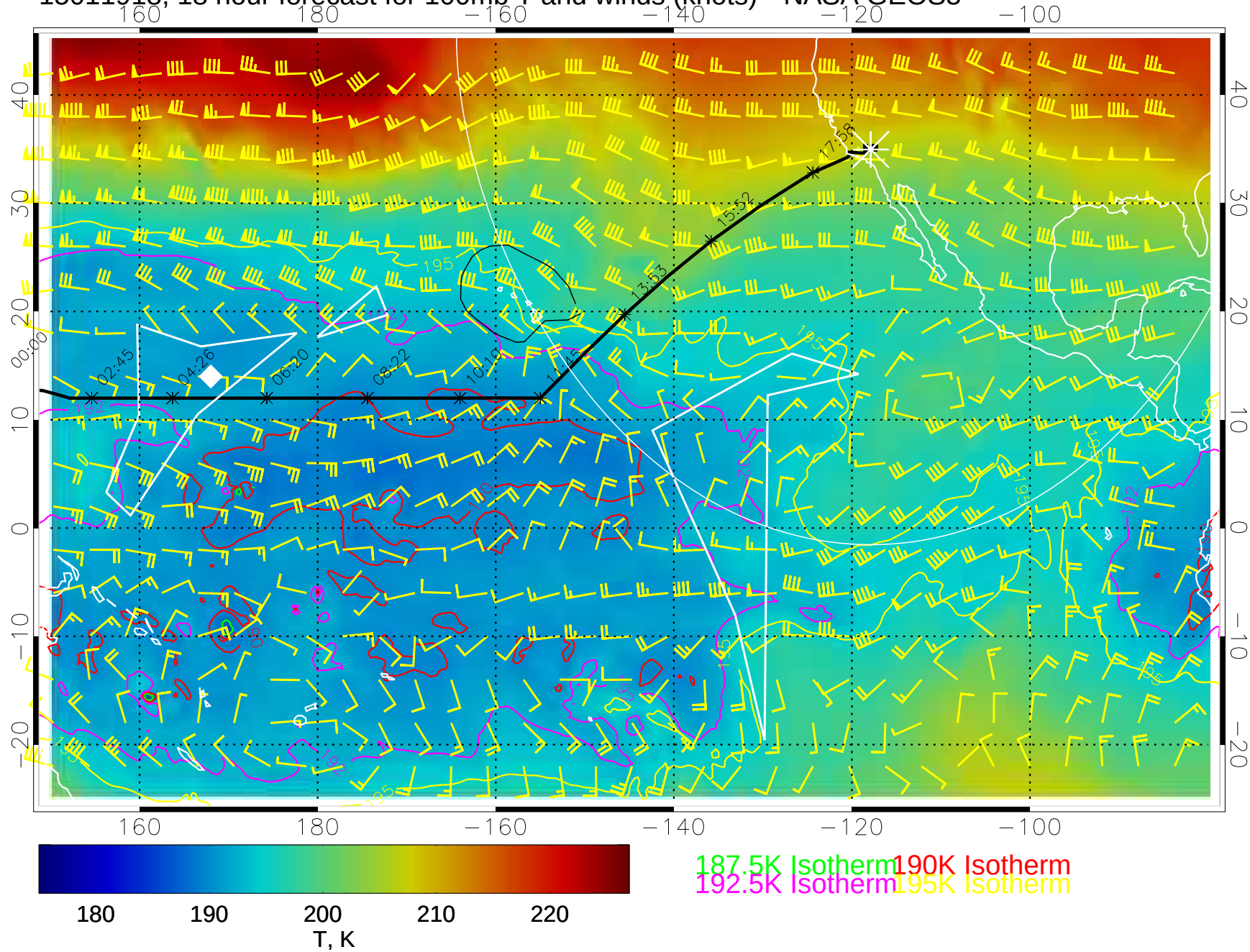
15011918, 18 hour forecast for 100mb T and winds (knots)-- NASA GEOS5
