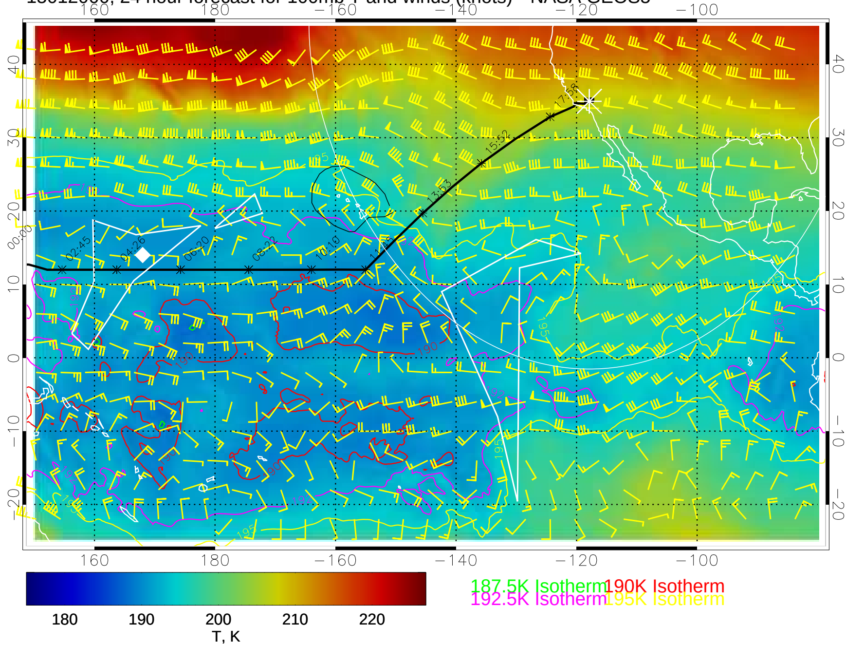
15012000, 24 hour forecast for 100mb T and winds (knots)-- NASA GEOS5
