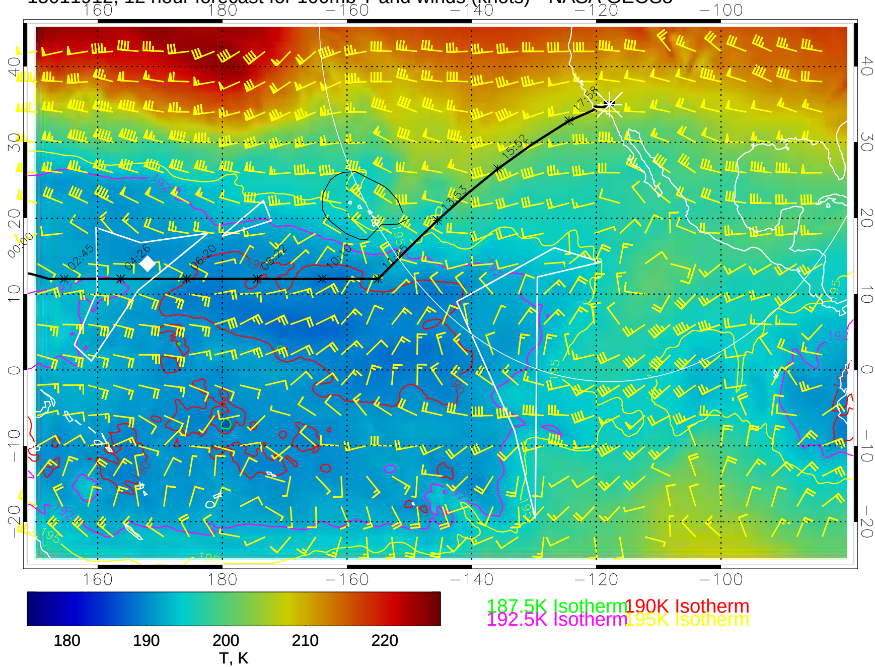
15011912, 12 hour forecast for 100mb T and winds (knots)-- NASA GEOS5
