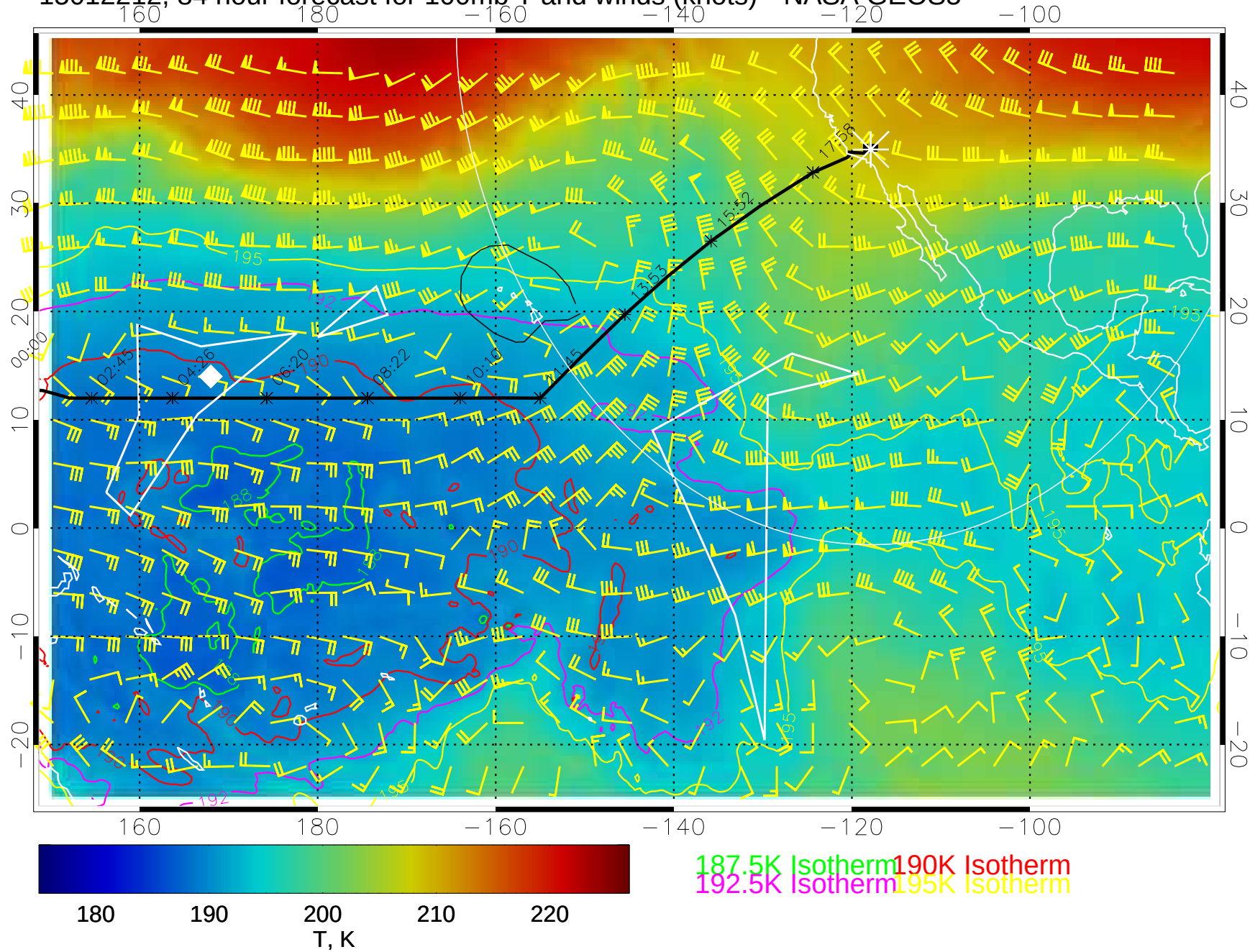
15012212, 84 hour forecast for 100mb T and winds (knots)-- NASA GEOS5
