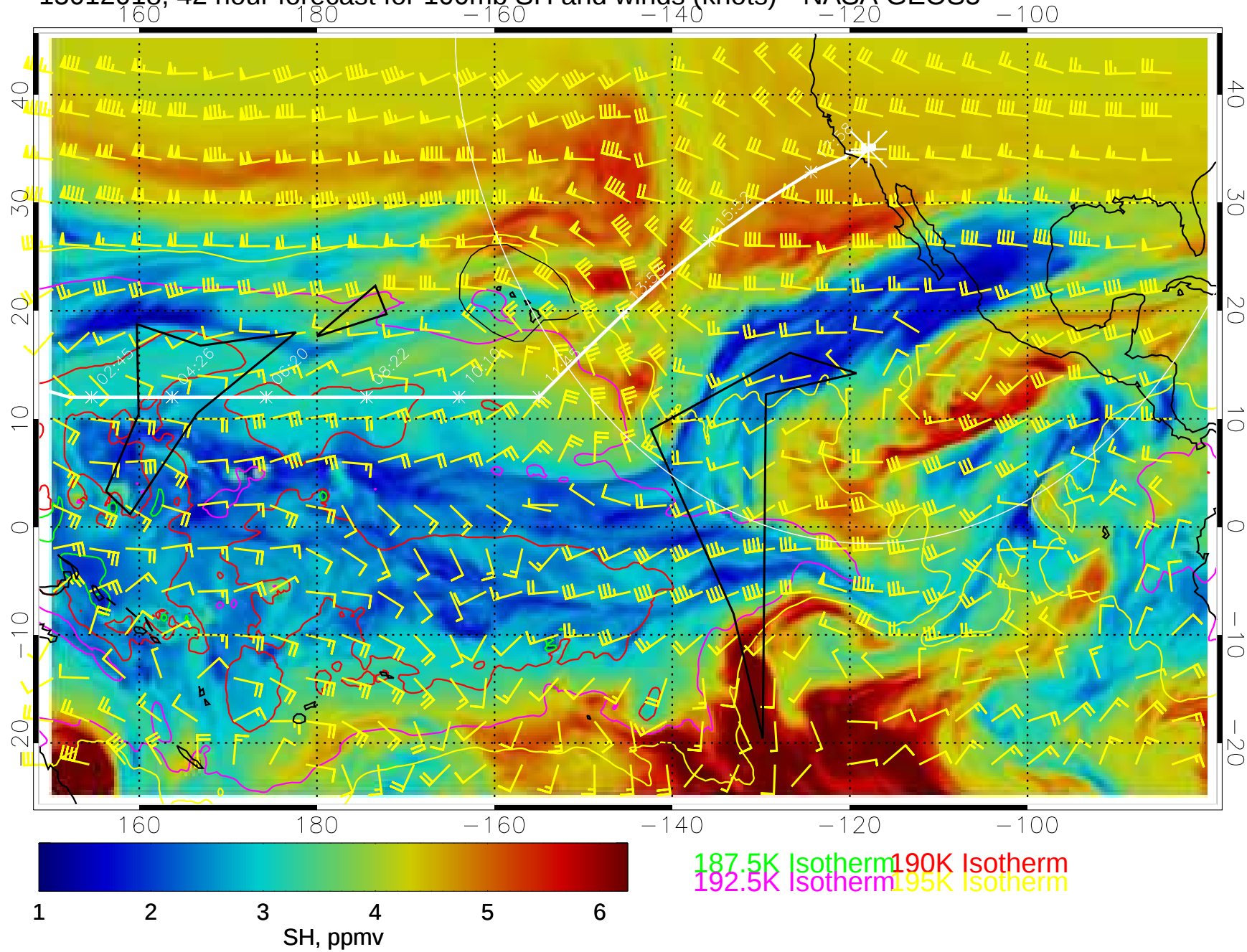
15012018, 42 hour forecast for 100mb SH and winds (knots)-- NASA GEOS5
