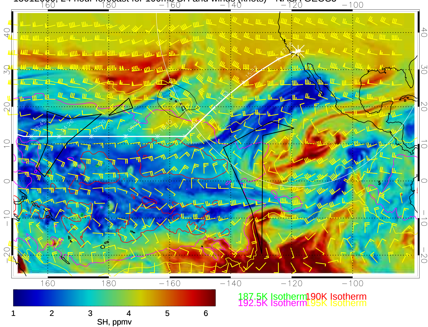
15012000, 24 hour forecast for 100mb SH and winds (knots)-- NASA GEOS5
