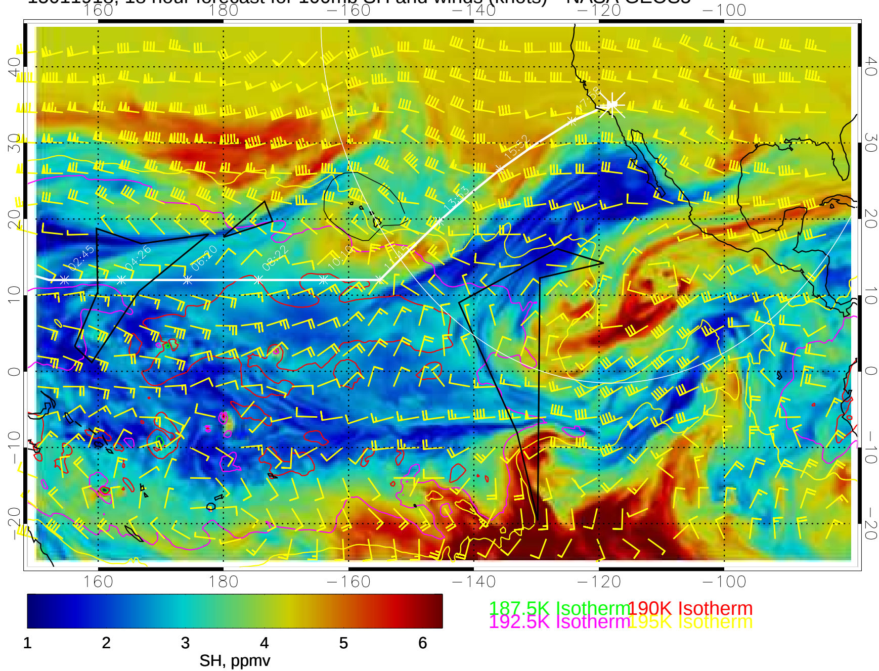
15011918, 18 hour forecast for 100mb SH and winds (knots)-- NASA GEOS5
