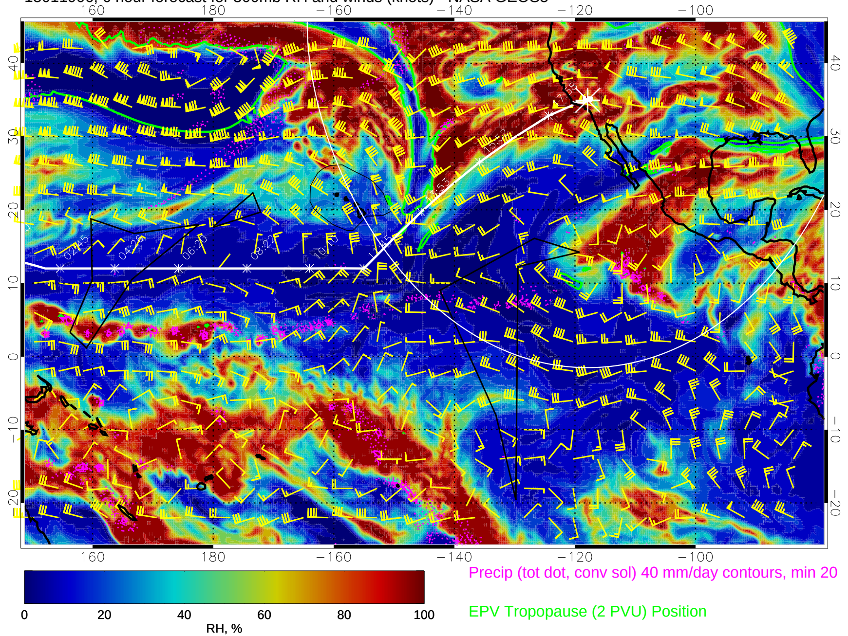
15011906, 6 hour forecast for 300mb RH and winds (knots) - NASA GEOS5
