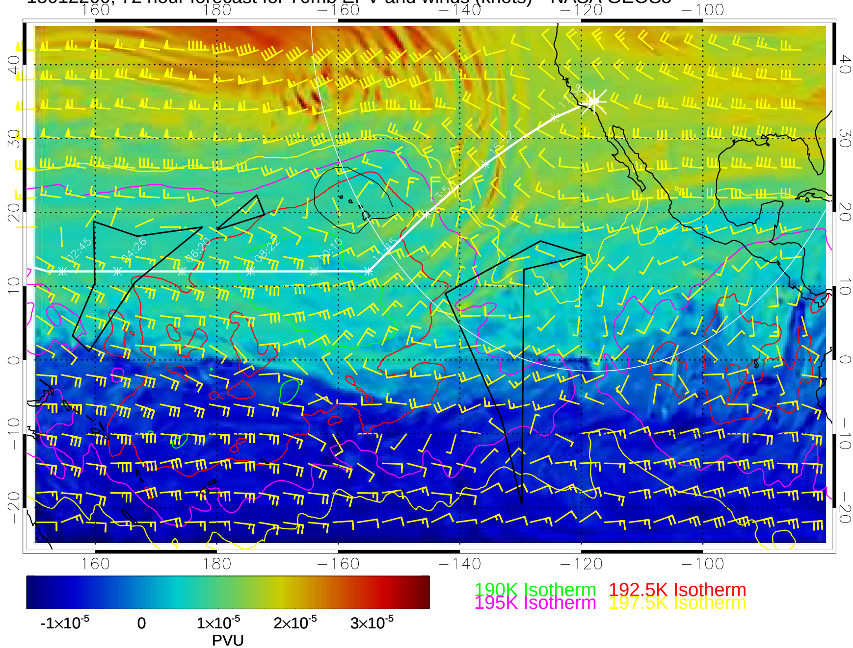
15012200, 72 hour forecast for 70mb EPV and winds (knots)-- NASA GEOS5
