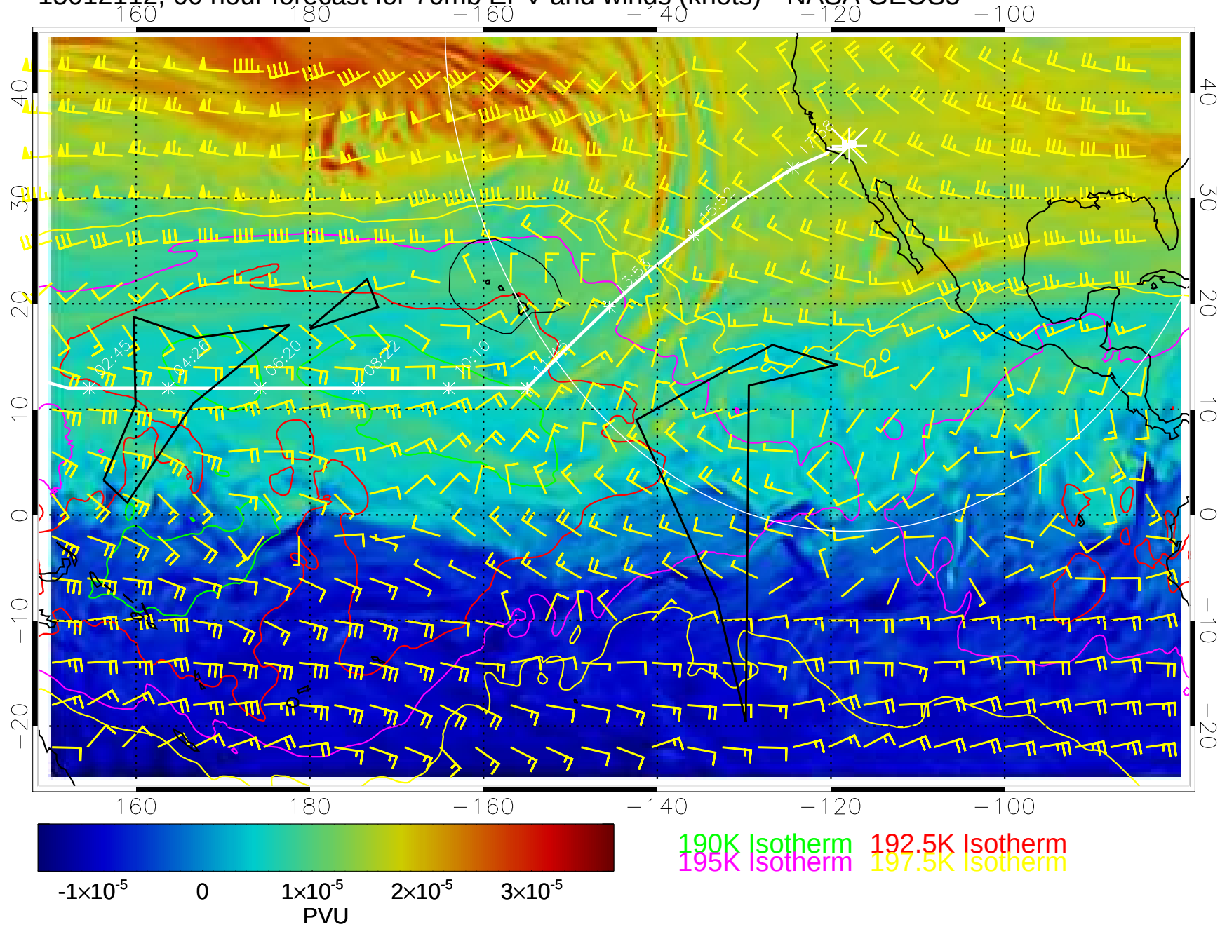
15012112, 60 hour forecast for 70mb EPV and winds (knots)-- NASA GEOS5
