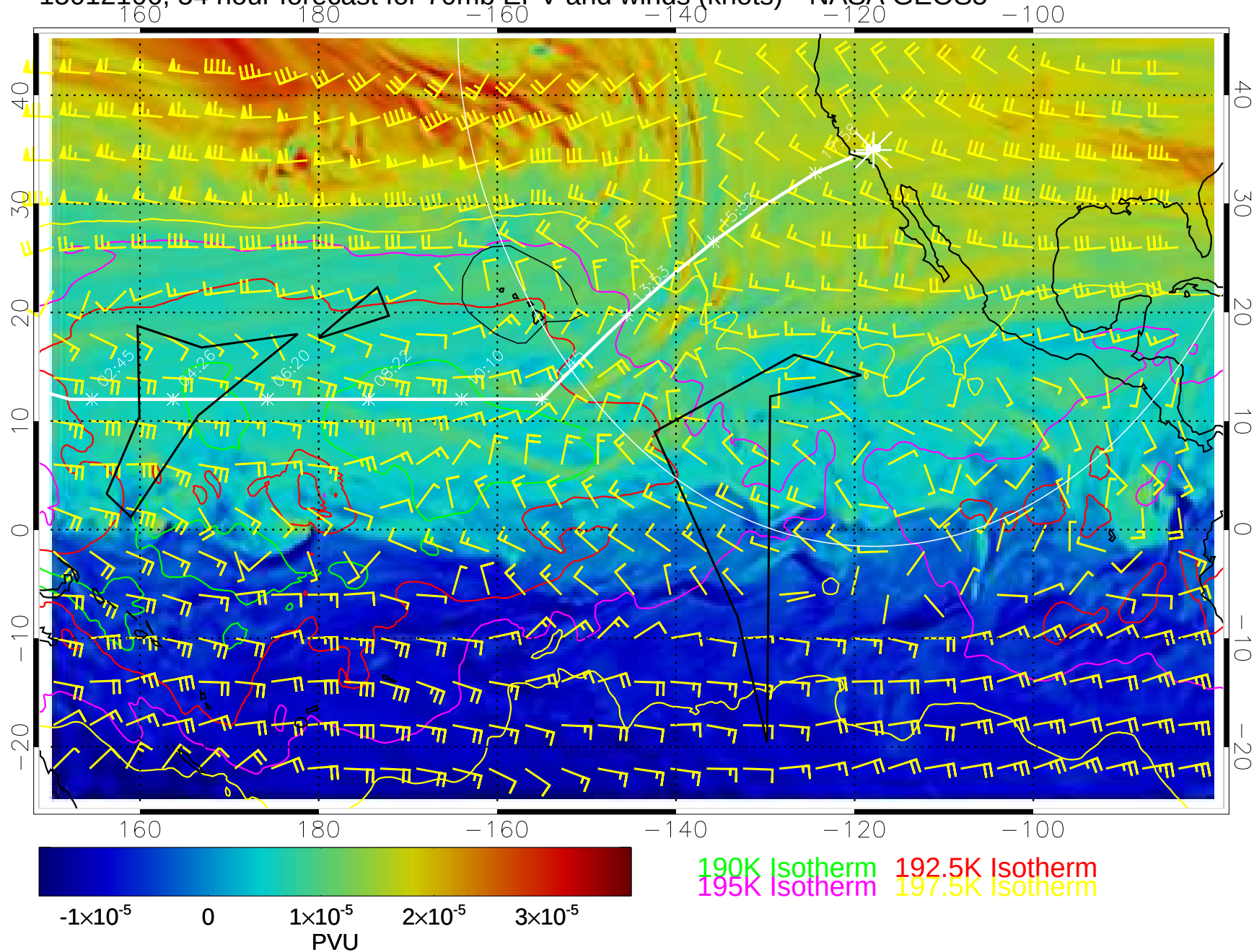
15012106, 54 hour forecast for 70mb EPV and winds (knots)-- NASA GEOS5
