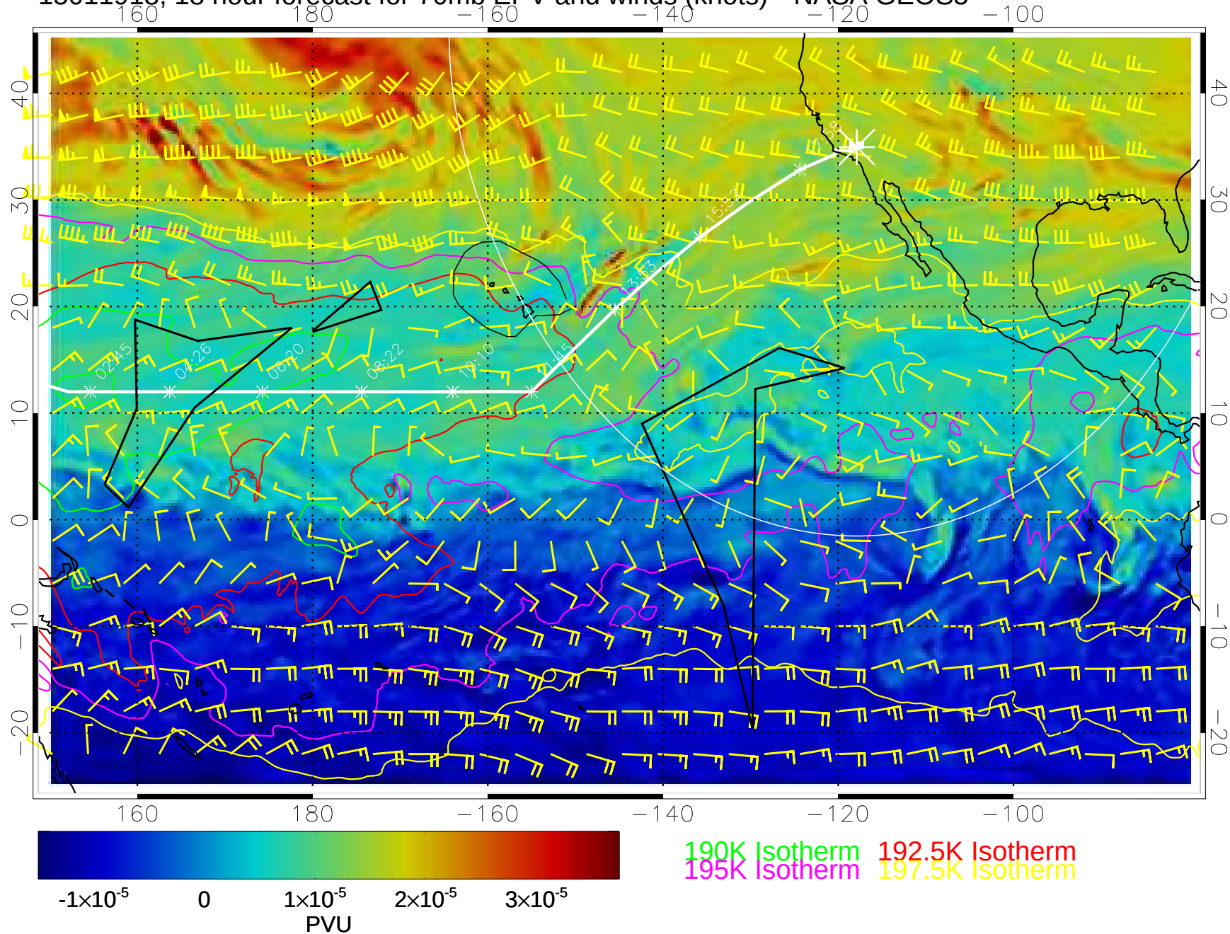
15011918, 18 hour forecast for 70mb EPV and winds (knots)-- NASA GEOS5
