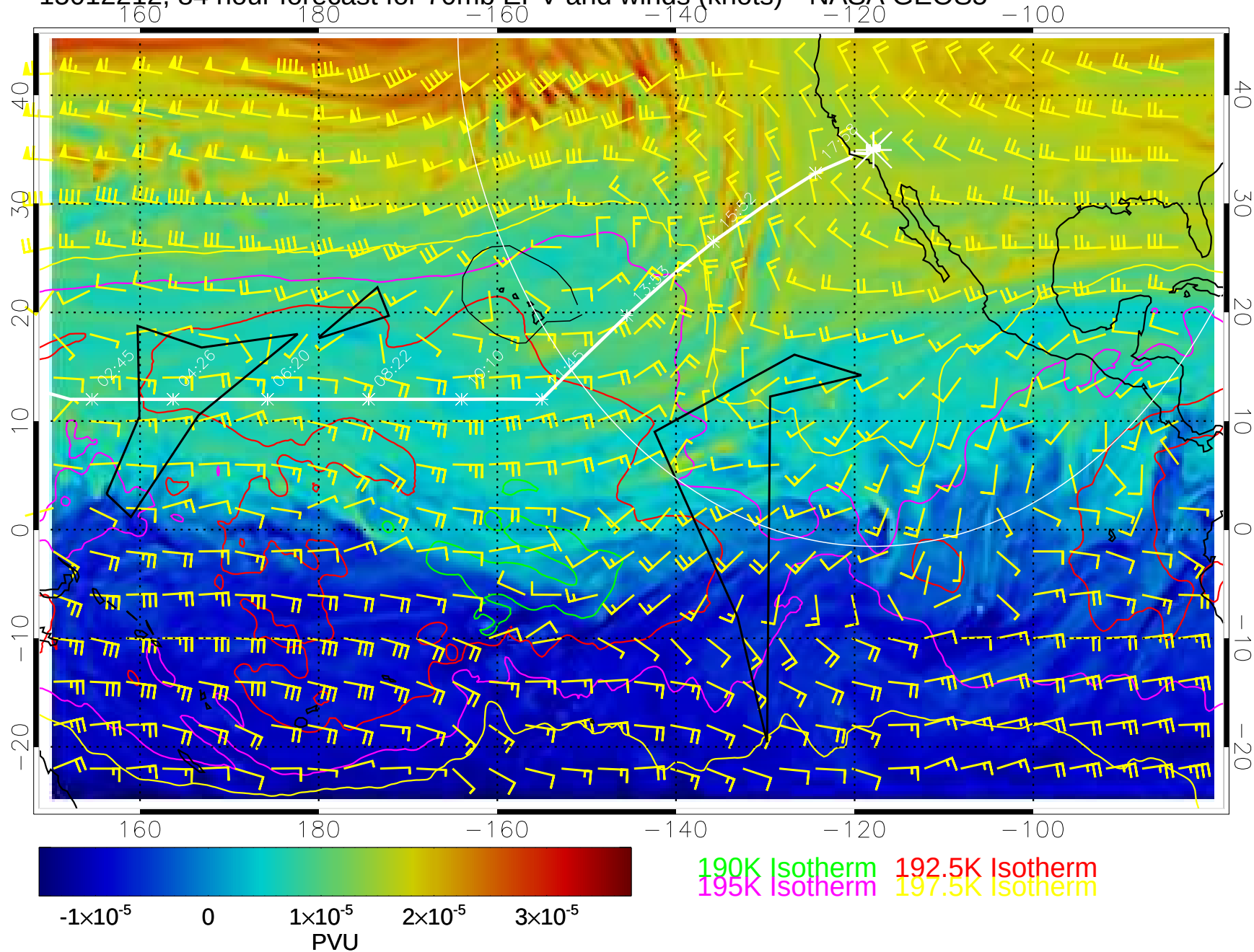
15012212, 84 hour forecast for 70mb EPV and winds (knots)-- NASA GEOS5
