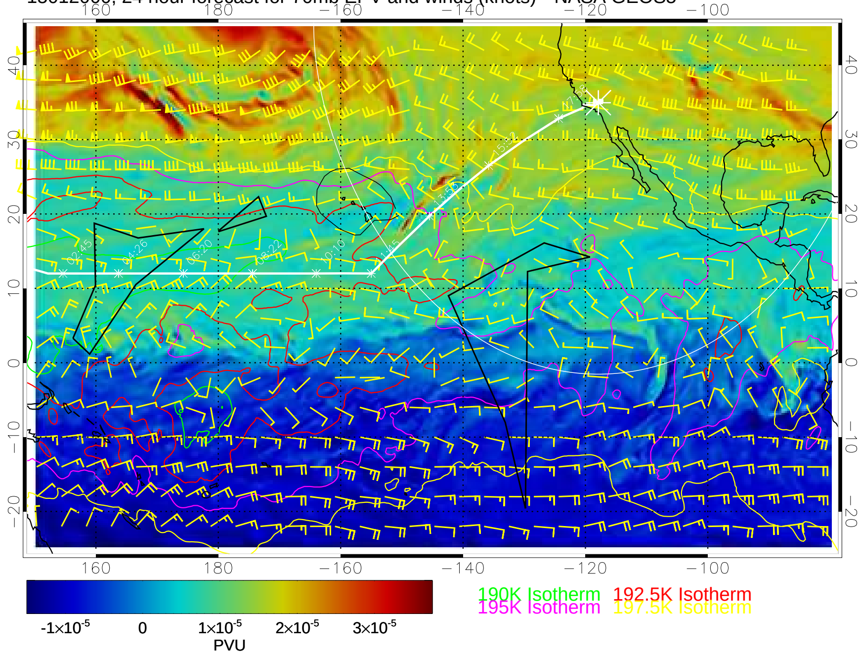
15012000, 24 hour forecast for 70mb EPV and winds (knots)-- NASA GEOS5
