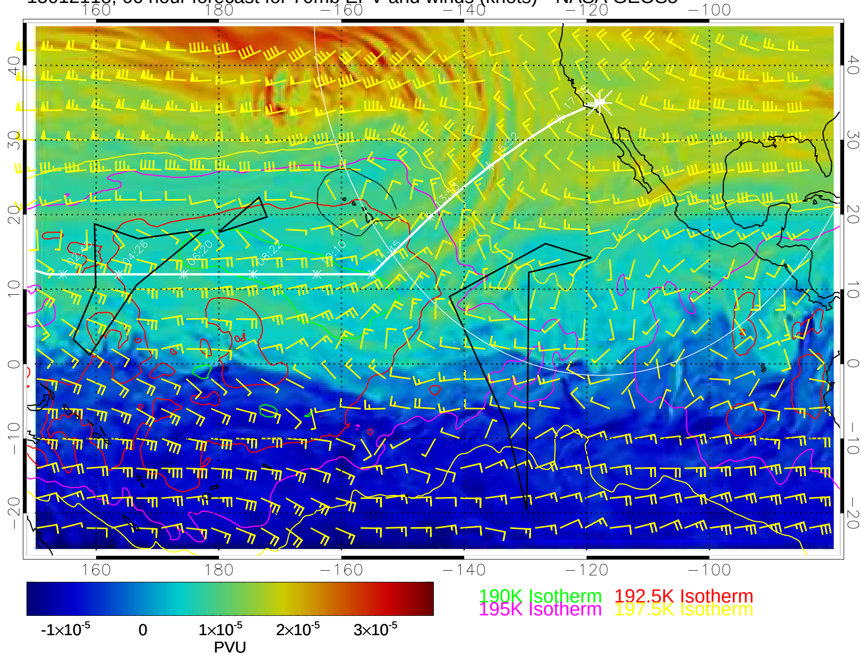
15012118, 66 hour forecast for 70mb EPV and winds (knots)-- NASA GEOS5
