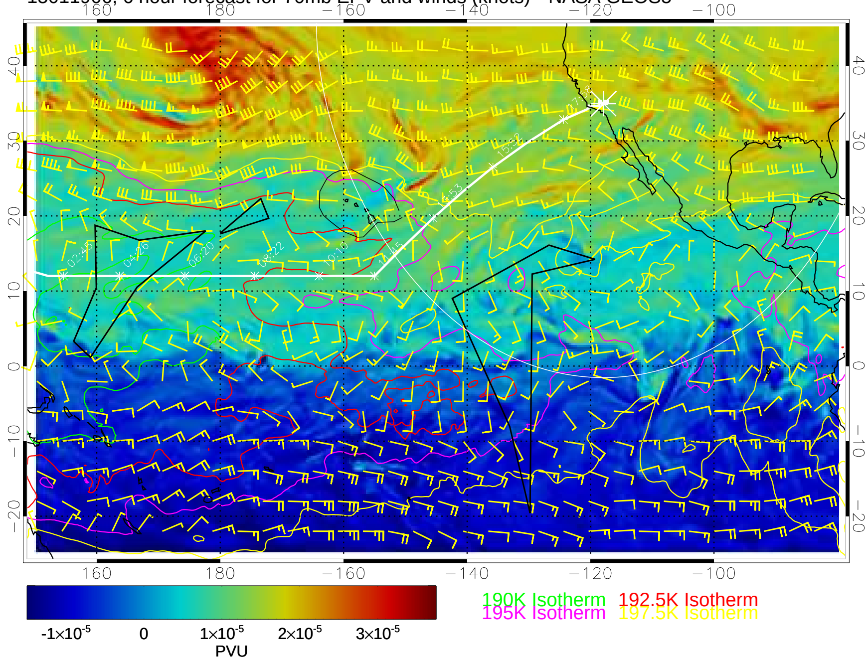
15011906, 6 hour forecast for 70mb EPV and winds (knots)-- NASA GEOS5
