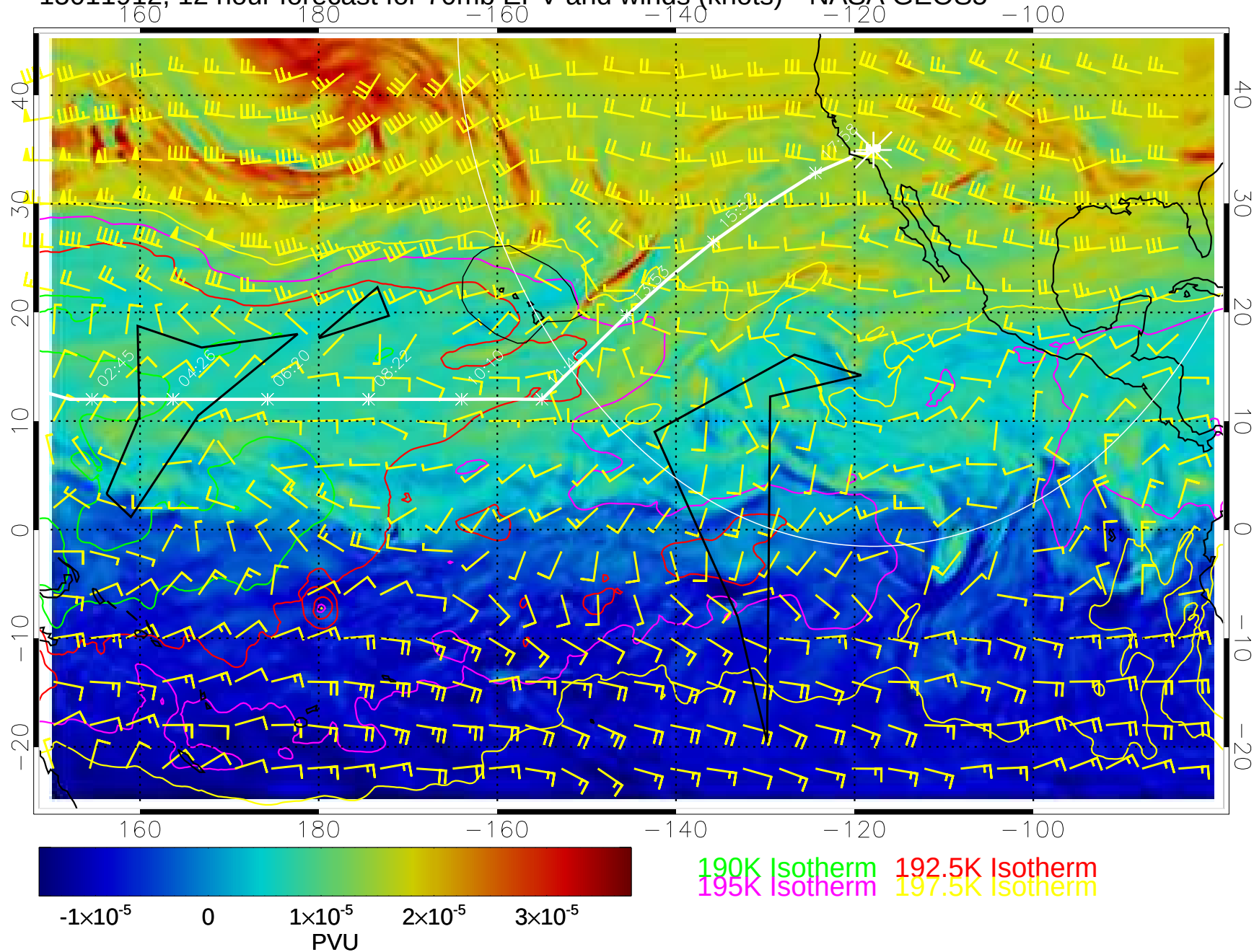
15011912, 12 hour forecast for 70mb EPV and winds (knots)-- NASA GEOS5
