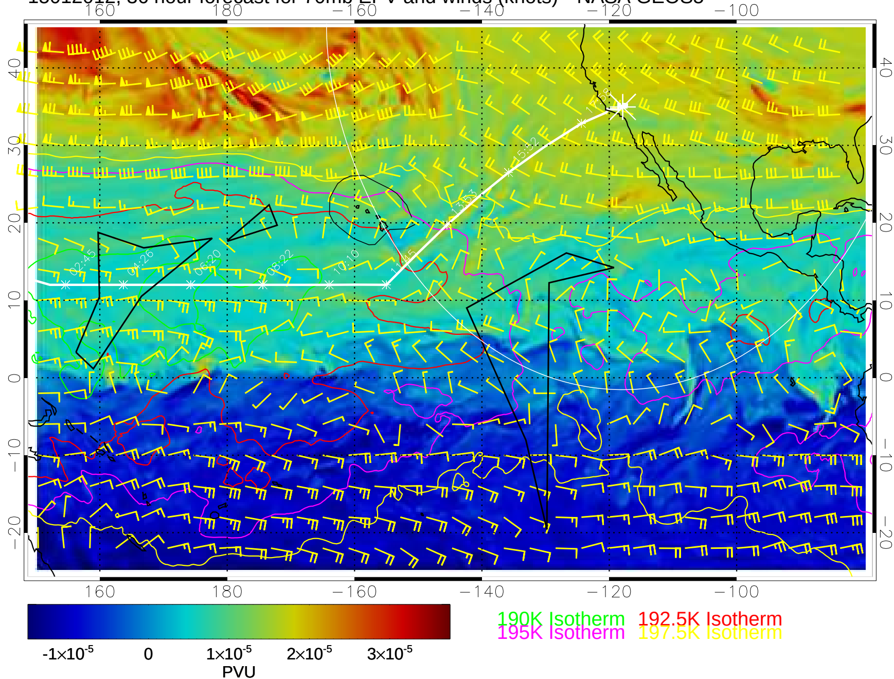
15012012, 36 hour forecast for 70mb EPV and winds (knots)-- NASA GEOS5
