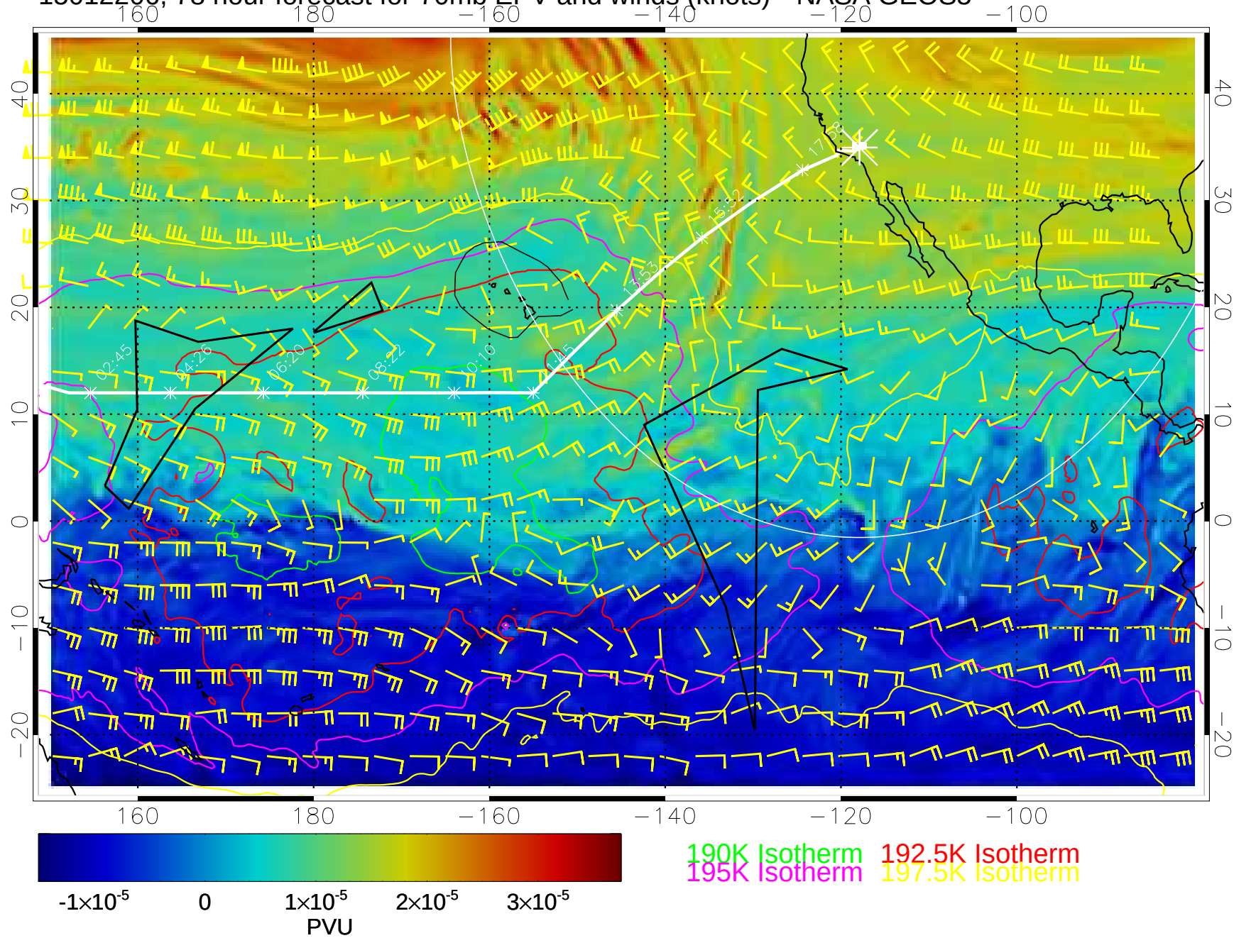
15012206, 78 hour forecast for 70mb EPV and winds (knots)-- NASA GEOS5
