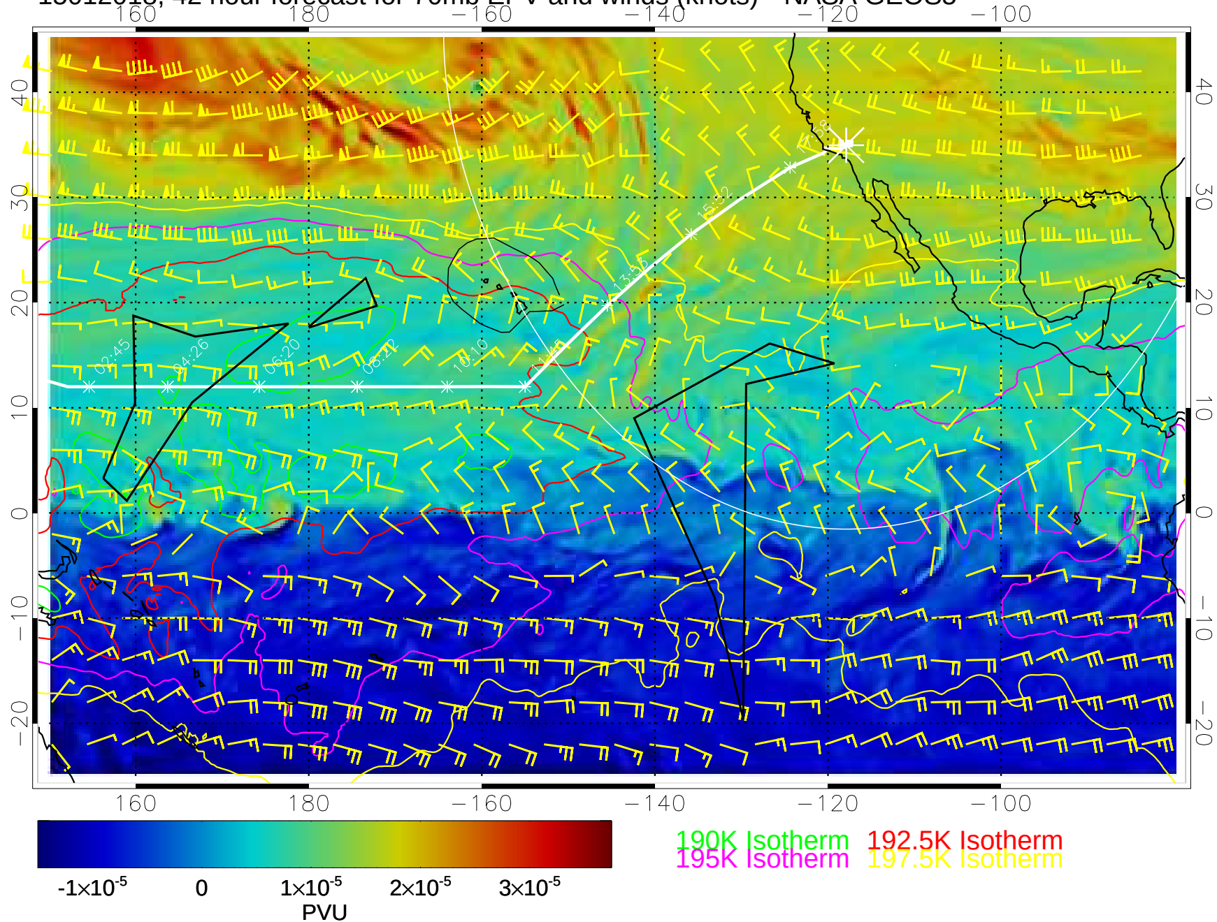
15012018, 42 hour forecast for 70mb EPV and winds (knots)-- NASA GEOS5
