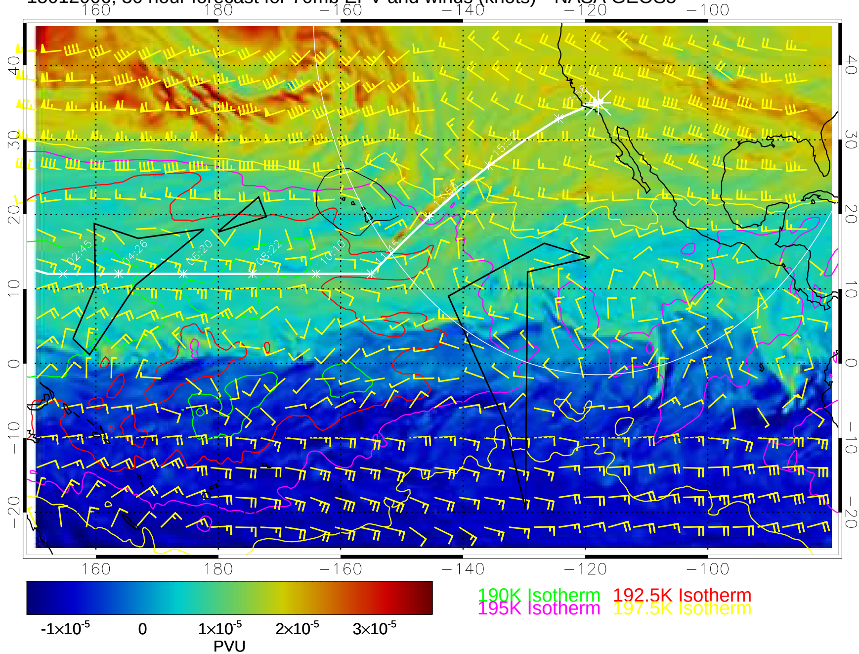
15012006, 30 hour forecast for 70mb EPV and winds (knots)-- NASA GEOS5
