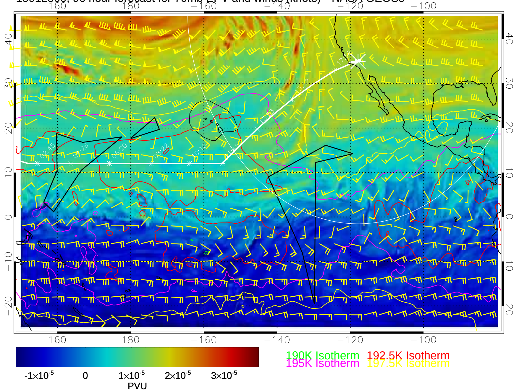
15012300, 96 hour forecast for 70mb EPV and winds (knots)-- NASA GEOS5
