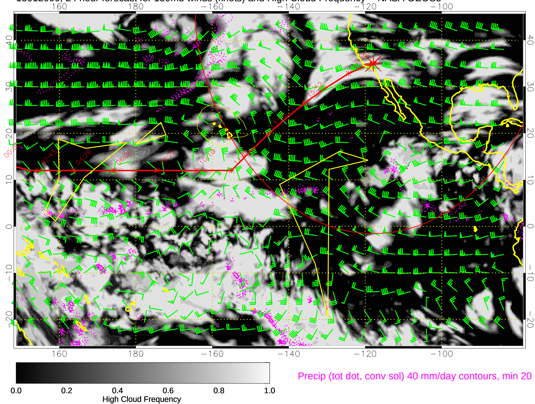
15012000, 24 hour forecast for 150mb winds (knots) and High Cloud Frequency -- NASA GEOS5
