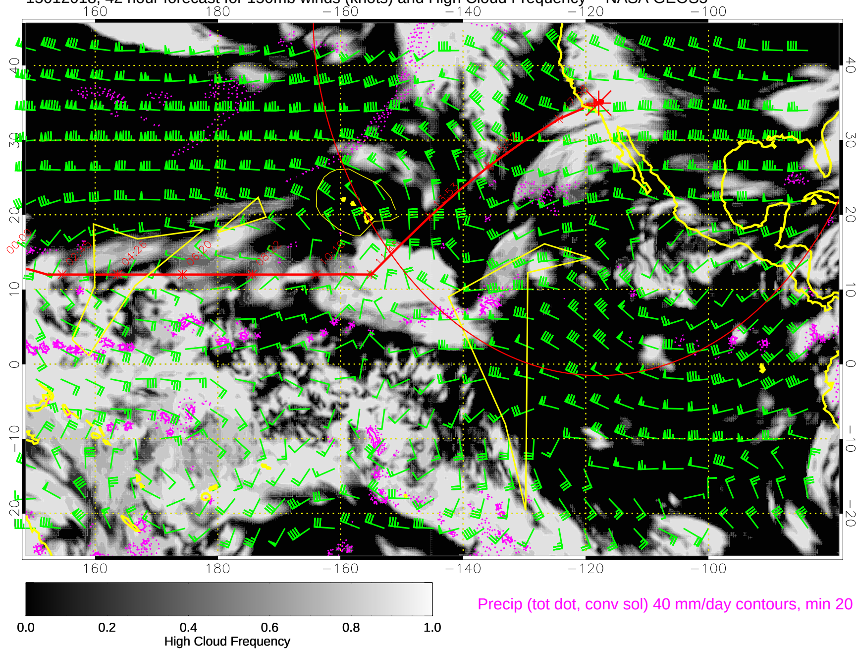
15012018, 42 hour forecast for 150mb winds (knots) and High Cloud Frequency -- NASA GEOS5
