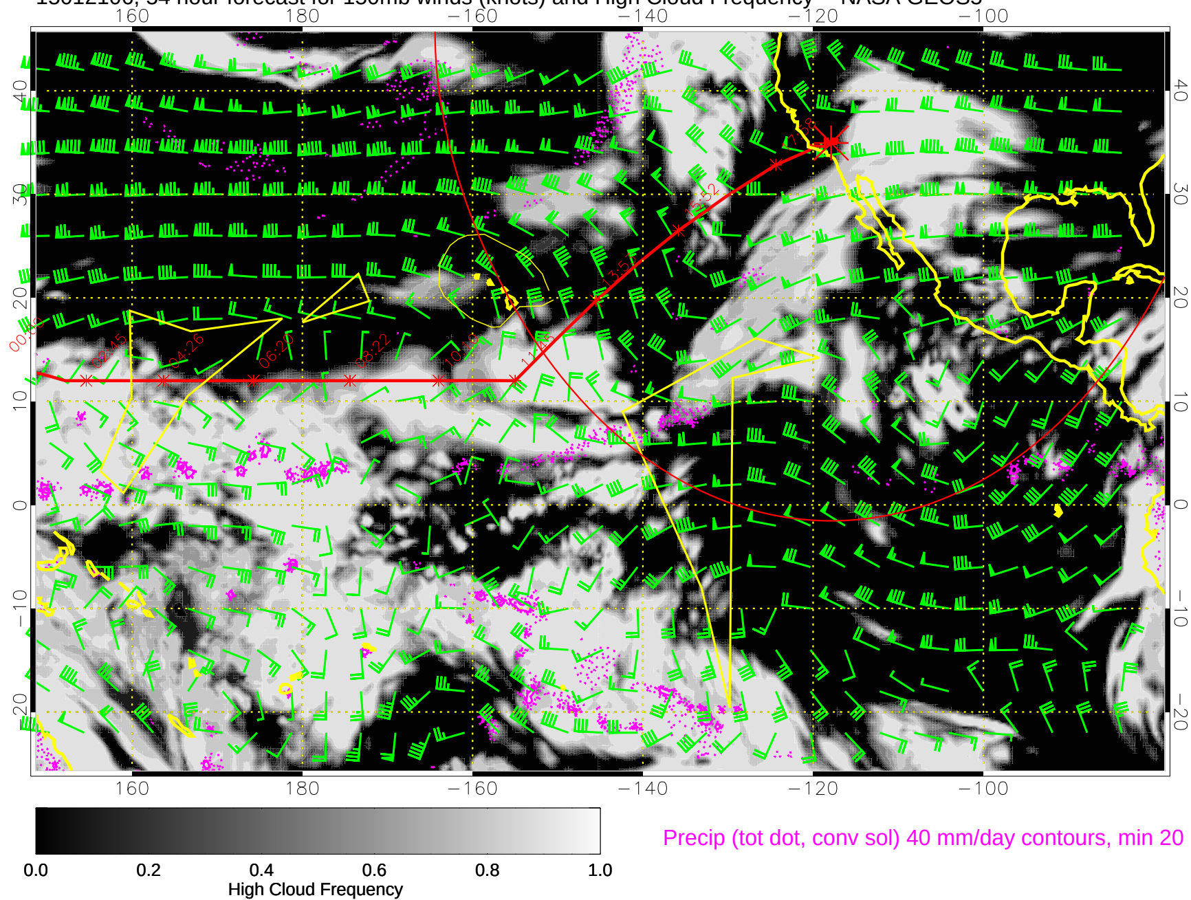
15012106, 54 hour forecast for 150mb winds (knots) and High Cloud Frequency -- NASA GEOS5
