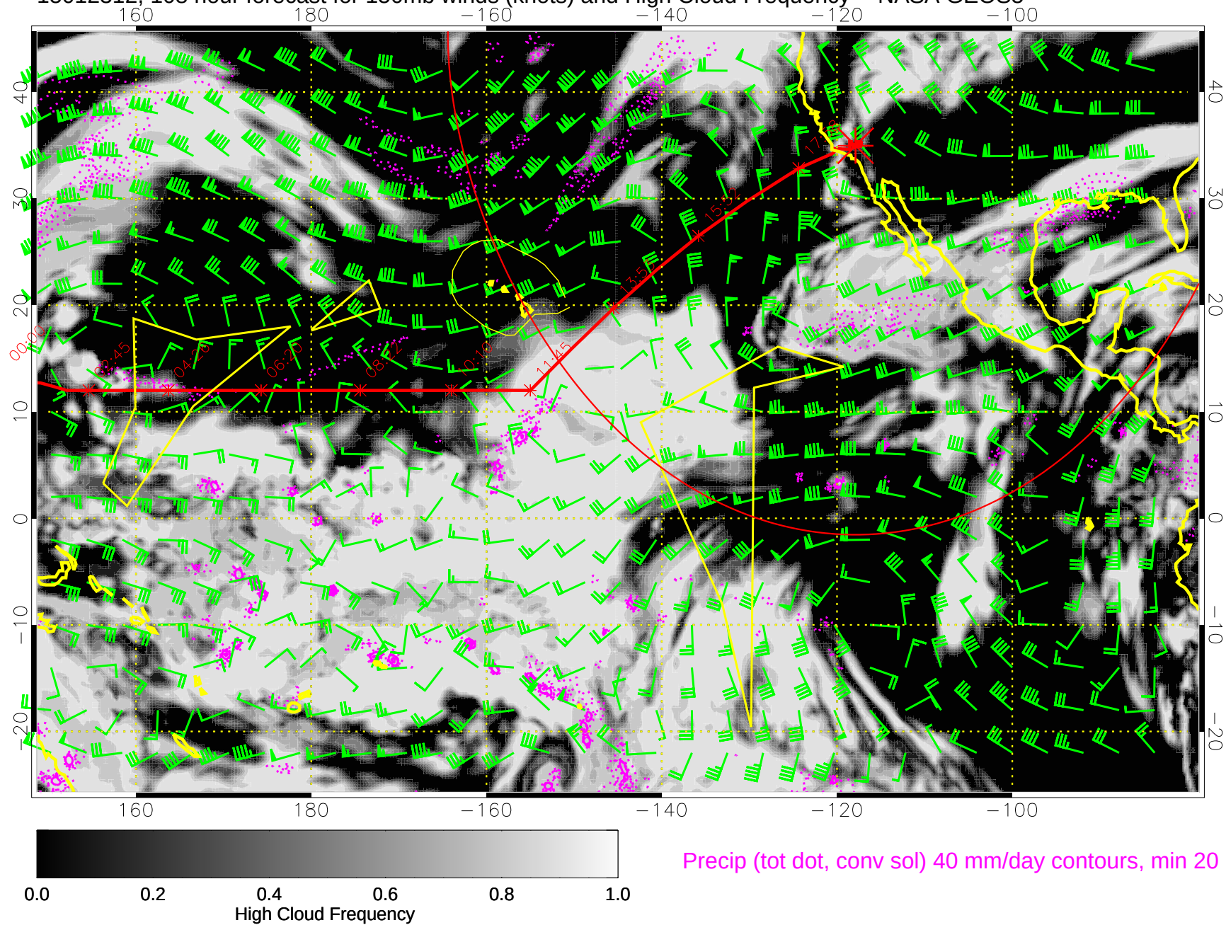
15012312, 108 hour forecast for 150mb winds (knots) and High Cloud Frequency -- NASA GEOS5
