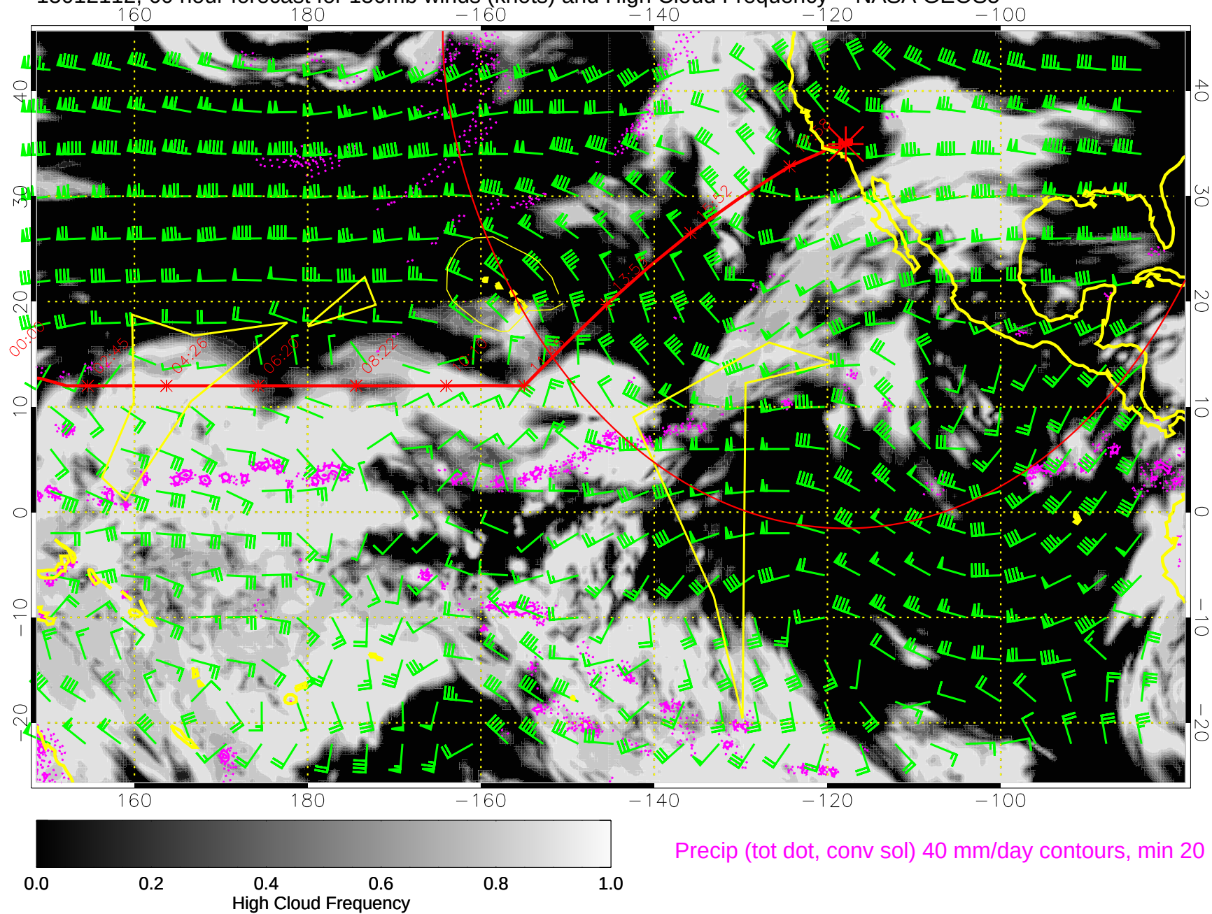
15012112, 60 hour forecast for 150mb winds (knots) and High Cloud Frequency -- NASA GEOS5
