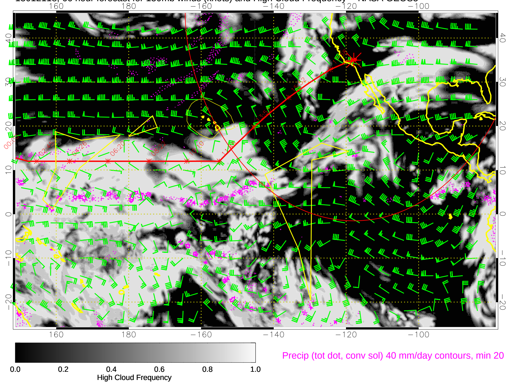
15012118, 66 hour forecast for 150mb winds (knots) and High Cloud Frequency -- NASA GEOS5
