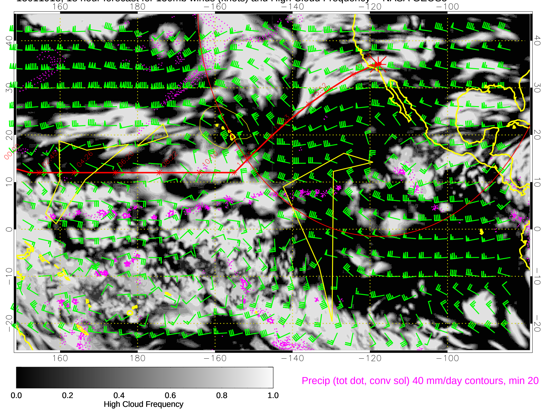
15011918, 18 hour forecast for 150mb winds (knots) and High Cloud Frequency -- NASA GEOS5
