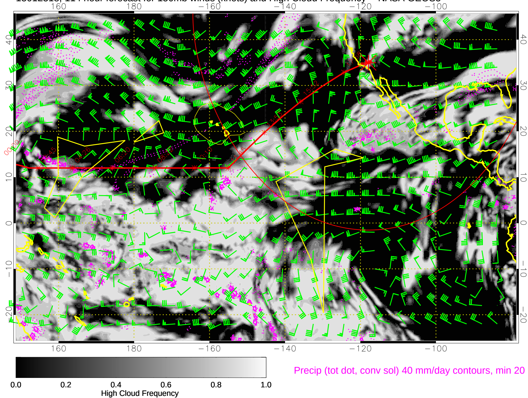
15012318, 114 hour forecast for 150mb winds (knots) and High Cloud Frequency -- NASA GEOS5
