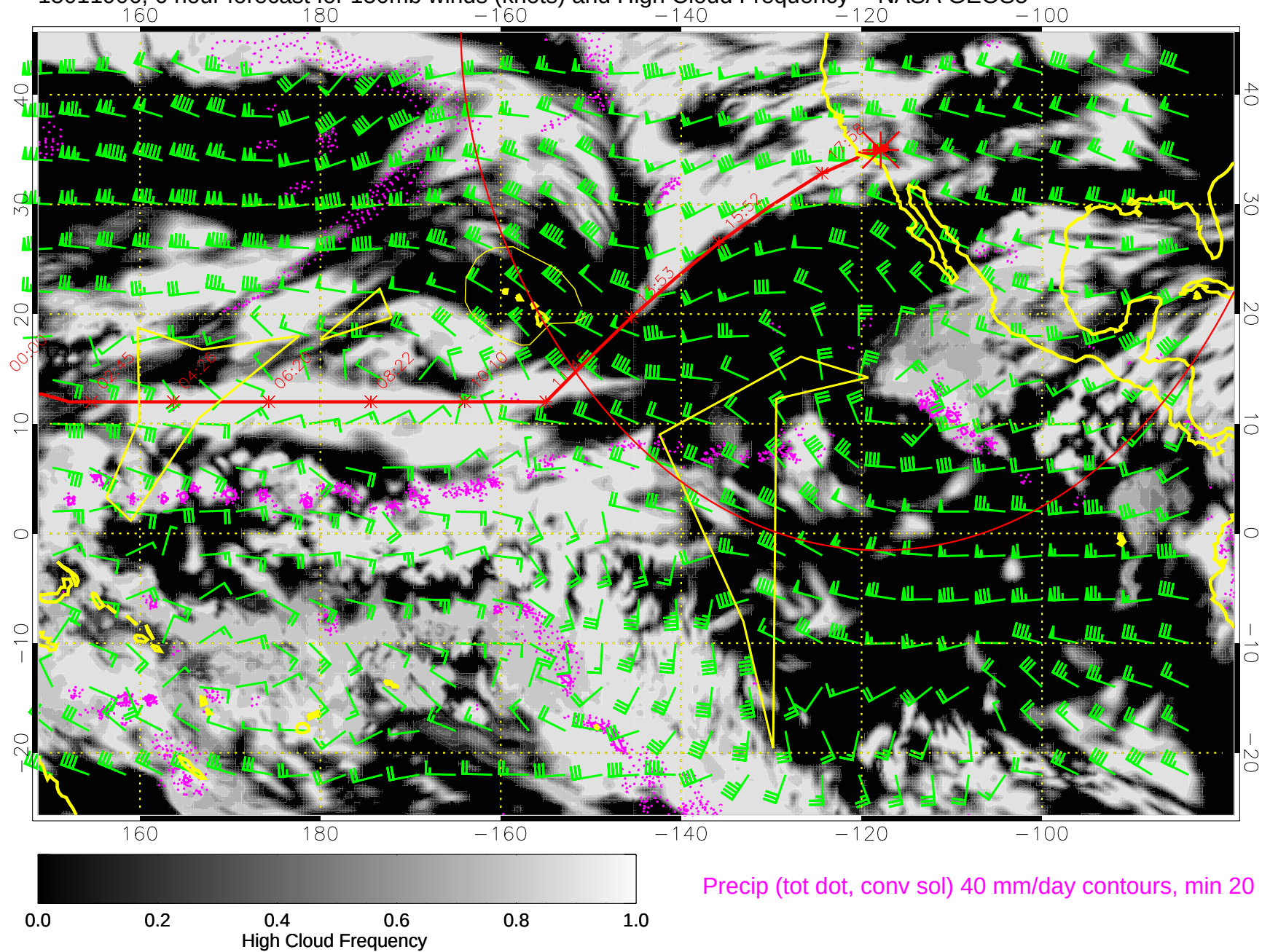
15011906, 6 hour forecast for 150mb winds (knots) and High Cloud Frequency -- NASA GEOS5
