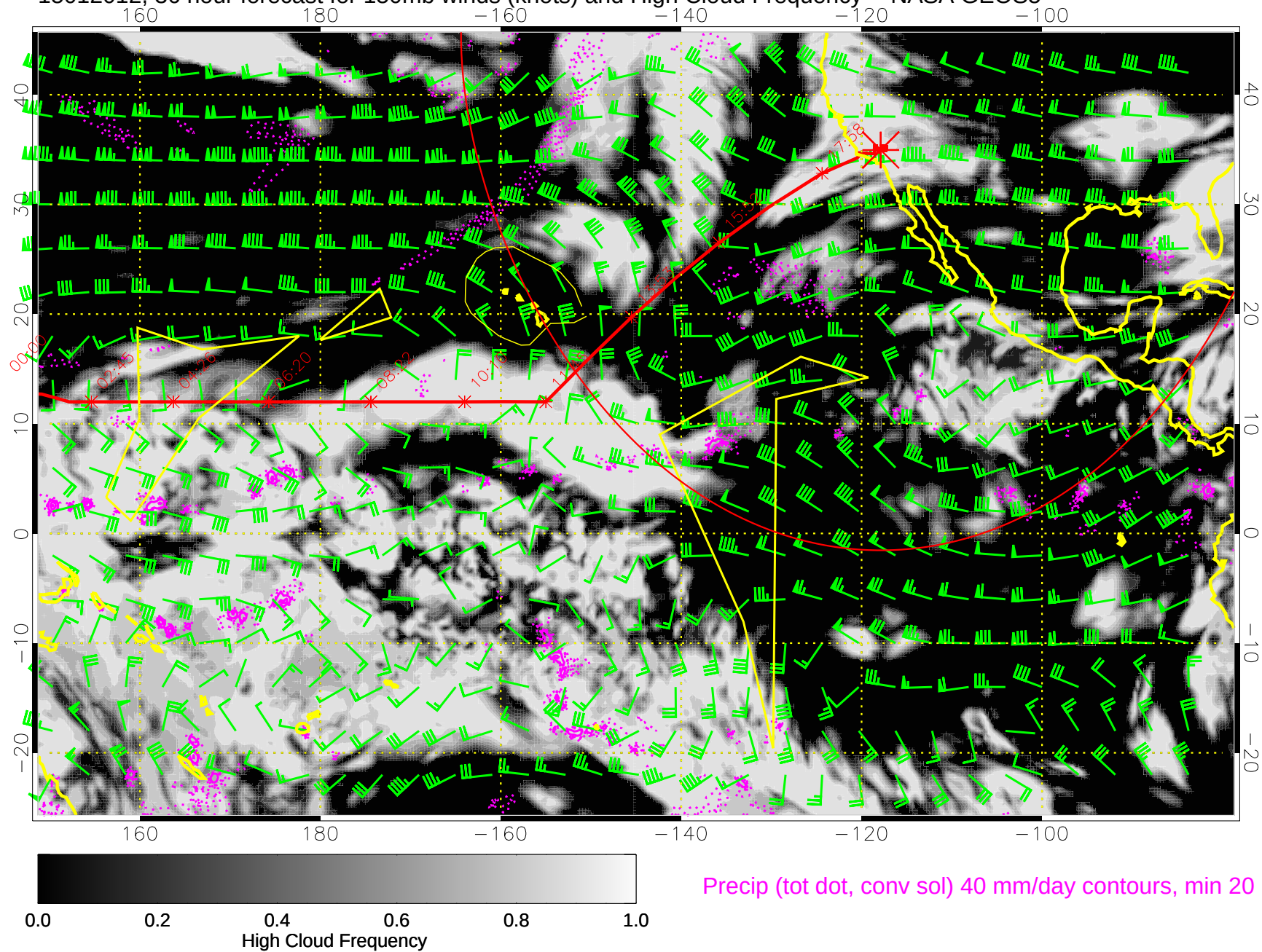
15012012, 36 hour forecast for 150mb winds (knots) and High Cloud Frequency -- NASA GEOS5
