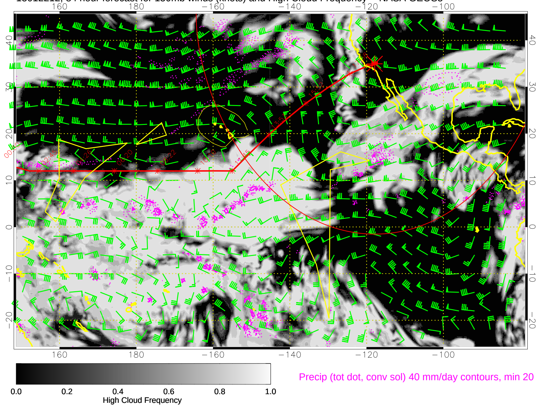
15012212, 84 hour forecast for 150mb winds (knots) and High Cloud Frequency -- NASA GEOS5
