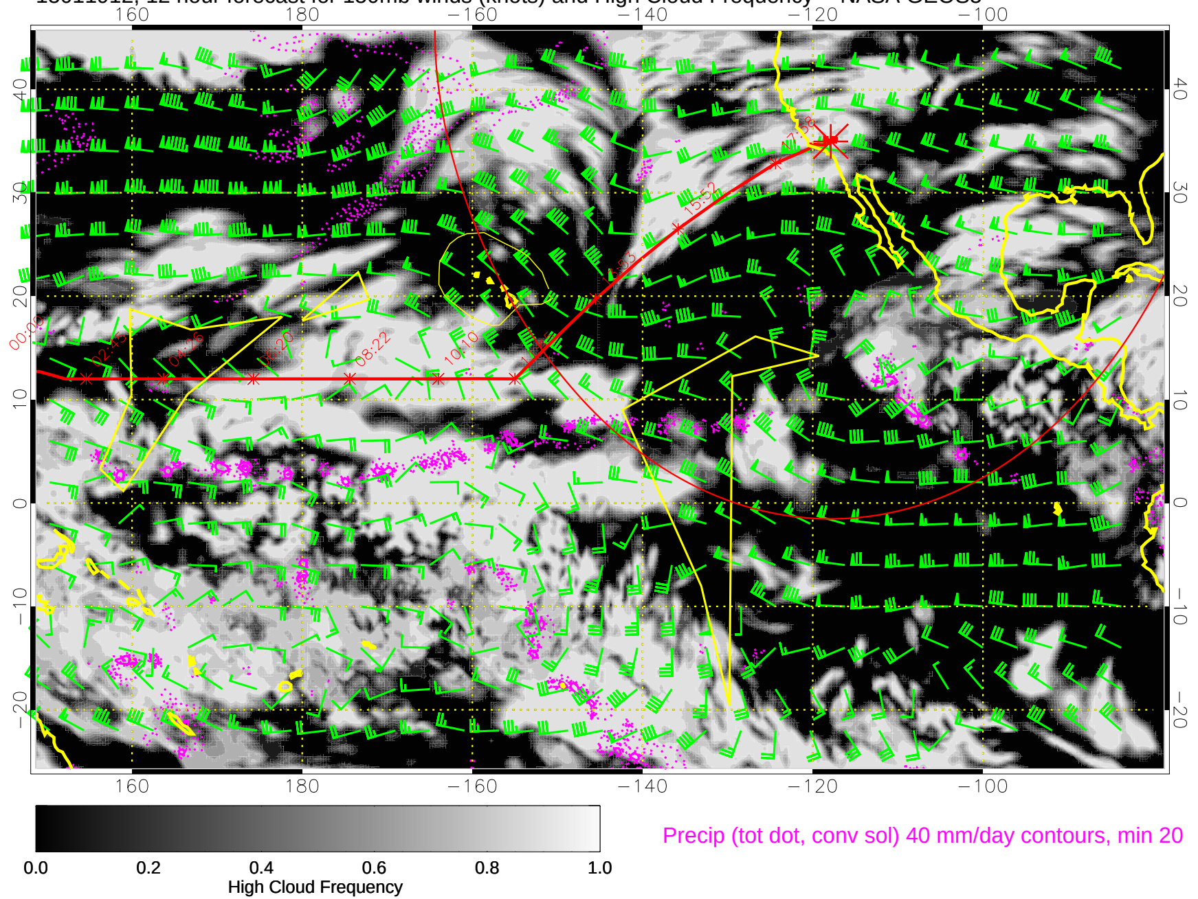
15011912, 12 hour forecast for 150mb winds (knots) and High Cloud Frequency -- NASA GEOS5
