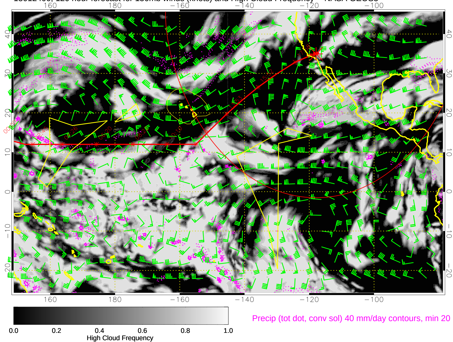
15012400, 120 hour forecast for 150mb winds (knots) and High Cloud Frequency -- NASA GEOS5
