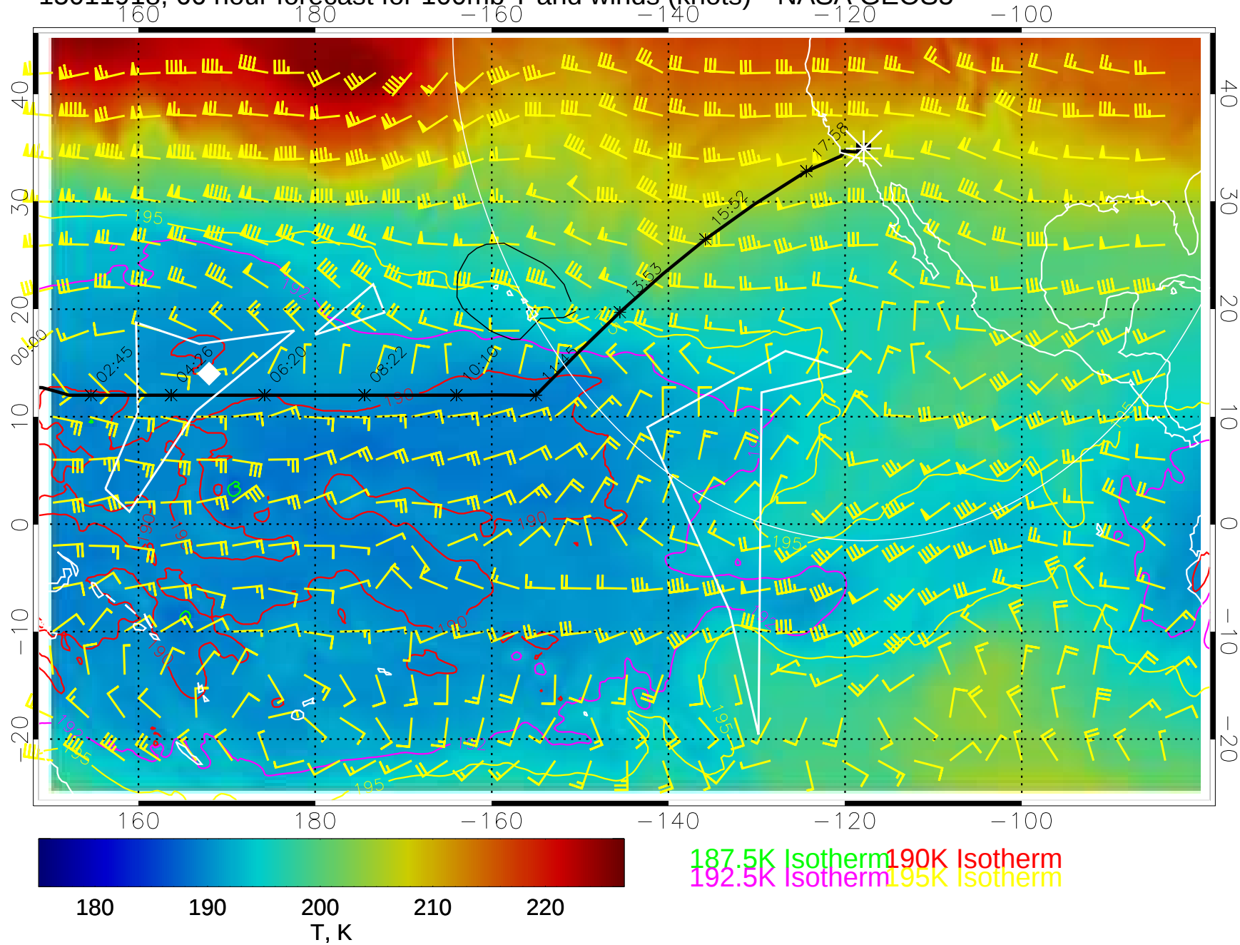
15011918, 66 hour forecast for 100mb T and winds (knots)-- NASA GEOS5
