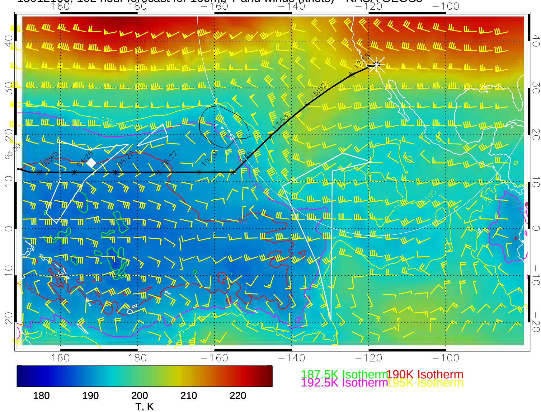
15012106, 102 hour forecast for 100mb T and winds (knots)-- NASA GEOS5
