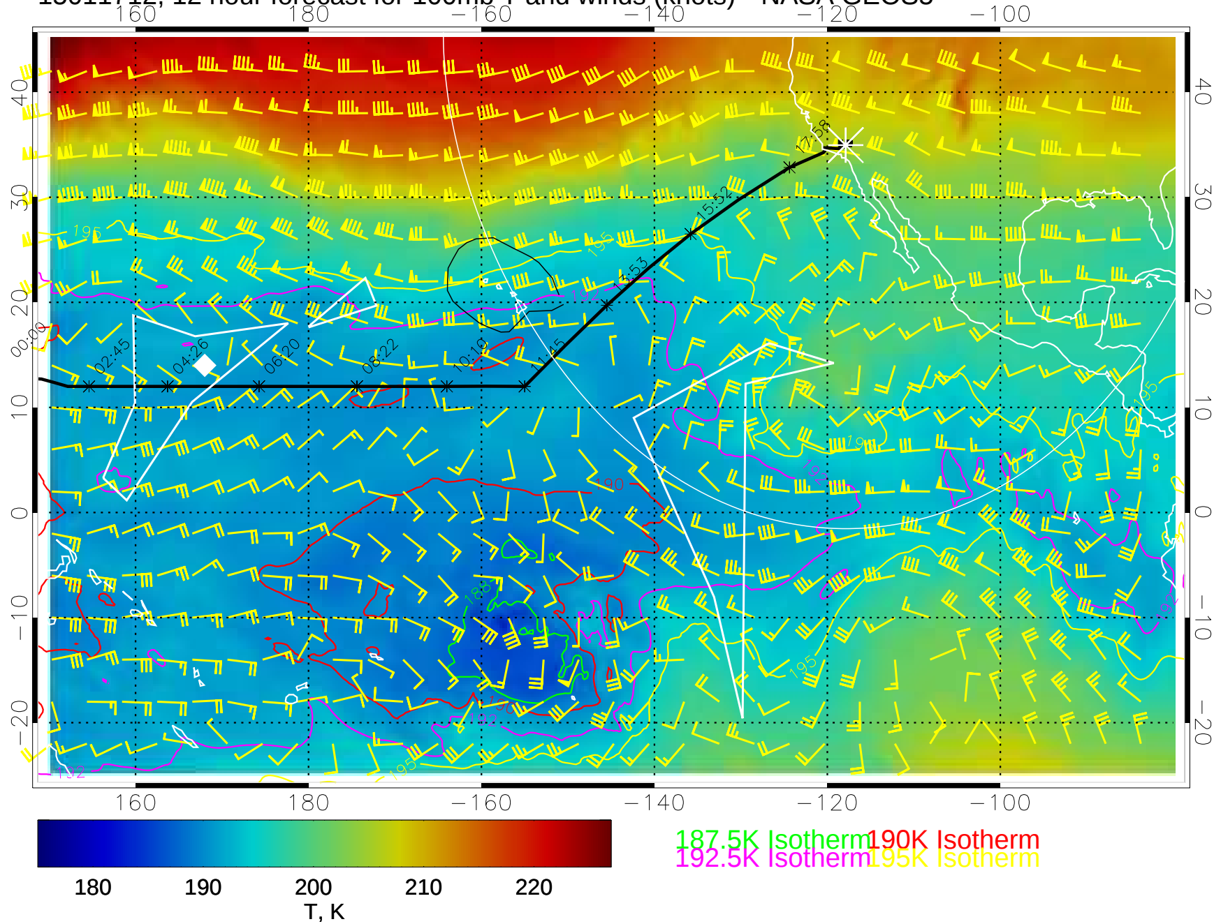
15011712, 12 hour forecast for 100mb T and winds (knots)-- NASA GEOS5
