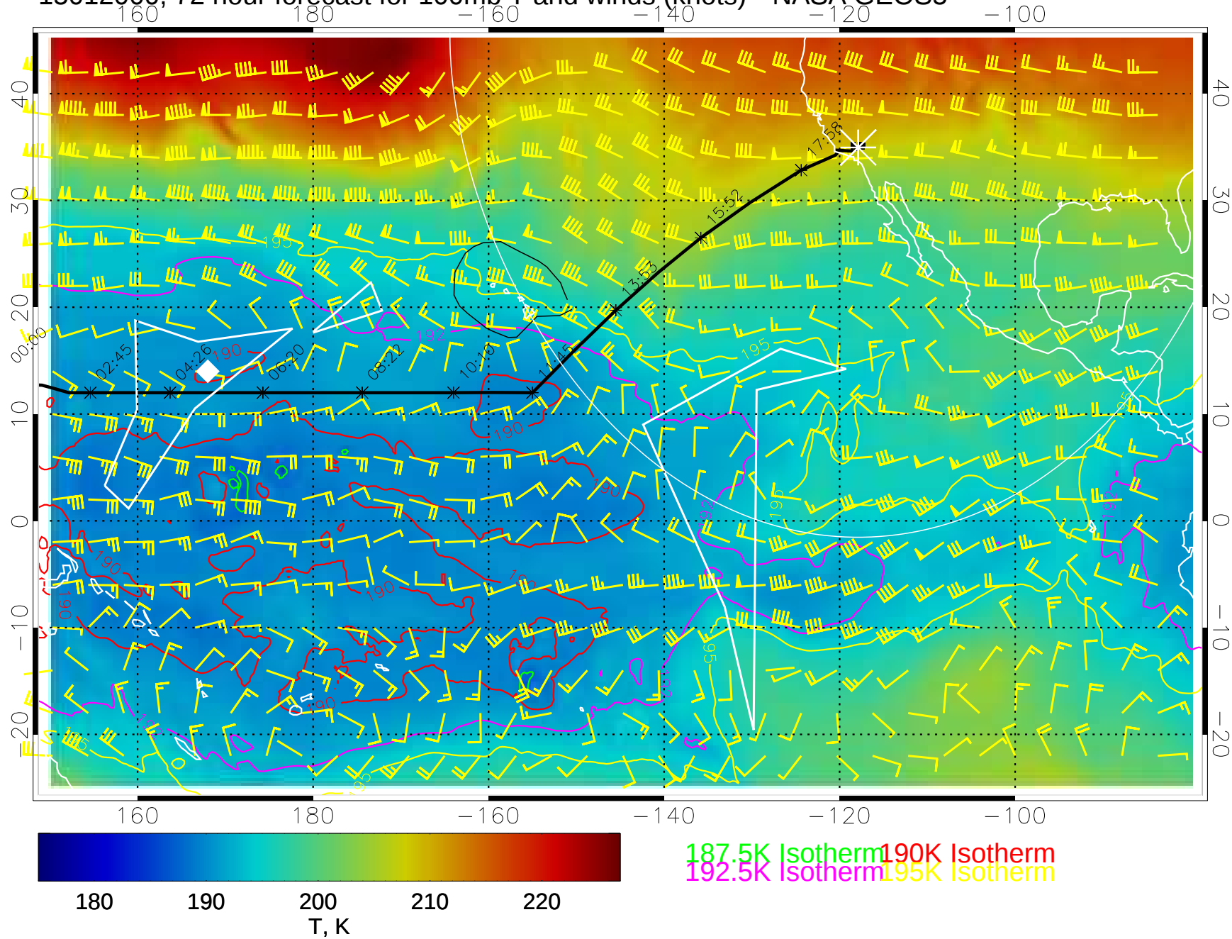
15012000, 72 hour forecast for 100mb T and winds (knots)-- NASA GEOS5
