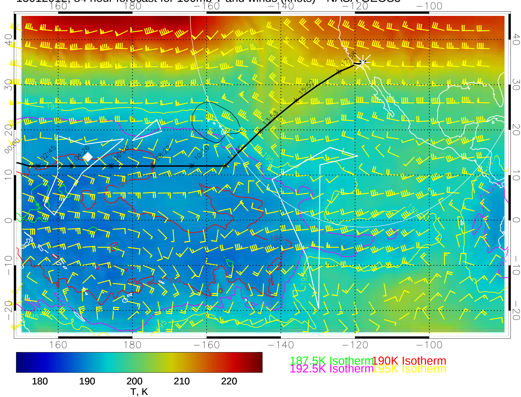
15012012, 84 hour forecast for 100mb T and winds (knots)-- NASA GEOS5
