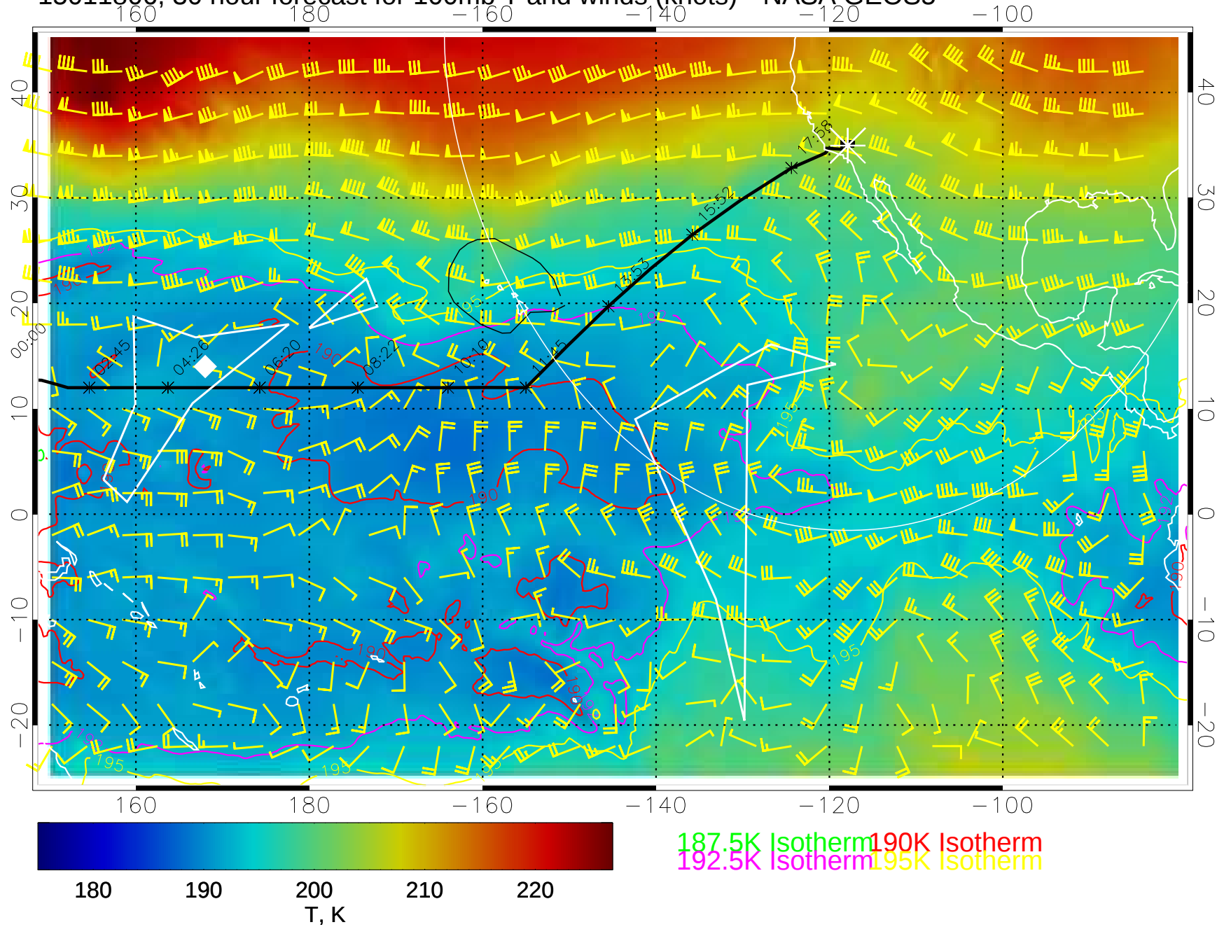
15011806, 30 hour forecast for 100mb T and winds (knots)-- NASA GEOS5
