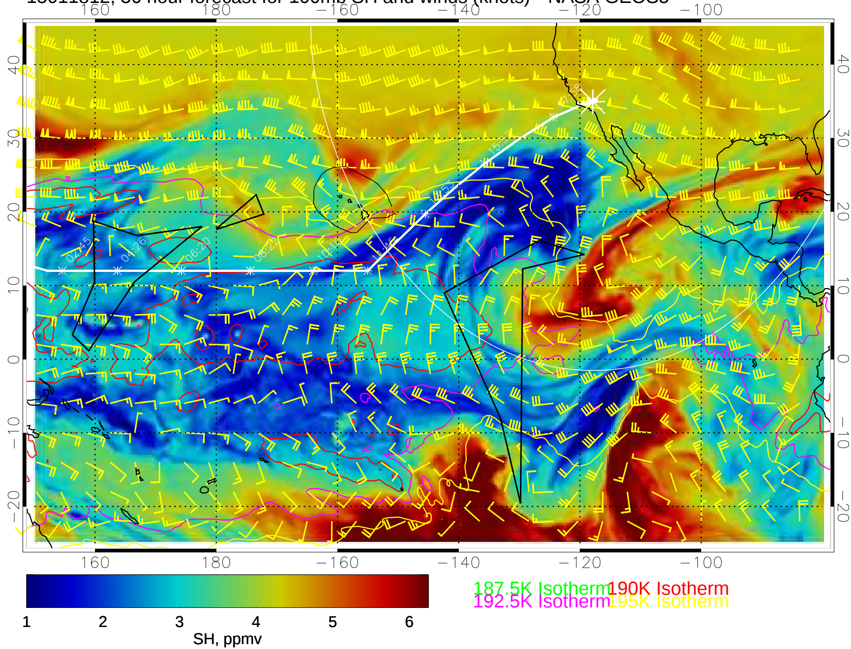
15011812, 36 hour forecast for 100mb SH and winds (knots)-- NASA GEOS5
