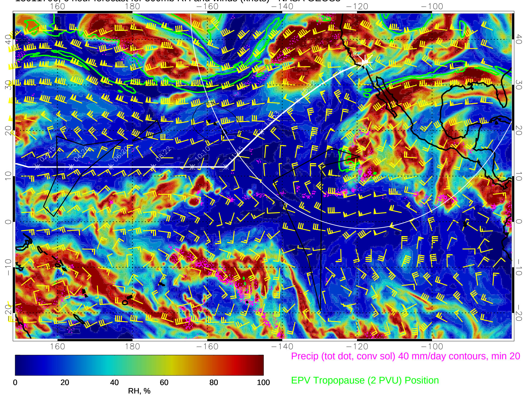
15011706, 6 hour forecast for 300mb RH and winds (knots) - NASA GEOS5
