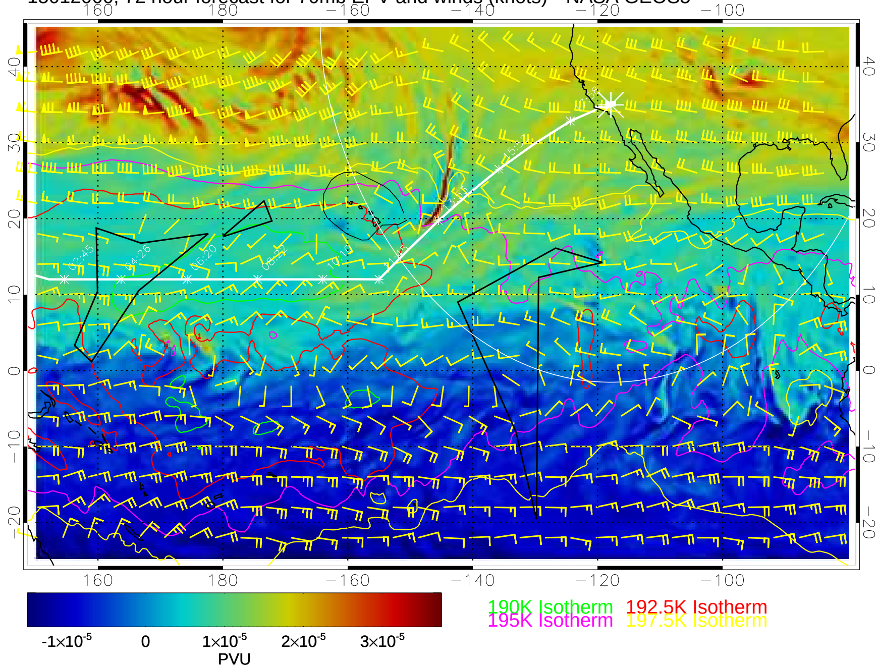
15012000, 72 hour forecast for 70mb EPV and winds (knots)-- NASA GEOS5
