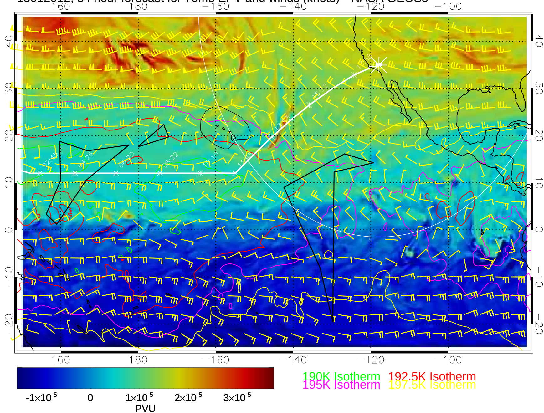
15012012, 84 hour forecast for 70mb EPV and winds (knots)-- NASA GEOS5
