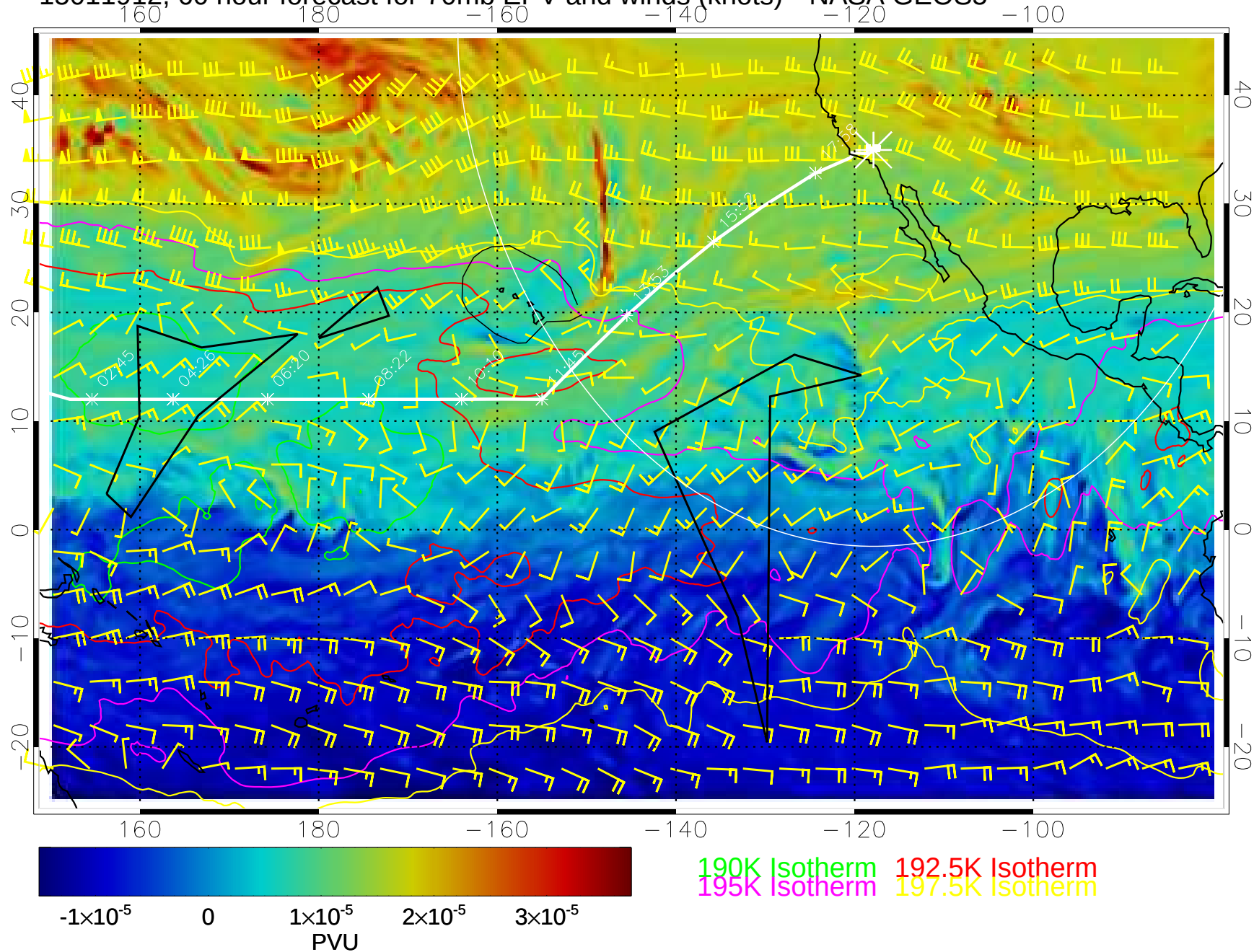
15011912, 60 hour forecast for 70mb EPV and winds (knots)-- NASA GEOS5
