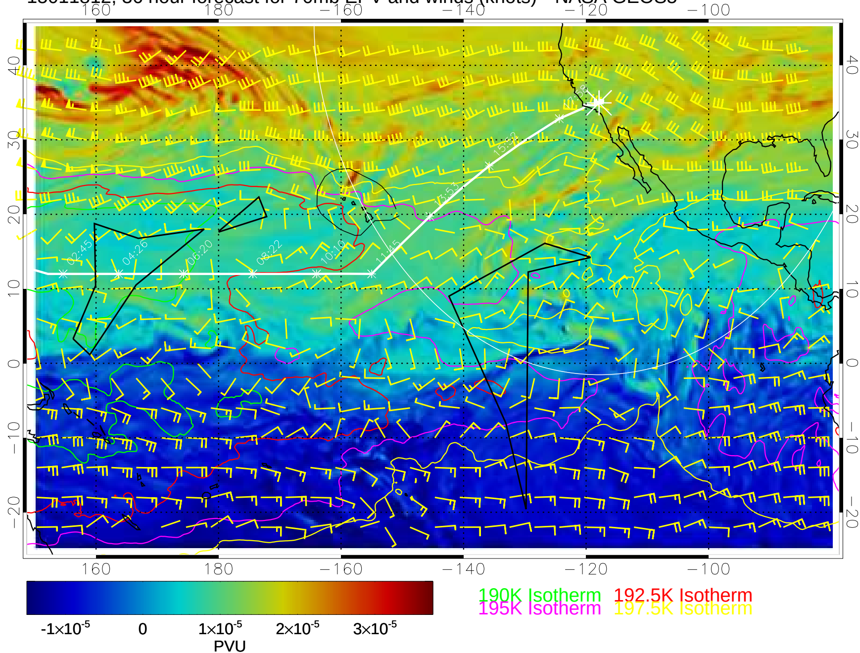
15011812, 36 hour forecast for 70mb EPV and winds (knots)-- NASA GEOS5
