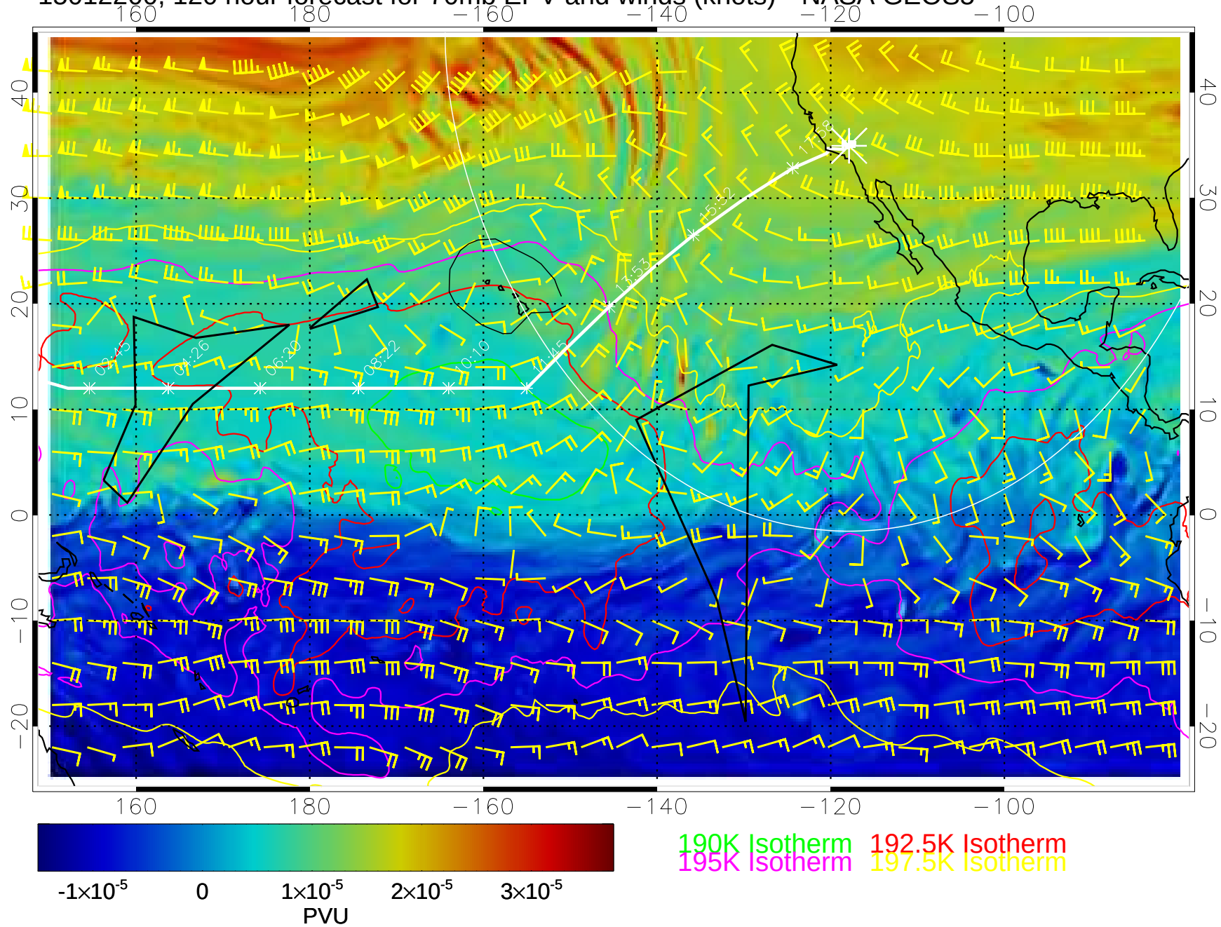
15012200, 120 hour forecast for 70mb EPV and winds (knots)-- NASA GEOS5
