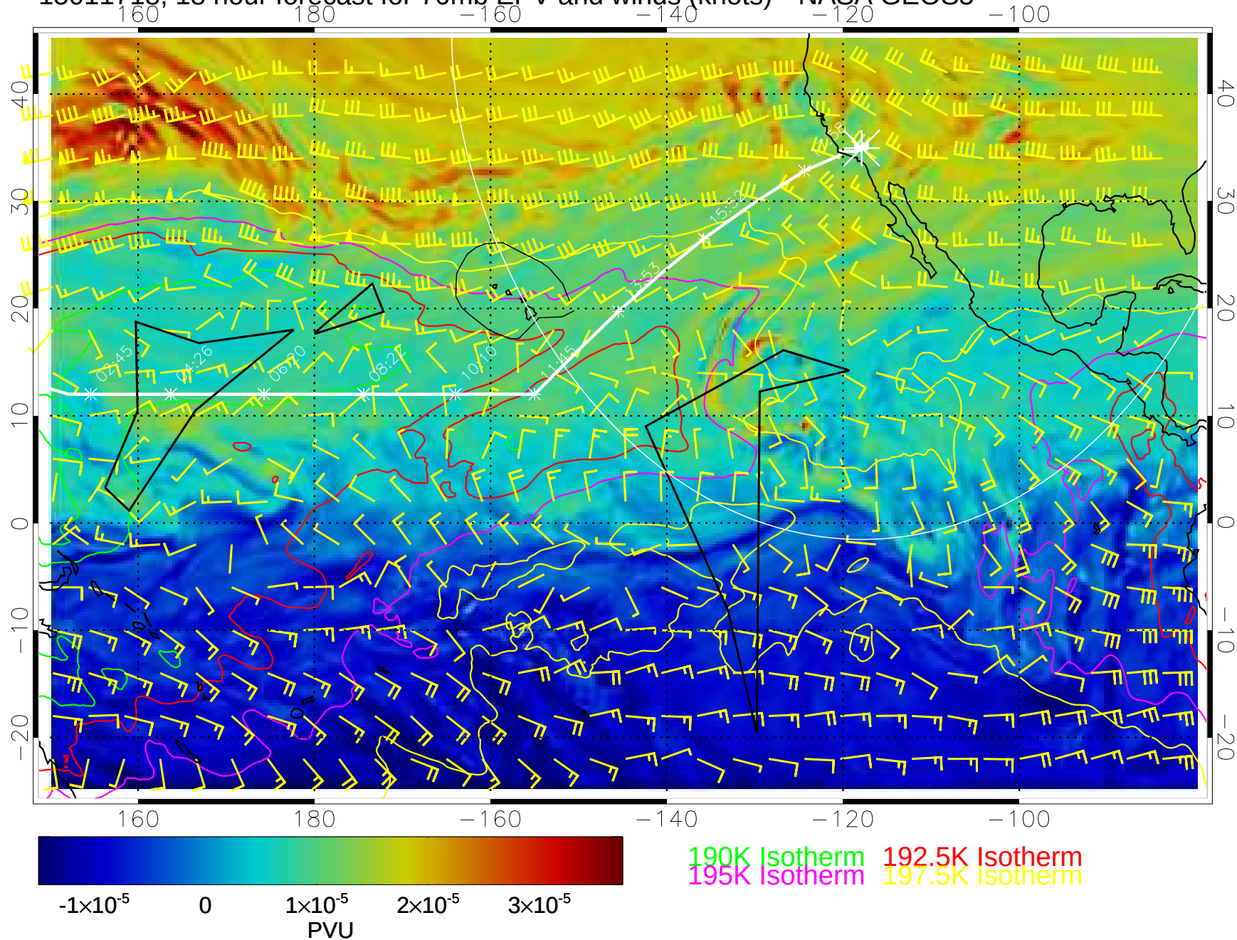
15011718, 18 hour forecast for 70mb EPV and winds (knots)-- NASA GEOS5
