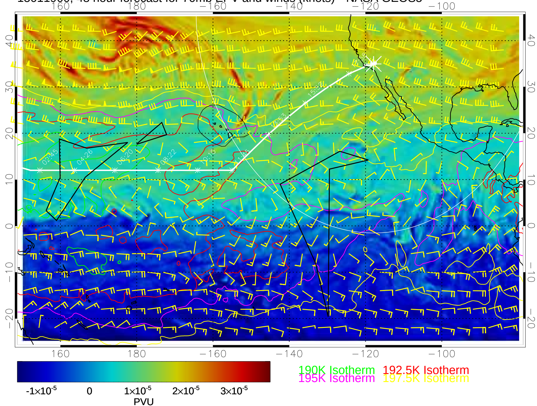
15011900, 48 hour forecast for 70mb EPV and winds (knots)-- NASA GEOS5
