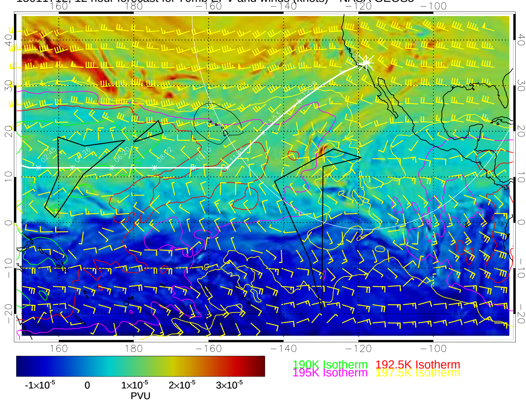
15011712, 12 hour forecast for 70mb EPV and winds (knots)-- NASA GEOS5
