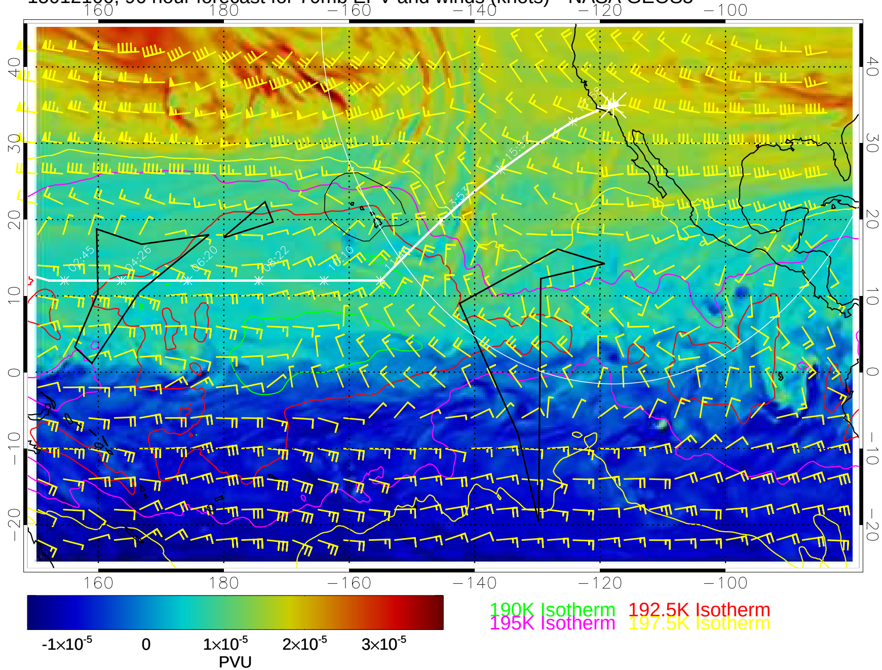
15012100, 96 hour forecast for 70mb EPV and winds (knots)-- NASA GEOS5
