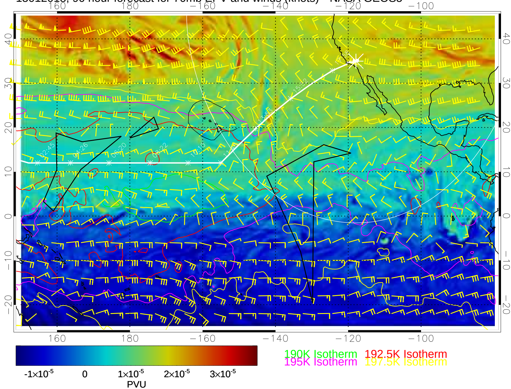
15012018, 90 hour forecast for 70mb EPV and winds (knots)-- NASA GEOS5
