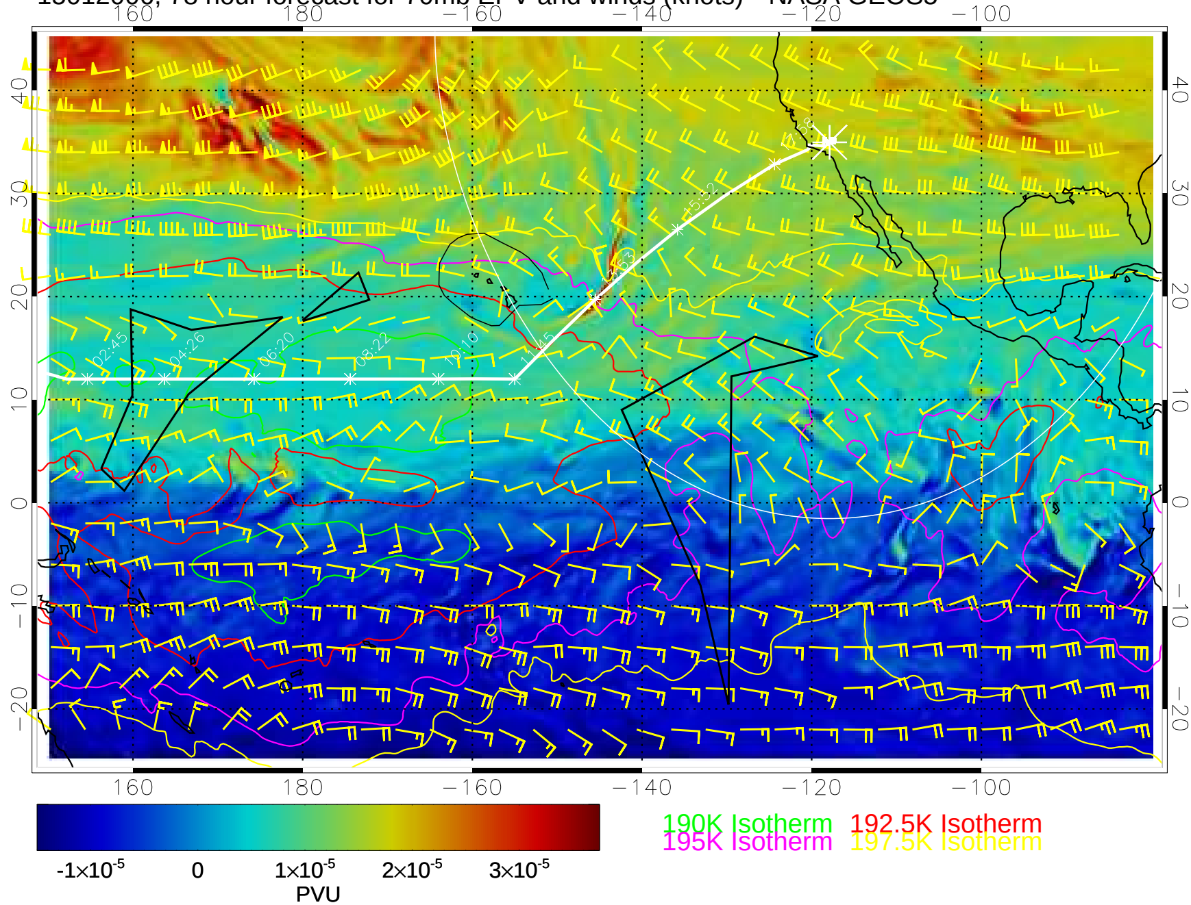
15012006, 78 hour forecast for 70mb EPV and winds (knots)-- NASA GEOS5
