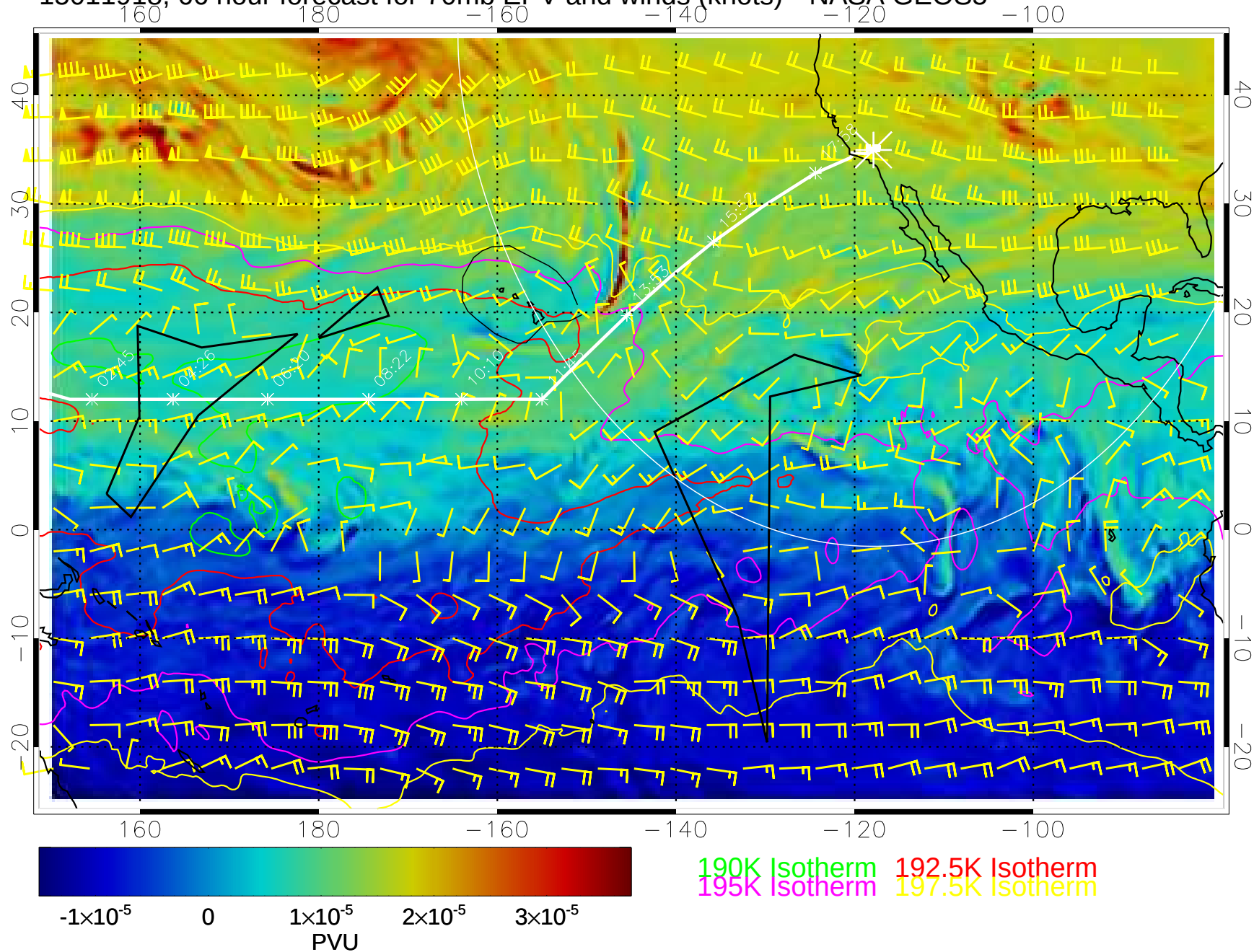
15011918, 66 hour forecast for 70mb EPV and winds (knots)-- NASA GEOS5
