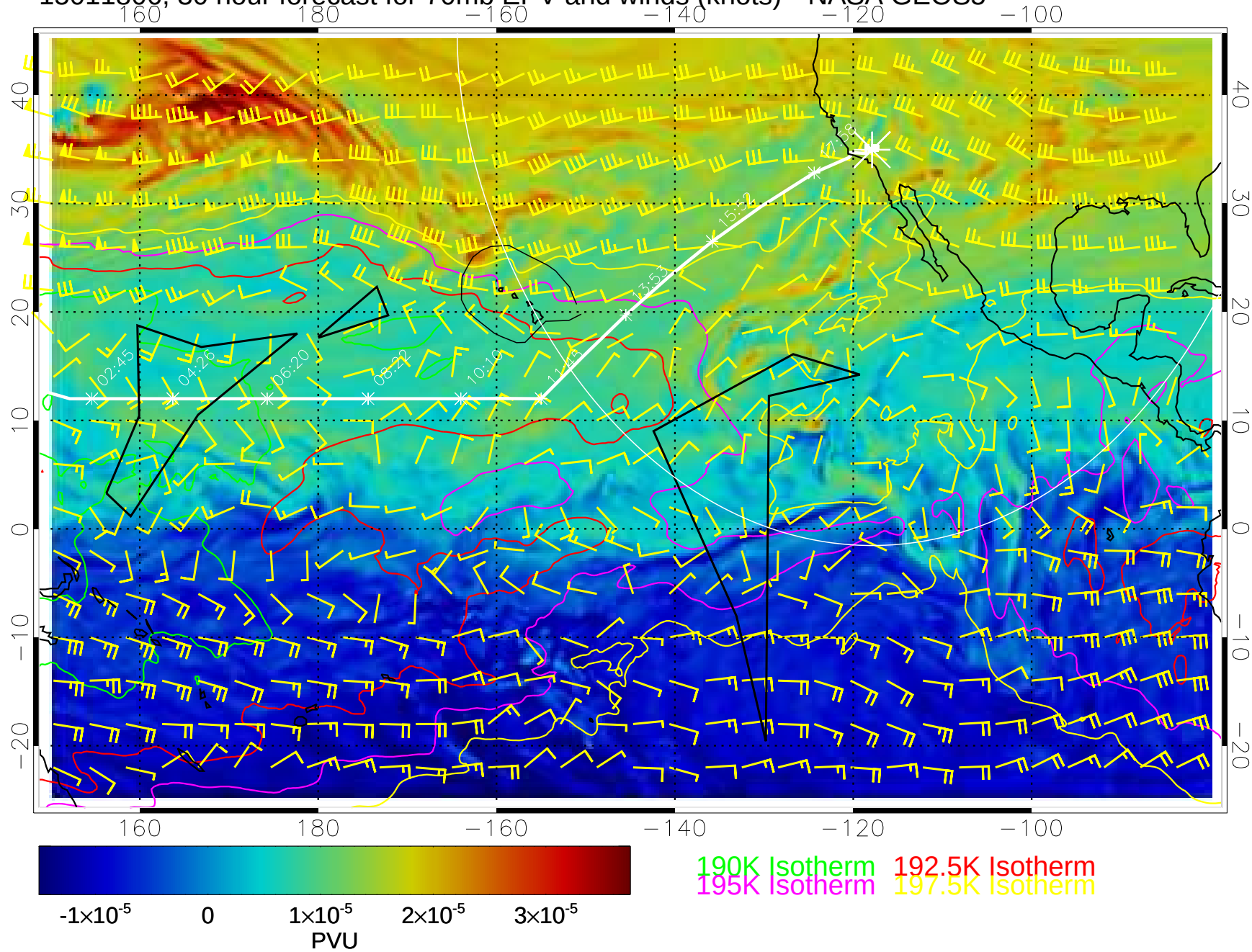
15011806, 30 hour forecast for 70mb EPV and winds (knots)-- NASA GEOS5
