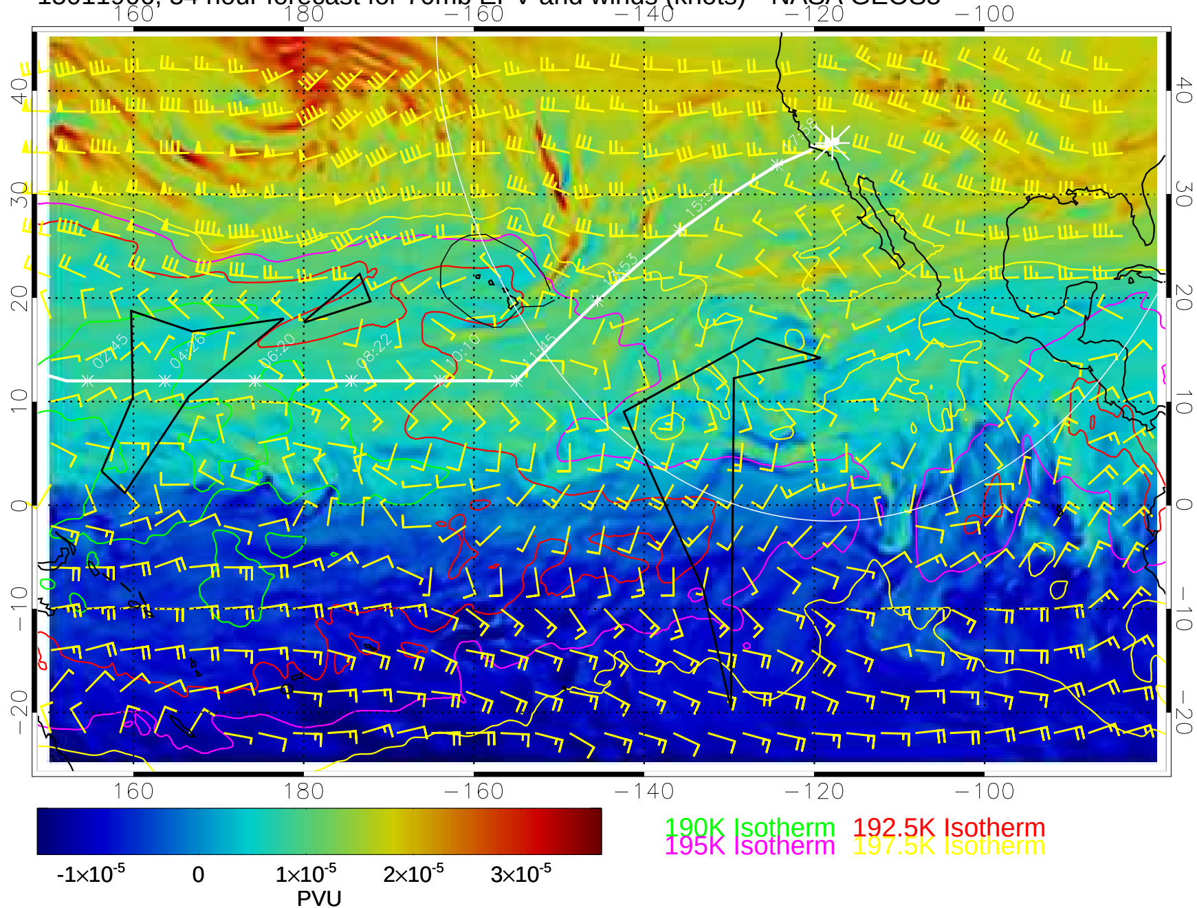
15011906, 54 hour forecast for 70mb EPV and winds (knots)-- NASA GEOS5
