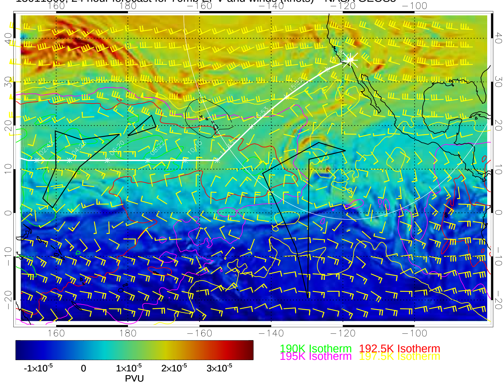
15011800, 24 hour forecast for 70mb EPV and winds (knots)-- NASA GEOS5
