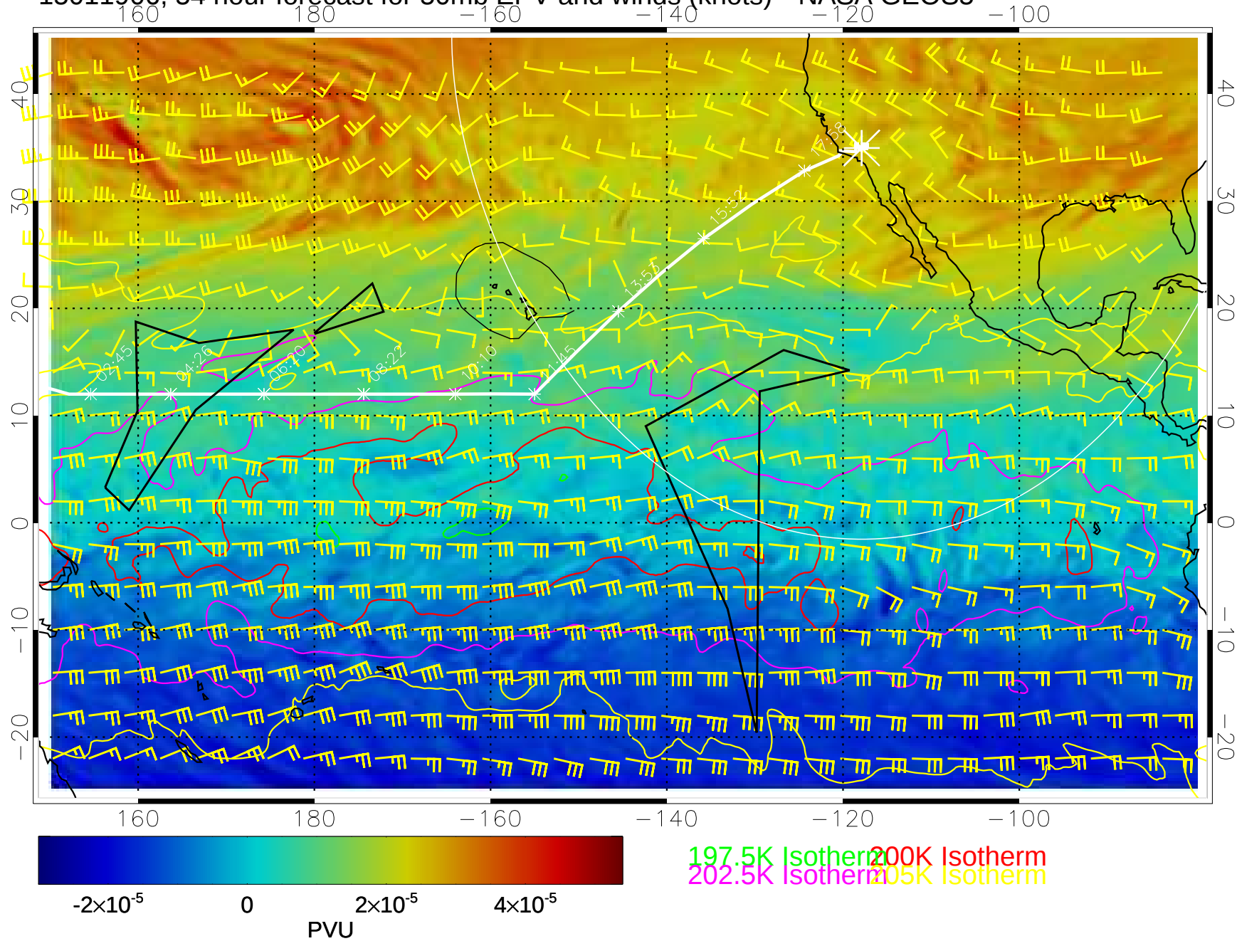
15011906, 54 hour forecast for 50mb EPV and winds (knots)-- NASA GEOS5
