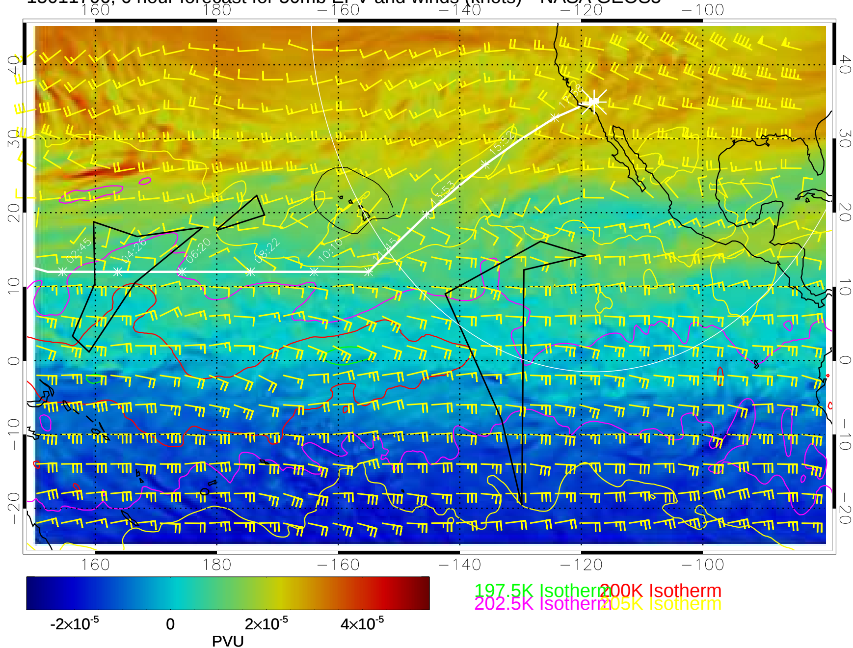
15011706, 6 hour forecast for 50mb EPV and winds (knots)-- NASA GEOS5
