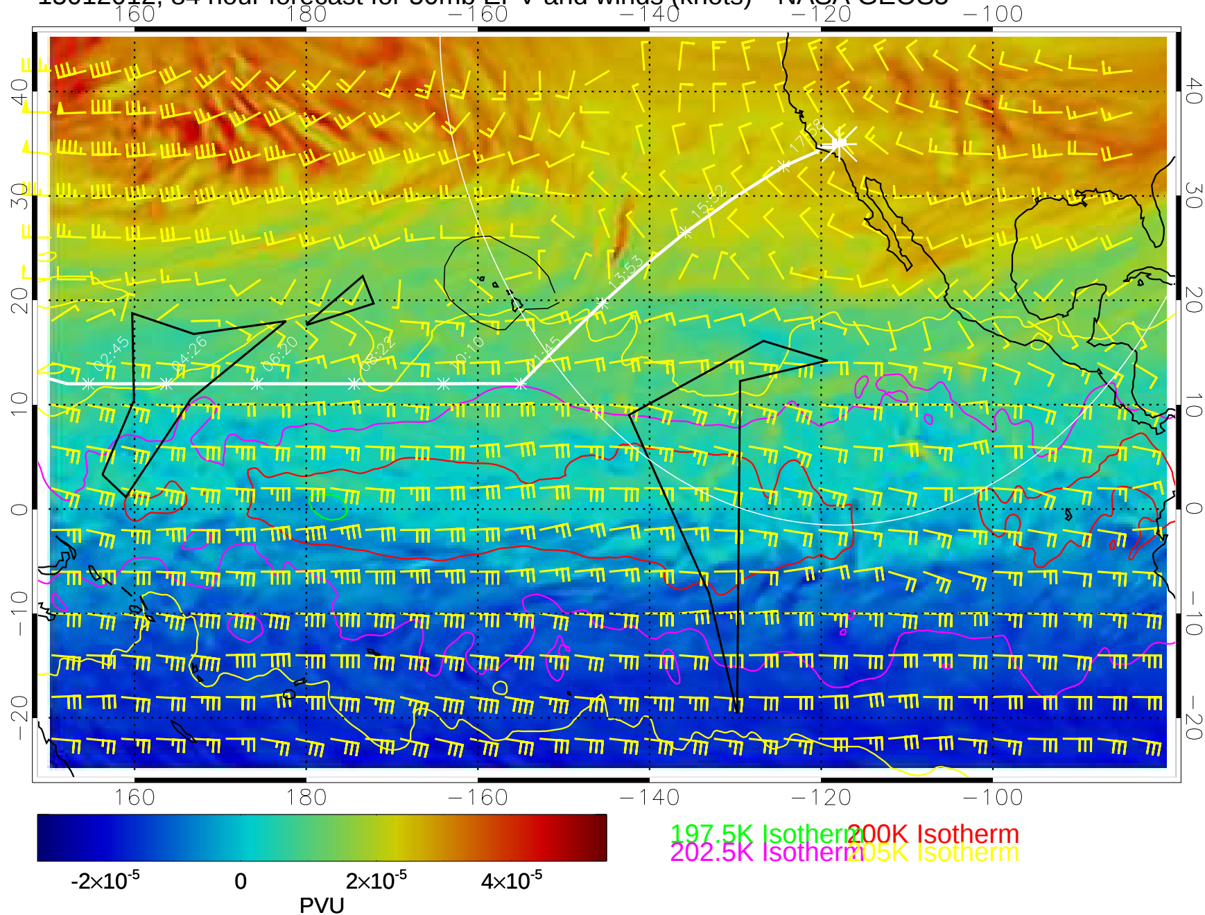
15012012, 84 hour forecast for 50mb EPV and winds (knots)-- NASA GEOS5
