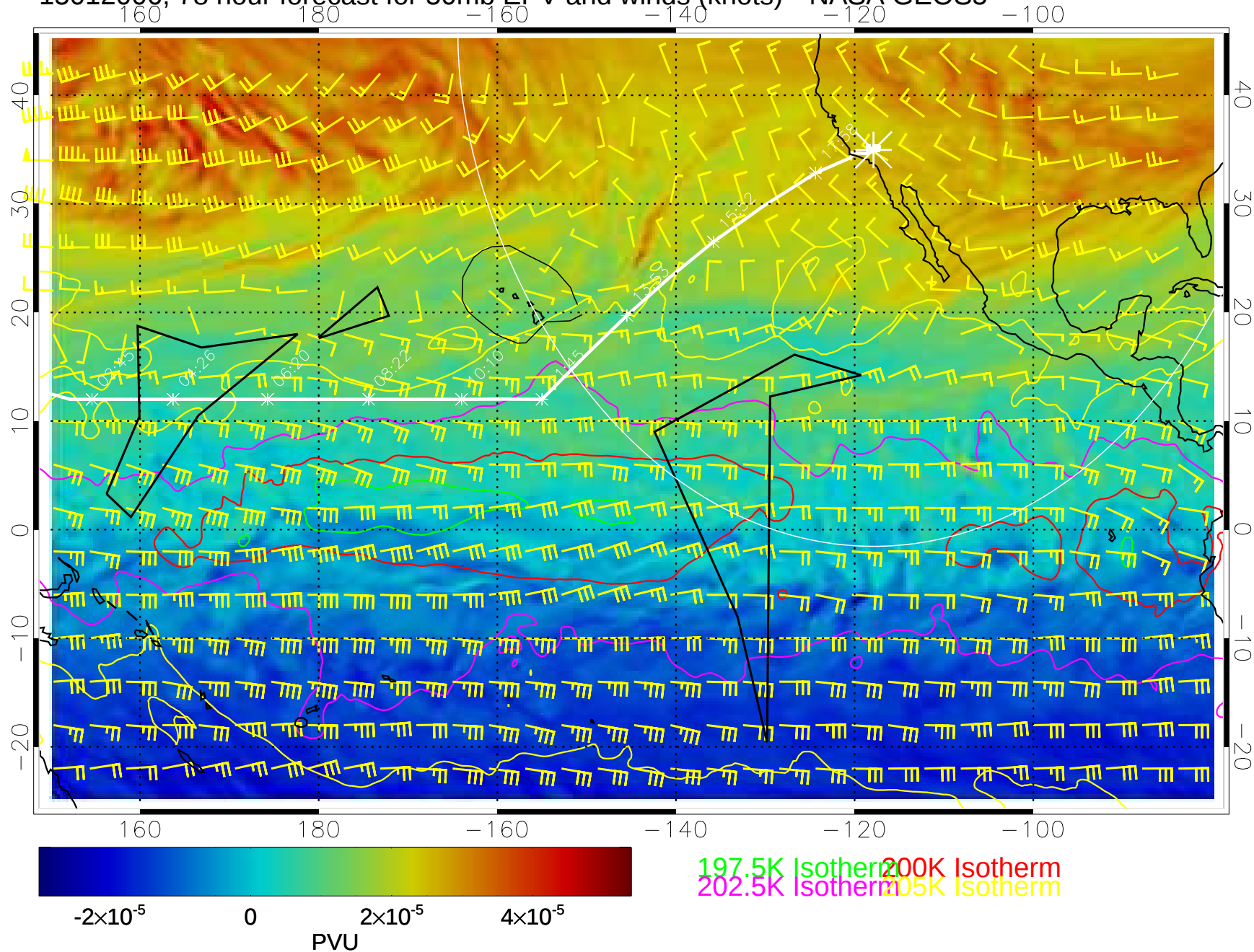
15012006, 78 hour forecast for 50mb EPV and winds (knots)-- NASA GEOS5
