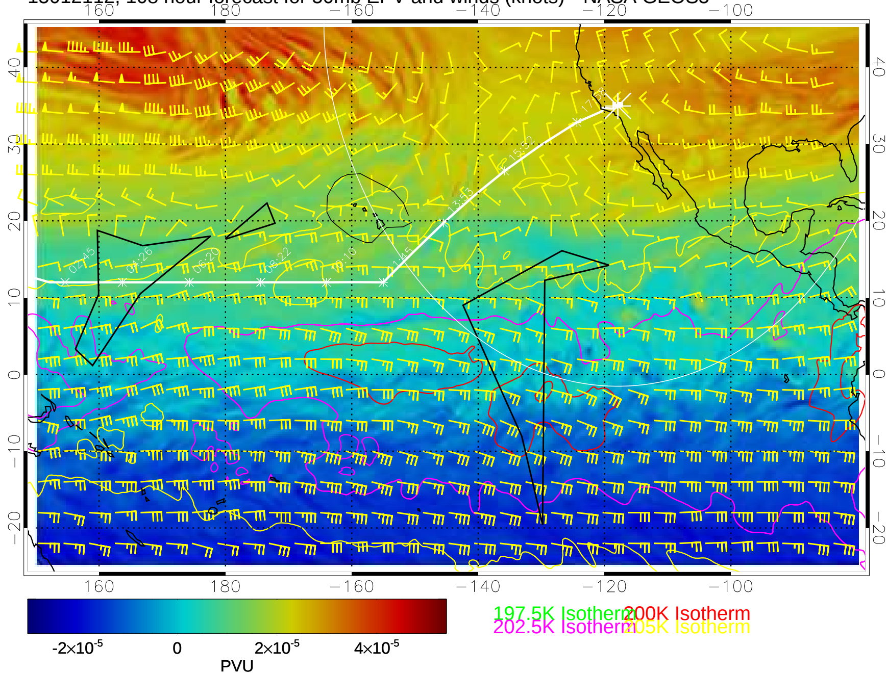
15012112, 108 hour forecast for 50mb EPV and winds (knots)-- NASA GEOS5
