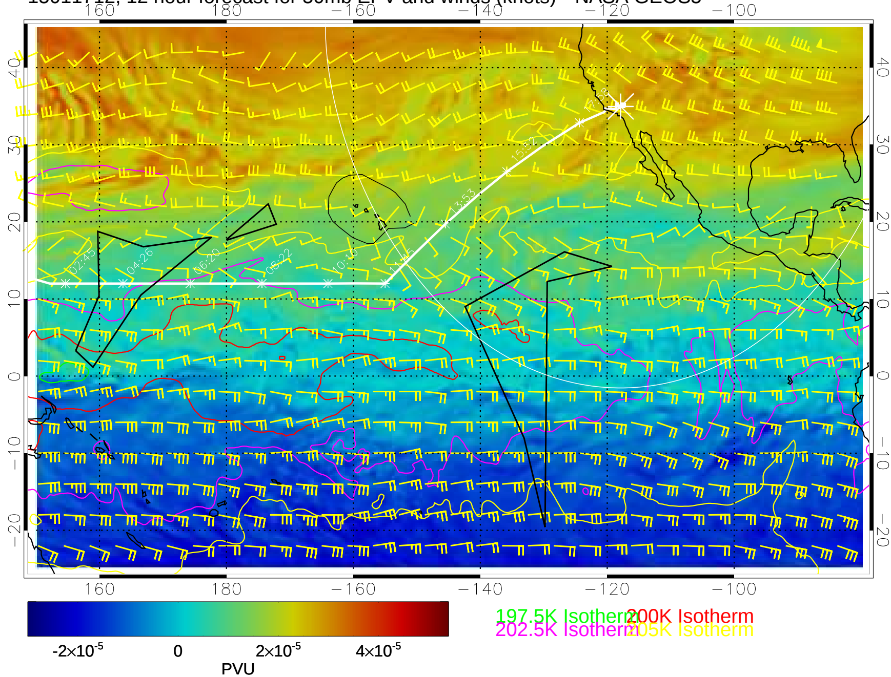
15011712, 12 hour forecast for 50mb EPV and winds (knots)-- NASA GEOS5
