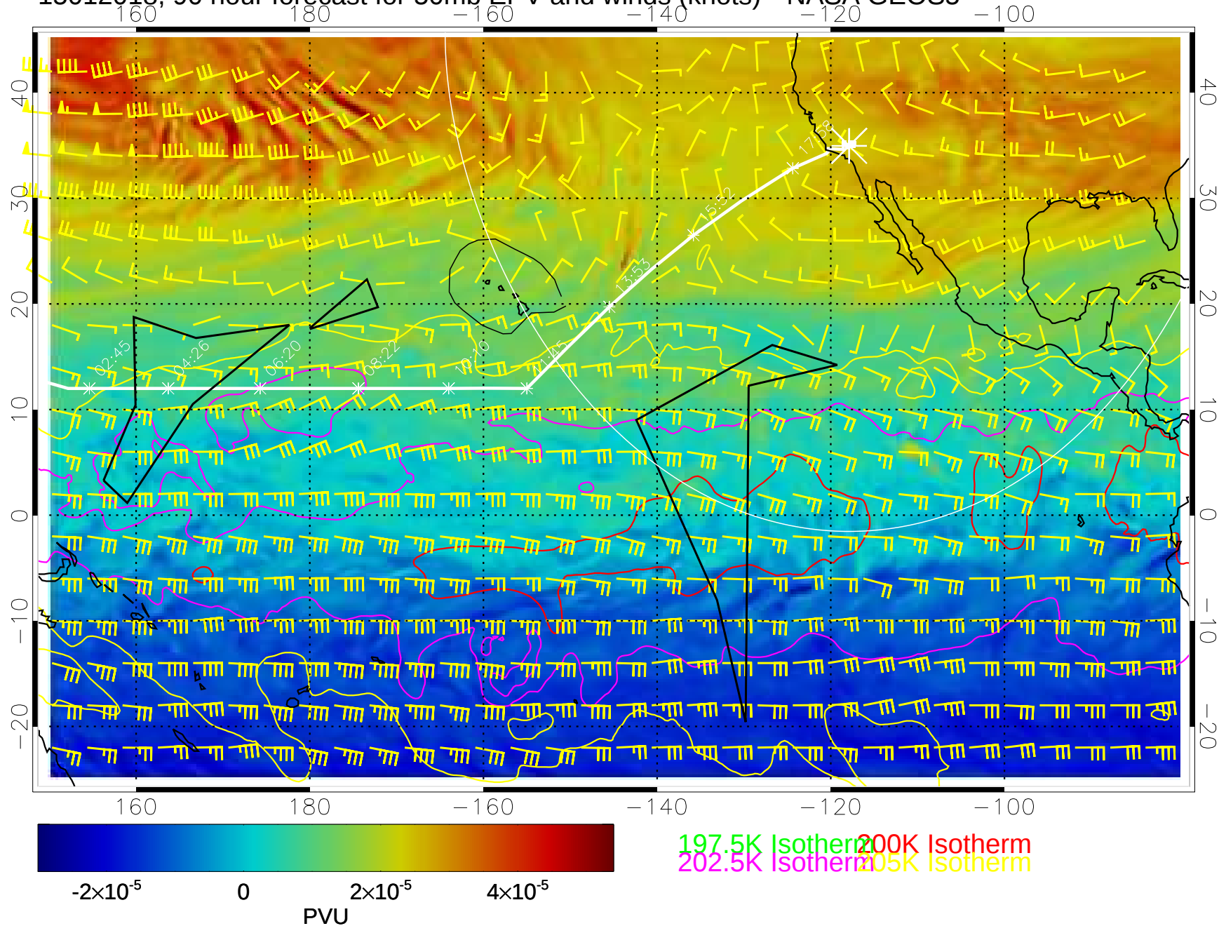
15012018, 90 hour forecast for 50mb EPV and winds (knots)-- NASA GEOS5
