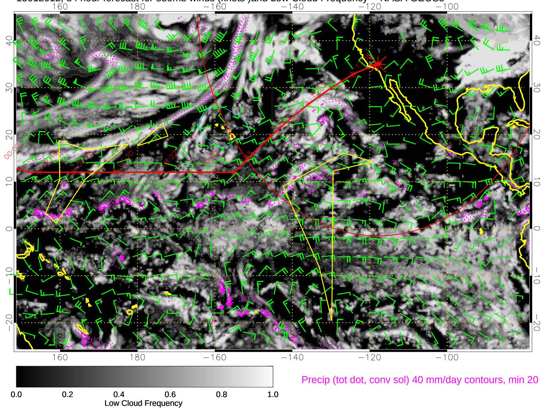
15012012, 84 hour forecast for 850mb winds (knots) and Low Cloud Frequency -- NASA GEOS5
