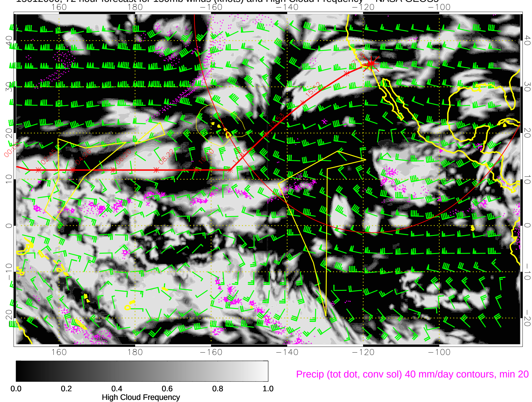
15012000, 72 hour forecast for 150mb winds (knots) and High Cloud Frequency -- NASA GEOS5
