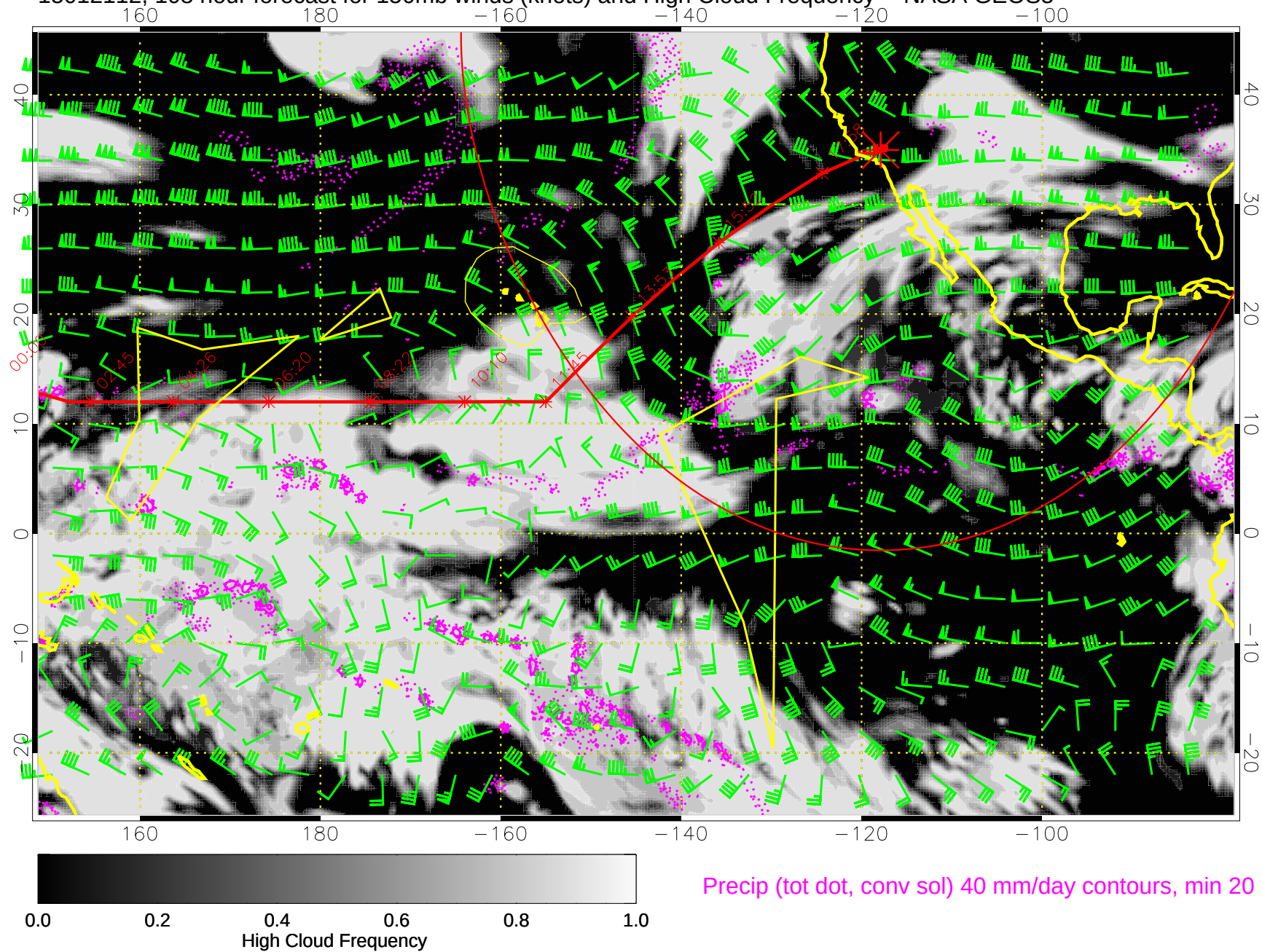
15012112, 108 hour forecast for 150mb winds (knots) and High Cloud Frequency -- NASA GEOS5
