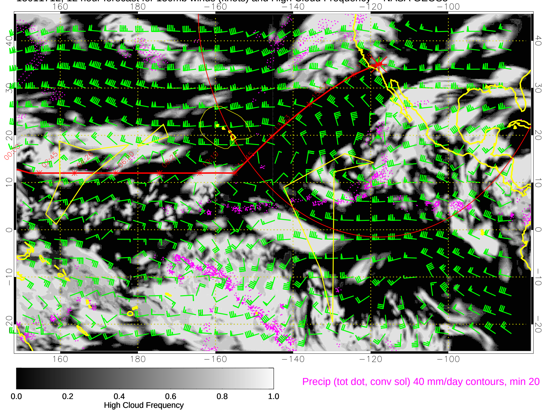
15011712, 12 hour forecast for 150mb winds (knots) and High Cloud Frequency -- NASA GEOS5
