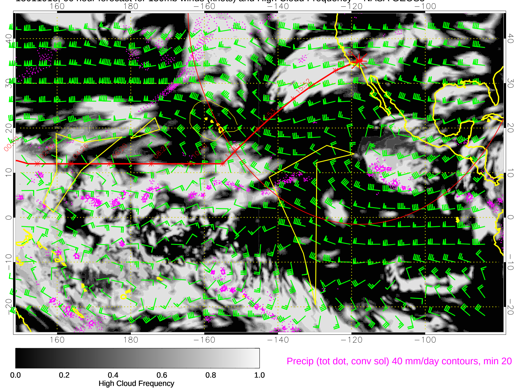
15011918, 66 hour forecast for 150mb winds (knots) and High Cloud Frequency -- NASA GEOS5
