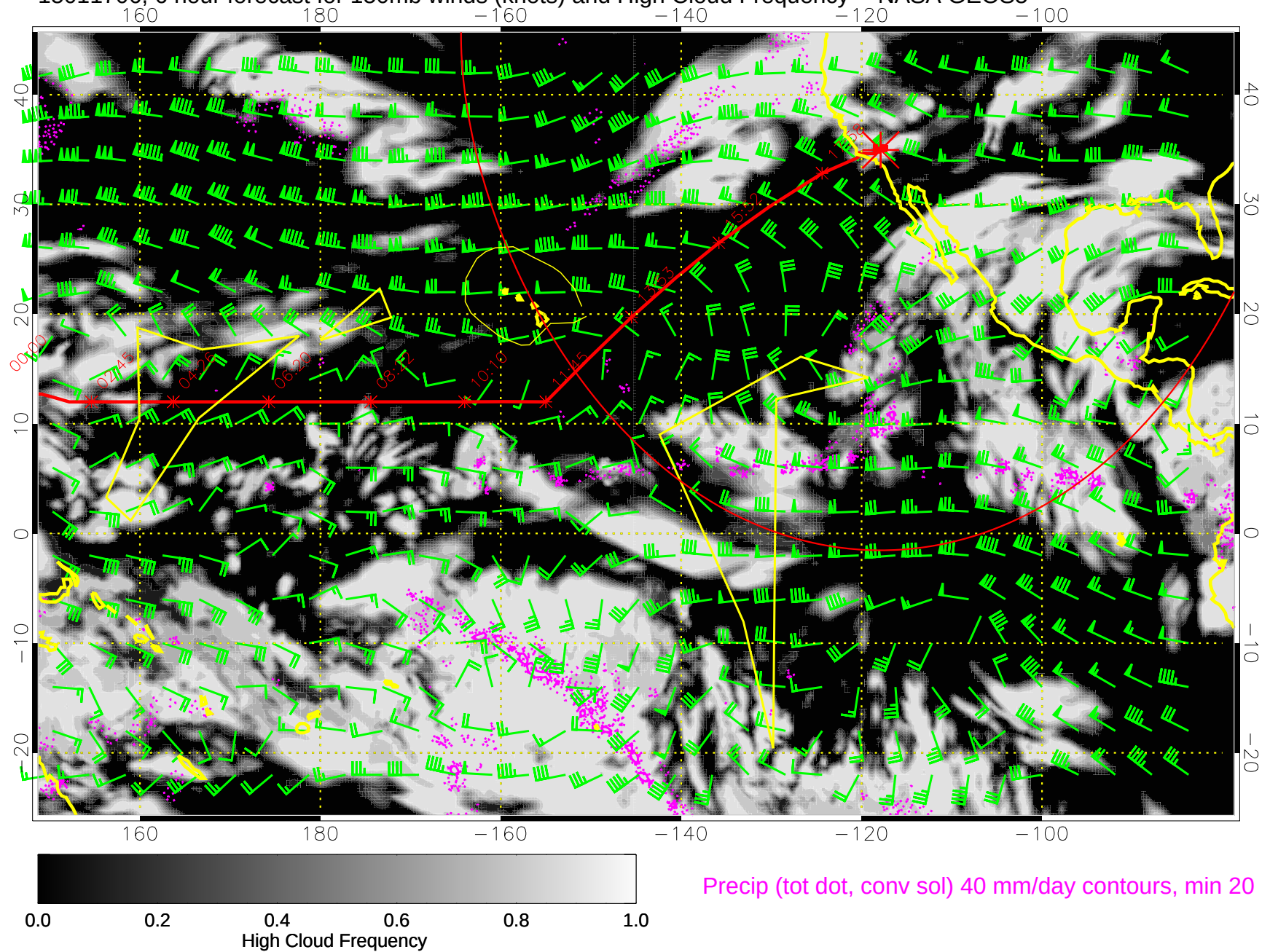
15011706, 6 hour forecast for 150mb winds (knots) and High Cloud Frequency -- NASA GEOS5
