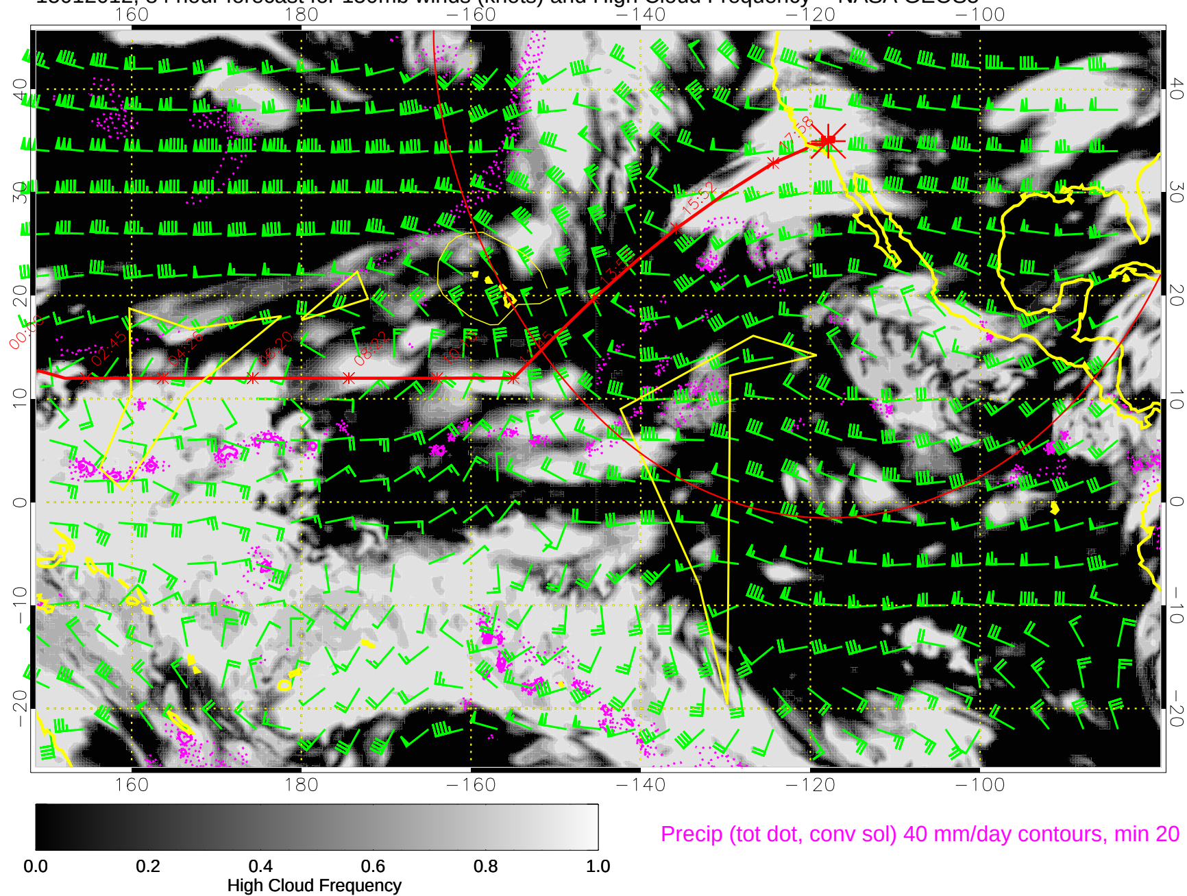
15012012, 84 hour forecast for 150mb winds (knots) and High Cloud Frequency -- NASA GEOS5
