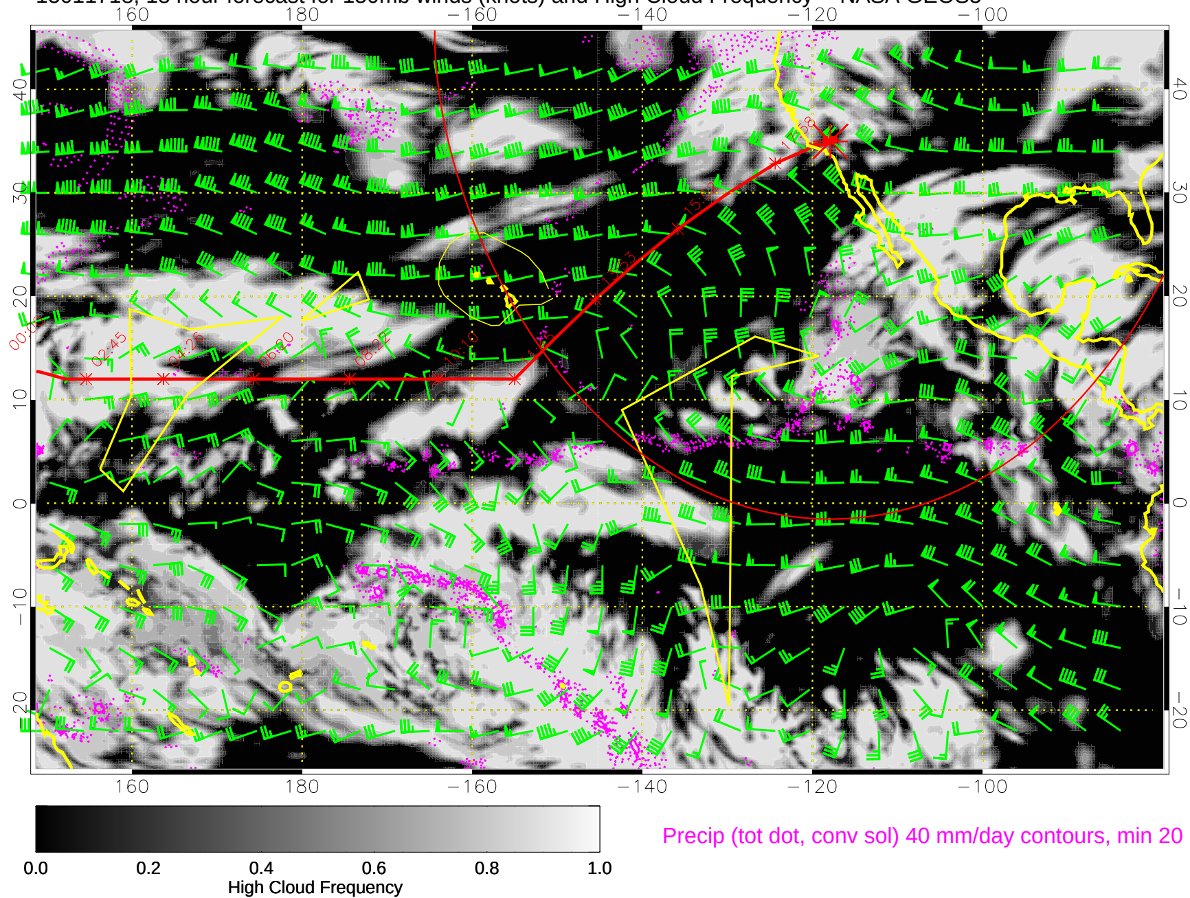
15011718, 18 hour forecast for 150mb winds (knots) and High Cloud Frequency -- NASA GEOS5
