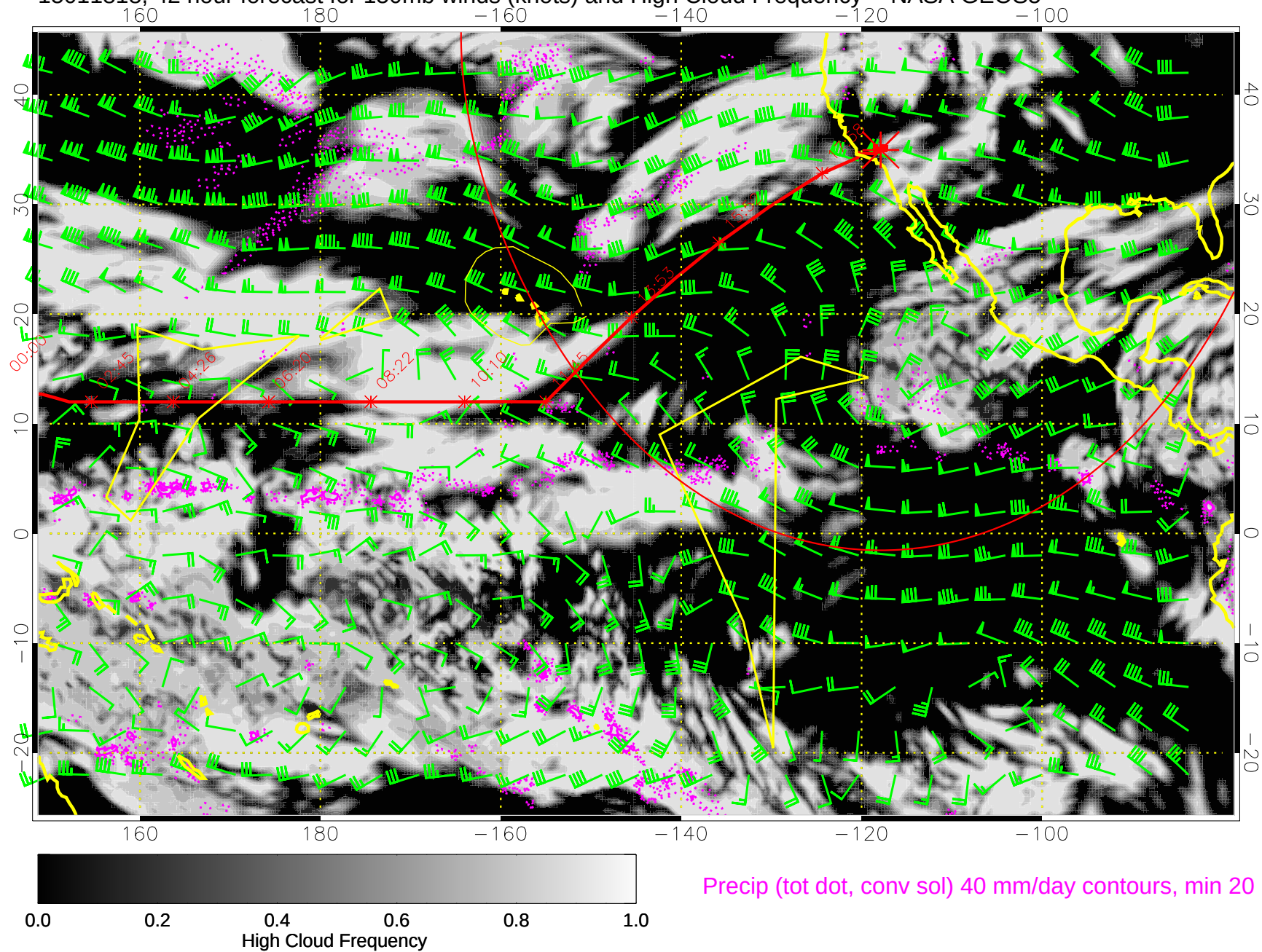
15011818, 42 hour forecast for 150mb winds (knots) and High Cloud Frequency -- NASA GEOS5
