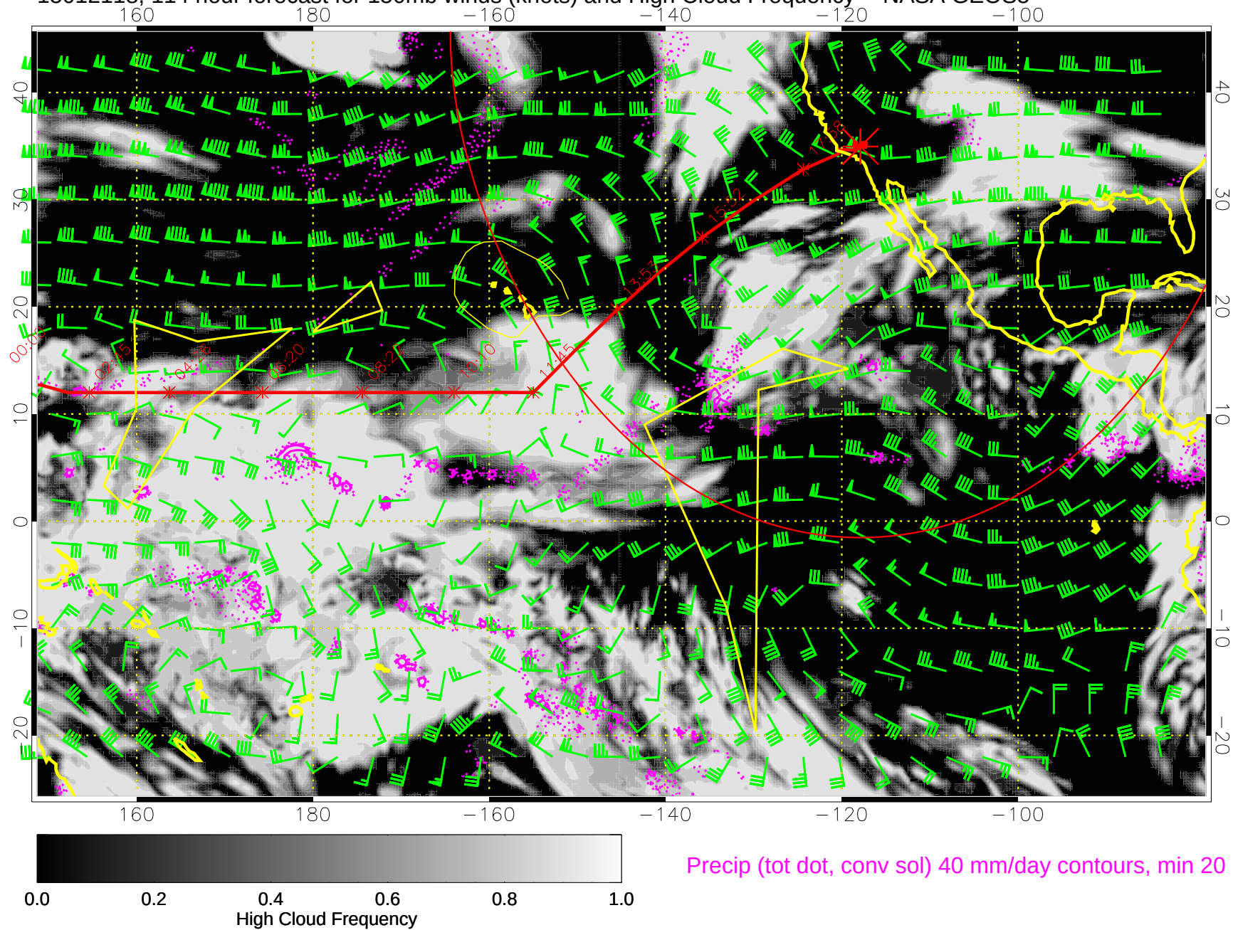
15012118, 114 hour forecast for 150mb winds (knots) and High Cloud Frequency -- NASA GEOS5
