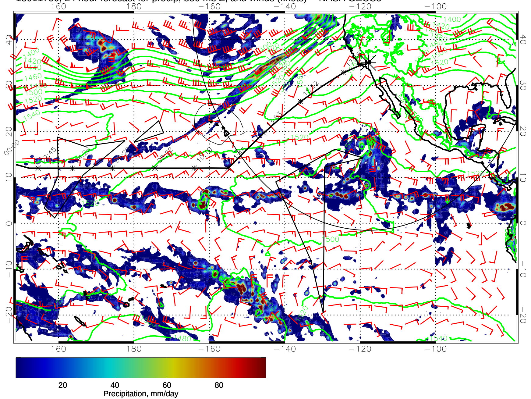
15011700, 24 hour forecast for precip, 850 mb Z, and winds (knots) -- NASA GEOS5
