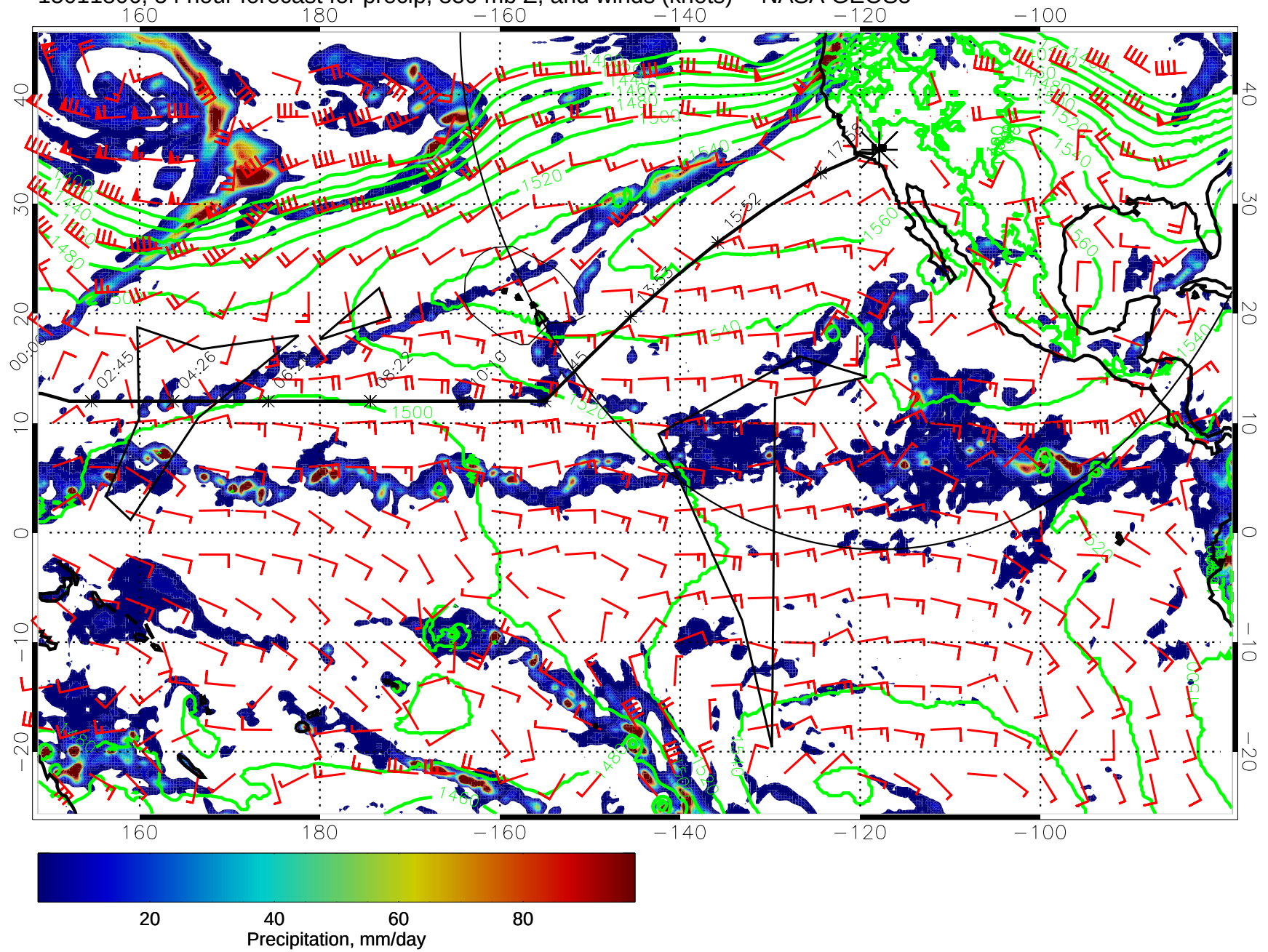
15011806, 54 hour forecast for precip, 850 mb Z, and winds (knots) -- NASA GEOS5
