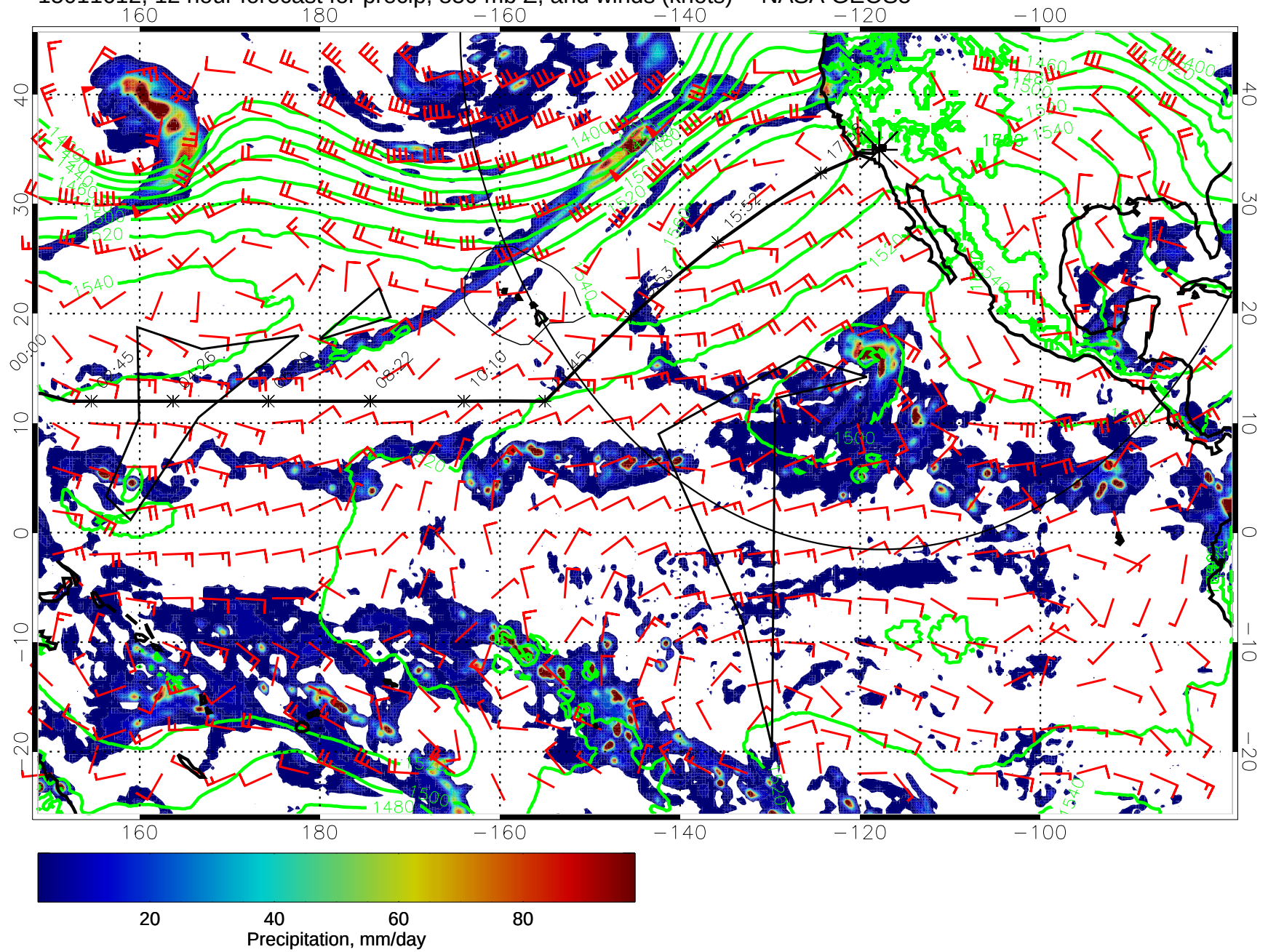
15011612, 12 hour forecast for precip, 850 mb Z, and winds (knots) -- NASA GEOS5
