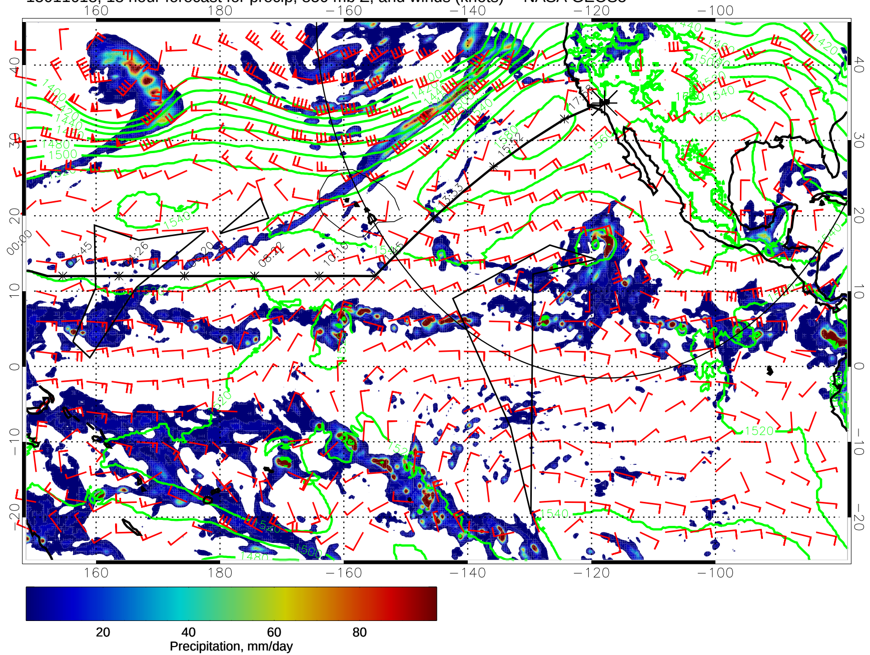
15011618, 18 hour forecast for precip, 850 mb Z, and winds (knots) -- NASA GEOS5
