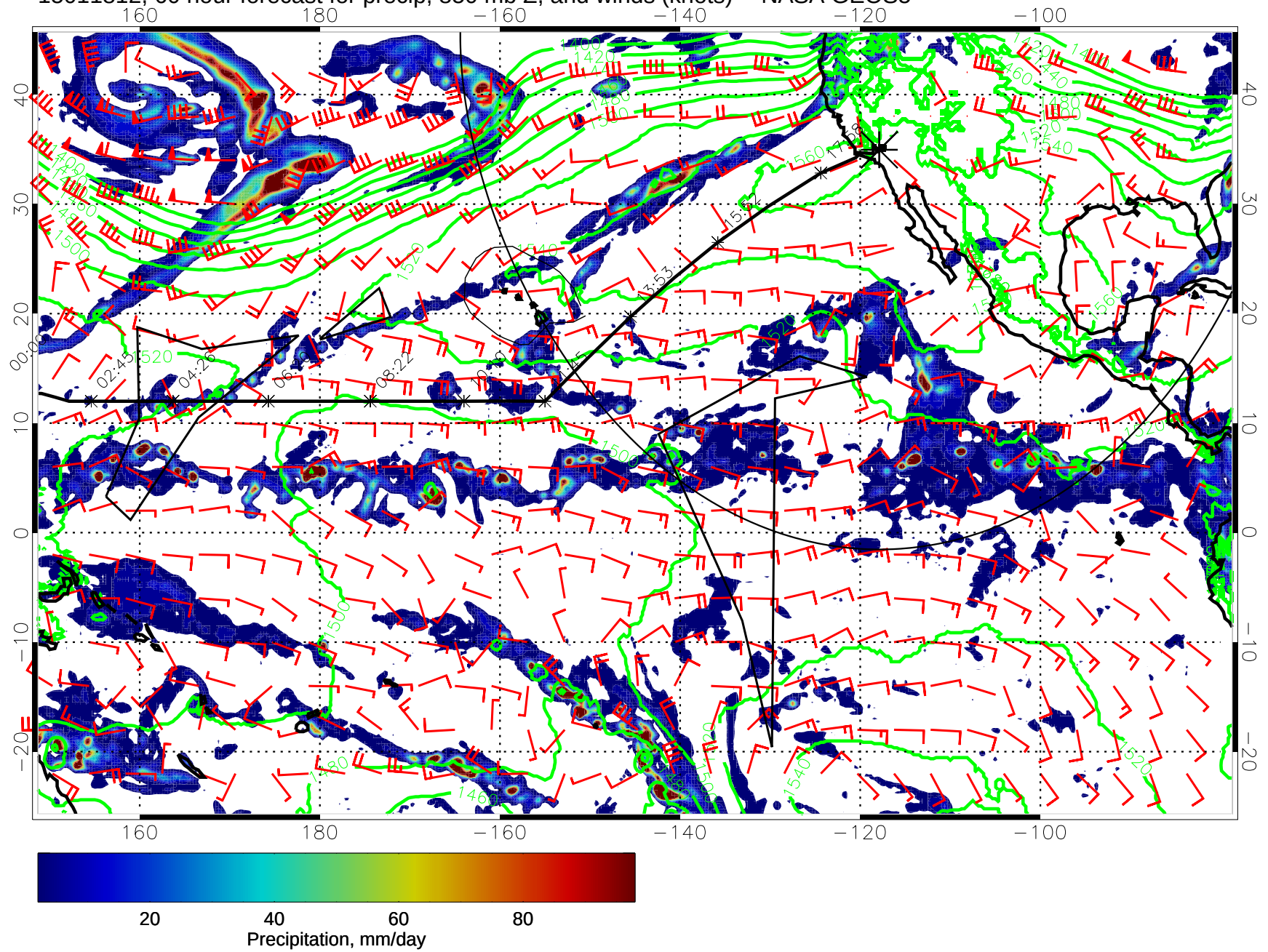
15011812, 60 hour forecast for precip, 850 mb Z, and winds (knots) -- NASA GEOS5
