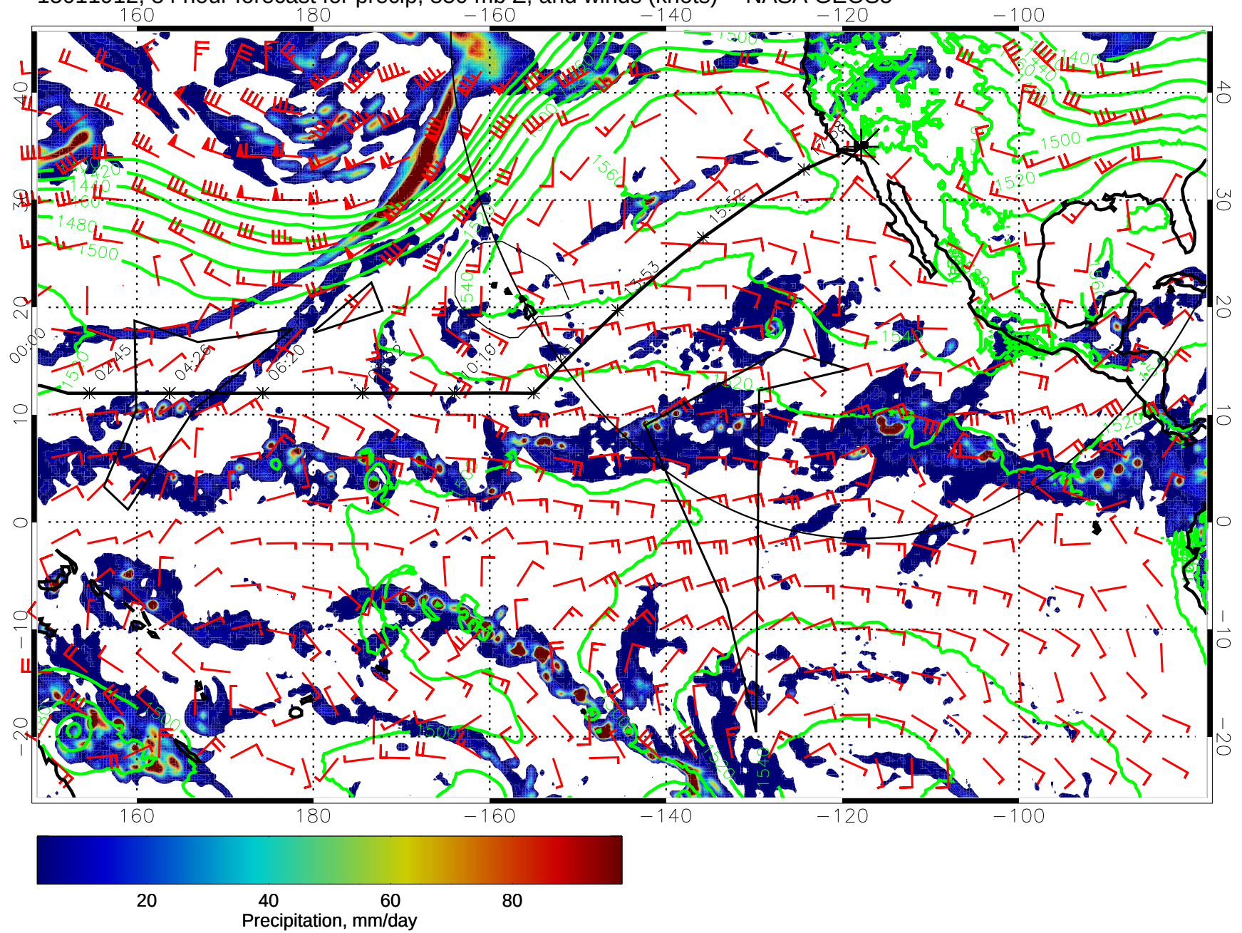
15011912, 84 hour forecast for precip, 850 mb Z, and winds (knots) -- NASA GEOS5
