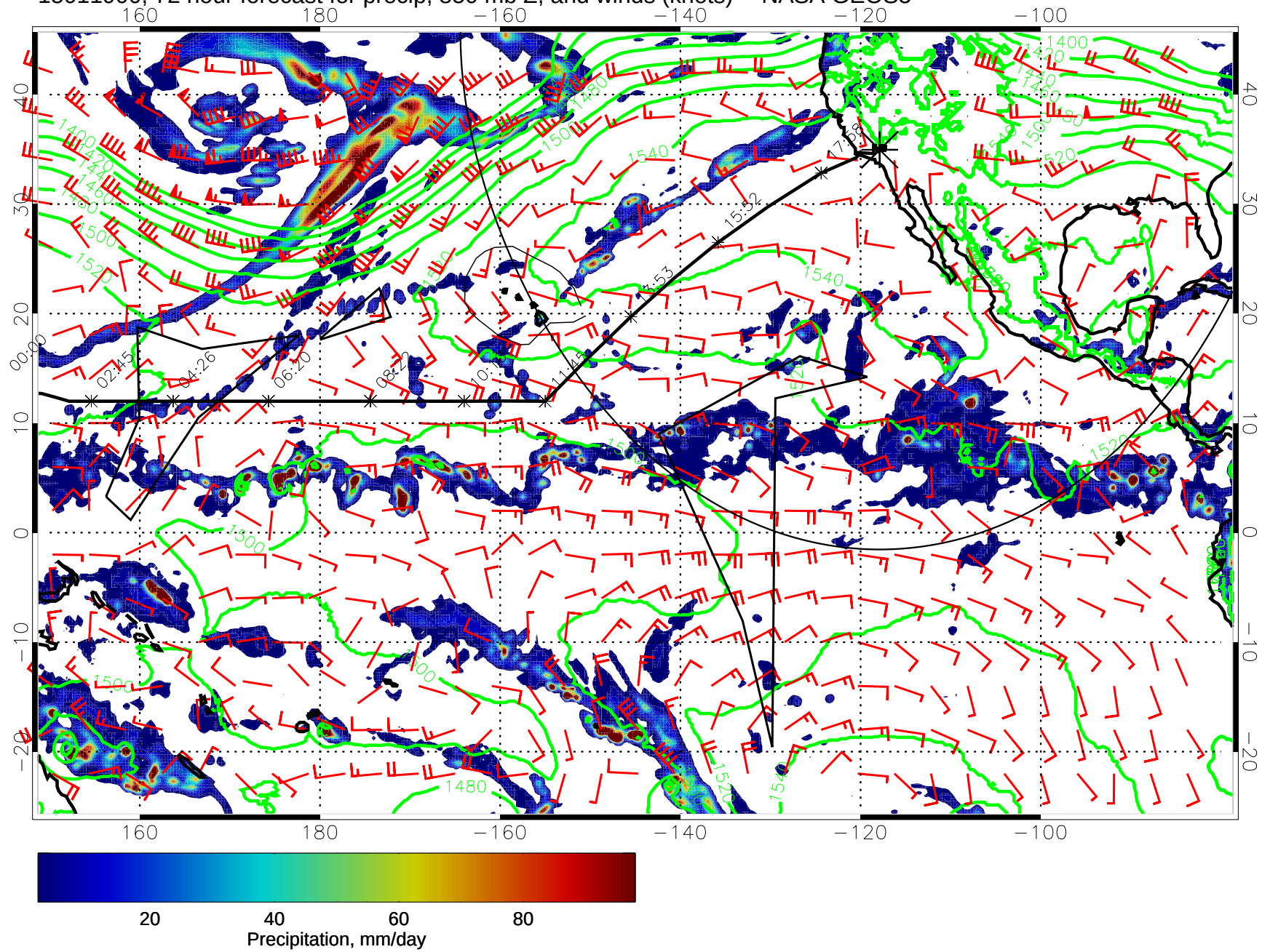
15011900, 72 hour forecast for precip, 850 mb Z, and winds (knots) -- NASA GEOS5
