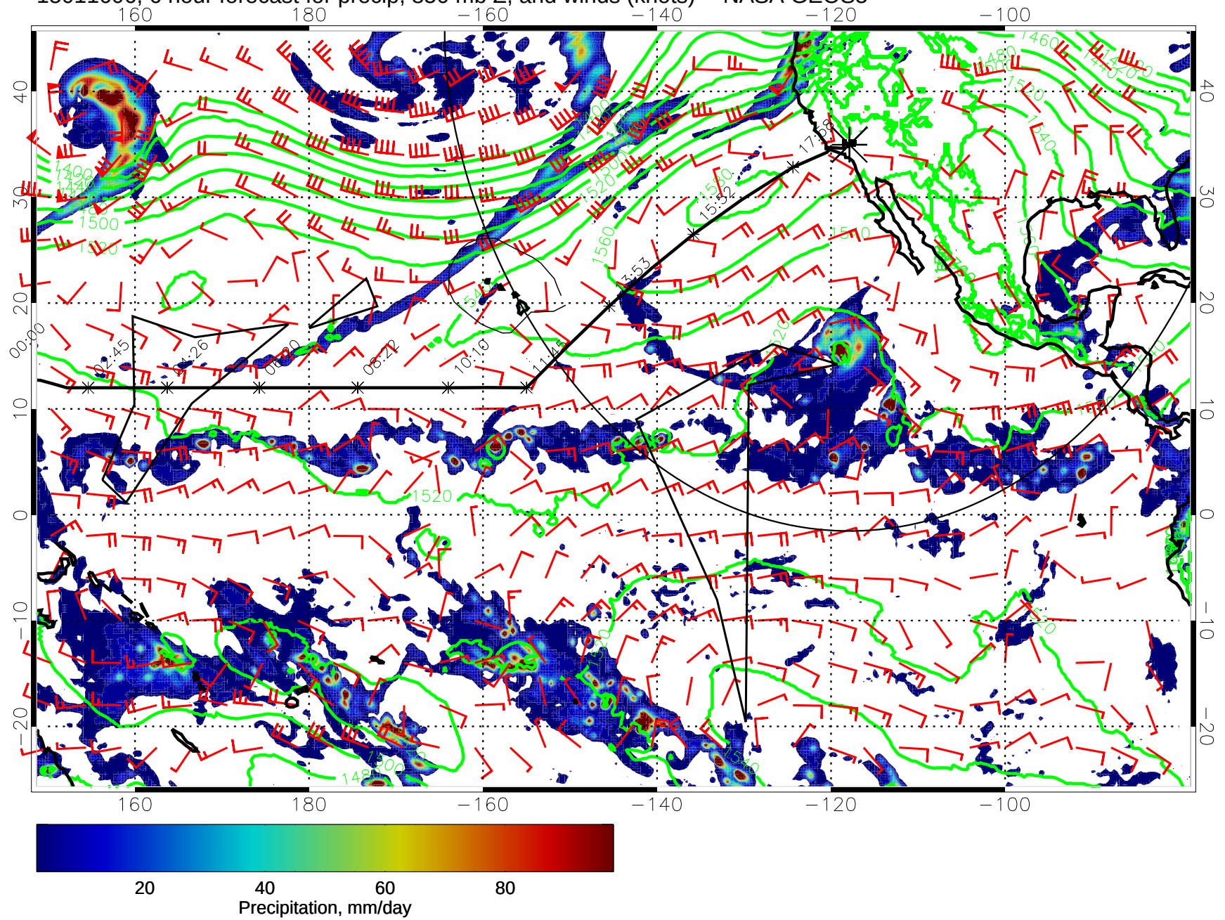
15011606, 6 hour forecast for precip, 850 mb Z, and winds (knots) -- NASA GEOS5
