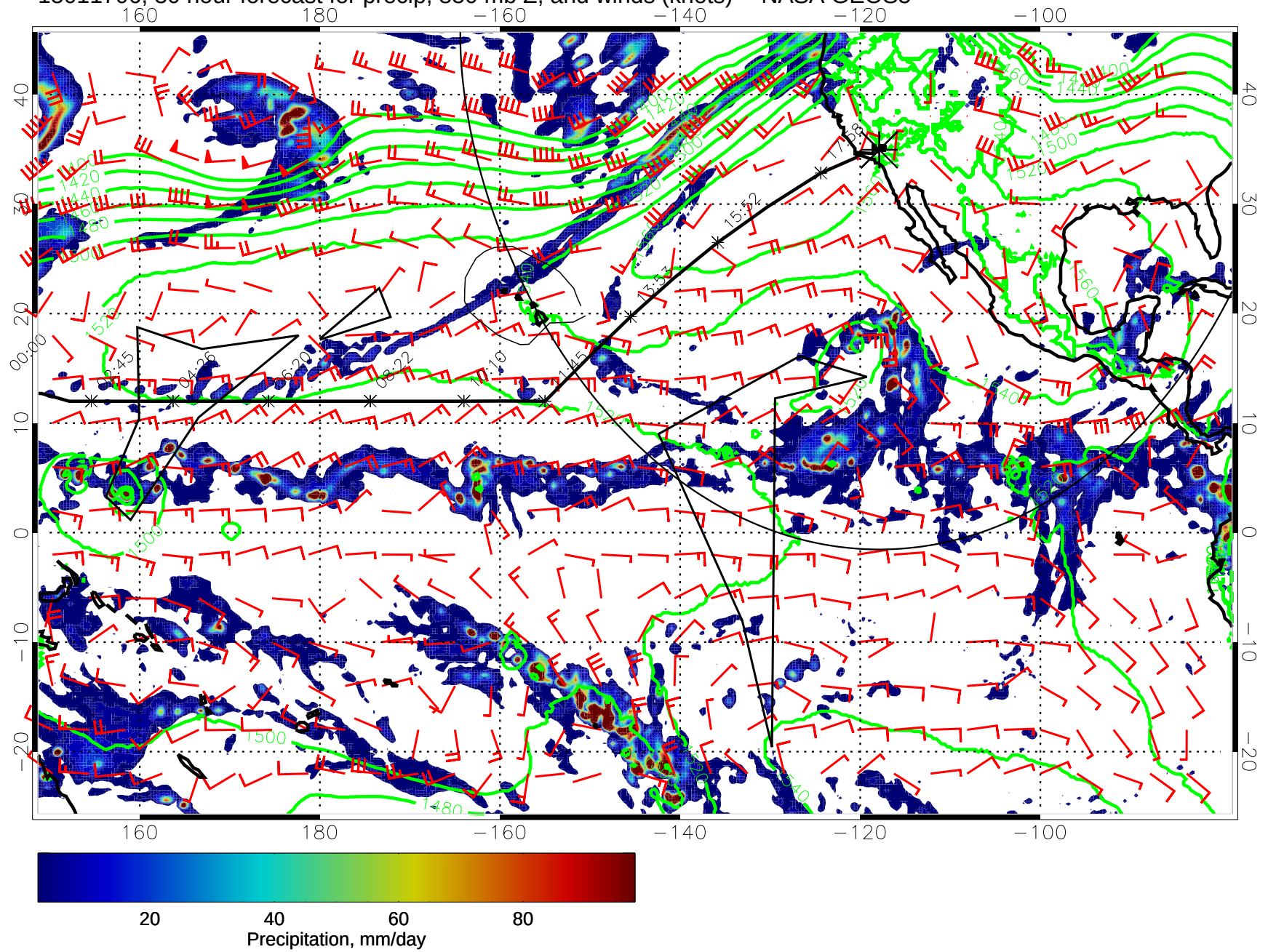
15011706, 30 hour forecast for precip, 850 mb Z, and winds (knots) -- NASA GEOS5
