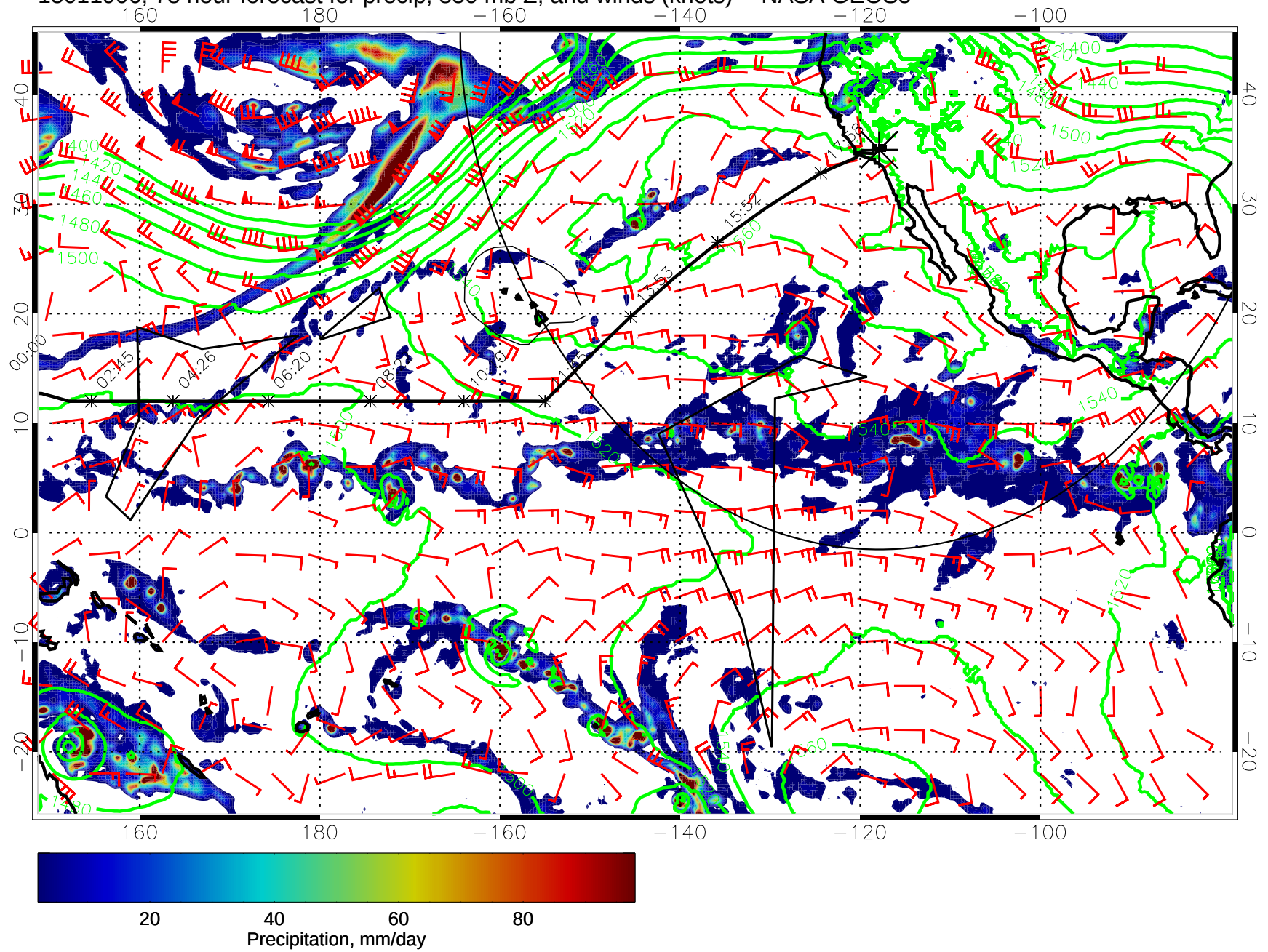
15011906, 78 hour forecast for precip, 850 mb Z, and winds (knots) -- NASA GEOS5
