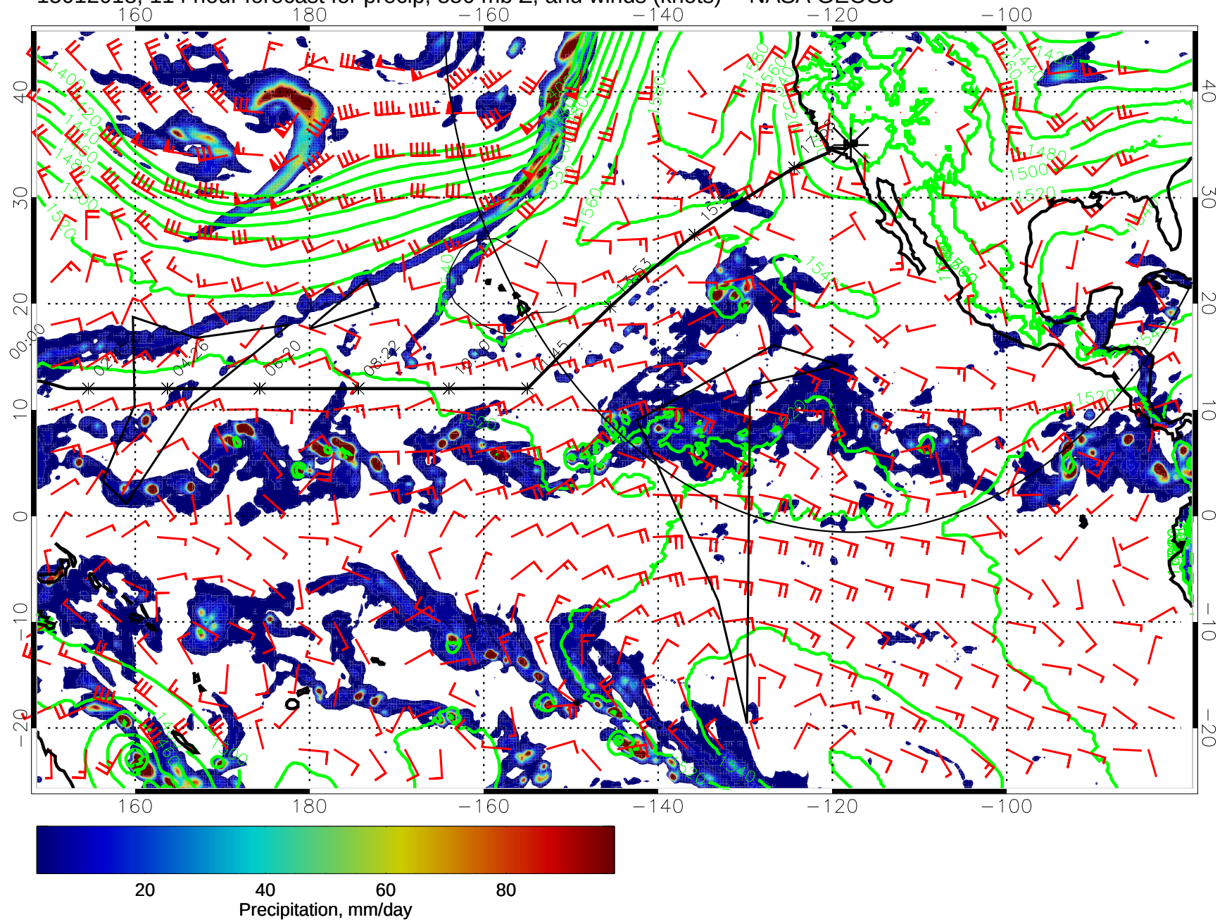
15012018, 114 hour forecast for precip, 850 mb Z, and winds (knots) -- NASA GEOS5
