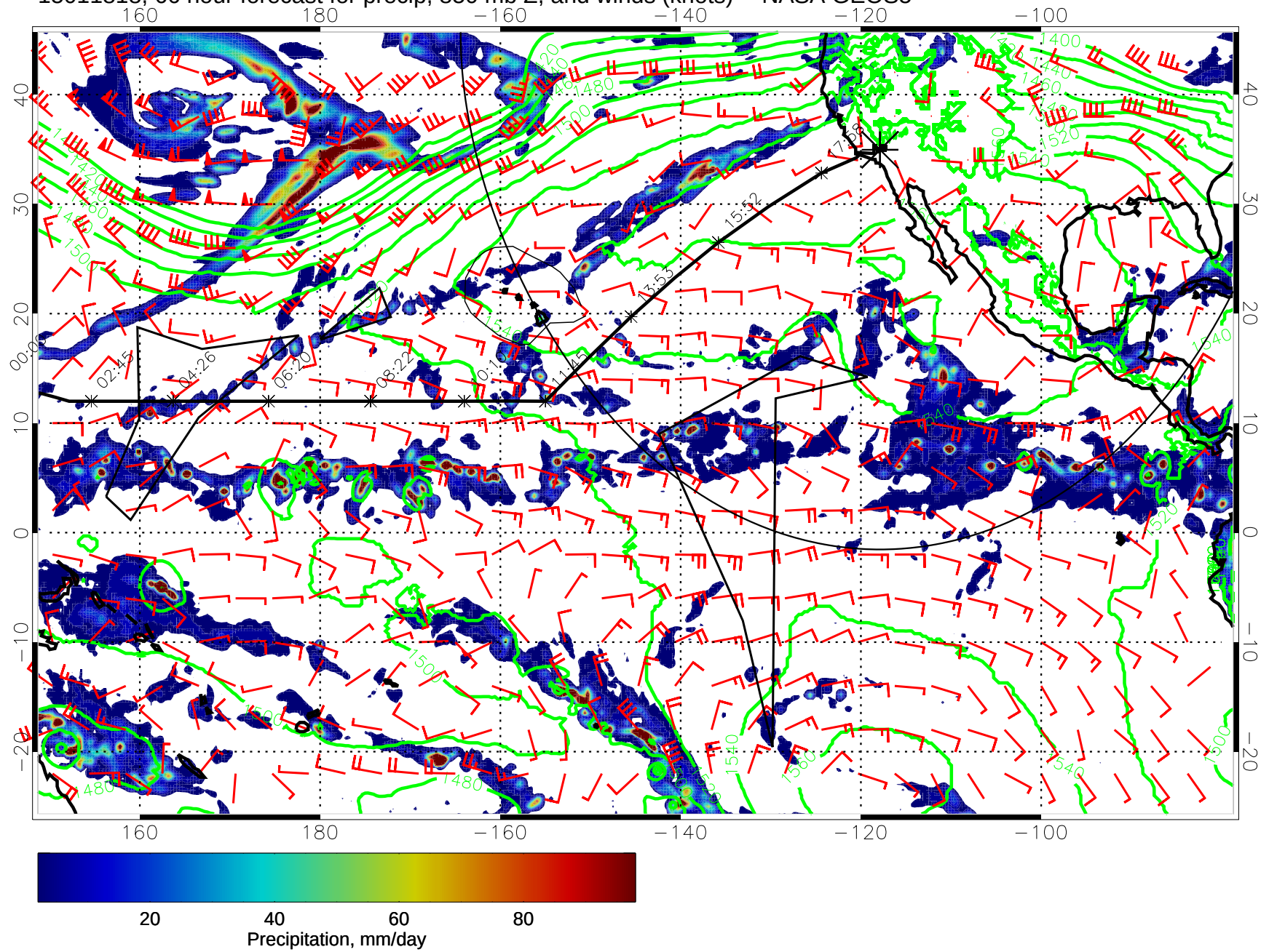
15011818, 66 hour forecast for precip, 850 mb Z, and winds (knots) -- NASA GEOS5
