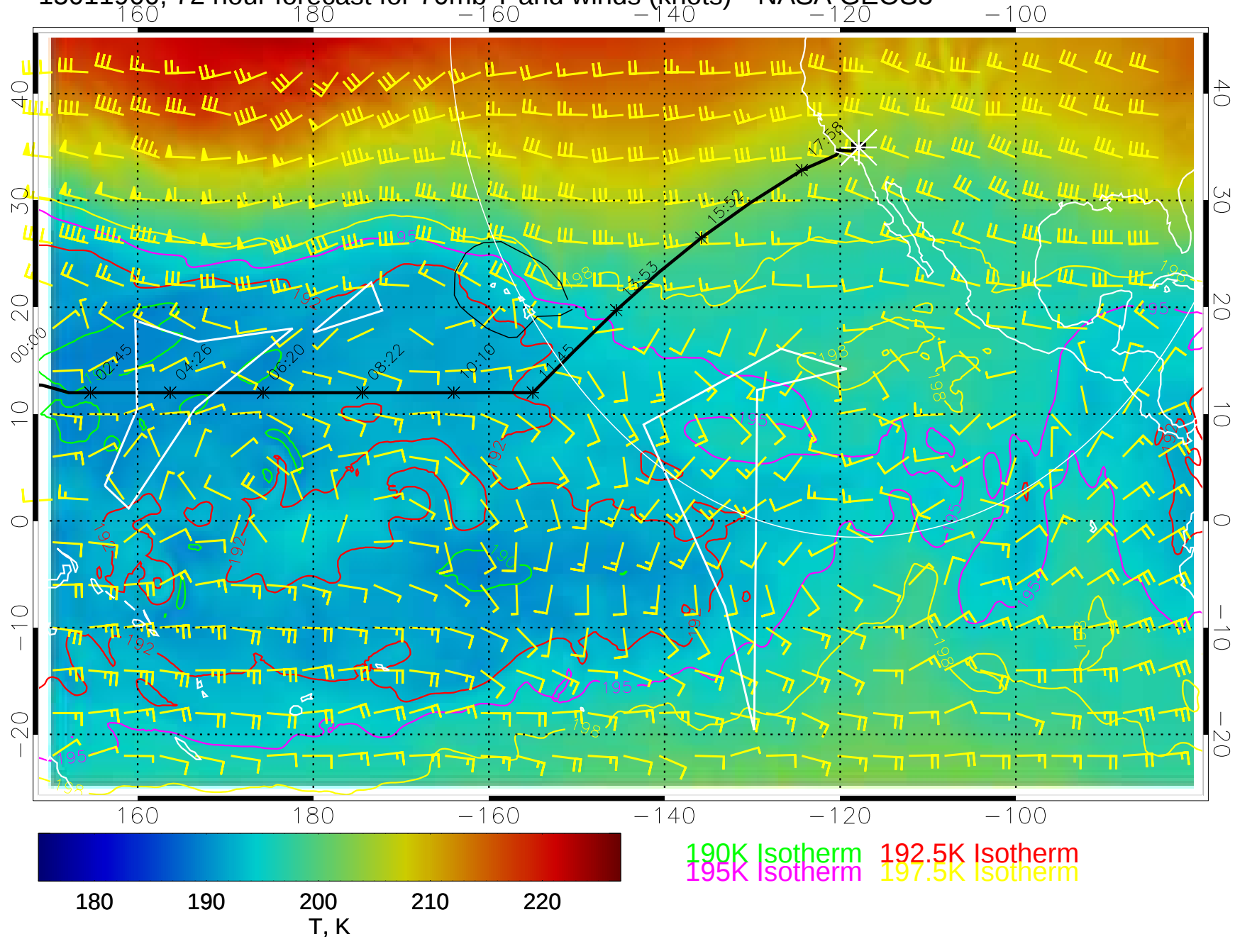
15011900, 72 hour forecast for 70mb T and winds (knots)-- NASA GEOS5
