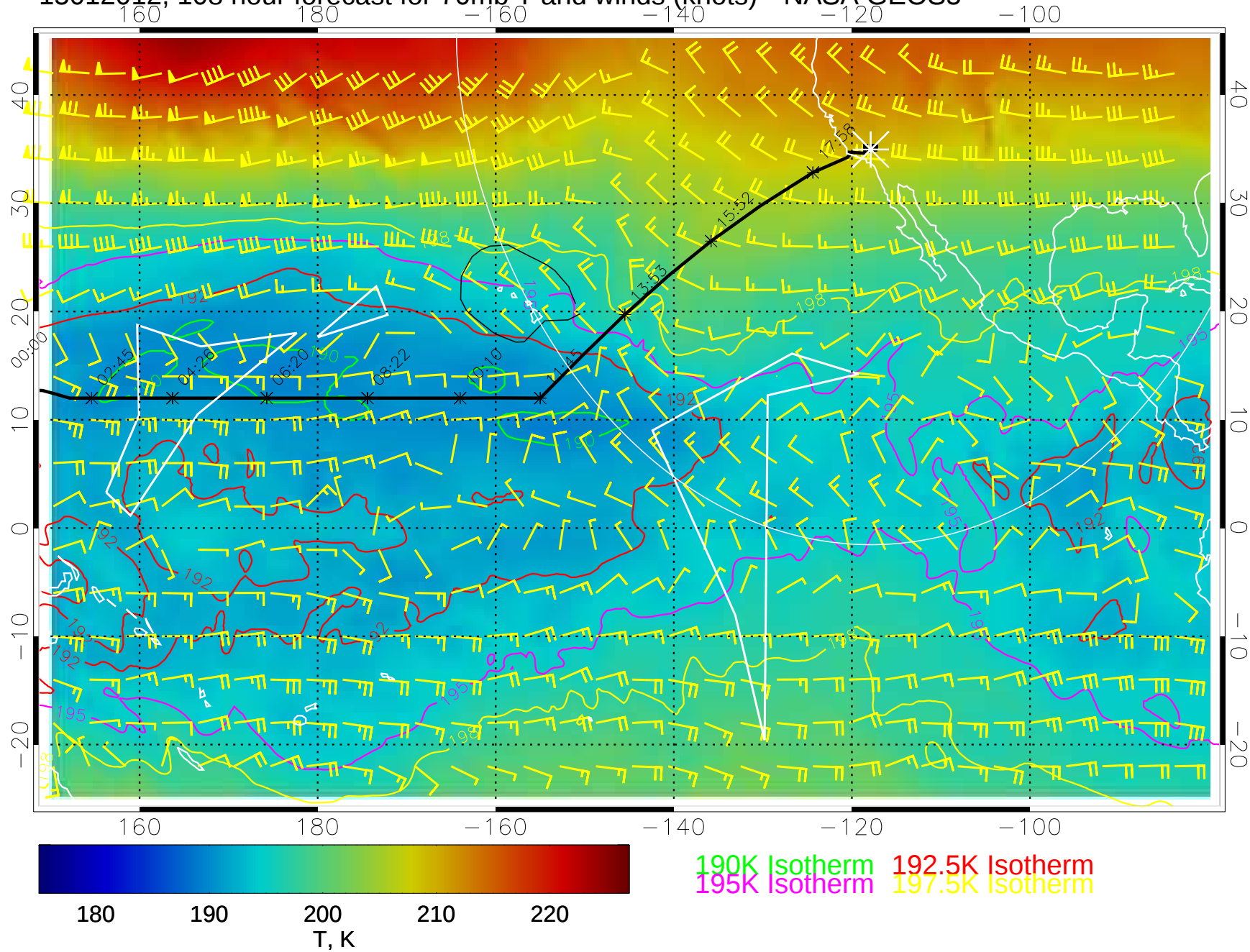
15012012, 108 hour forecast for 70mb T and winds (knots)-- NASA GEOS5
