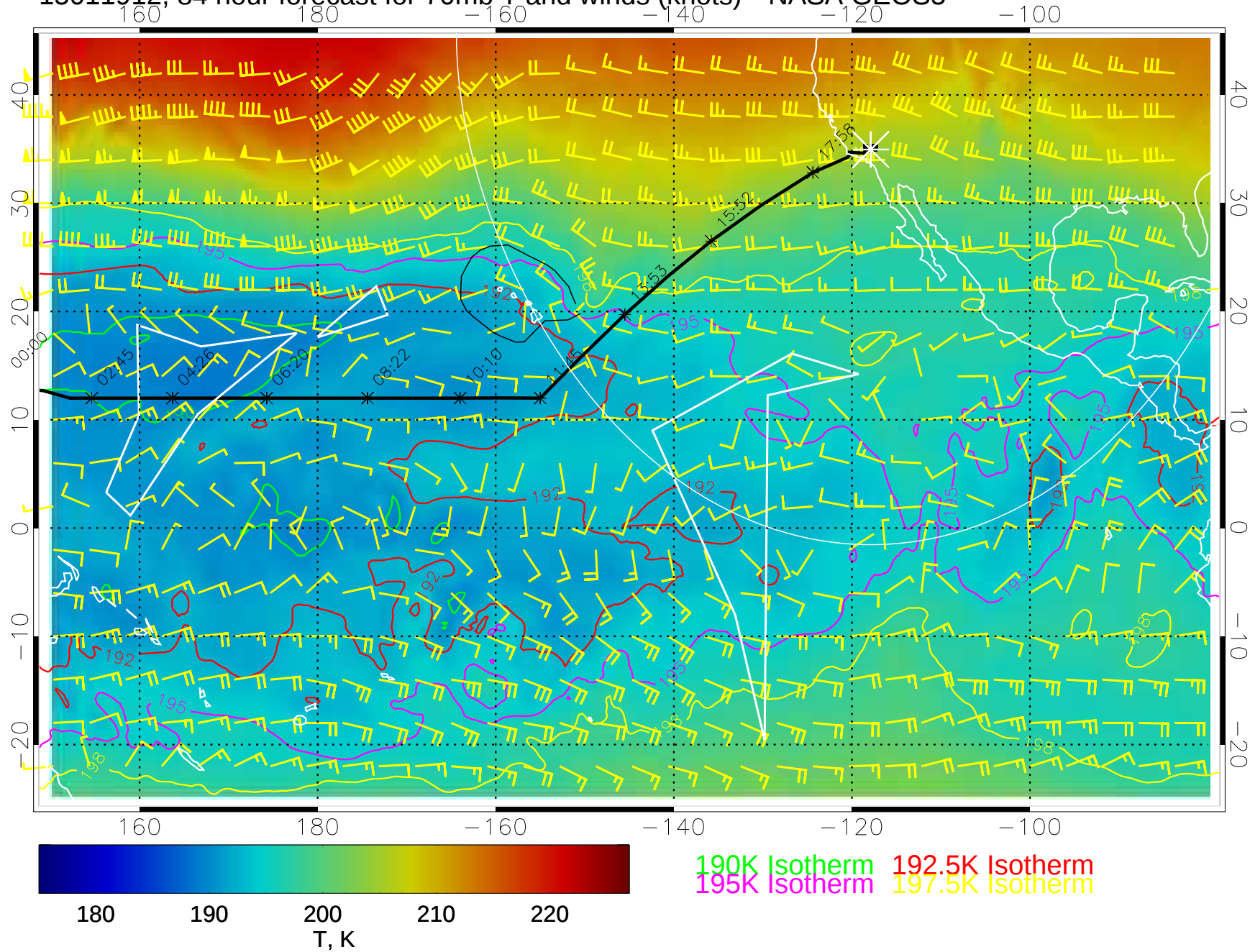
15011912, 84 hour forecast for 70mb T and winds (knots)-- NASA GEOS5
