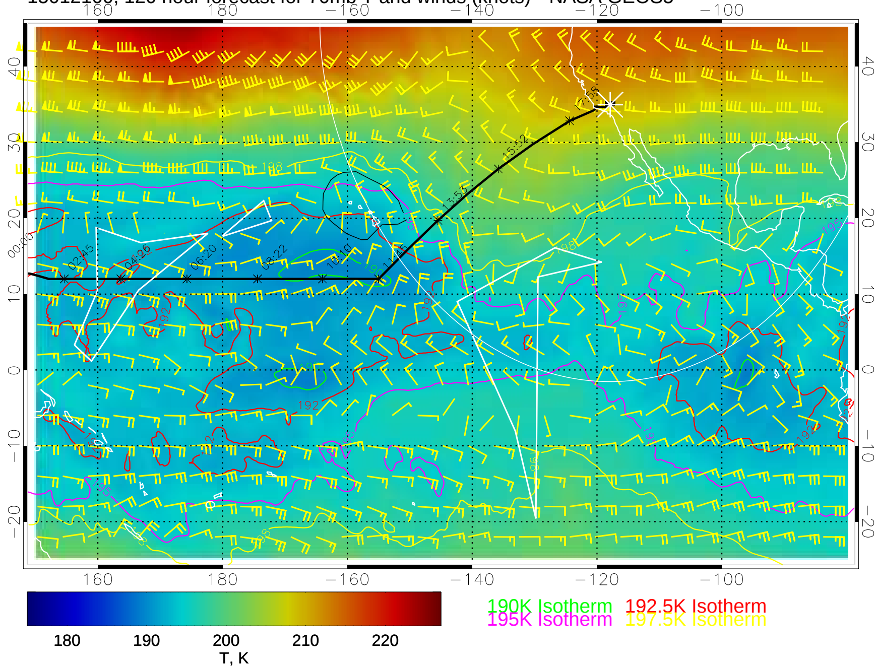
15012100, 120 hour forecast for 70mb T and winds (knots)-- NASA GEOS5
