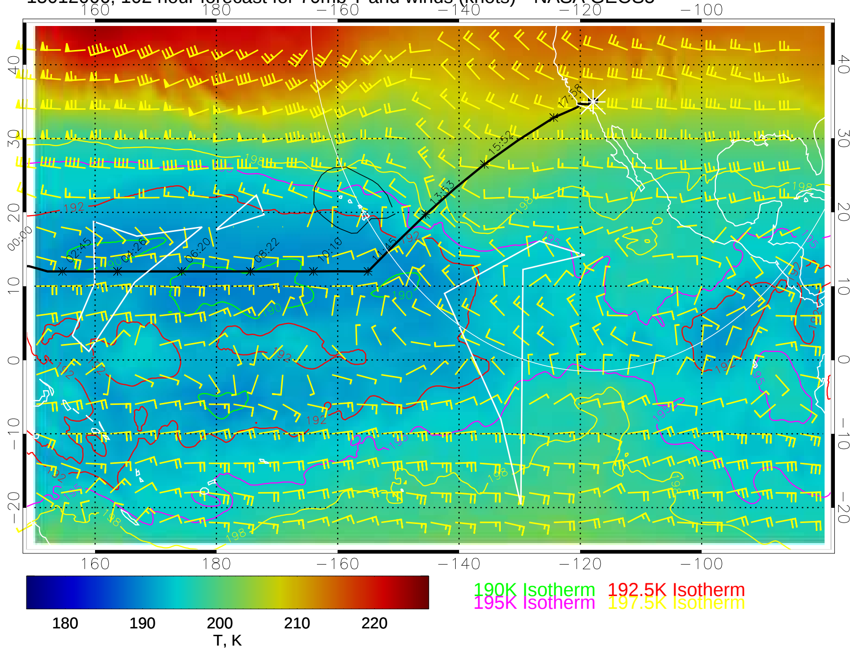
15012006, 102 hour forecast for 70mb T and winds (knots)-- NASA GEOS5
