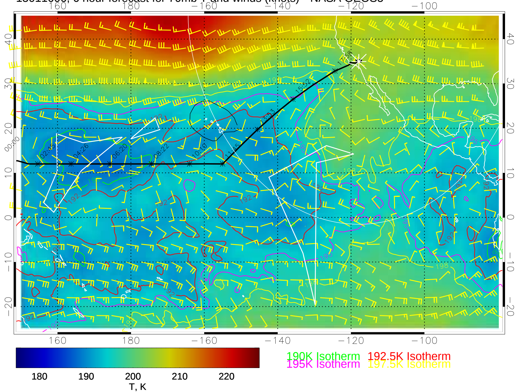
15011606, 6 hour forecast for 70mb T and winds (knots)-- NASA GEOS5
