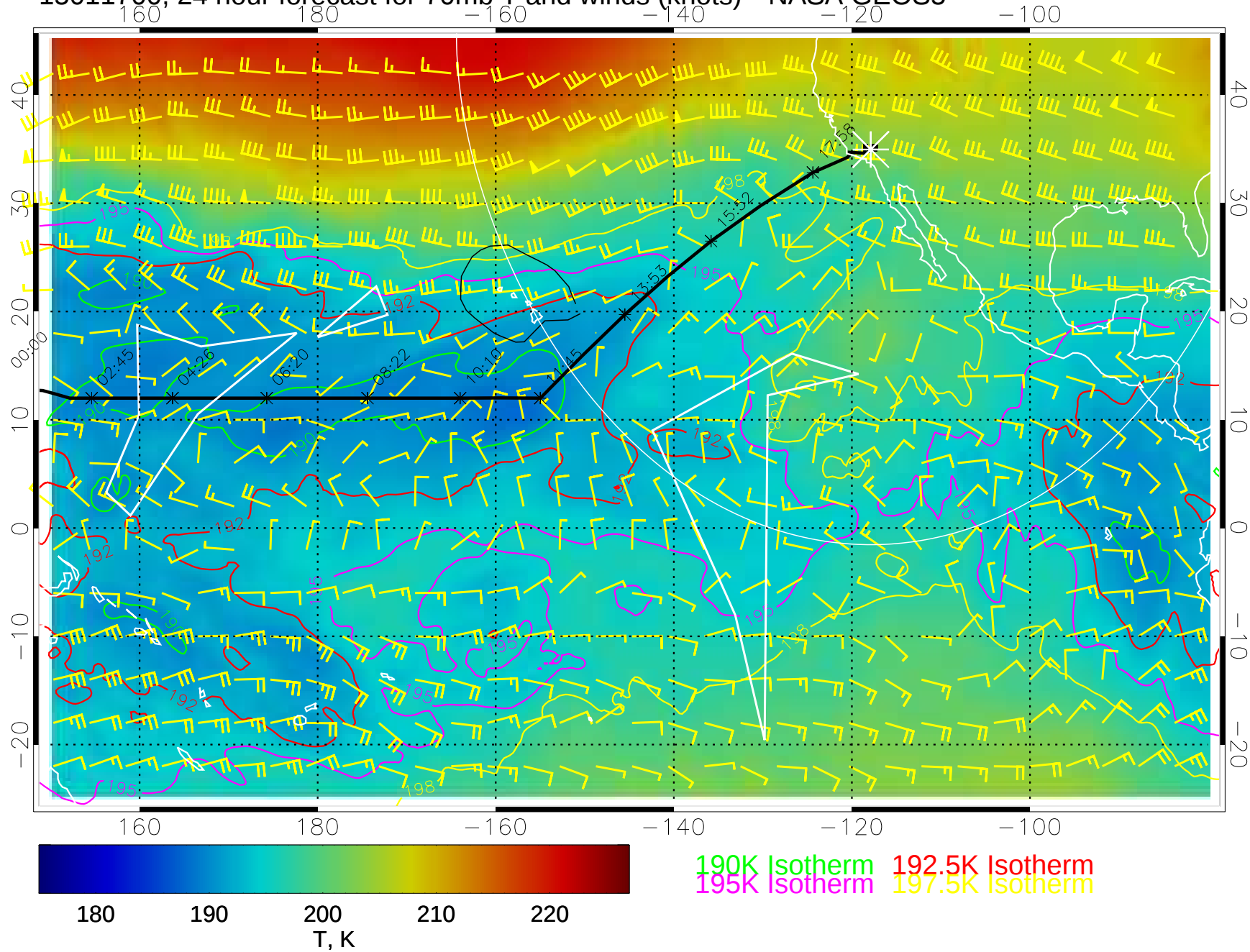
15011700, 24 hour forecast for 70mb T and winds (knots)-- NASA GEOS5
