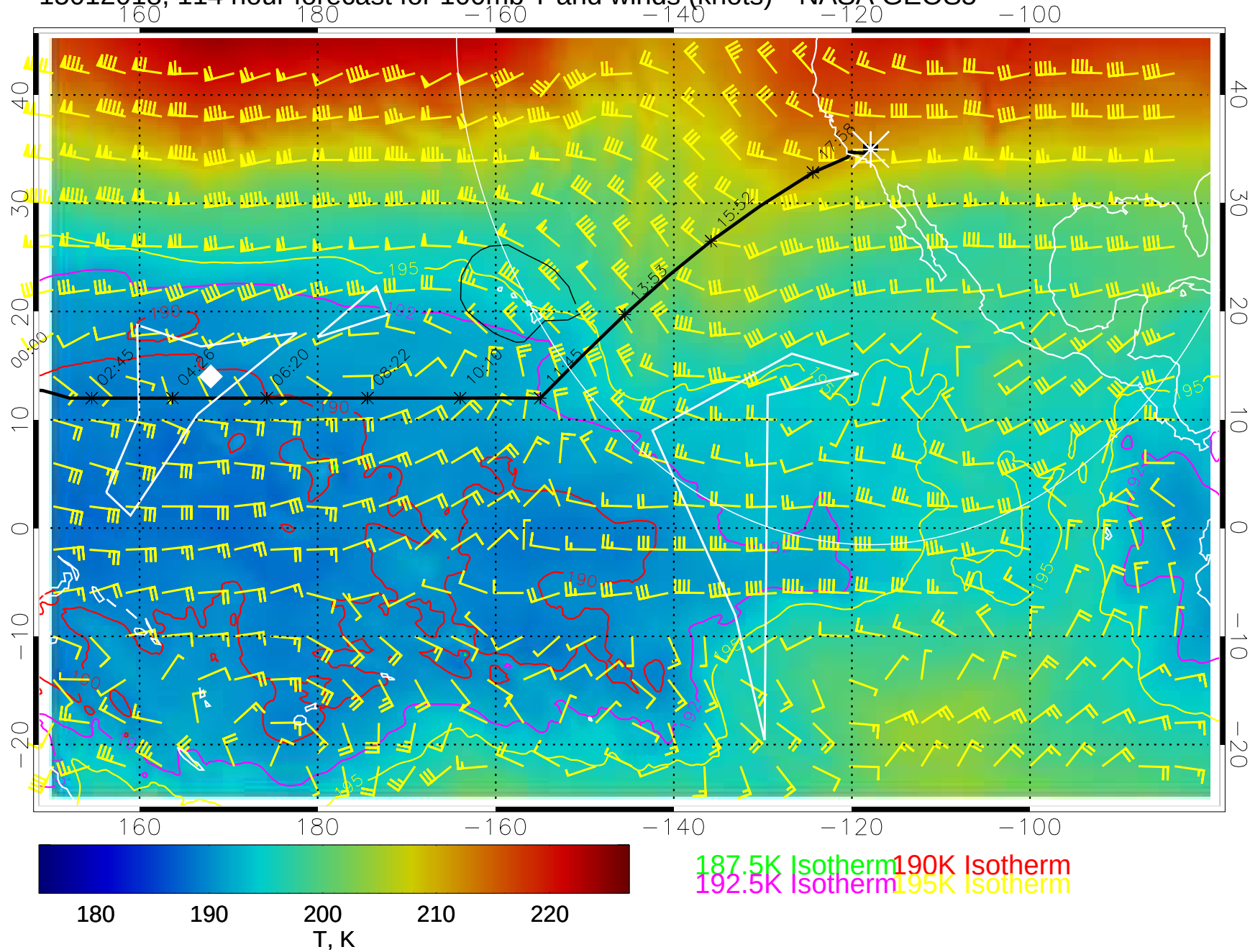
15012018, 114 hour forecast for 100mb T and winds (knots)-- NASA GEOS5
