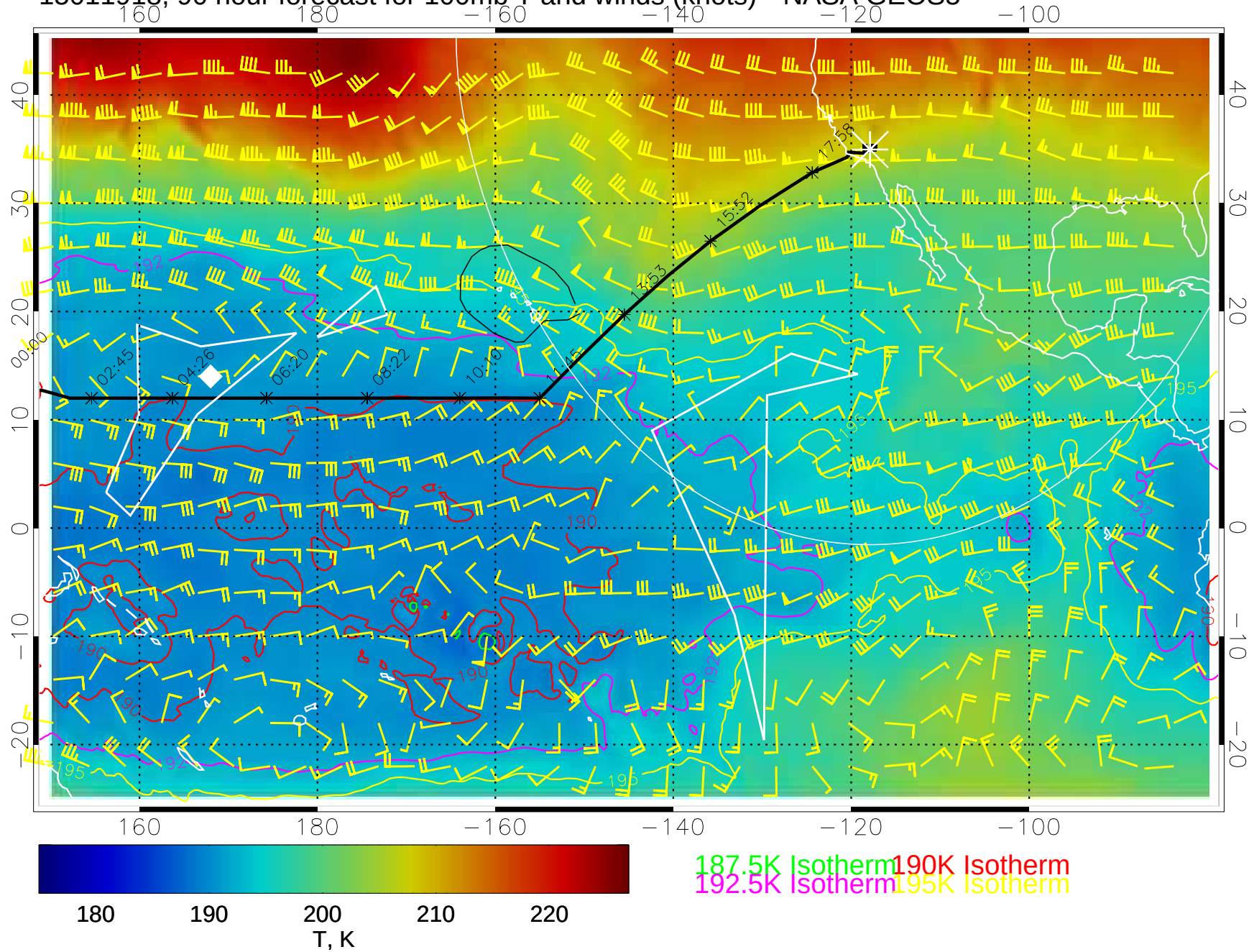
15011918, 90 hour forecast for 100mb T and winds (knots)-- NASA GEOS5
