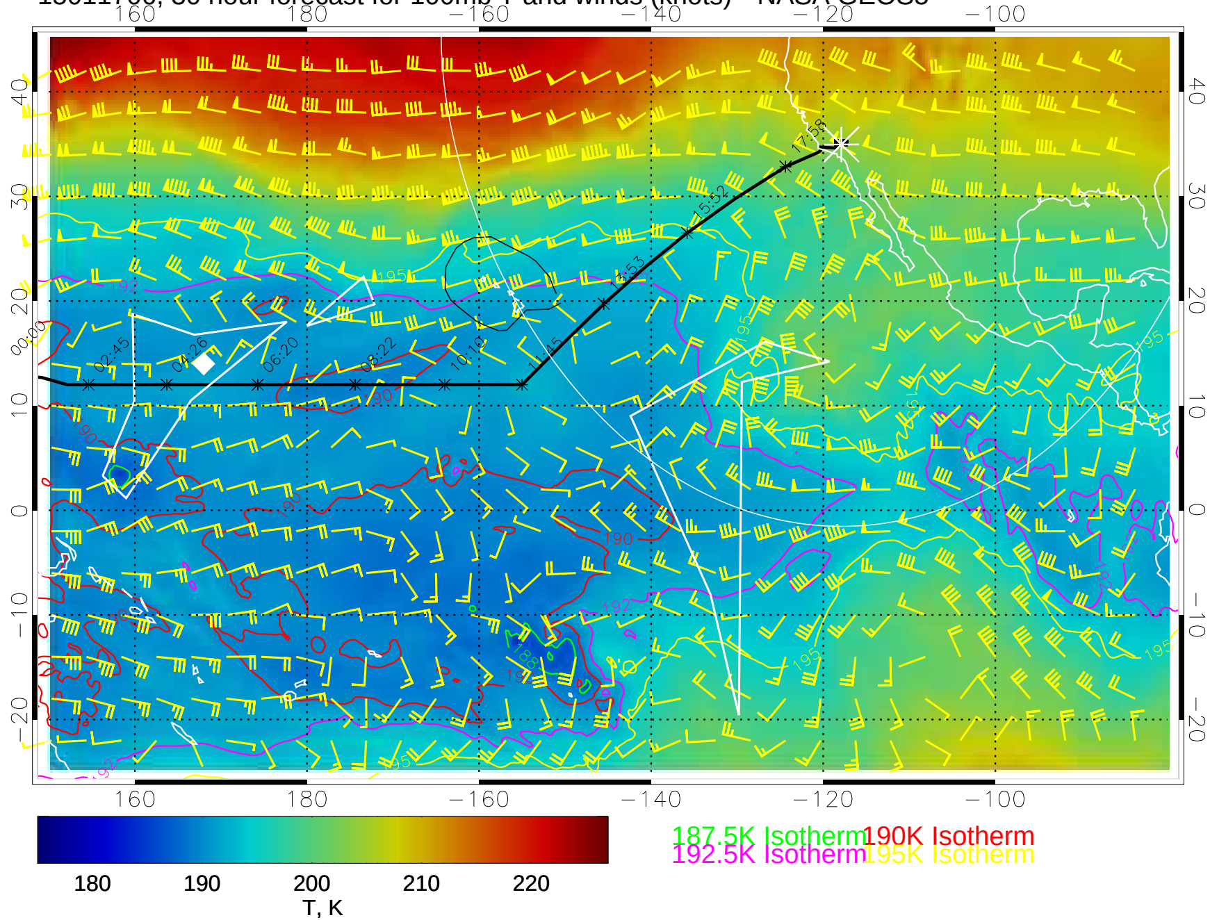
15011706, 30 hour forecast for 100mb T and winds (knots)-- NASA GEOS5
