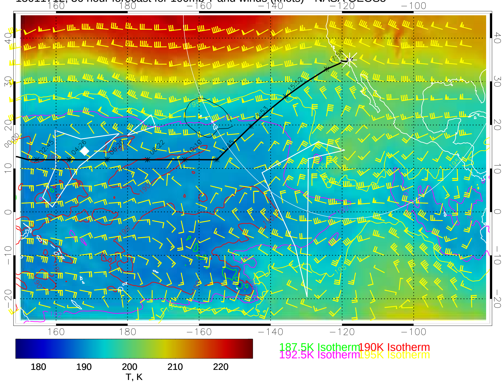
15011712, 36 hour forecast for 100mb T and winds (knots)-- NASA GEOS5
