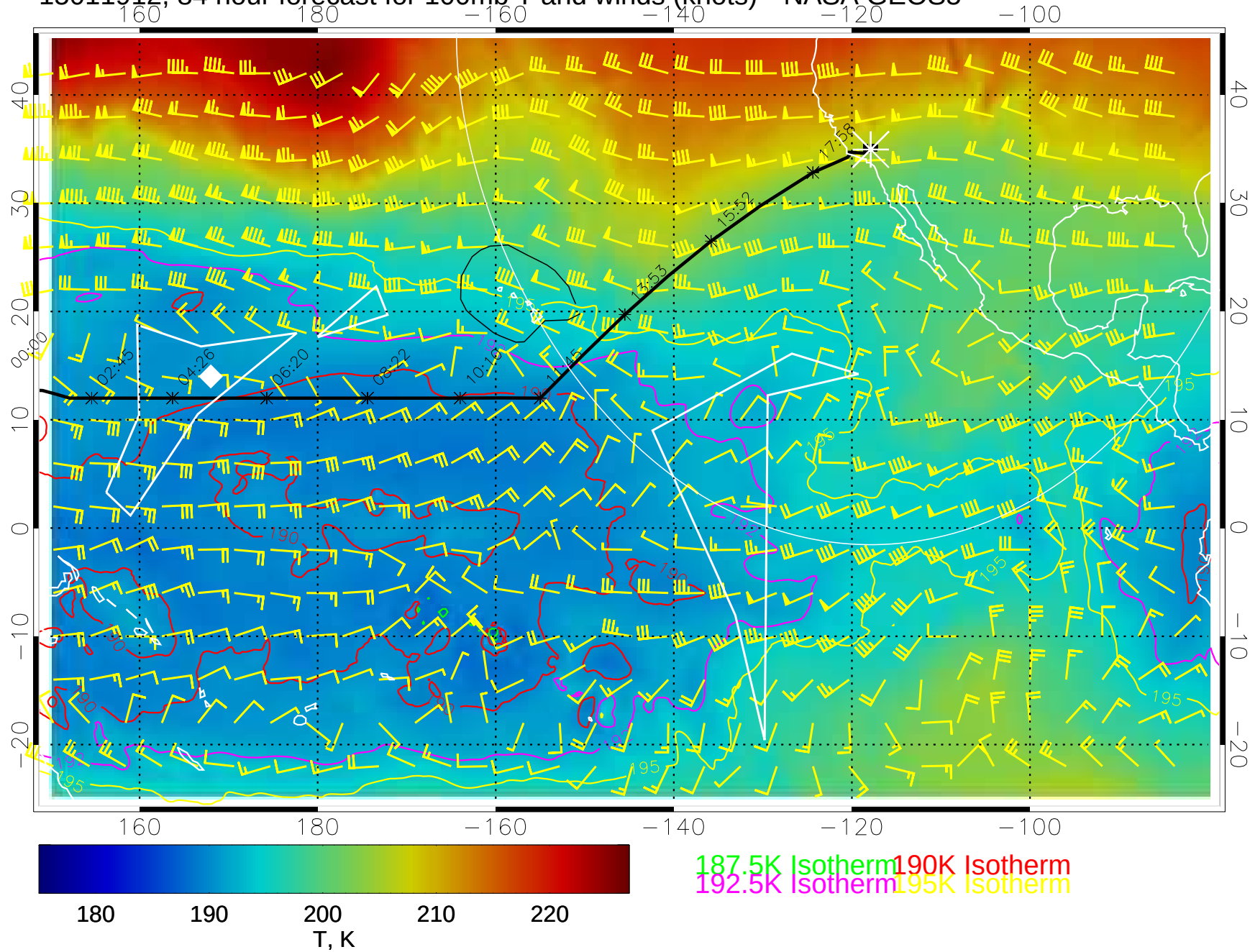
15011912, 84 hour forecast for 100mb T and winds (knots)-- NASA GEOS5
