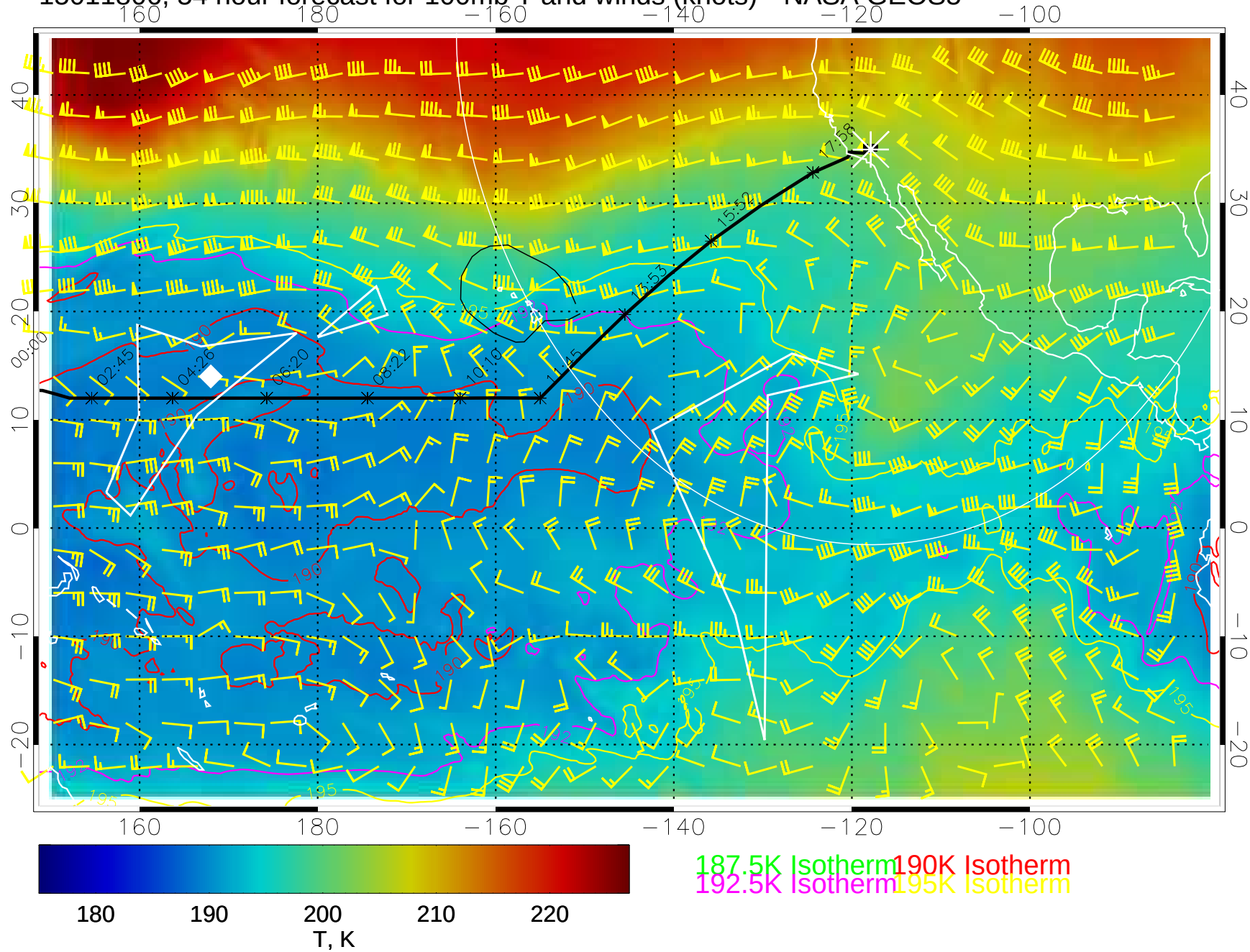
15011806, 54 hour forecast for 100mb T and winds (knots)-- NASA GEOS5
