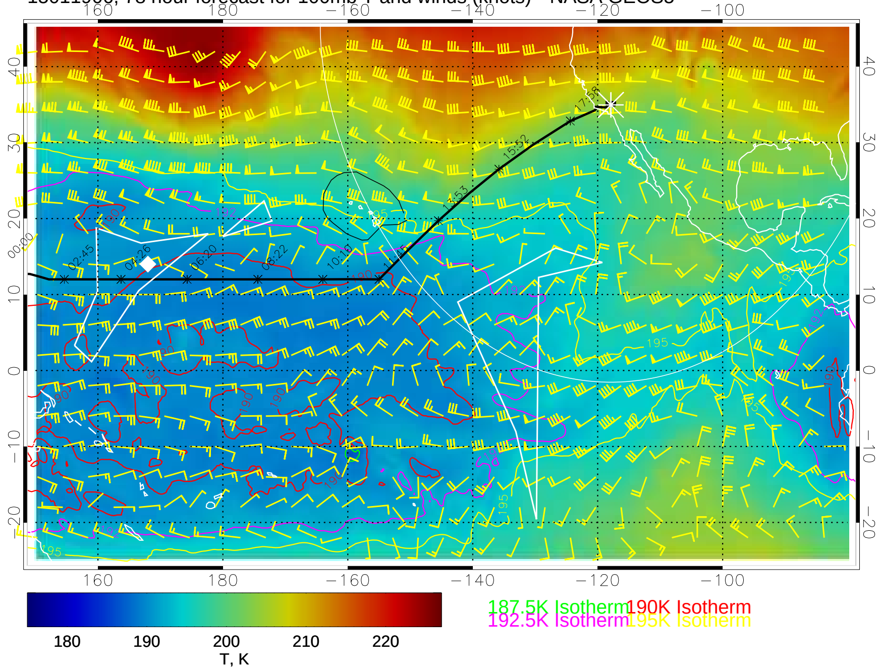
15011906, 78 hour forecast for 100mb T and winds (knots)-- NASA GEOS5
