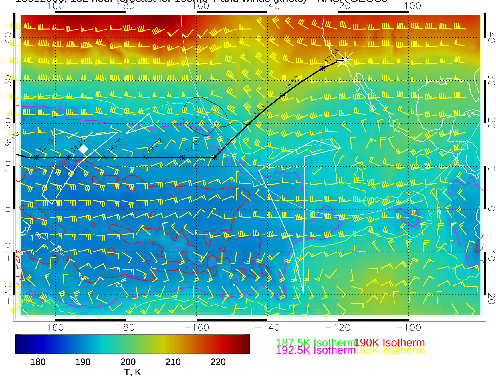
15012006, 102 hour forecast for 100mb T and winds (knots)-- NASA GEOS5
