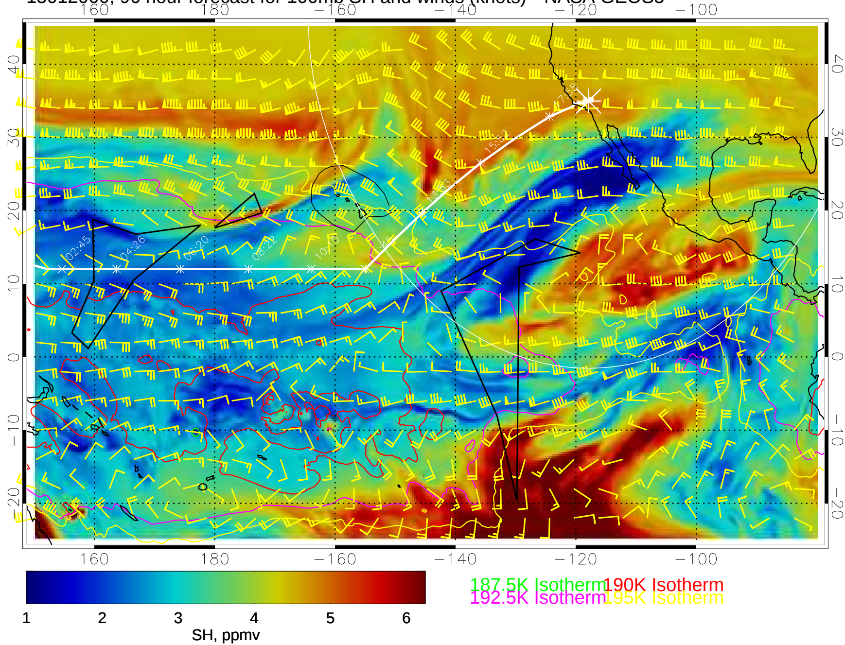
15012000, 96 hour forecast for 100mb SH and winds (knots)-- NASA GEOS5
