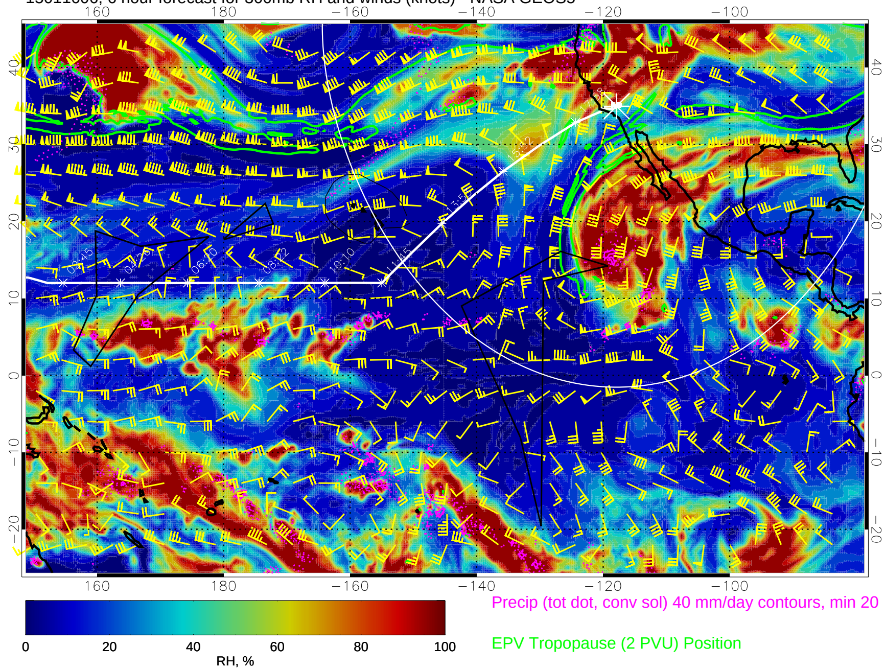
15011606, 6 hour forecast for 300mb RH and winds (knots) - NASA GEOS5
