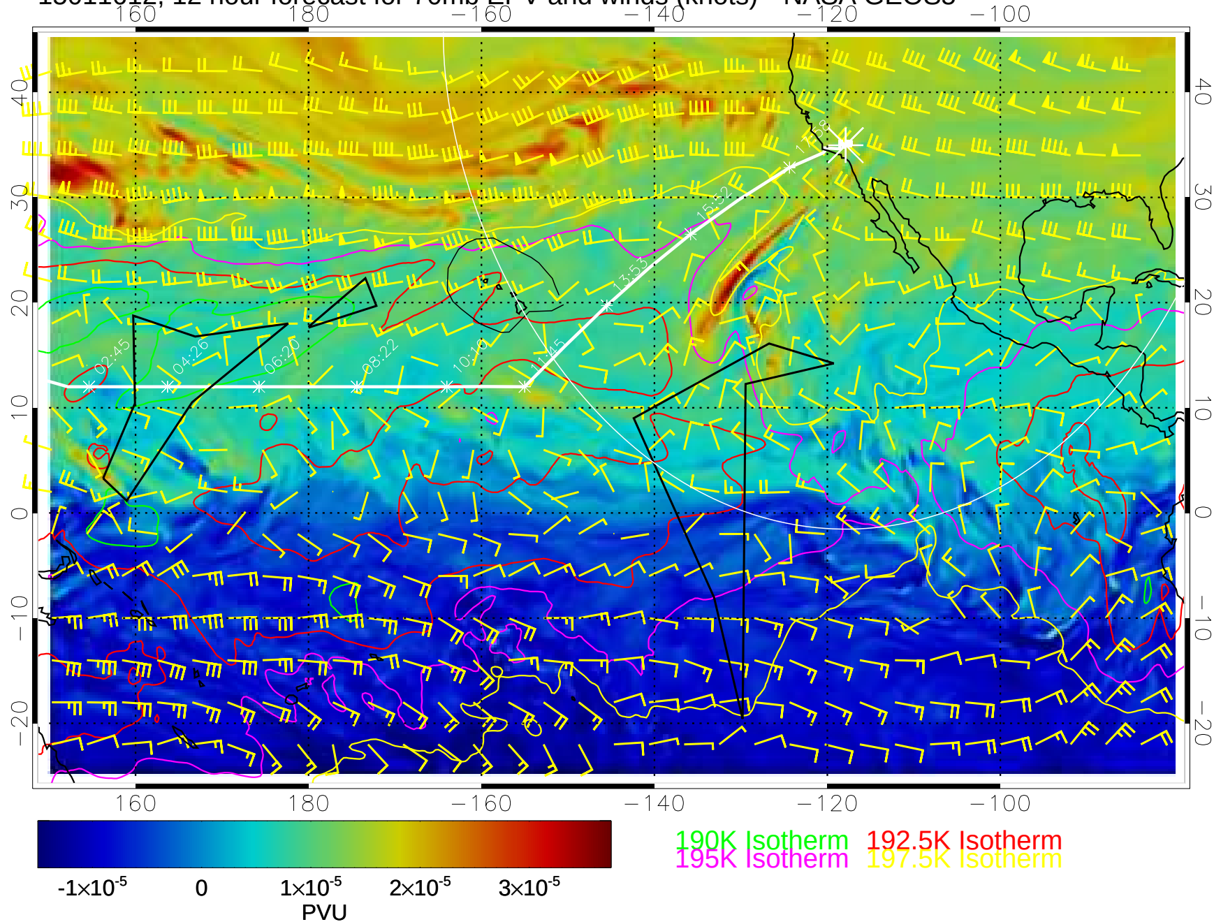
15011612, 12 hour forecast for 70mb EPV and winds (knots)-- NASA GEOS5
