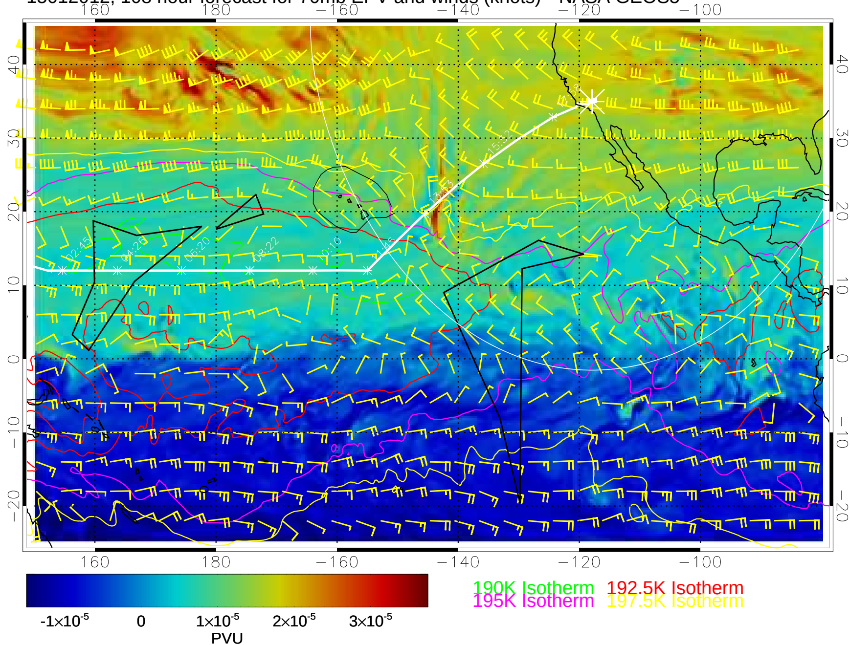
15012012, 108 hour forecast for 70mb EPV and winds (knots)-- NASA GEOS5
