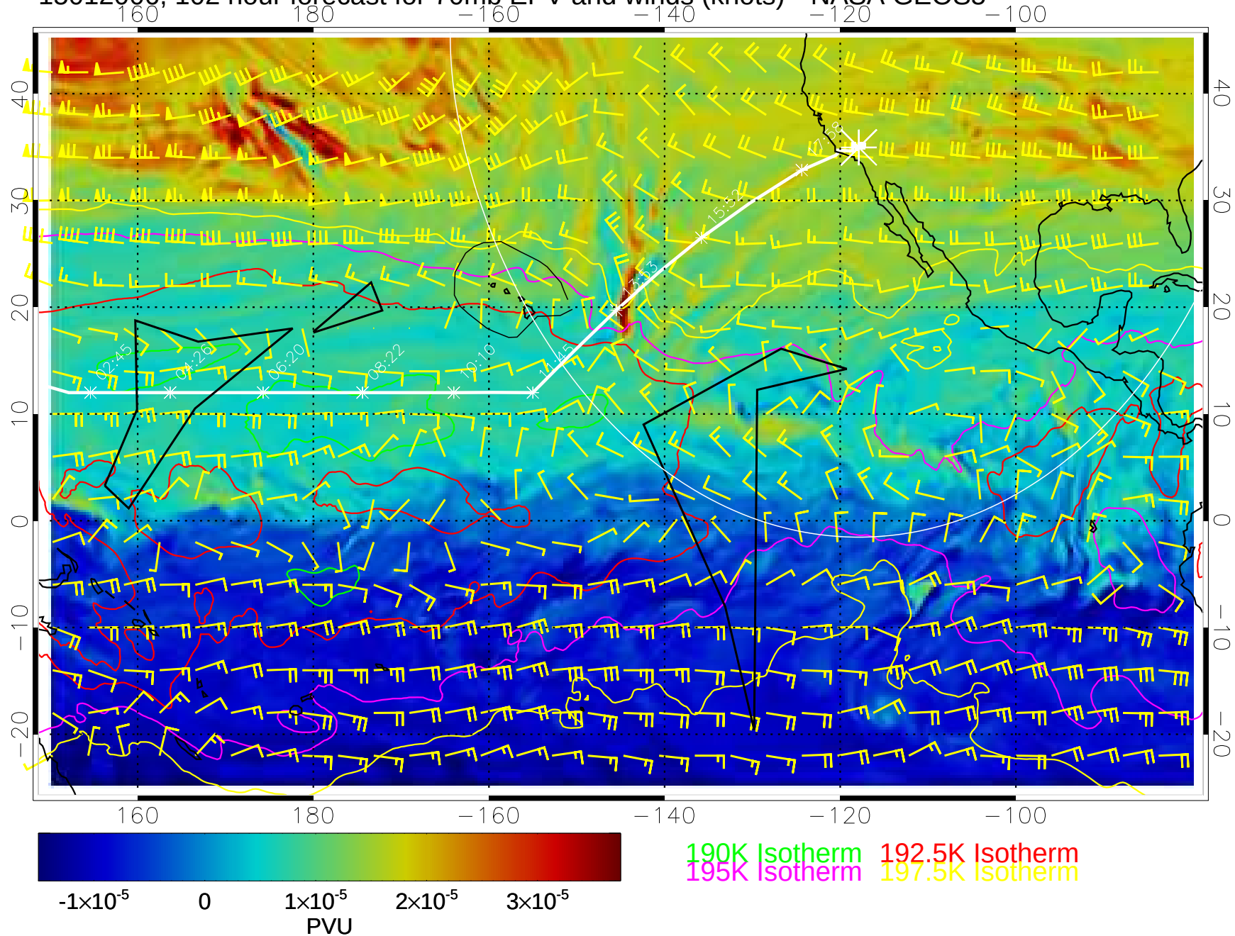
15012006, 102 hour forecast for 70mb EPV and winds (knots)-- NASA GEOS5
