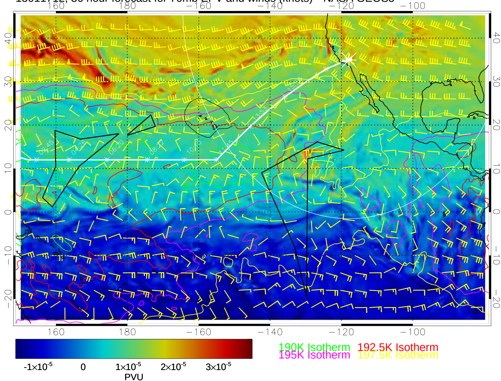
15011712, 36 hour forecast for 70mb EPV and winds (knots)-- NASA GEOS5
