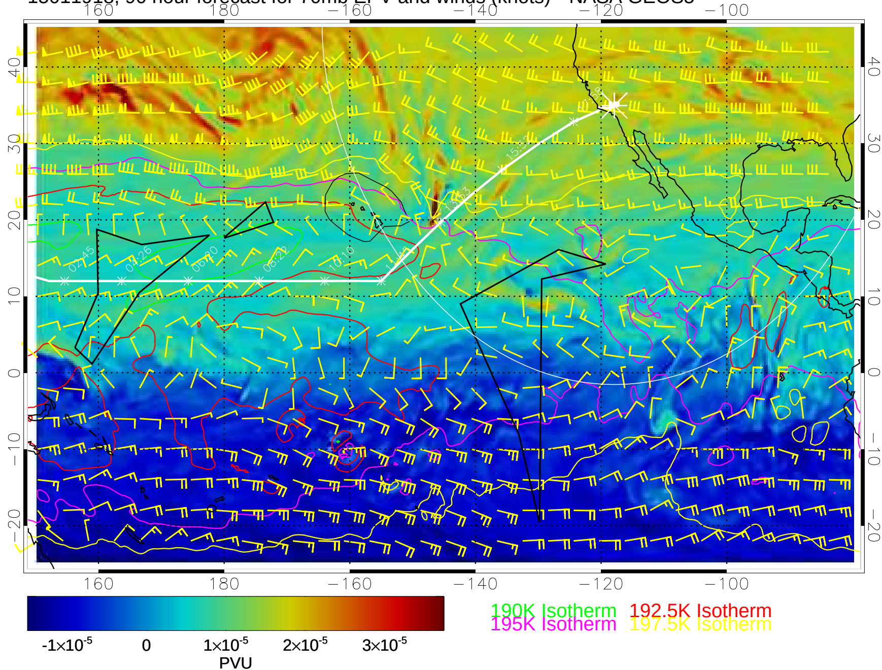
15011918, 90 hour forecast for 70mb EPV and winds (knots)-- NASA GEOS5
