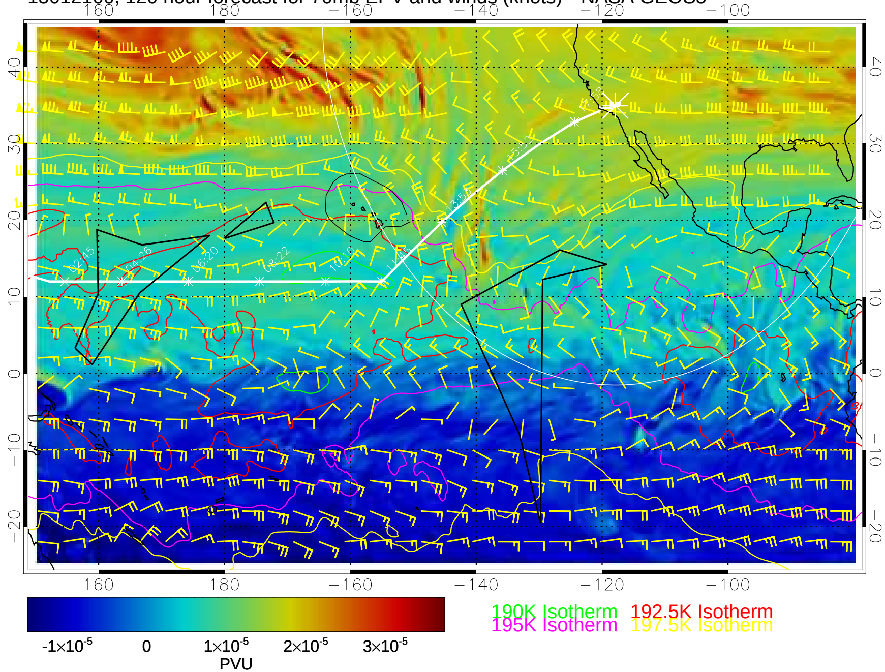
15012100, 120 hour forecast for 70mb EPV and winds (knots)-- NASA GEOS5
