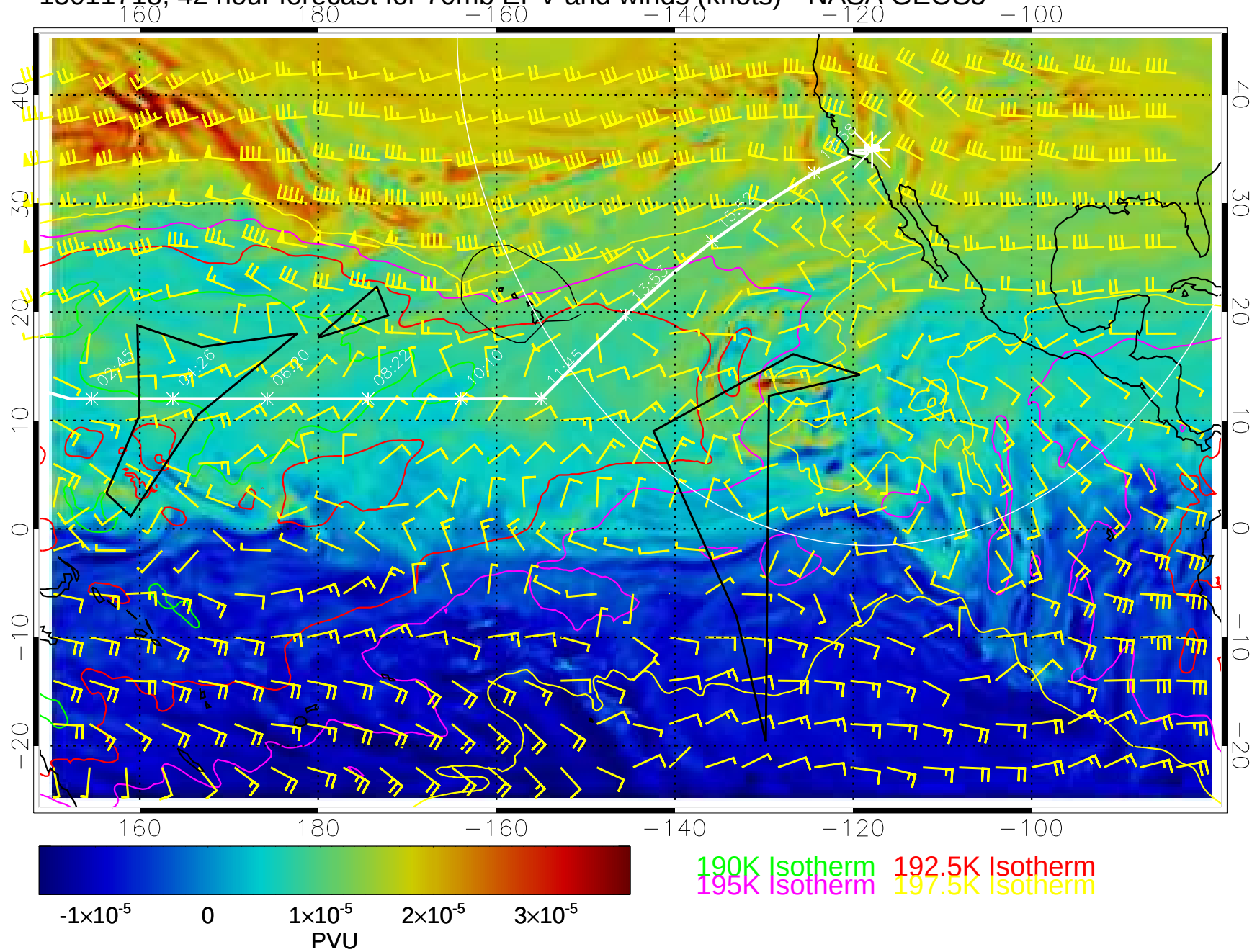
15011718, 42 hour forecast for 70mb EPV and winds (knots)-- NASA GEOS5
