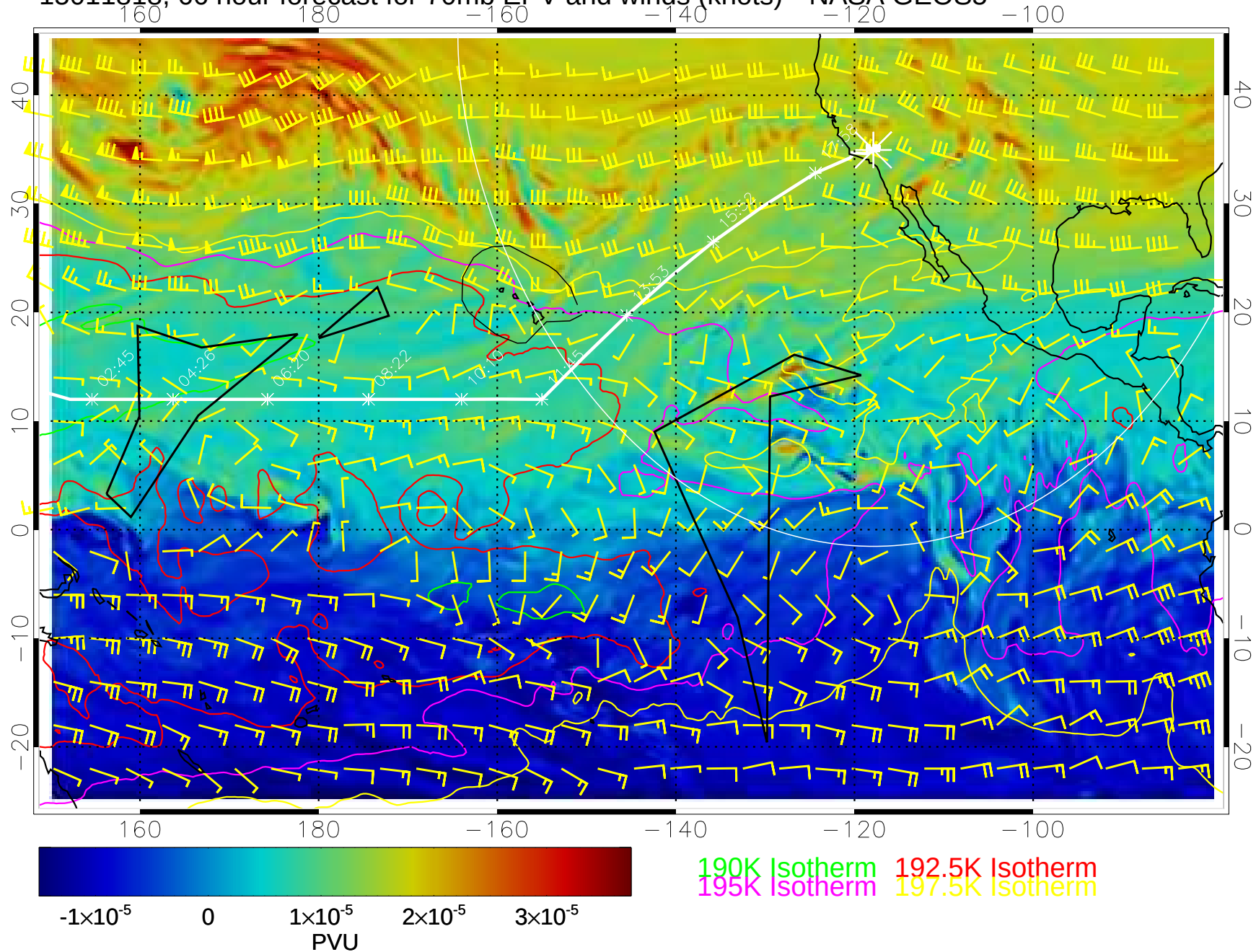
15011818, 66 hour forecast for 70mb EPV and winds (knots)-- NASA GEOS5
