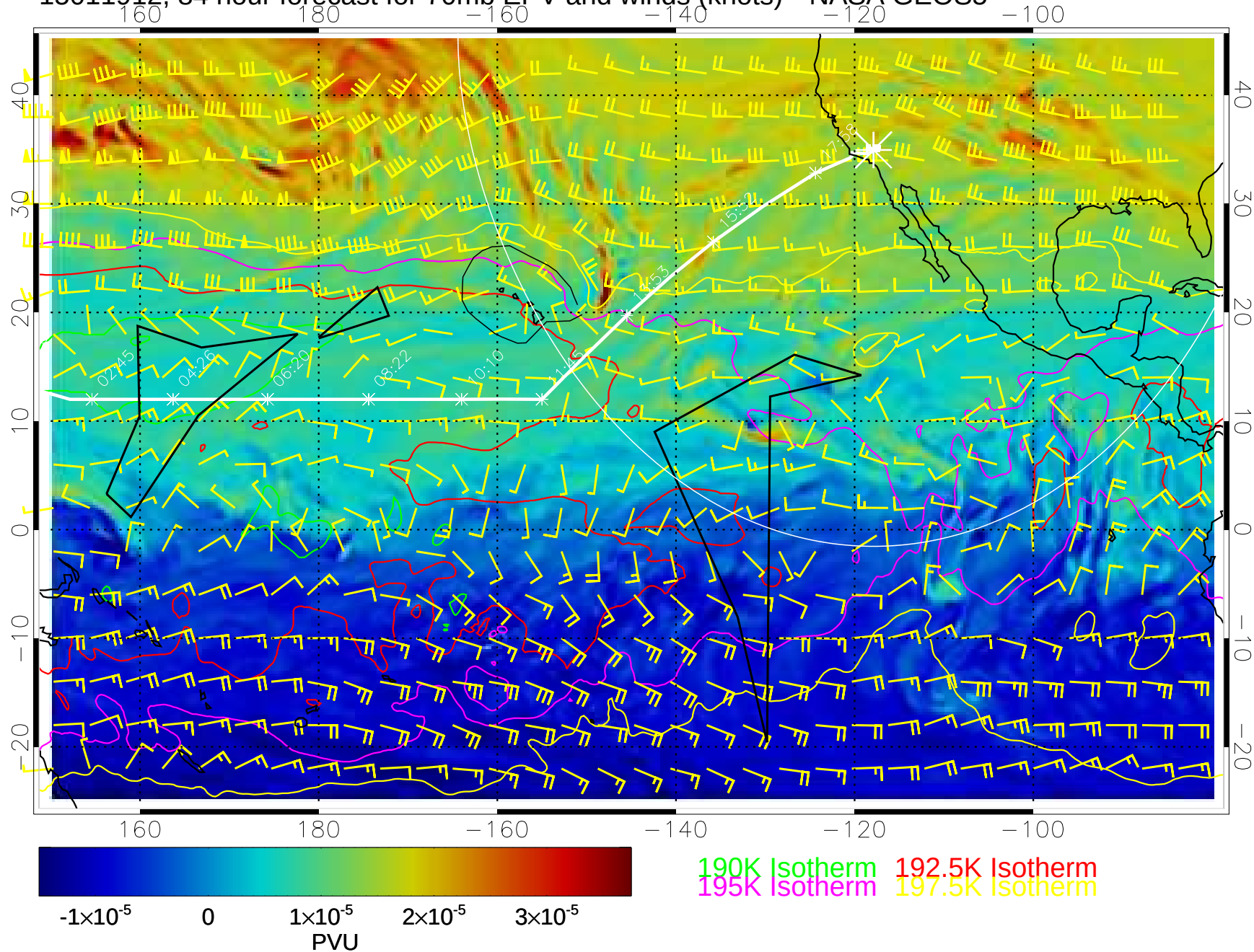
15011912, 84 hour forecast for 70mb EPV and winds (knots)-- NASA GEOS5
