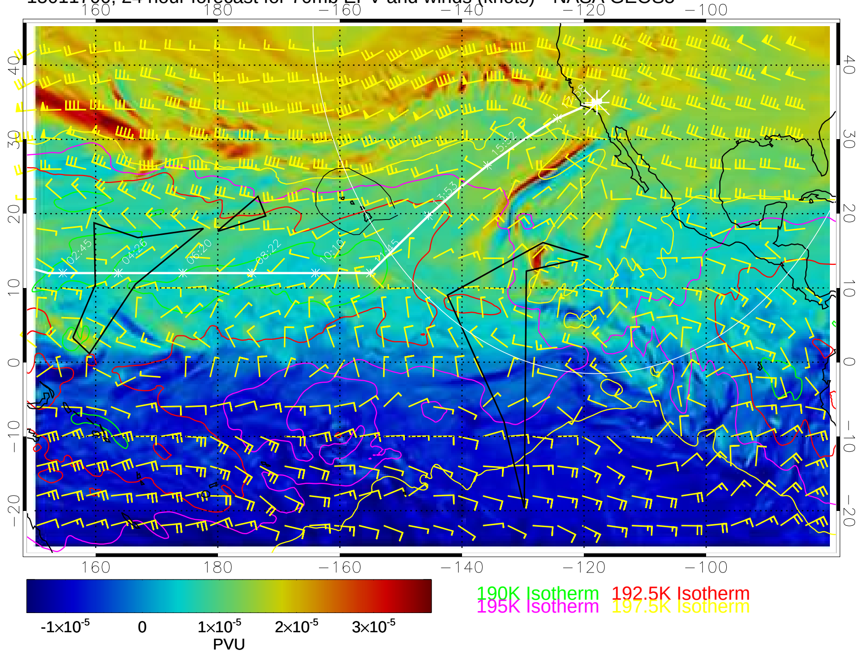
15011700, 24 hour forecast for 70mb EPV and winds (knots)-- NASA GEOS5
