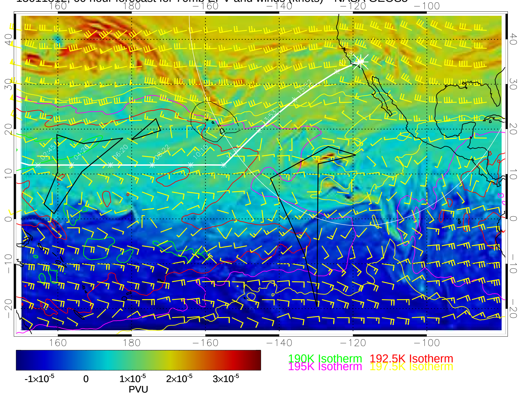
15011812, 60 hour forecast for 70mb EPV and winds (knots)-- NASA GEOS5
