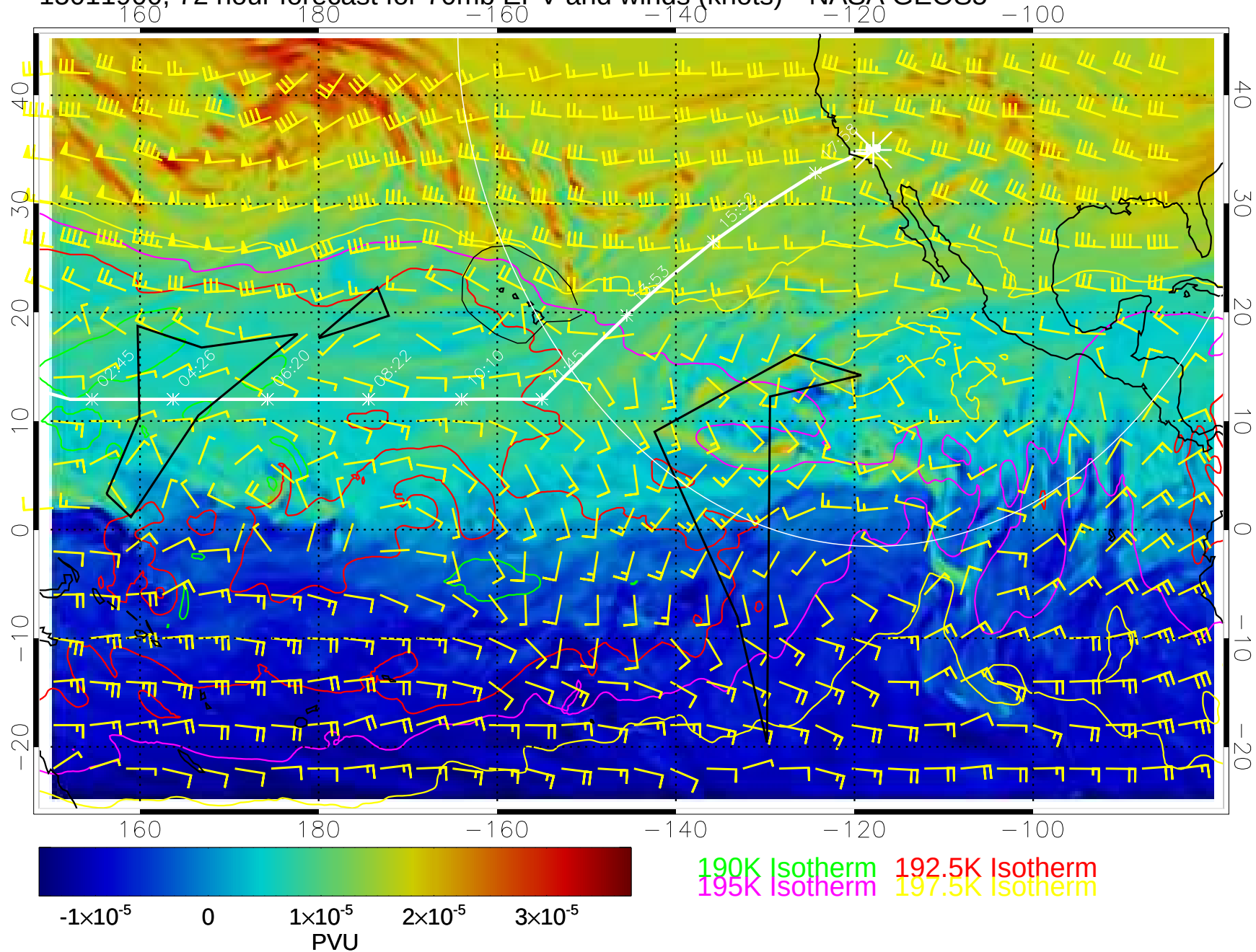
15011900, 72 hour forecast for 70mb EPV and winds (knots)-- NASA GEOS5
