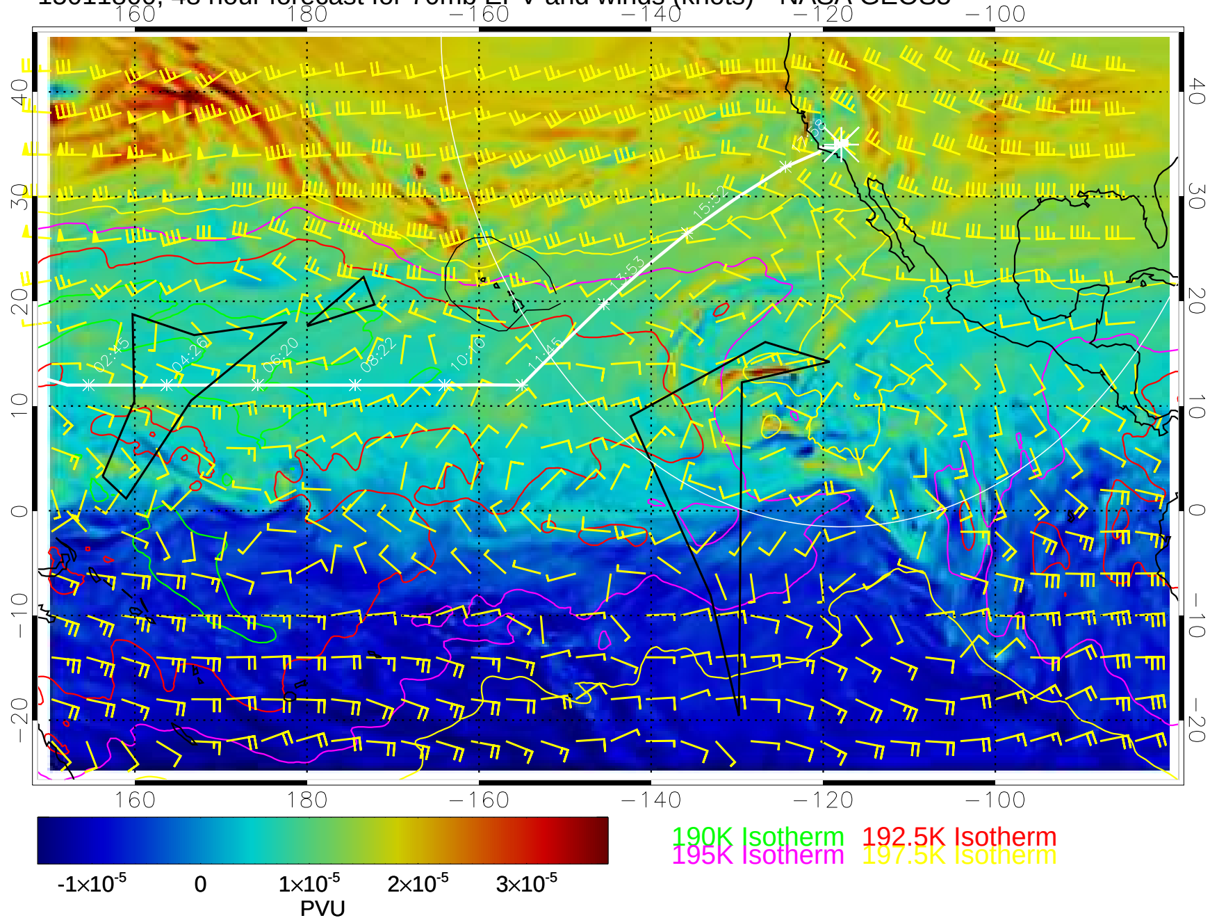
15011800, 48 hour forecast for 70mb EPV and winds (knots)-- NASA GEOS5
