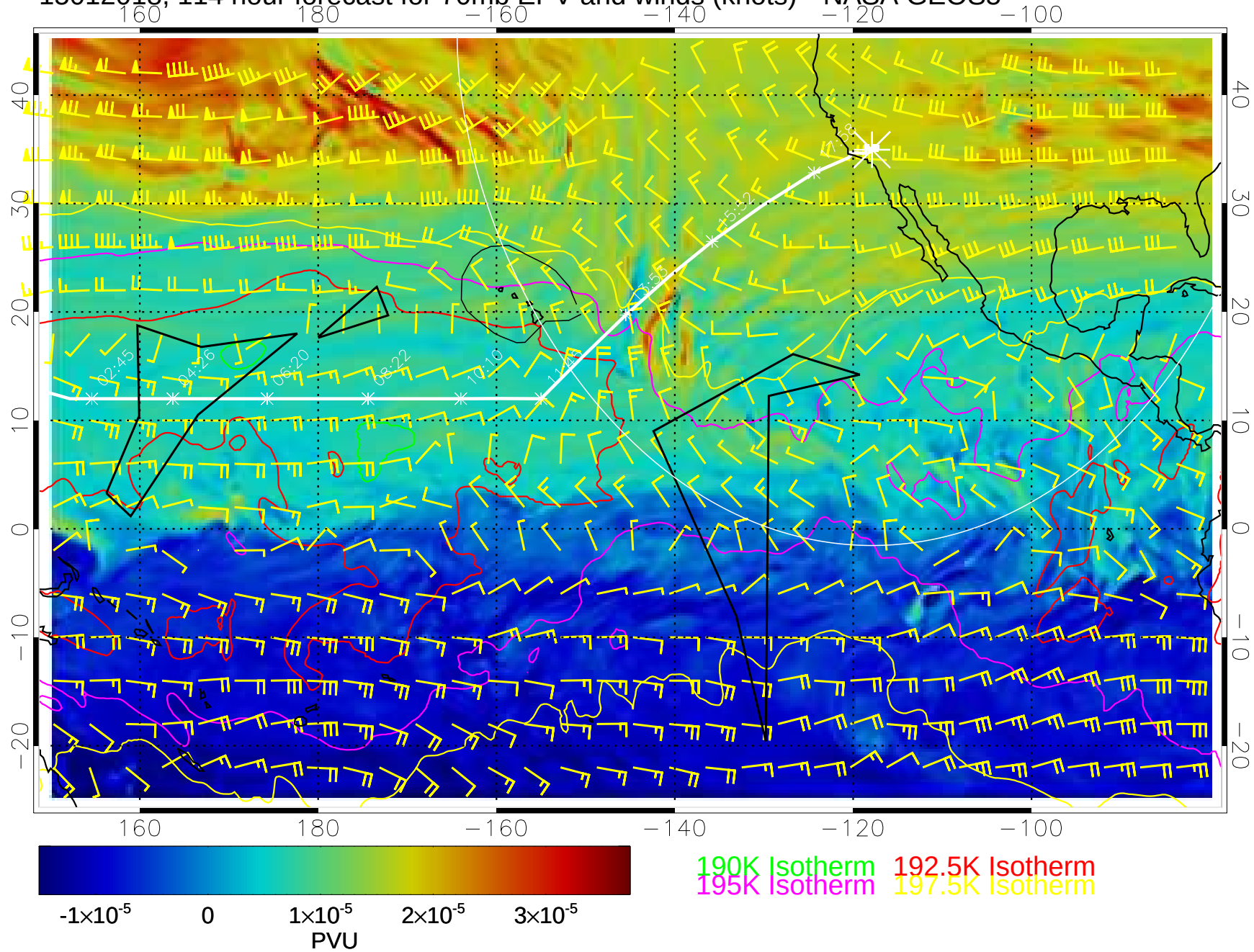
15012018, 114 hour forecast for 70mb EPV and winds (knots)-- NASA GEOS5
