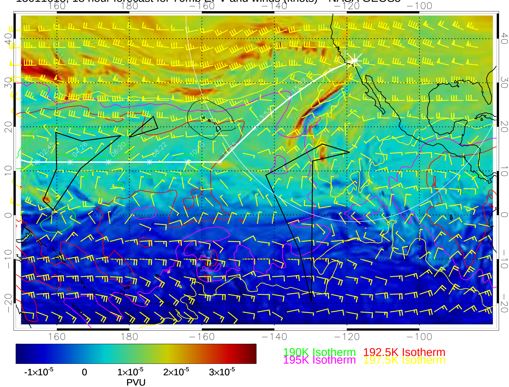
15011618, 18 hour forecast for 70mb EPV and winds (knots)-- NASA GEOS5
