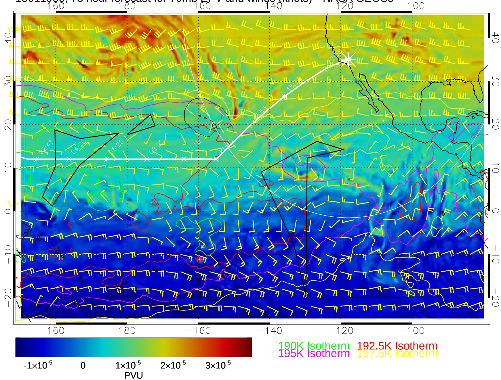
15011906, 78 hour forecast for 70mb EPV and winds (knots)-- NASA GEOS5
