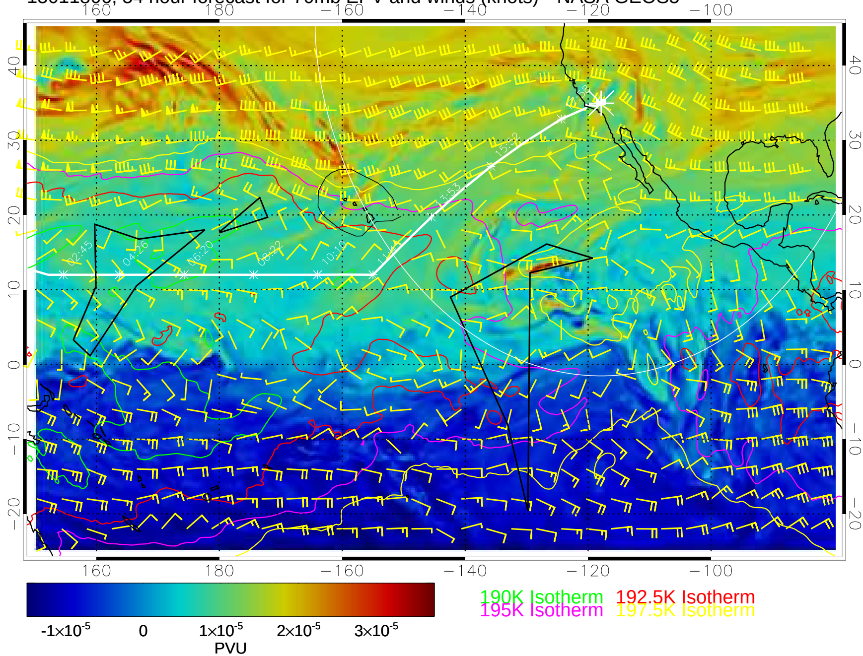
15011806, 54 hour forecast for 70mb EPV and winds (knots)-- NASA GEOS5
