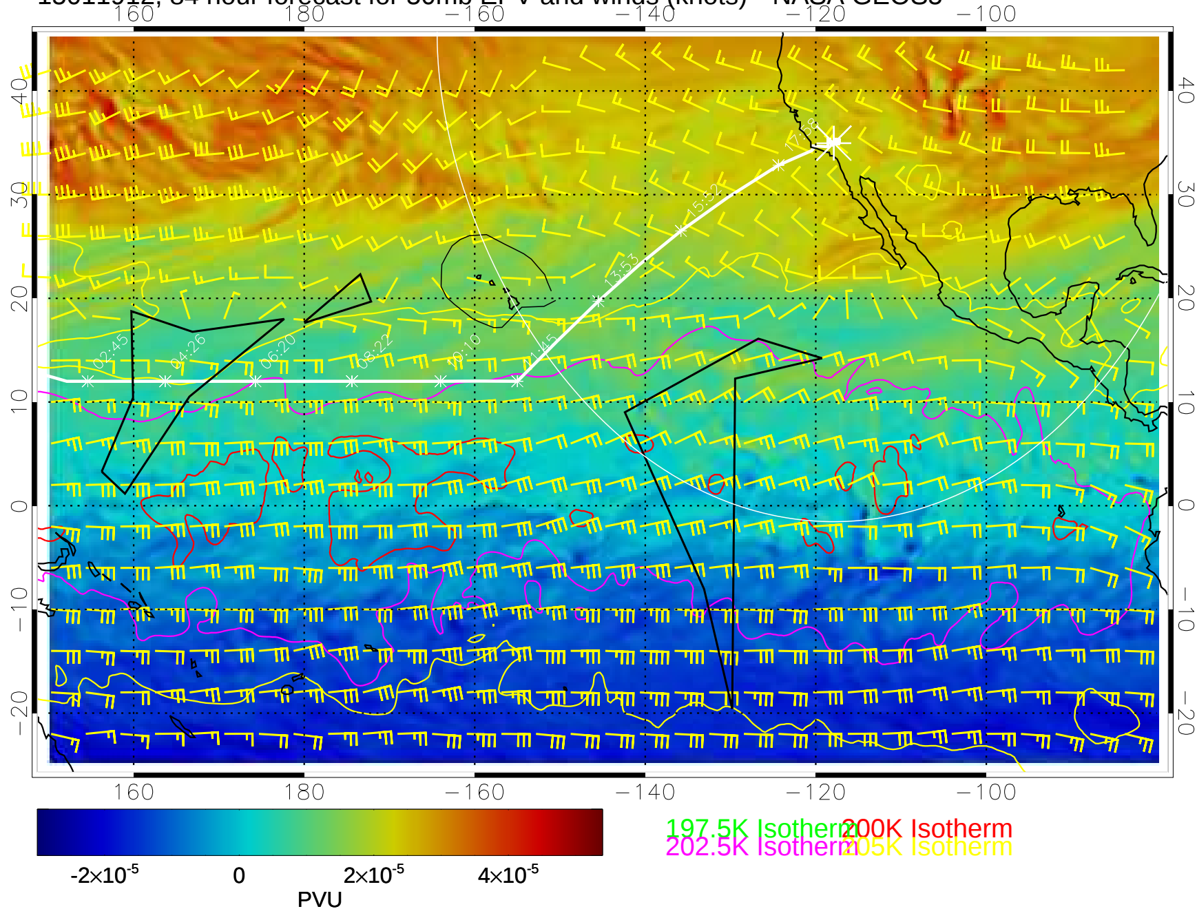
15011912, 84 hour forecast for 50mb EPV and winds (knots)-- NASA GEOS5
