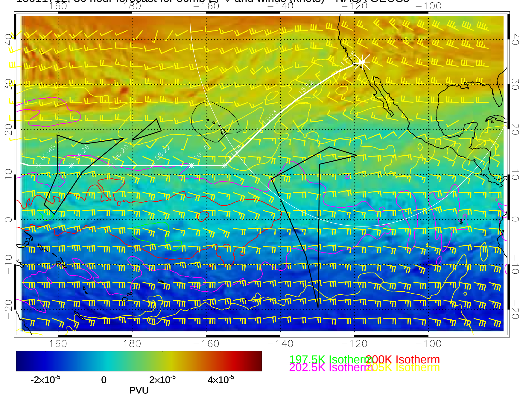
15011712, 36 hour forecast for 50mb EPV and winds (knots)-- NASA GEOS5
