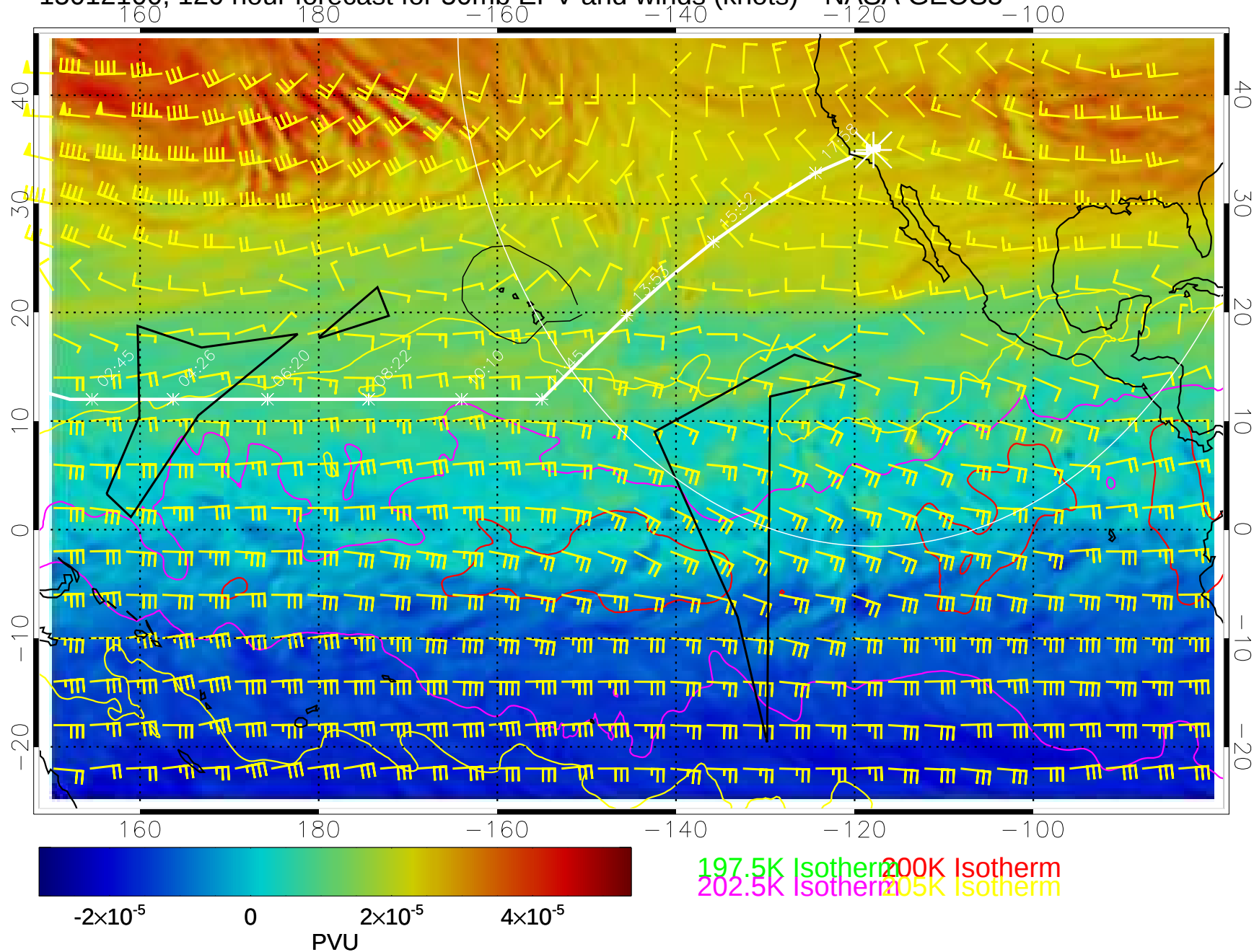
15012100, 120 hour forecast for 50mb EPV and winds (knots)-- NASA GEOS5
