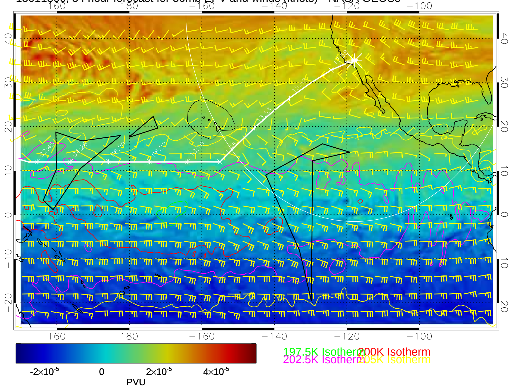
15011806, 54 hour forecast for 50mb EPV and winds (knots)-- NASA GEOS5
