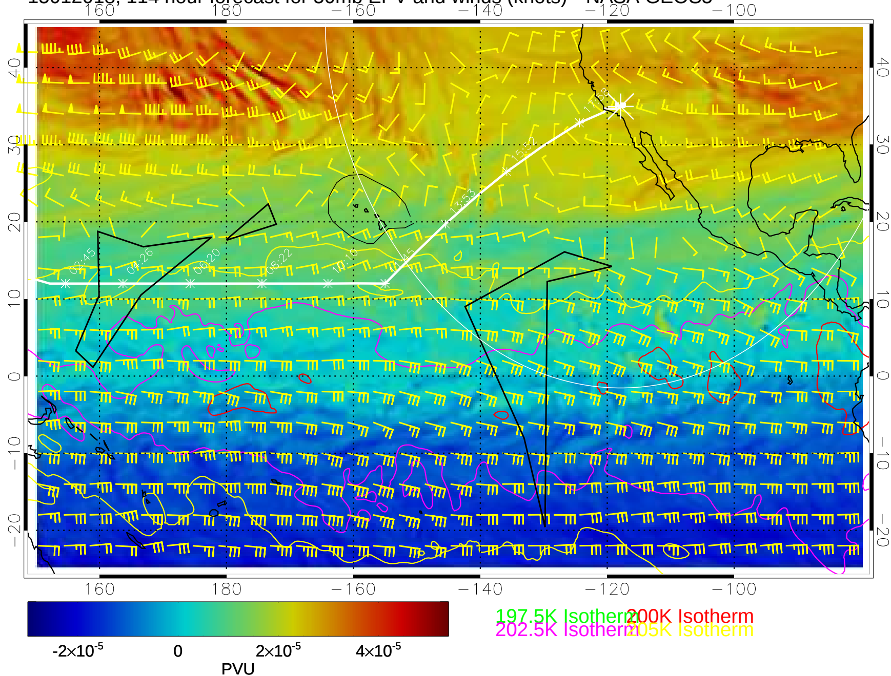
15012018, 114 hour forecast for 50mb EPV and winds (knots)-- NASA GEOS5
