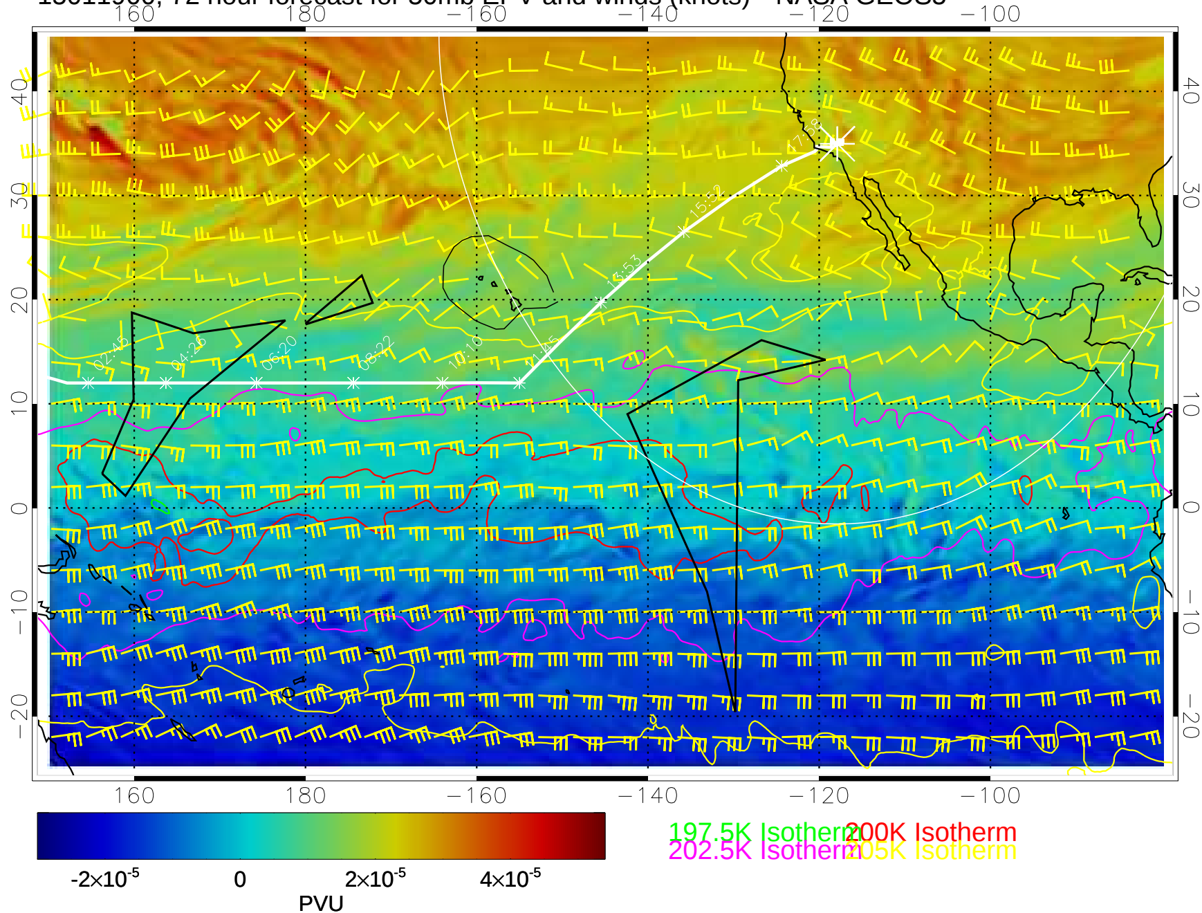
15011900, 72 hour forecast for 50mb EPV and winds (knots)-- NASA GEOS5
