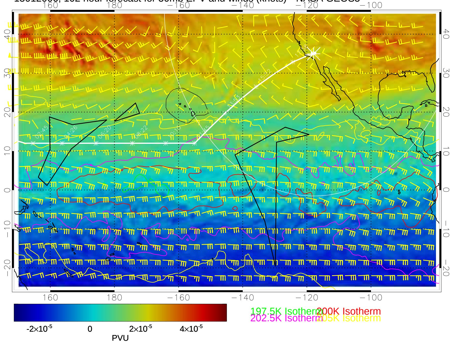
15012006, 102 hour forecast for 50mb EPV and winds (knots)-- NASA GEOS5
