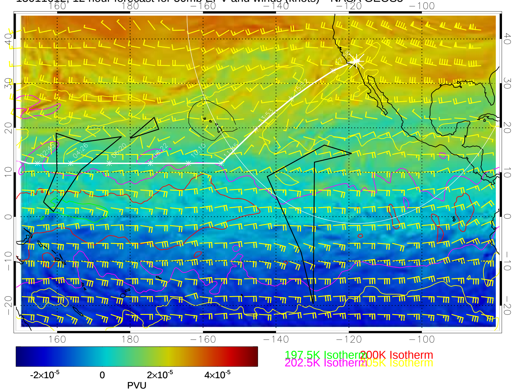
15011612, 12 hour forecast for 50mb EPV and winds (knots)-- NASA GEOS5
