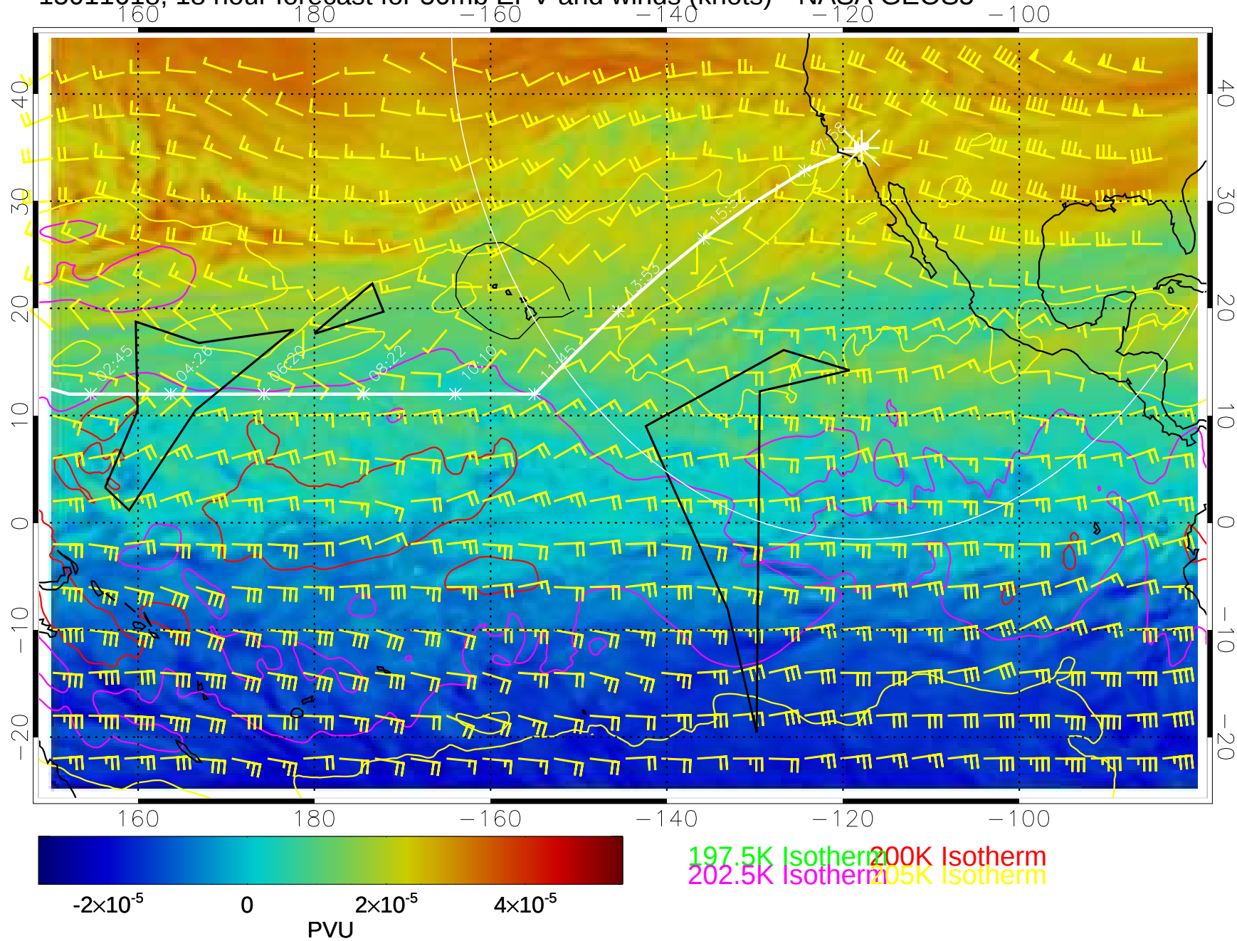
15011618, 18 hour forecast for 50mb EPV and winds (knots)-- NASA GEOS5
